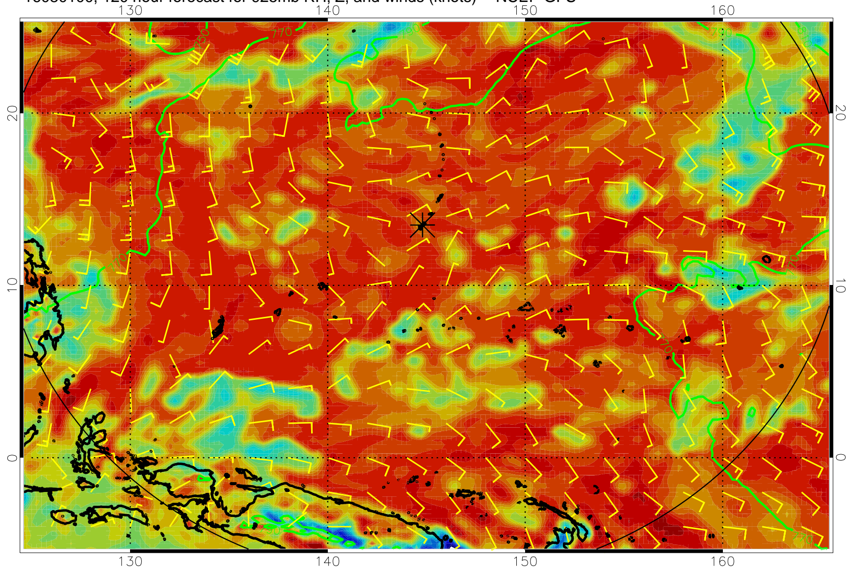
16080100, 120 hour forecast for 925mb RH, Z, and winds (knots) -- NCEP GFS
