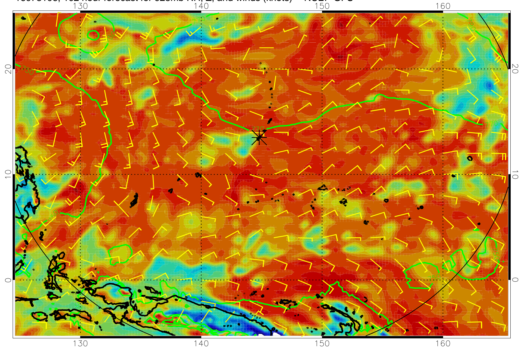
16073106, 102 hour forecast for 925mb RH, Z, and winds (knots) -- NCEP GFS
