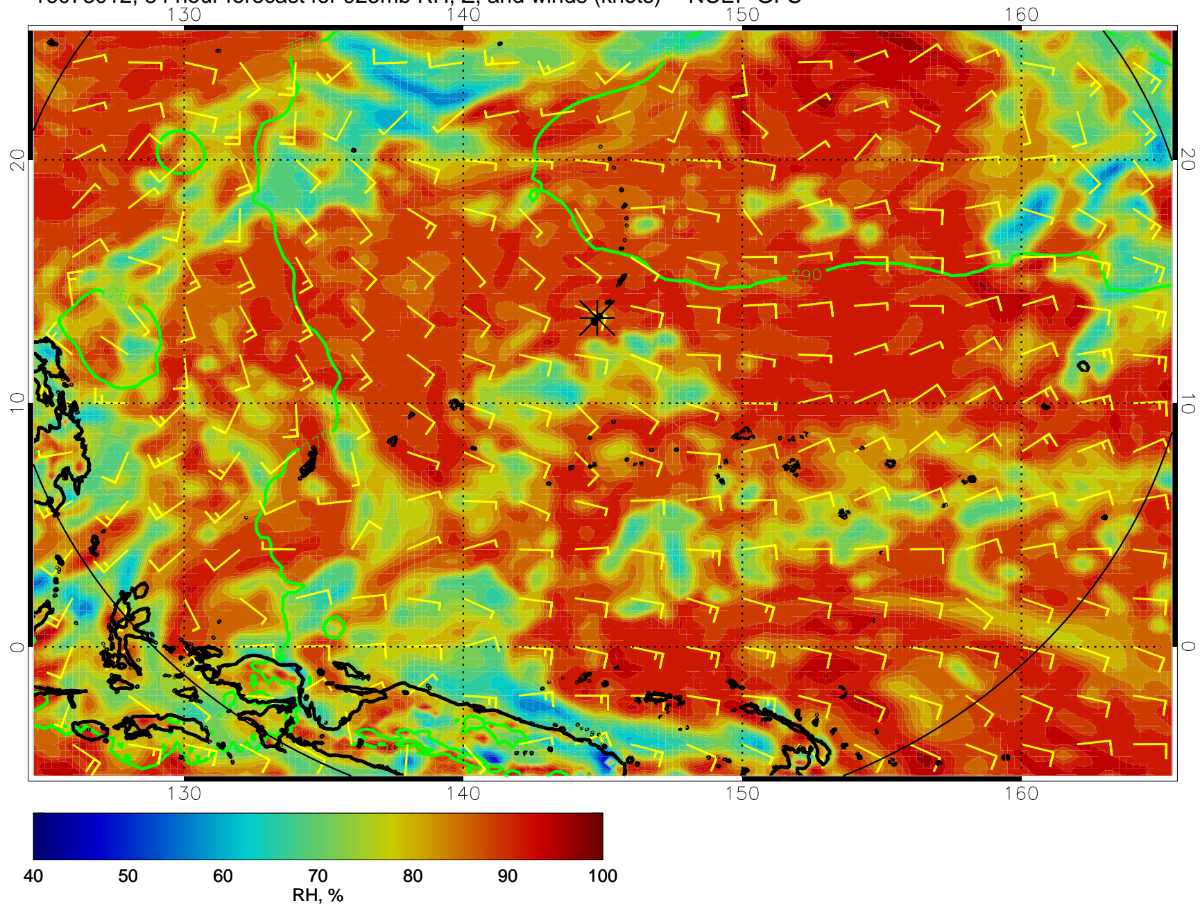
16073012, 84 hour forecast for 925mb RH, Z, and winds (knots) -- NCEP GFS
