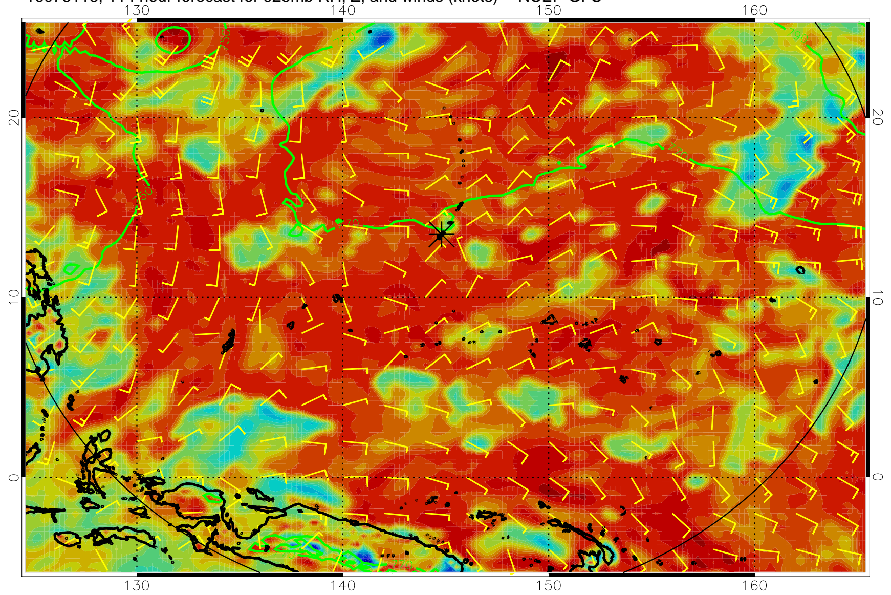
16073118, 114 hour forecast for 925mb RH, Z, and winds (knots) -- NCEP GFS
