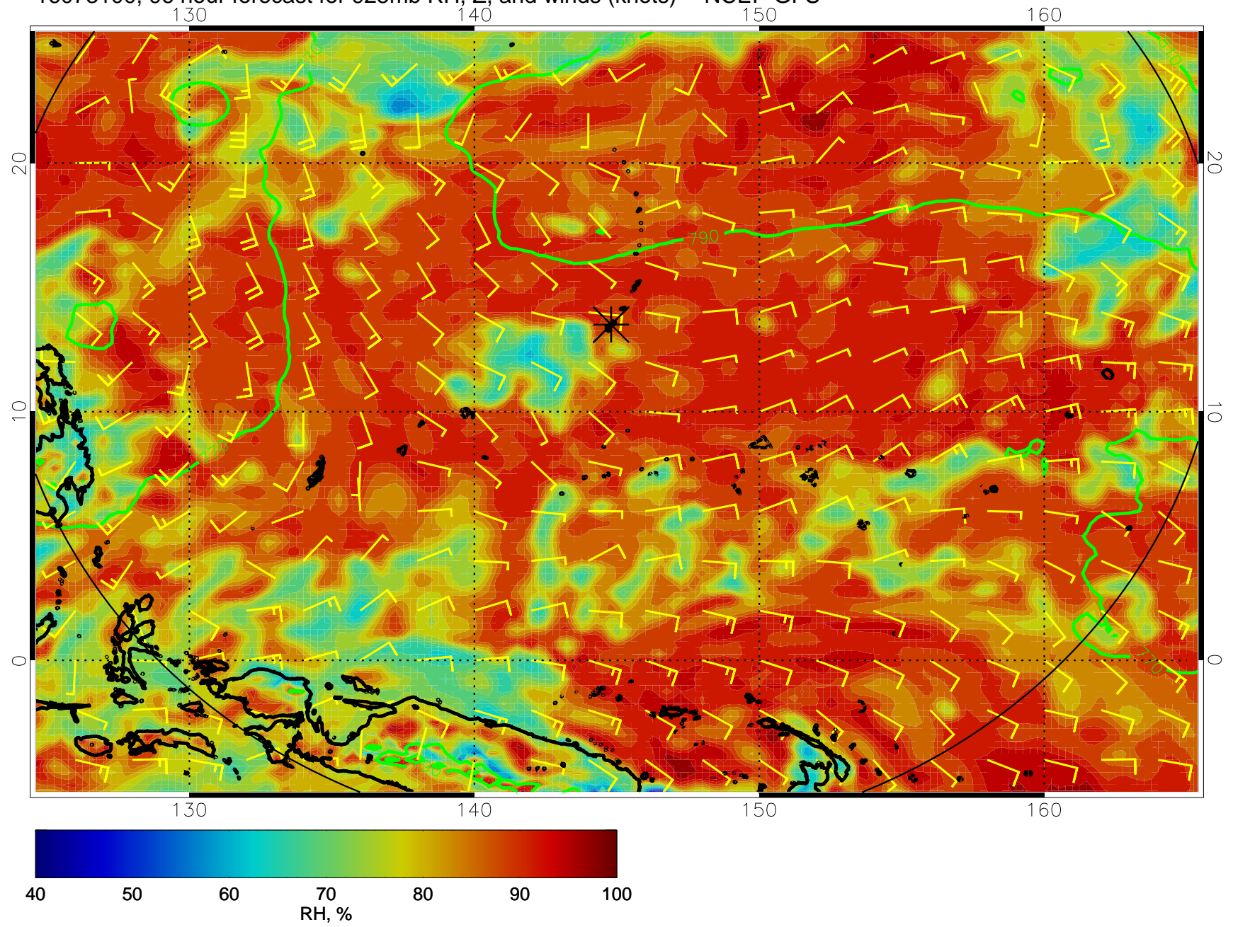
16073100, 96 hour forecast for 925mb RH, Z, and winds (knots) -- NCEP GFS
