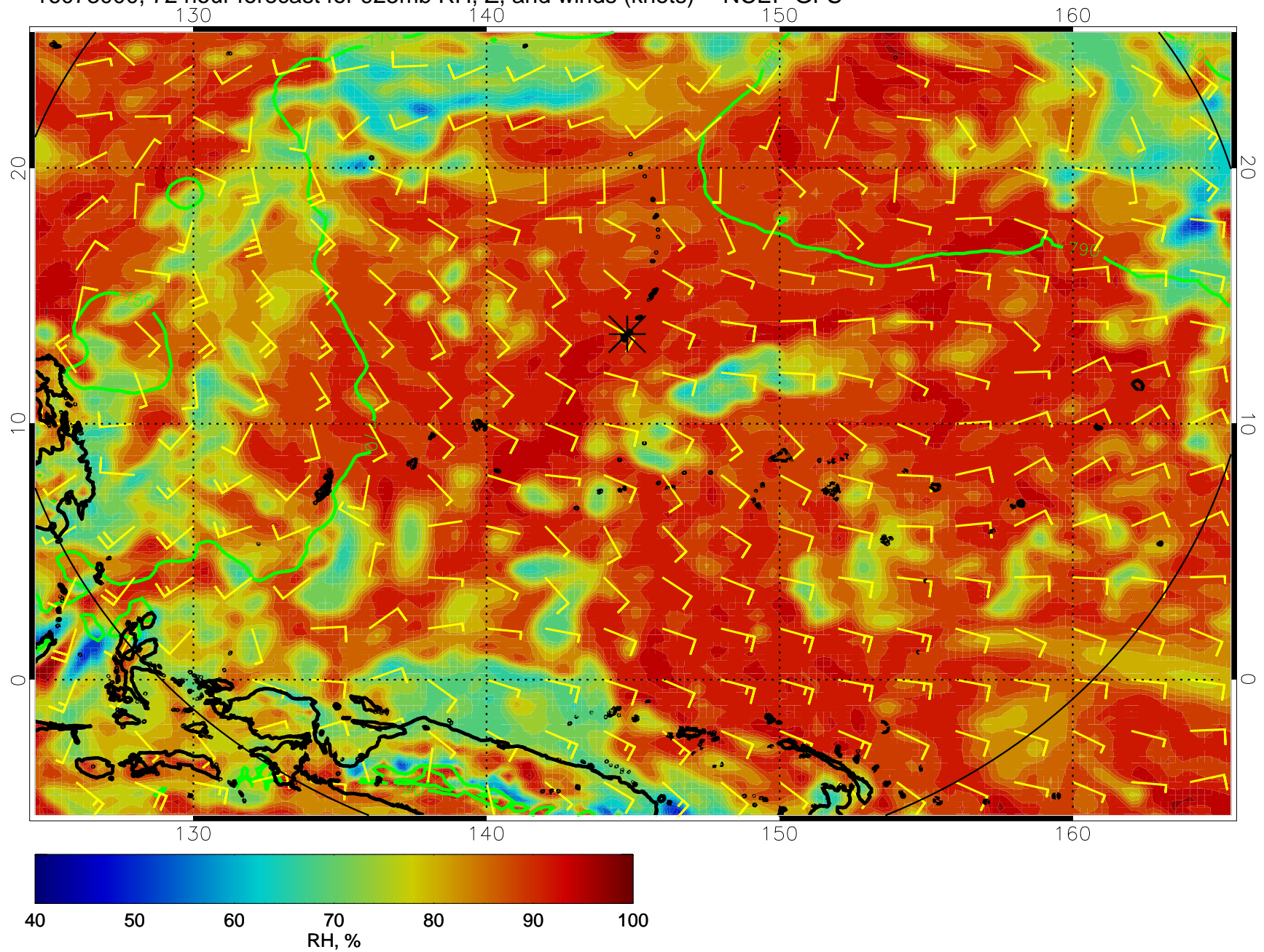
16073000, 72 hour forecast for 925mb RH, Z, and winds (knots) -- NCEP GFS
