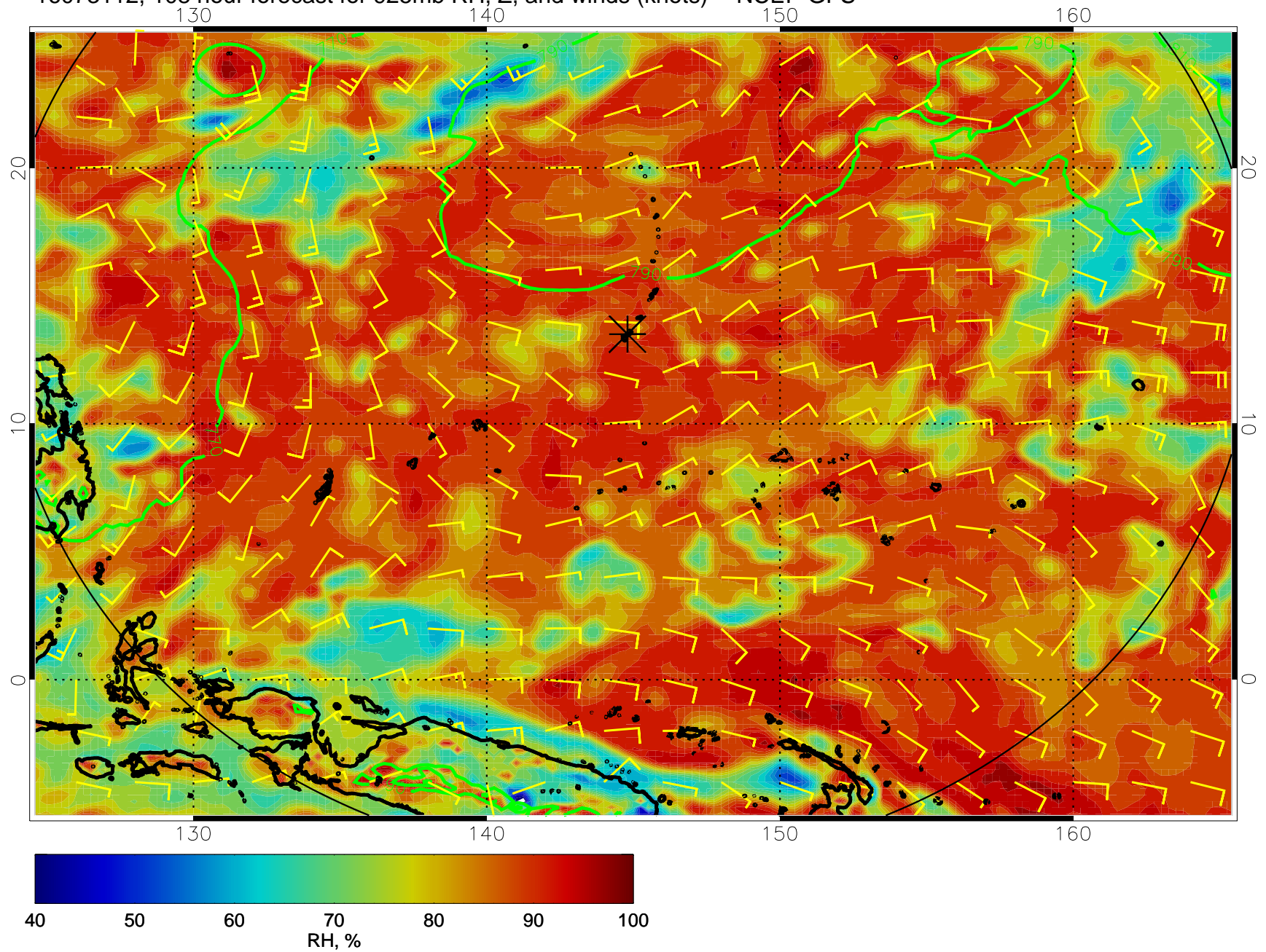
16073112, 108 hour forecast for 925mb RH, Z, and winds (knots) -- NCEP GFS
