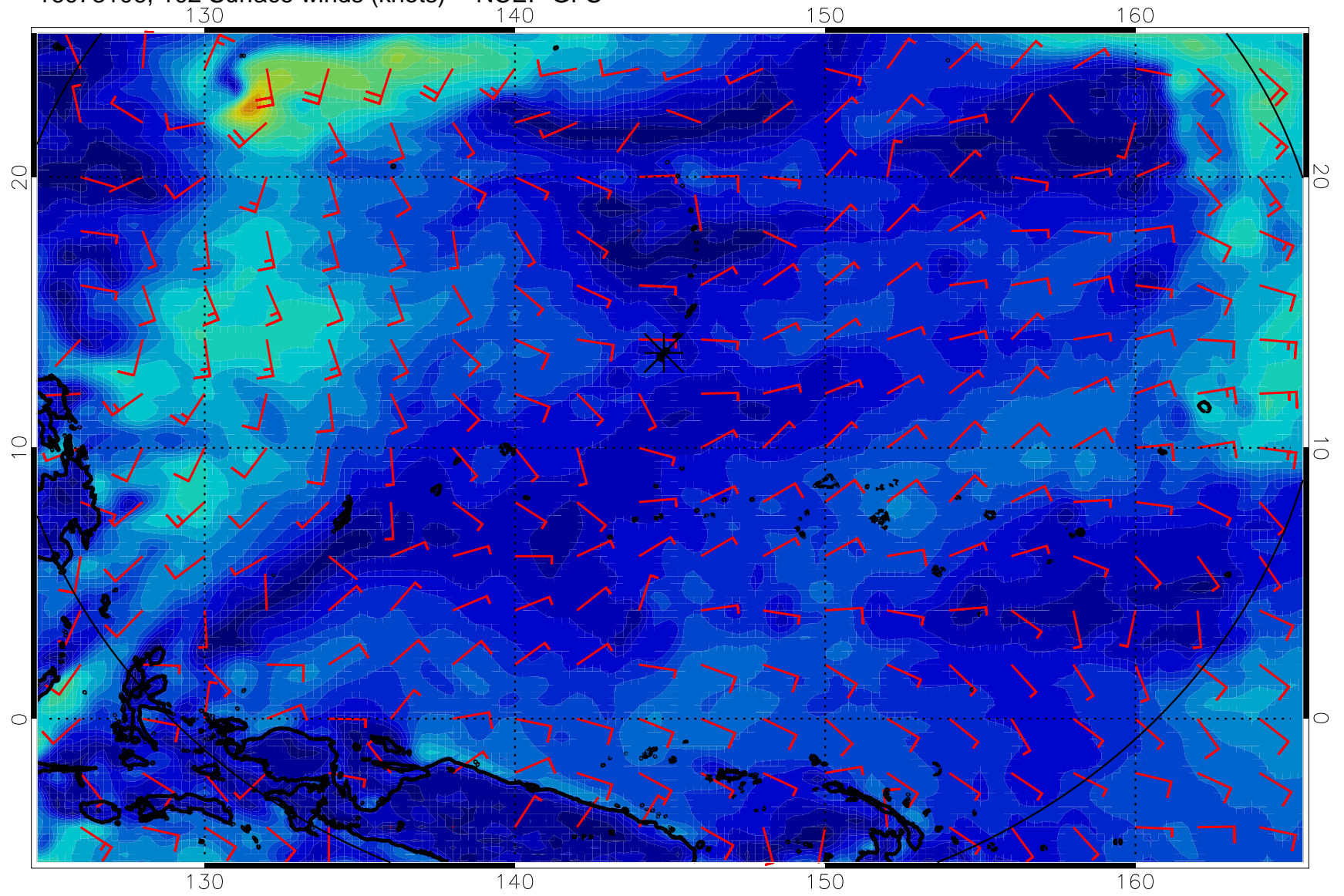
16073106, 102 Surface winds (knots) -- NCEP GFS
