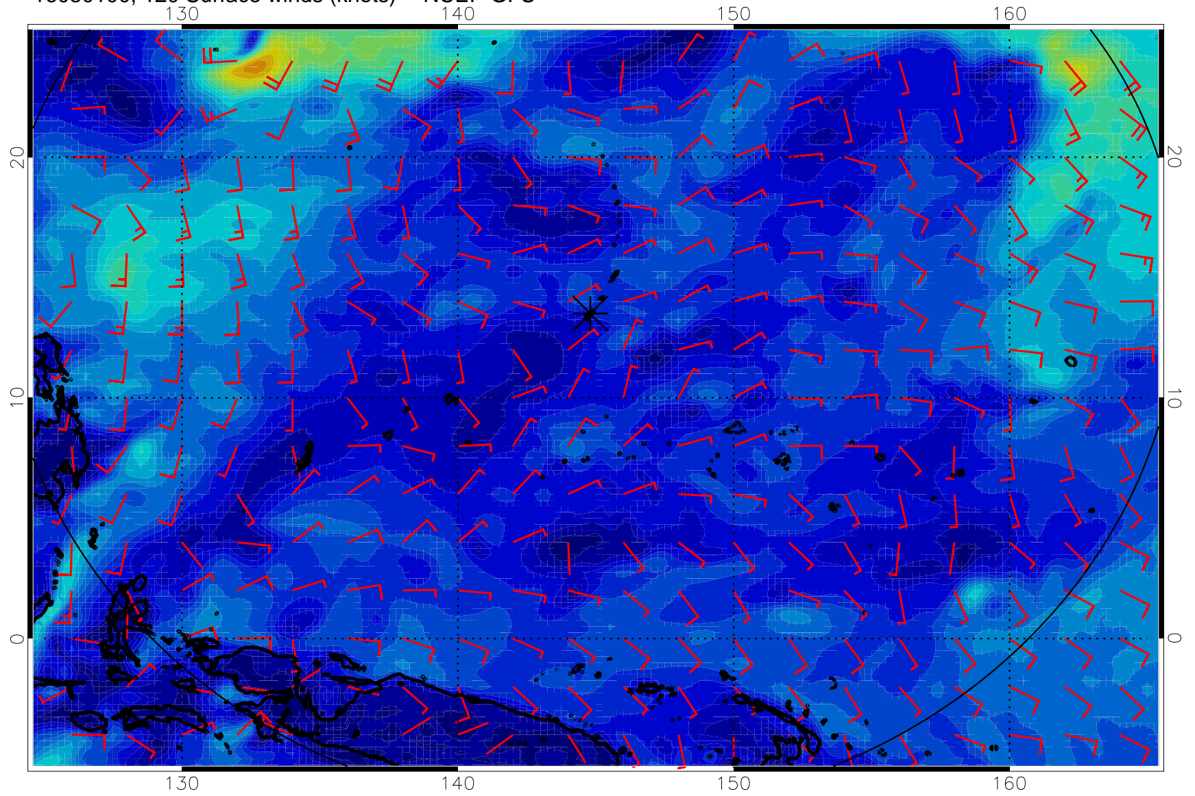
16080100, 120 Surface winds (knots) -- NCEP GFS
