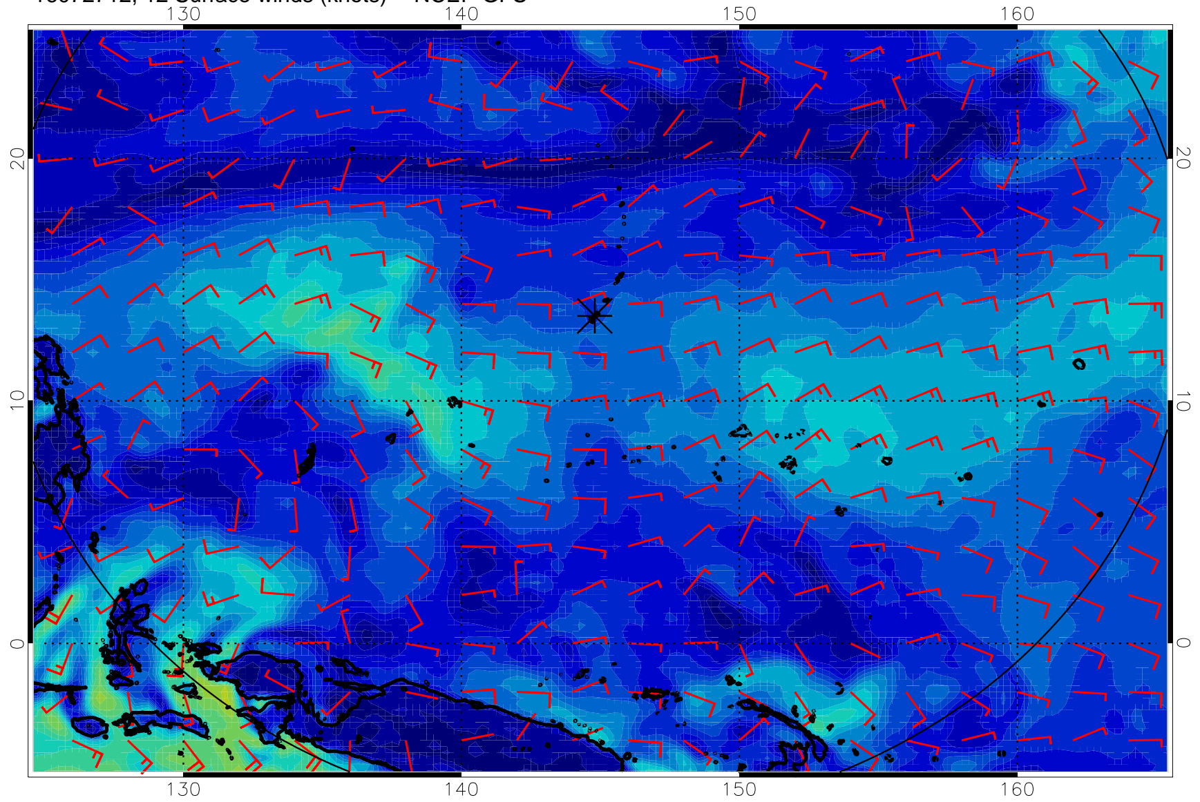
16072712, 12 Surface winds (knots) -- NCEP GFS
