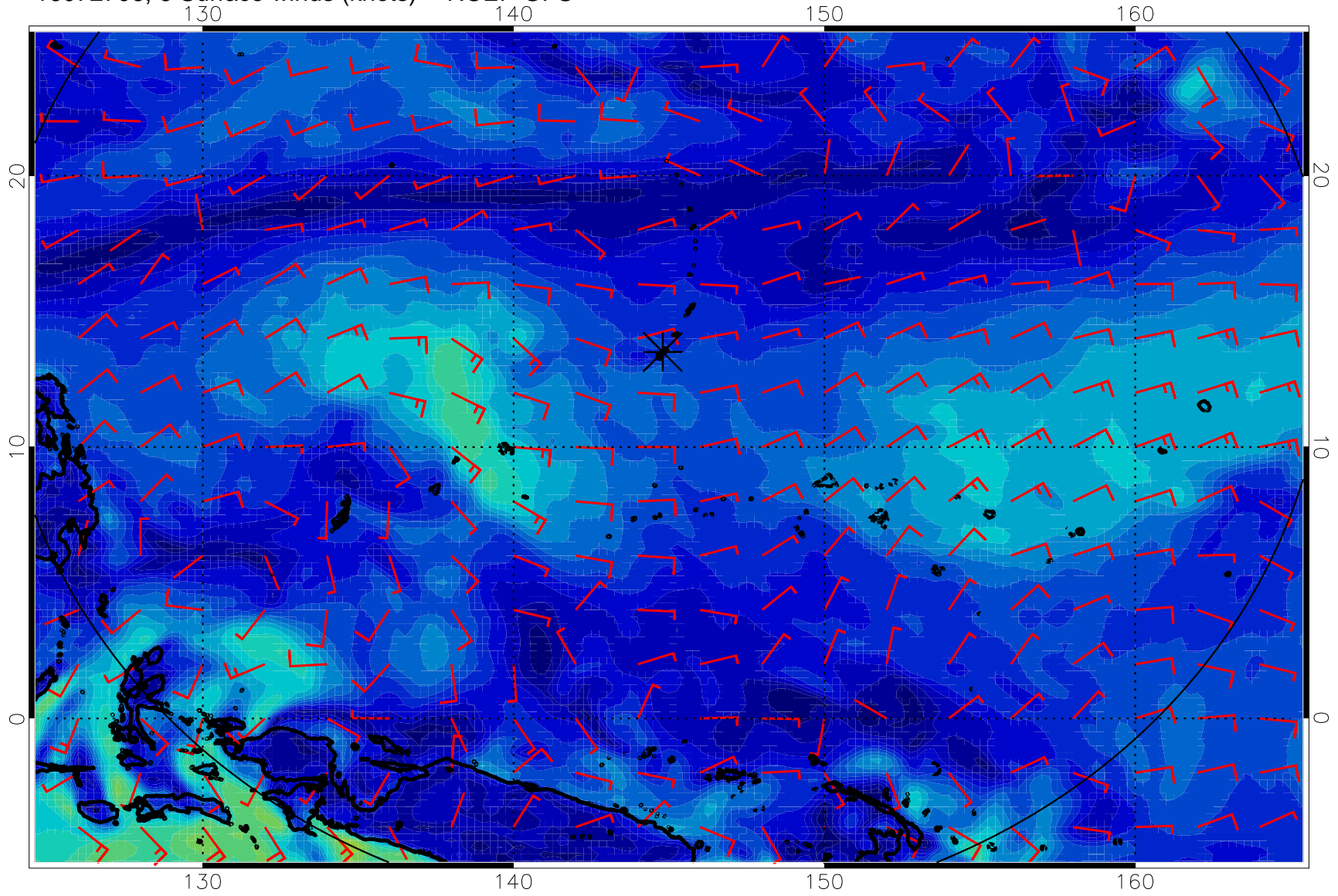
16072706, 6 Surface winds (knots) -- NCEP GFS
