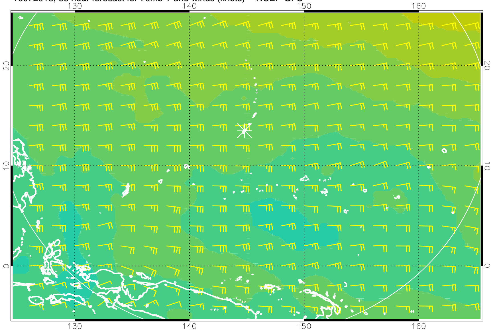
16072918, 66 hour forecast for 70mb T and winds (knots) -- NCEP GFS
