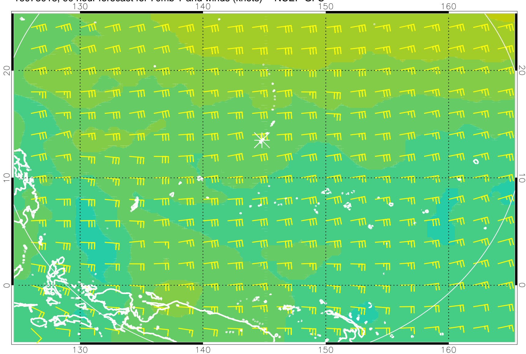
16073018, 90 hour forecast for 70mb T and winds (knots) -- NCEP GFS
