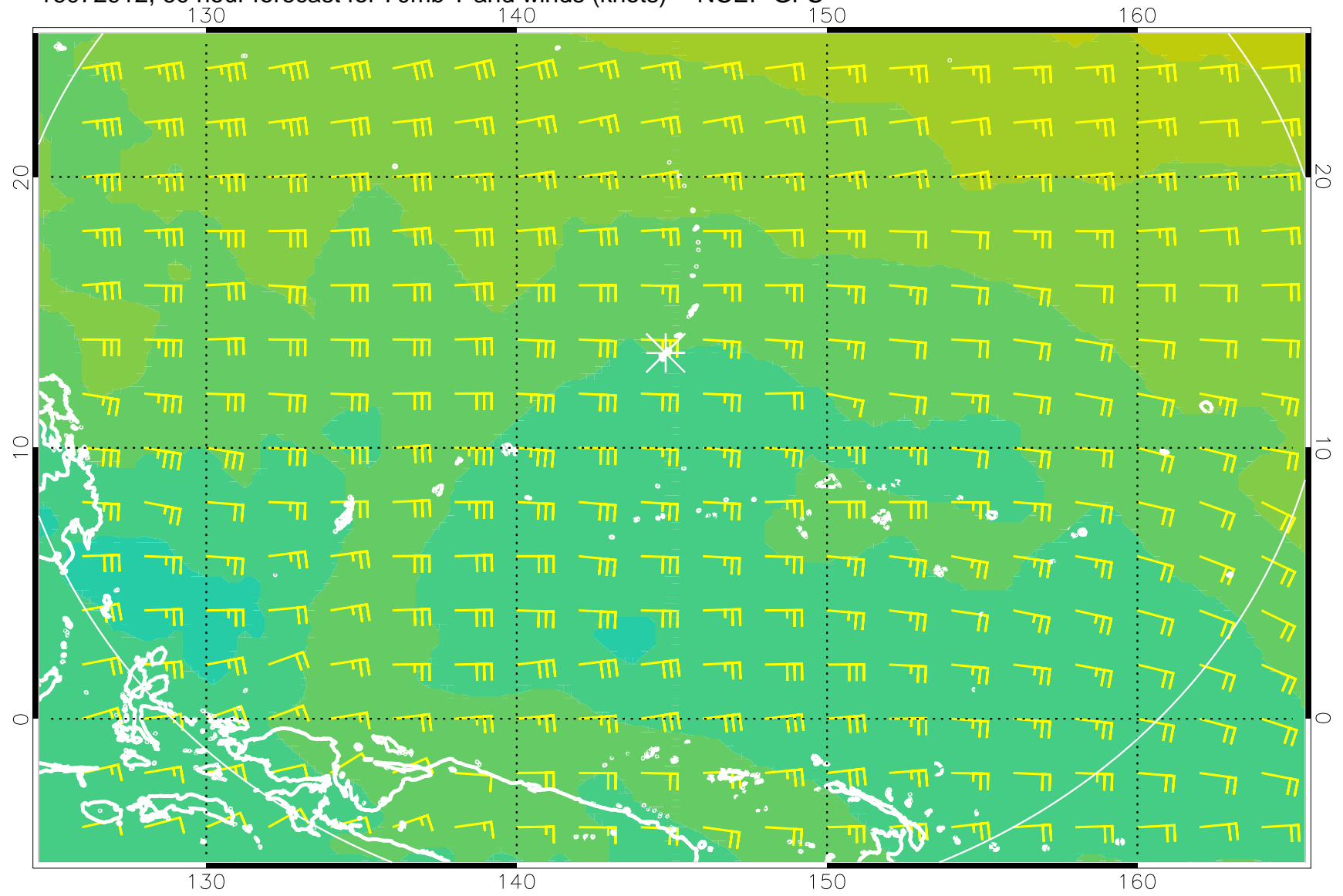
16072912, 60 hour forecast for 70mb T and winds (knots) -- NCEP GFS
