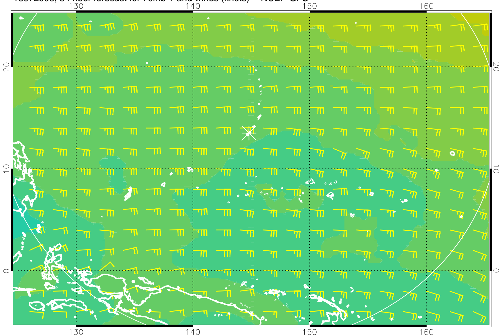
16072906, 54 hour forecast for 70mb T and winds (knots) -- NCEP GFS
