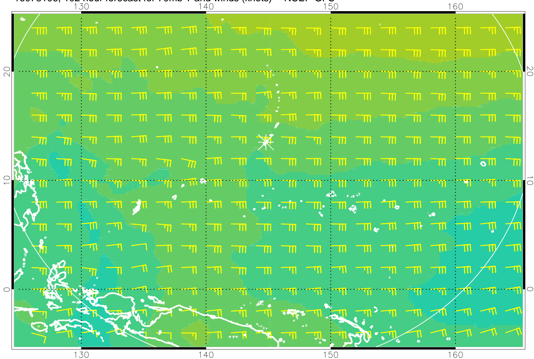
16073106, 102 hour forecast for 70mb T and winds (knots) -- NCEP GFS
