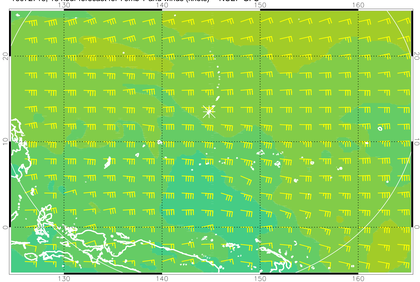
16072718, 18 hour forecast for 70mb T and winds (knots) -- NCEP GFS
