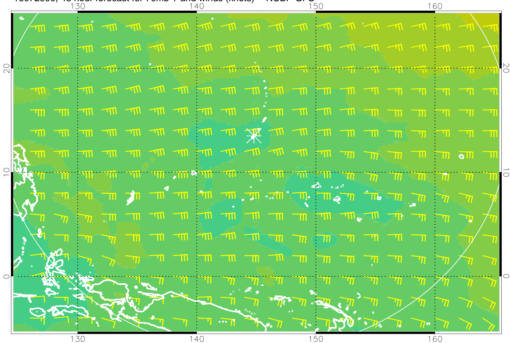
16072900, 48 hour forecast for 70mb T and winds (knots) -- NCEP GFS
