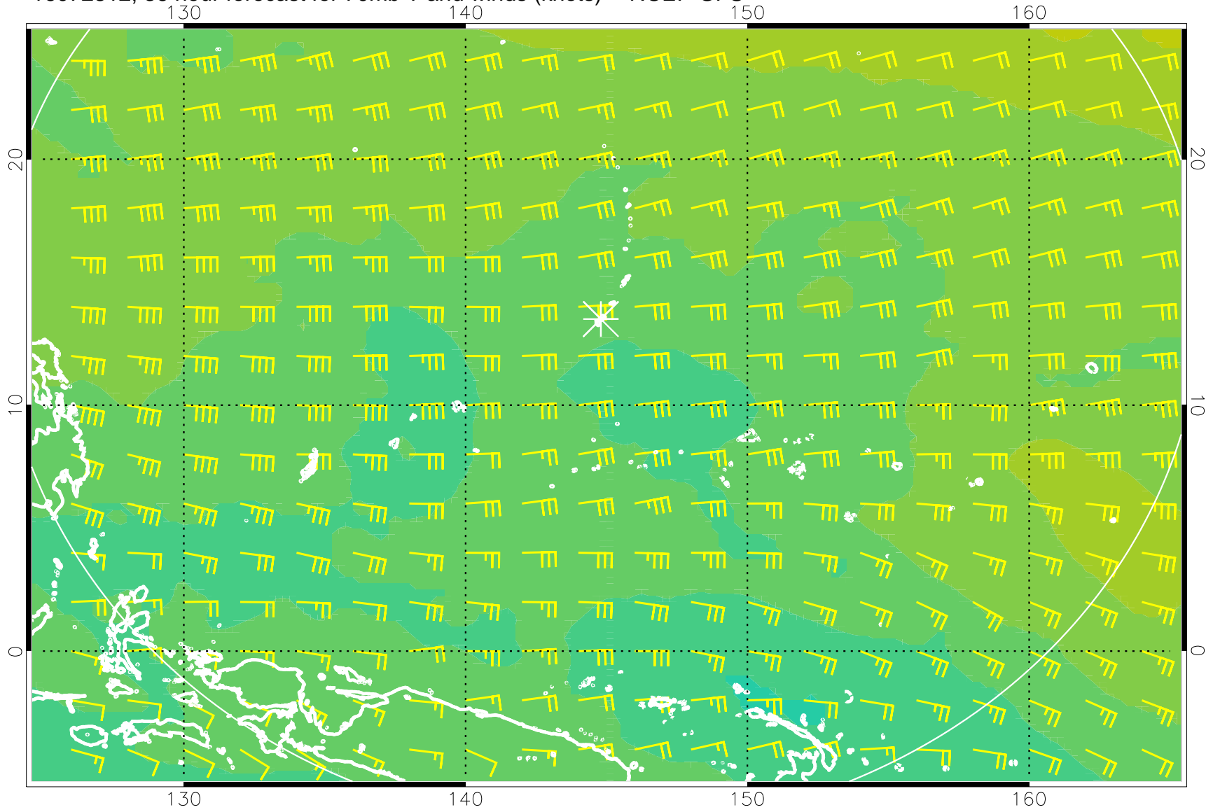
16072812, 36 hour forecast for 70mb T and winds (knots) -- NCEP GFS
