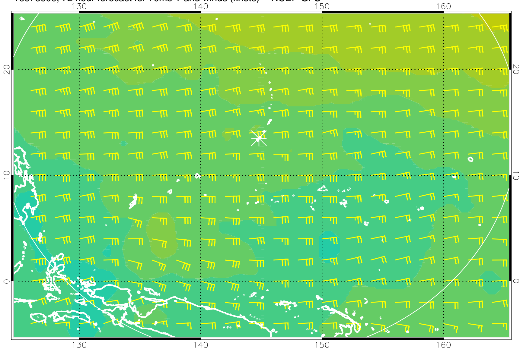
16073000, 72 hour forecast for 70mb T and winds (knots) -- NCEP GFS
