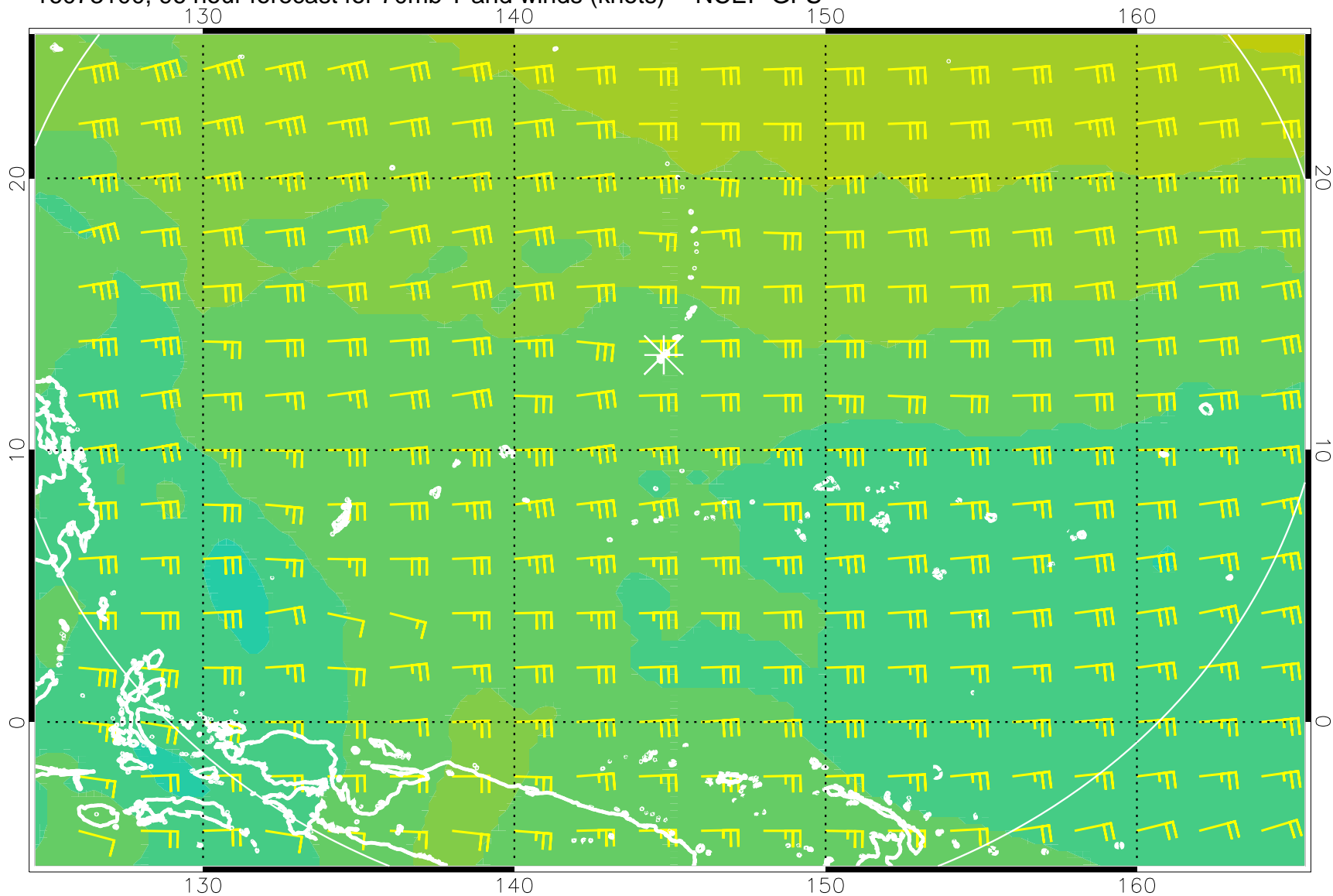
16073100, 96 hour forecast for 70mb T and winds (knots) -- NCEP GFS
