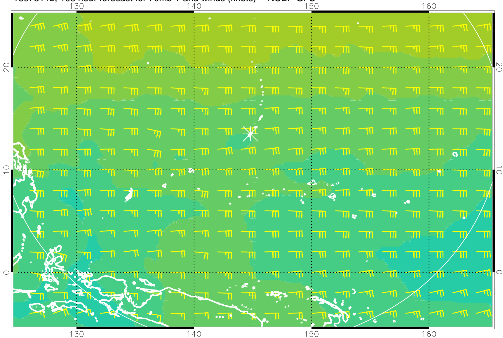
16073112, 108 hour forecast for 70mb T and winds (knots) -- NCEP GFS
