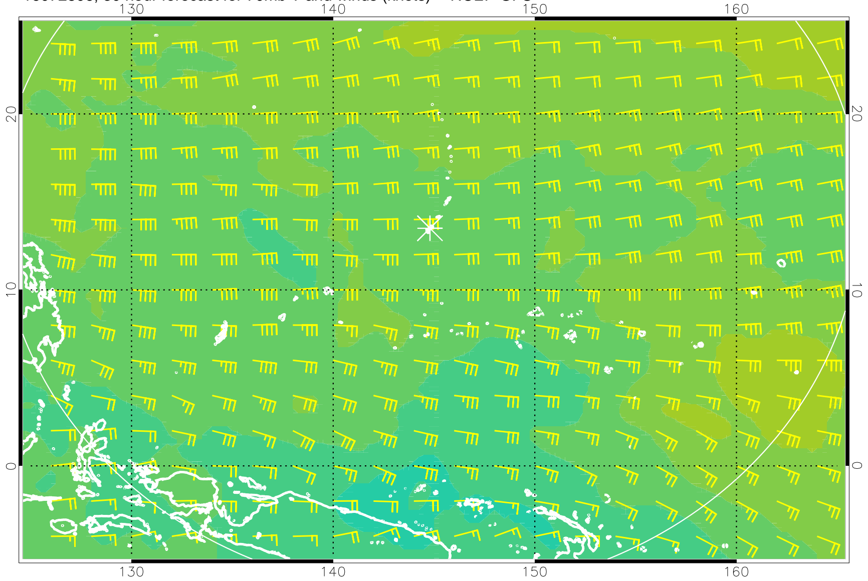
16072806, 30 hour forecast for 70mb T and winds (knots) -- NCEP GFS
