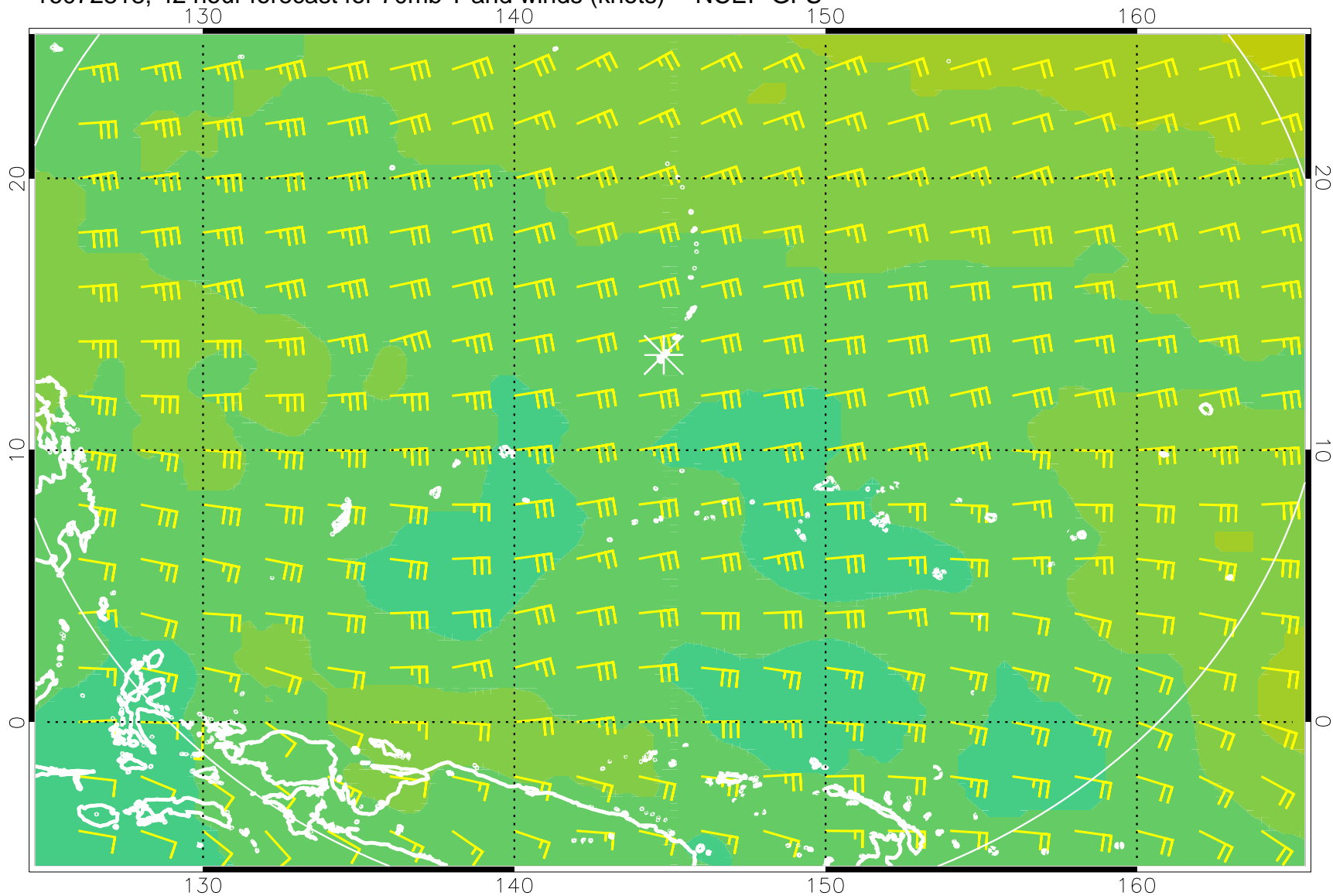
16072818, 42 hour forecast for 70mb T and winds (knots) -- NCEP GFS
