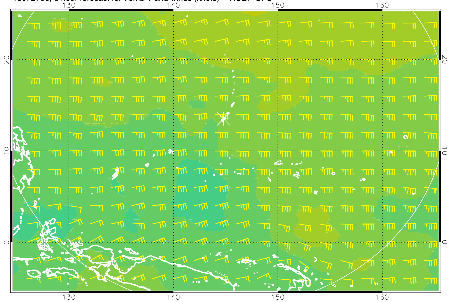
16072706, 6 hour forecast for 70mb T and winds (knots) -- NCEP GFS
