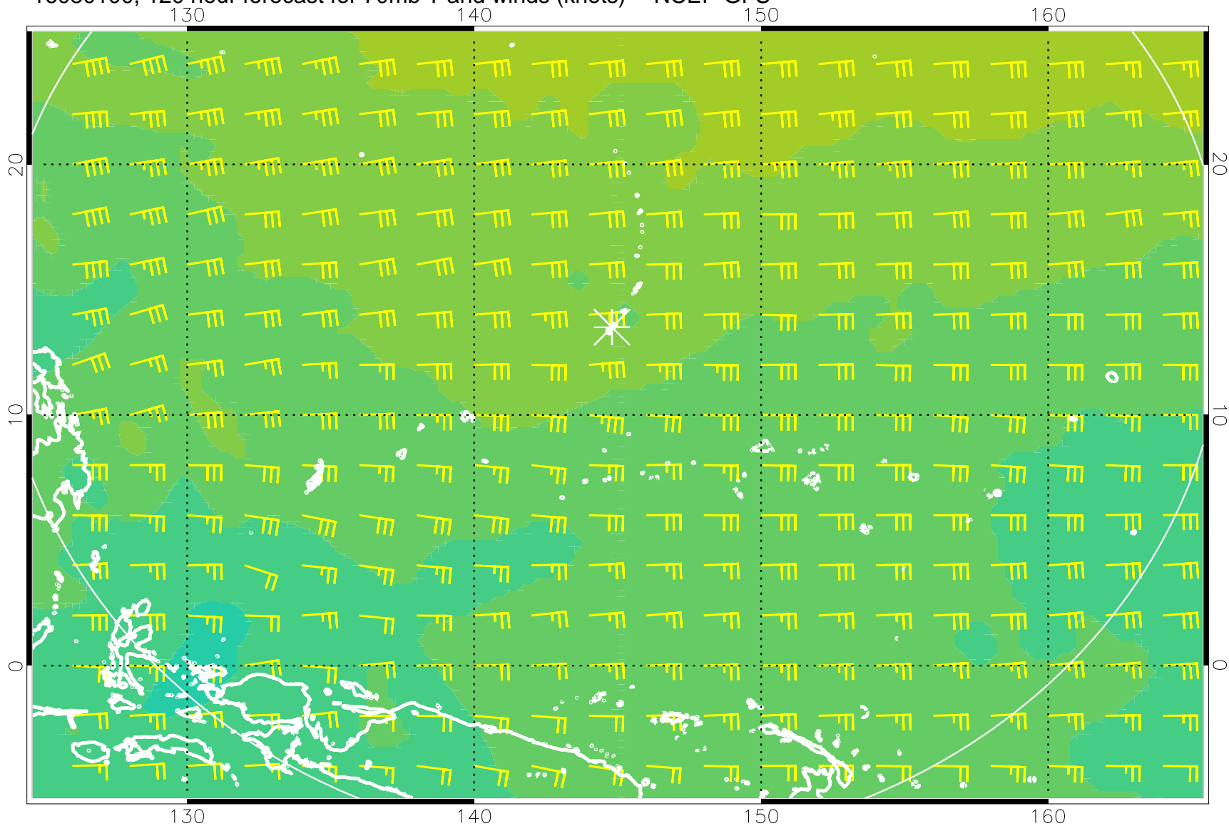
16080100, 120 hour forecast for 70mb T and winds (knots) -- NCEP GFS
