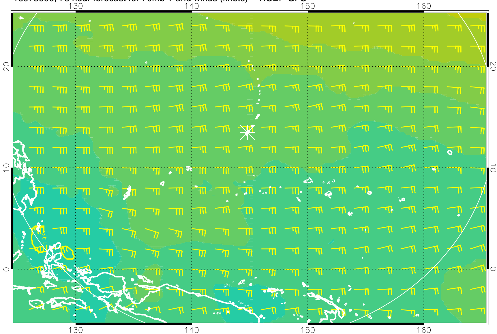
16073006, 78 hour forecast for 70mb T and winds (knots) -- NCEP GFS
