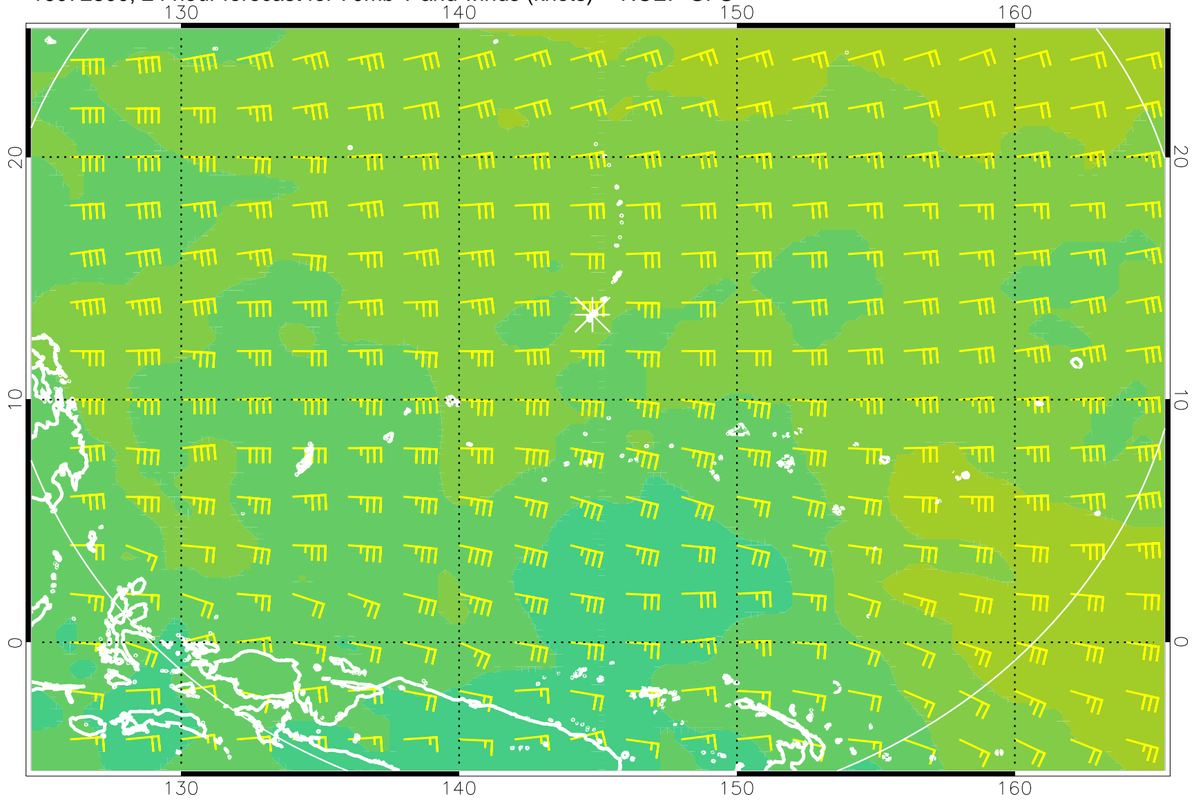
16072800, 24 hour forecast for 70mb T and winds (knots) -- NCEP GFS
