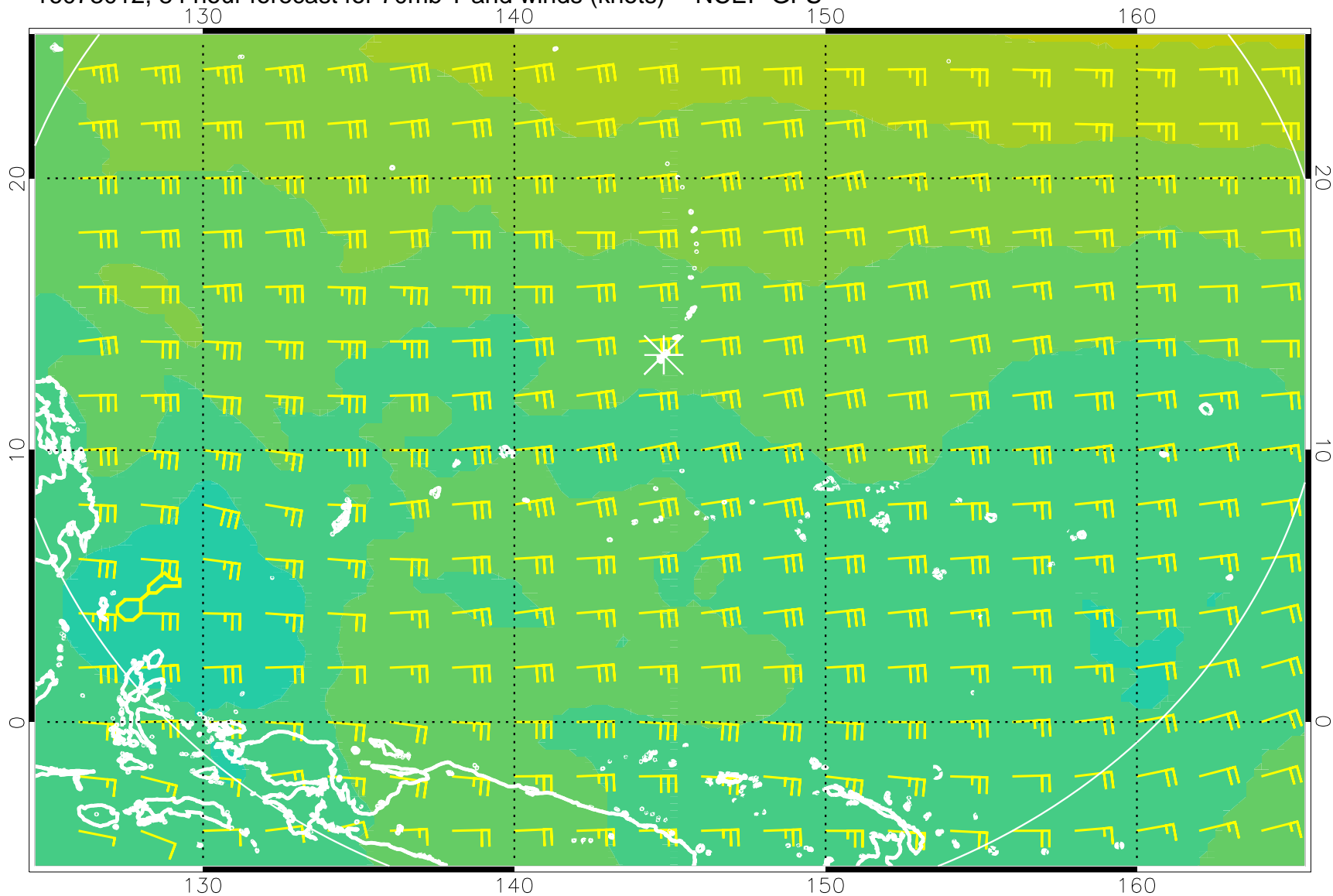
16073012, 84 hour forecast for 70mb T and winds (knots) -- NCEP GFS
