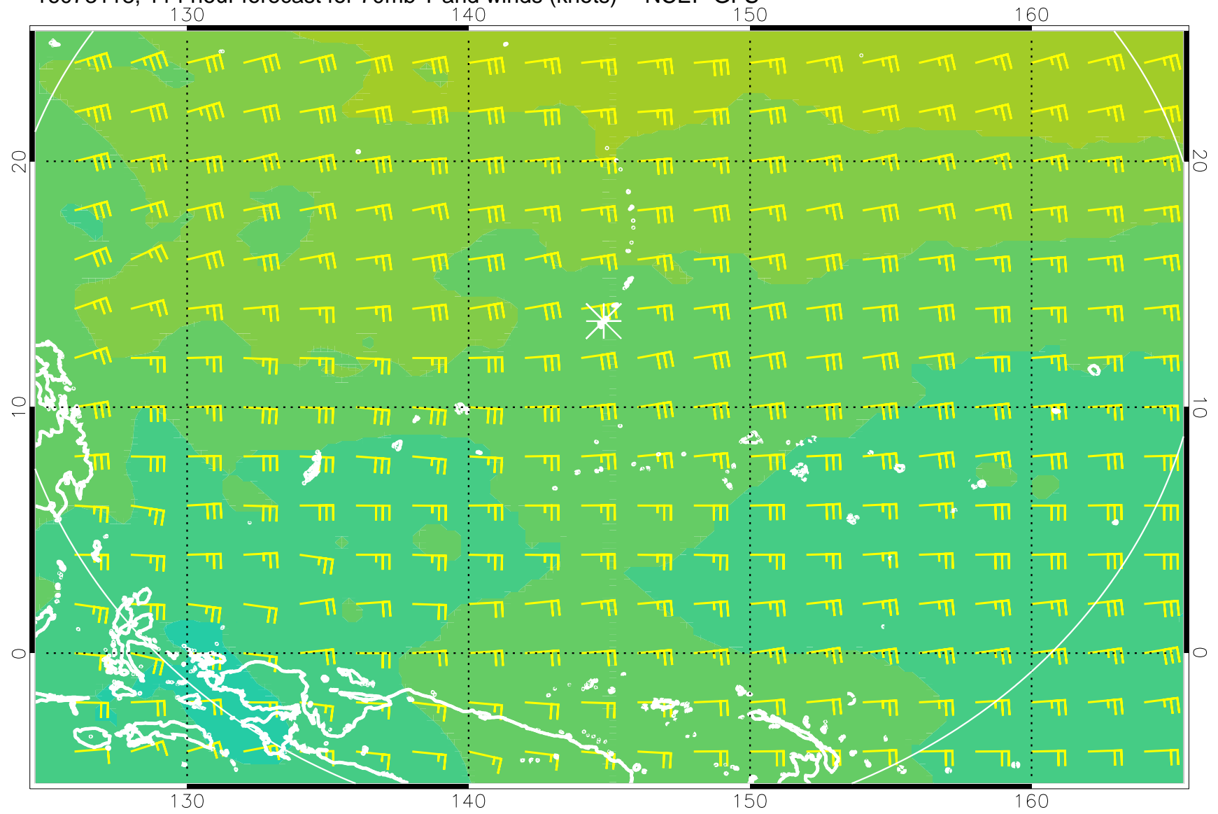
16073118, 114 hour forecast for 70mb T and winds (knots) -- NCEP GFS
