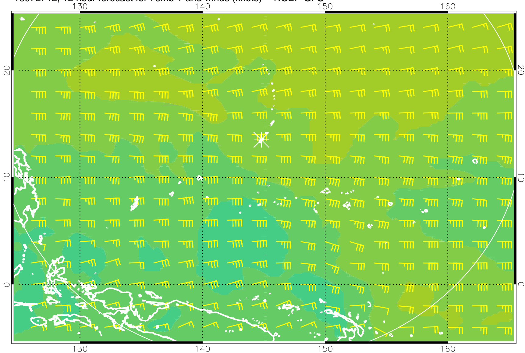
16072712, 12 hour forecast for 70mb T and winds (knots) -- NCEP GFS
