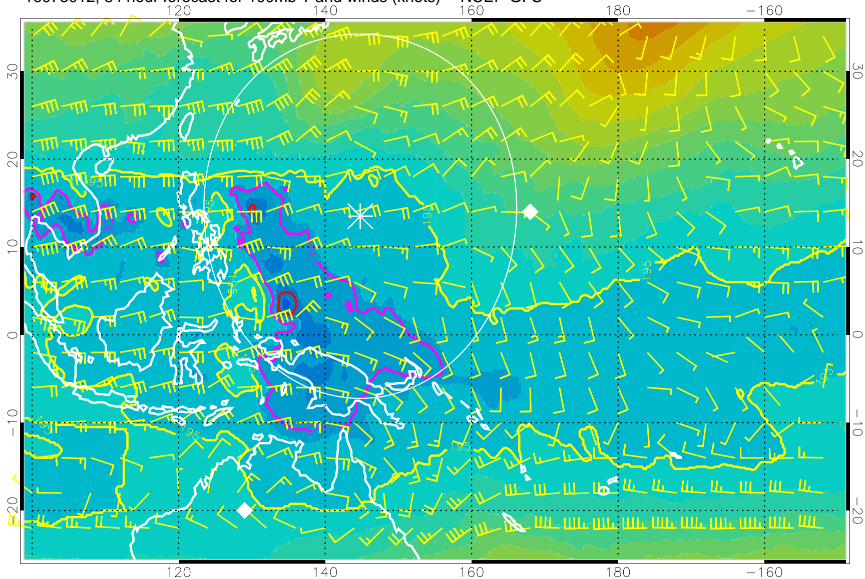
16073012, 84 hour forecast for 100mb T and winds (knots) -- NCEP GFS
