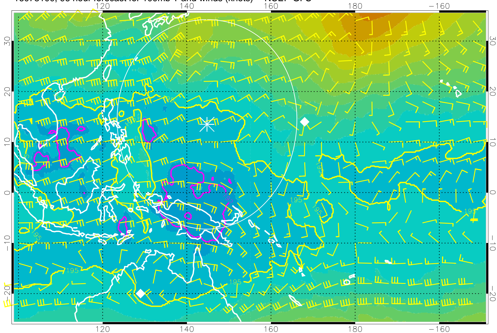
16073100, 96 hour forecast for 100mb T and winds (knots) -- NCEP GFS
