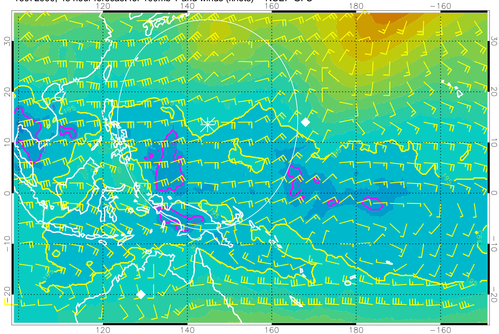
16072900, 48 hour forecast for 100mb T and winds (knots) -- NCEP GFS
