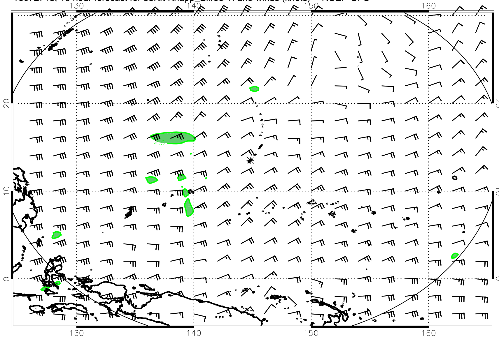
16072718, 18 hour forecast for 53Kft Knapp_Ellrod TI and winds (knots) -- NCEP GFS
