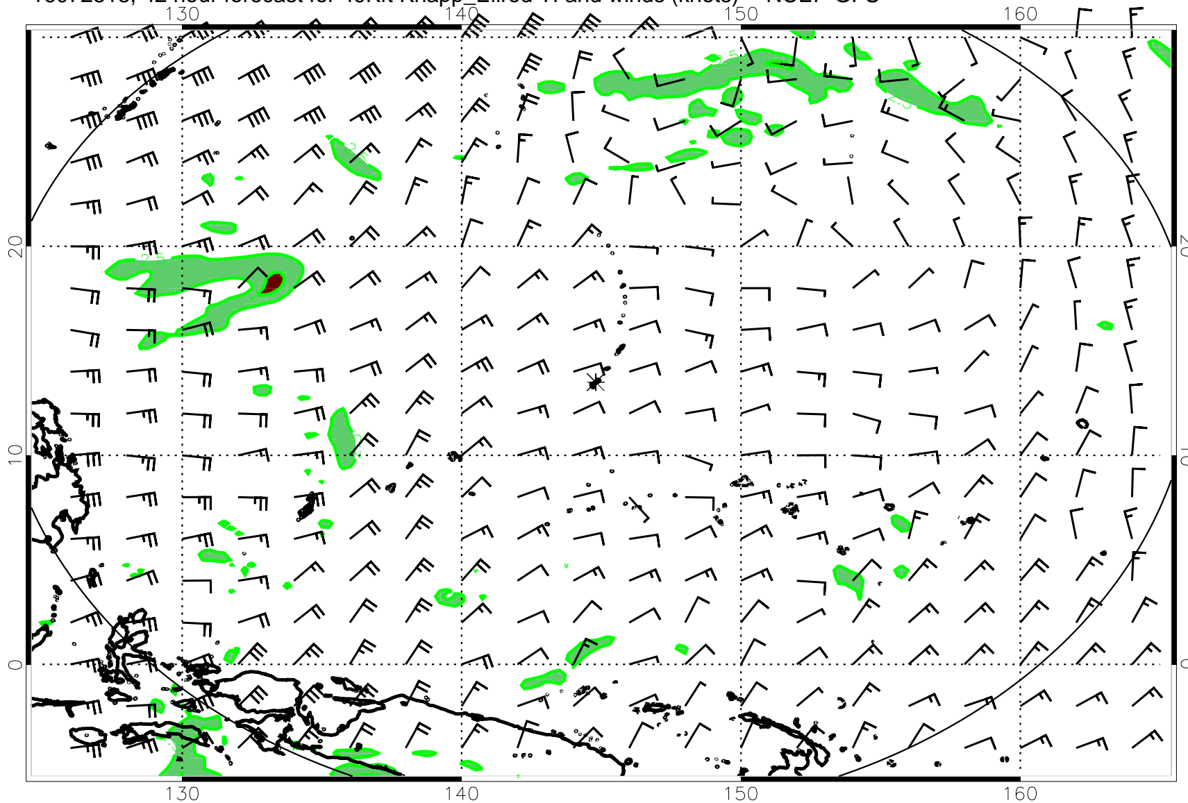
16072818, 42 hour forecast for 49Kft Knapp_Ellrod TI and winds (knots) -- NCEP GFS
