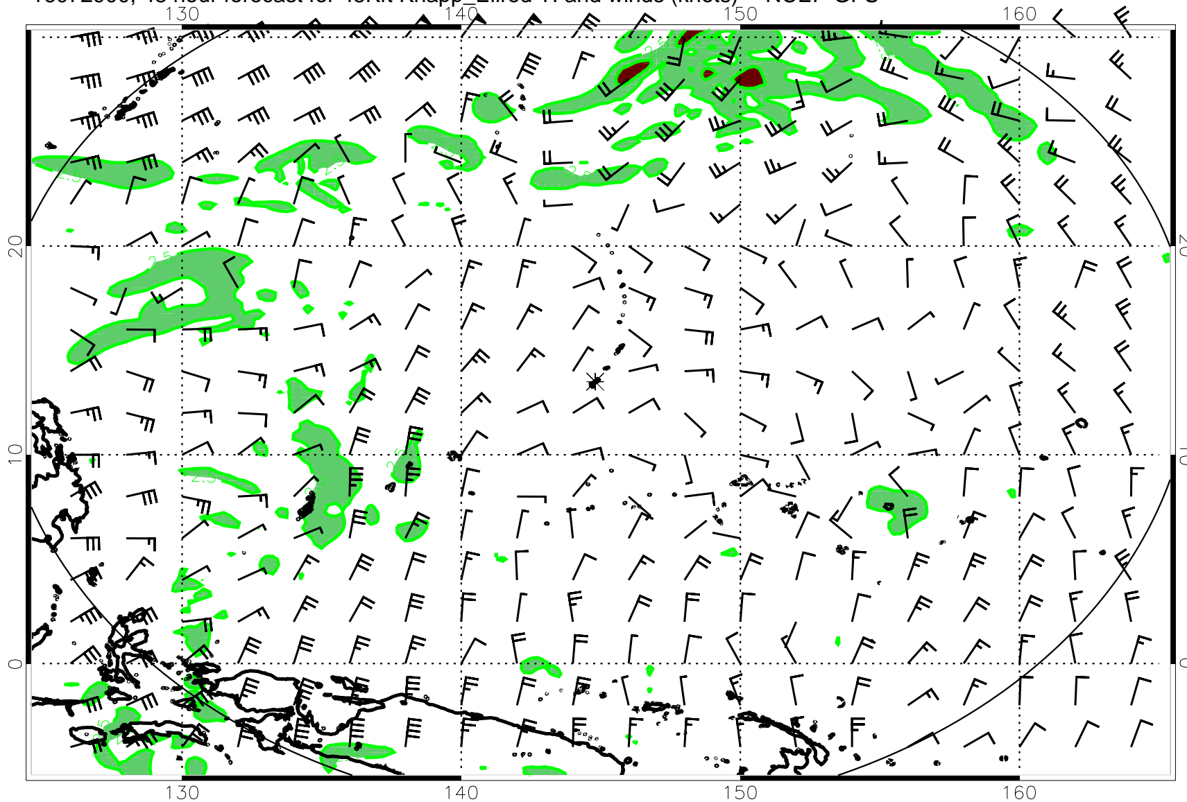
16072900, 48 hour forecast for 45Kft Knapp_Ellrod TI and winds (knots) -- NCEP GFS
