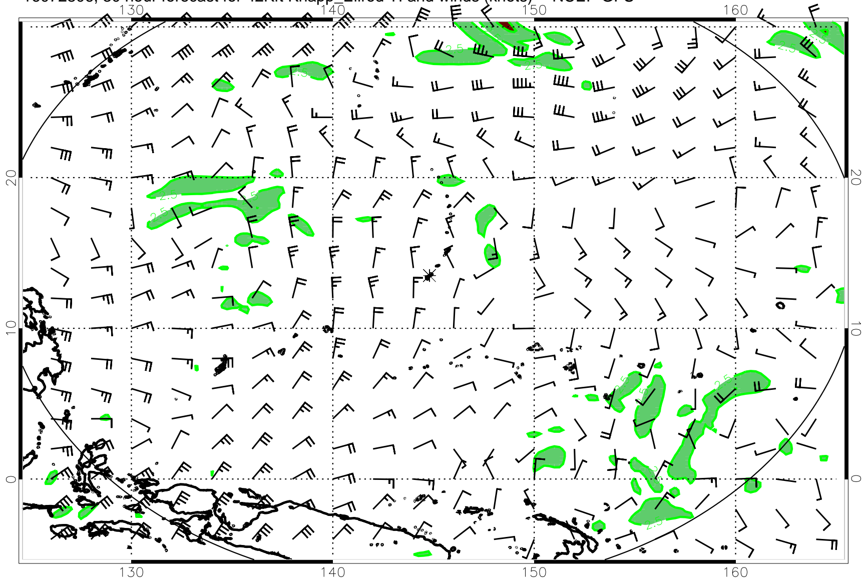
16072806, 30 hour forecast for 42Kft Knapp_Ellrod TI and winds (knots) -- NCEP GFS
