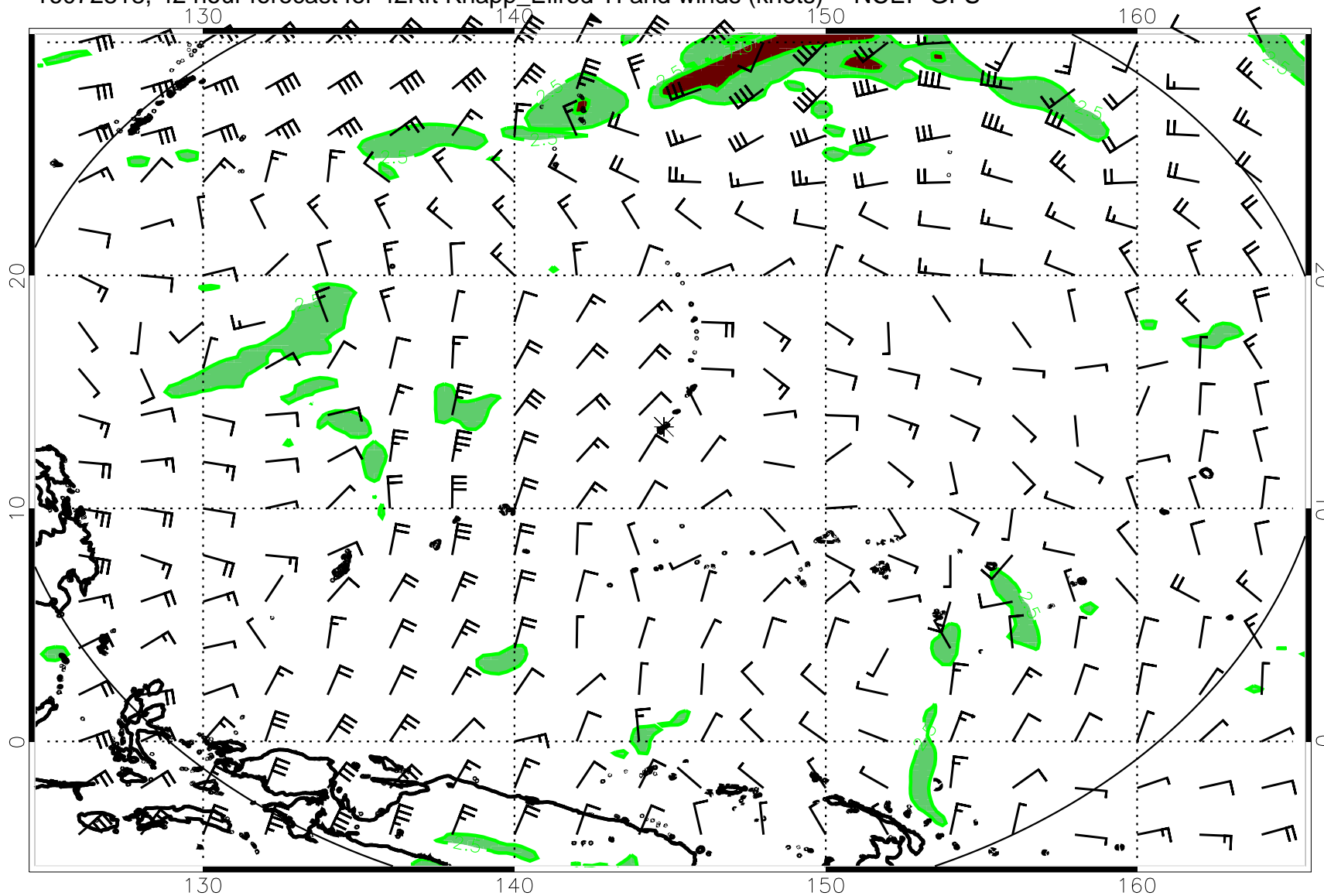
16072818, 42 hour forecast for 42Kft Knapp_Ellrod TI and winds (knots) -- NCEP GFS
