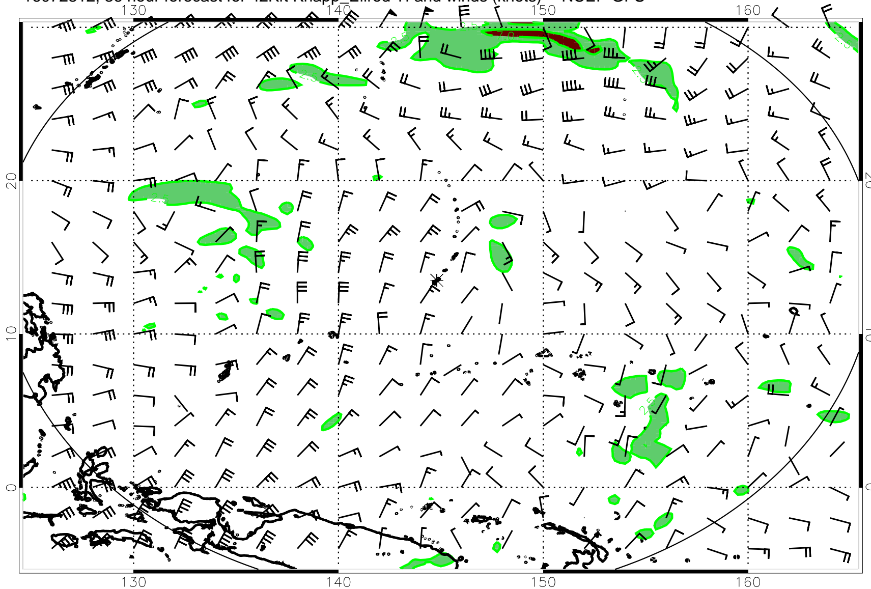
16072812, 36 hour forecast for 42Kft Knapp_Ellrod TI and winds (knots) -- NCEP GFS
