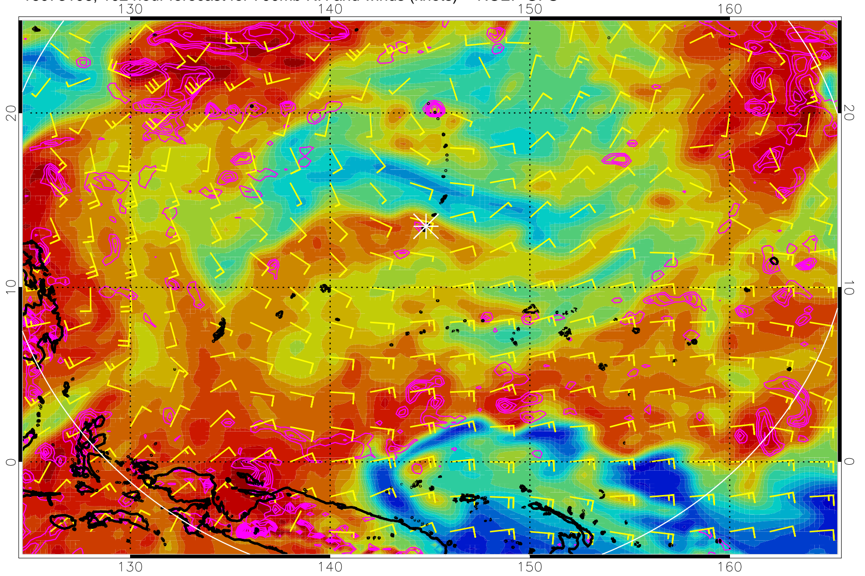
16073106, 102 hour forecast for 700mb RH and winds (knots) -- NCEP GFS
