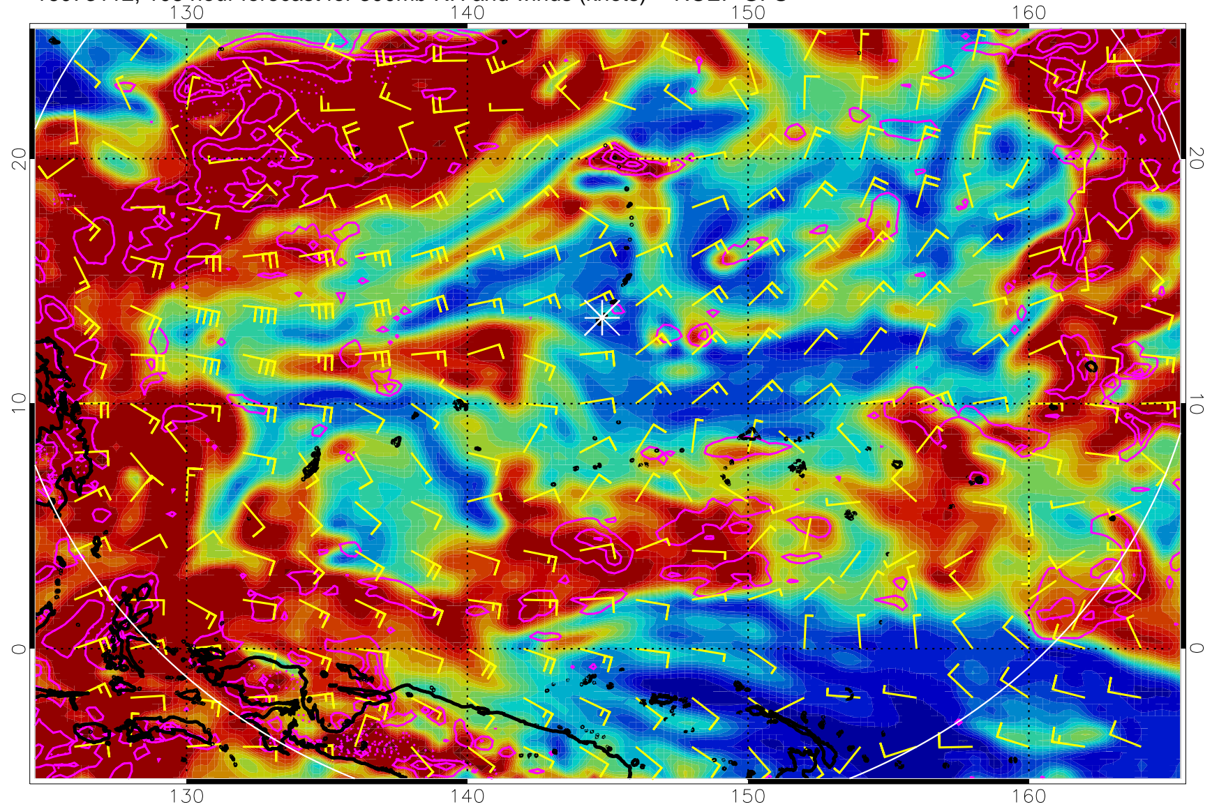
16073112, 108 hour forecast for 300mb RH and winds (knots) -- NCEP GFS
