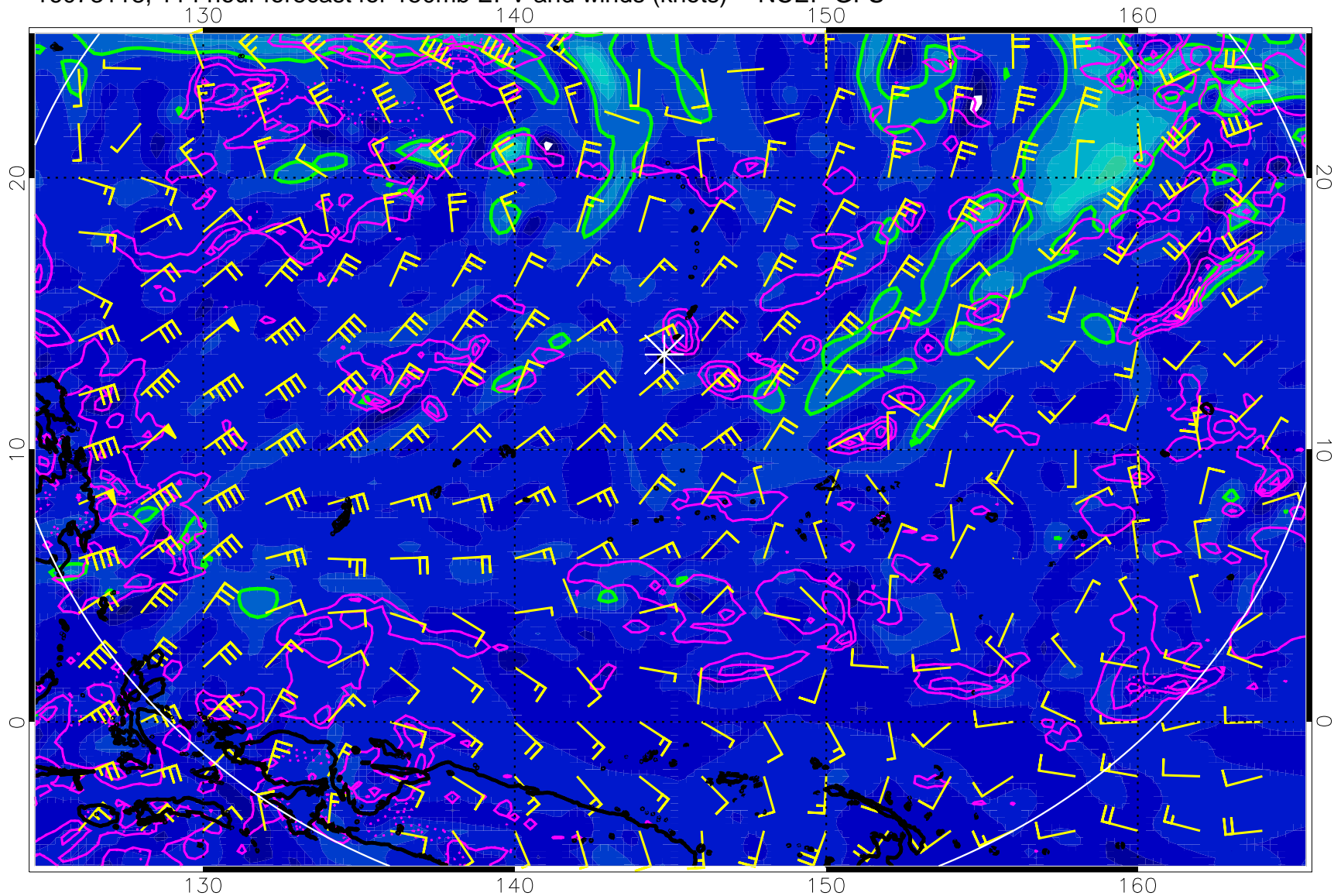
16073118, 114 hour forecast for 150mb EPV and winds (knots) -- NCEP GFS
