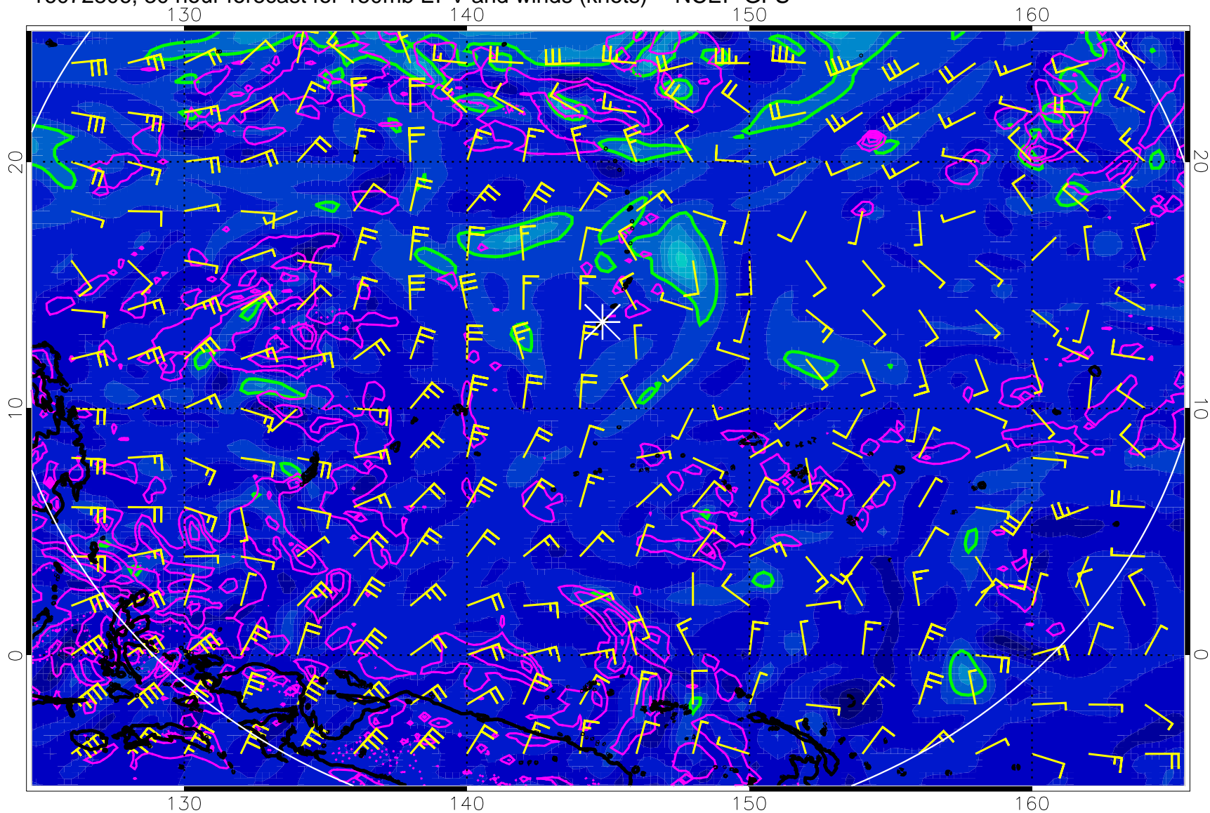
16072806, 30 hour forecast for 150mb EPV and winds (knots) -- NCEP GFS
