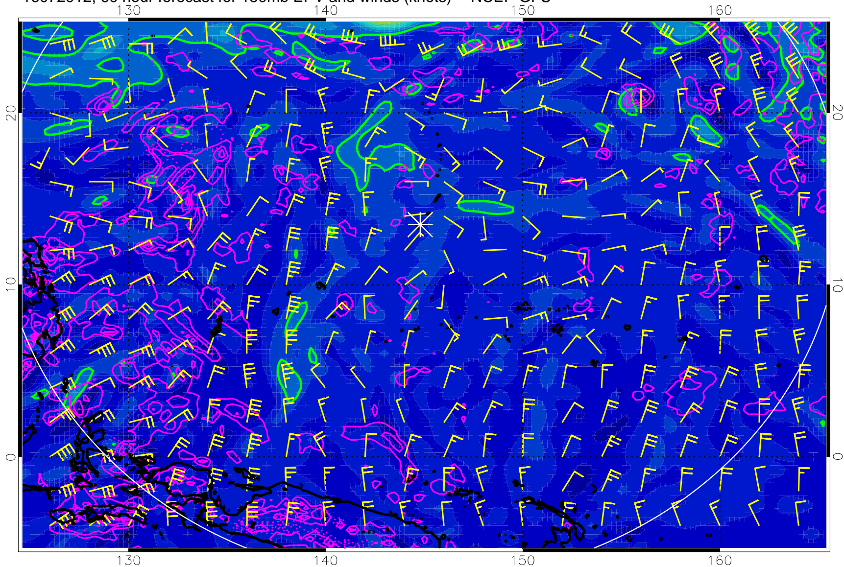
16072912, 60 hour forecast for 150mb EPV and winds (knots) -- NCEP GFS
