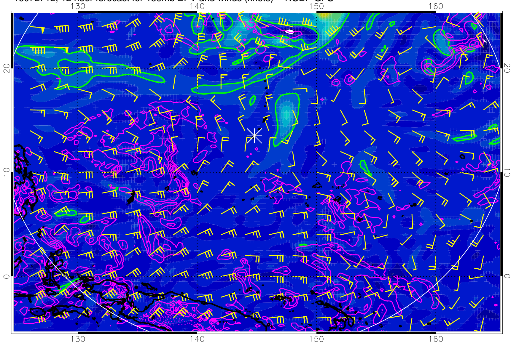
16072712, 12 hour forecast for 150mb EPV and winds (knots) -- NCEP GFS
