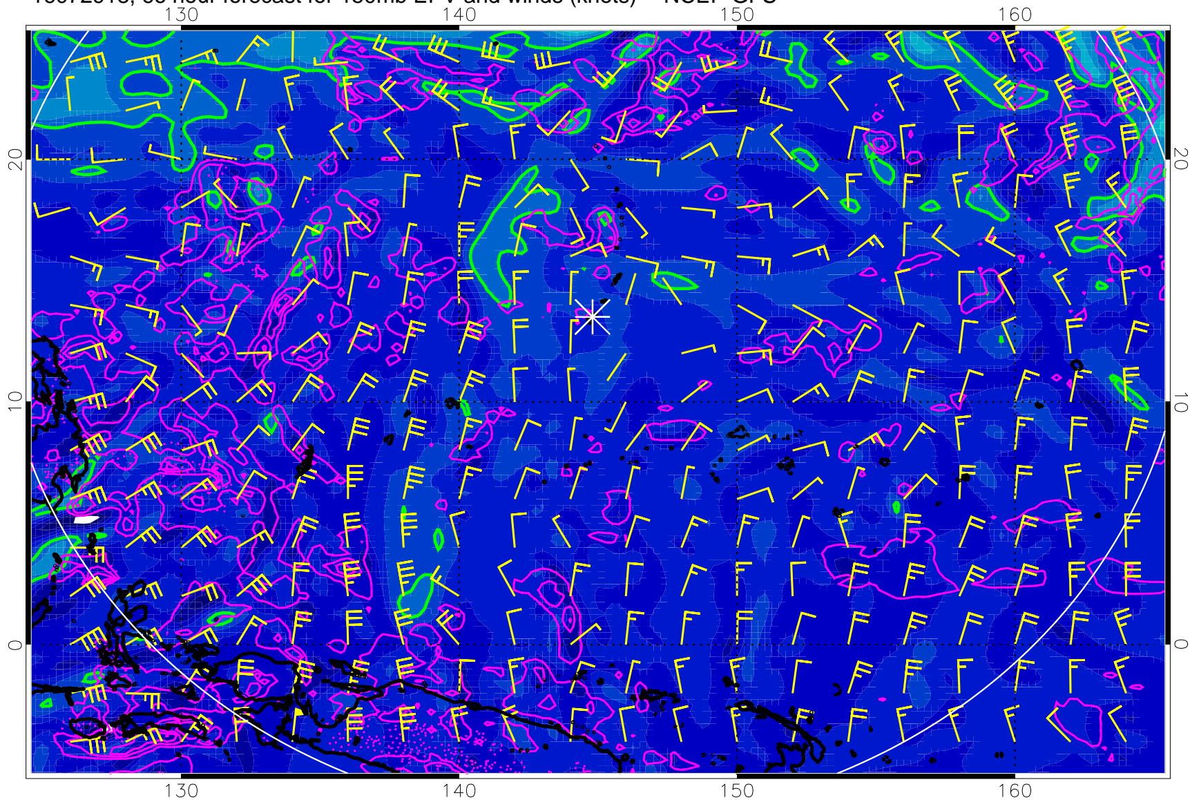
16072918, 66 hour forecast for 150mb EPV and winds (knots) -- NCEP GFS
