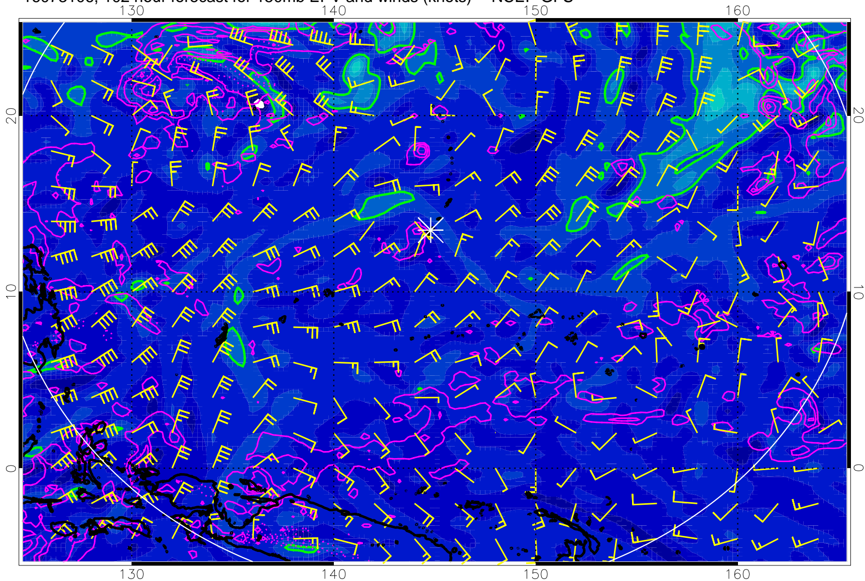
16073106, 102 hour forecast for 150mb EPV and winds (knots) -- NCEP GFS
