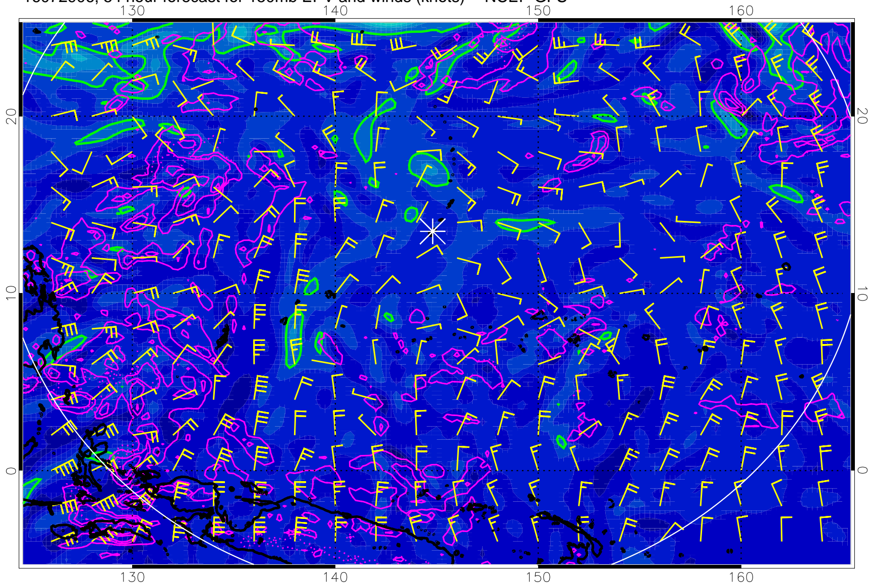
16072906, 54 hour forecast for 150mb EPV and winds (knots) -- NCEP GFS
