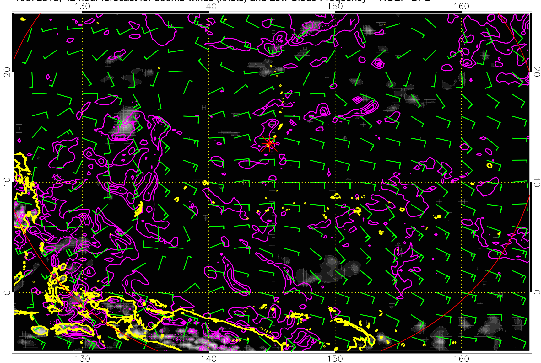
16072818, 42 hour forecast for 850mb winds (knots) and Low Cloud Frequency -- NCEP GFS
