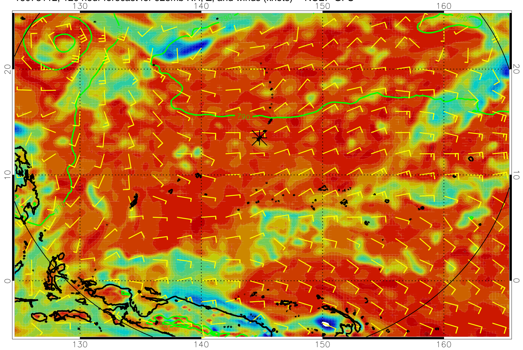
16073112, 120 hour forecast for 925mb RH, Z, and winds (knots) -- NCEP GFS
