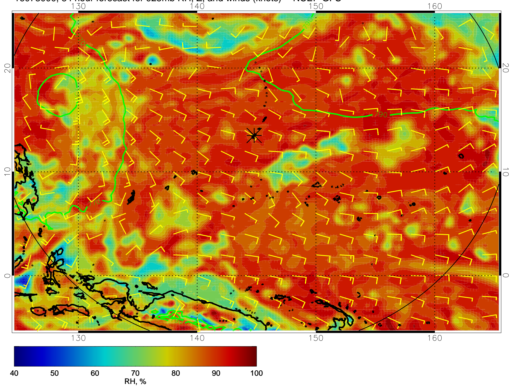
16073000, 84 hour forecast for 925mb RH, Z, and winds (knots) -- NCEP GFS
