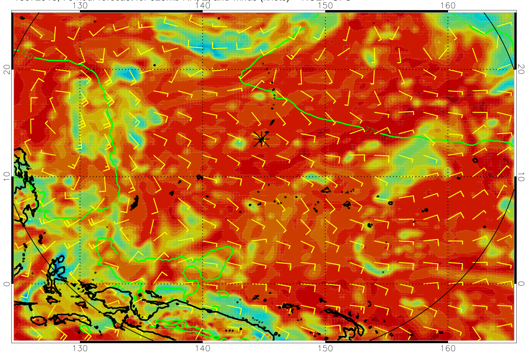
16072918, 78 hour forecast for 925mb RH, Z, and winds (knots) -- NCEP GFS
