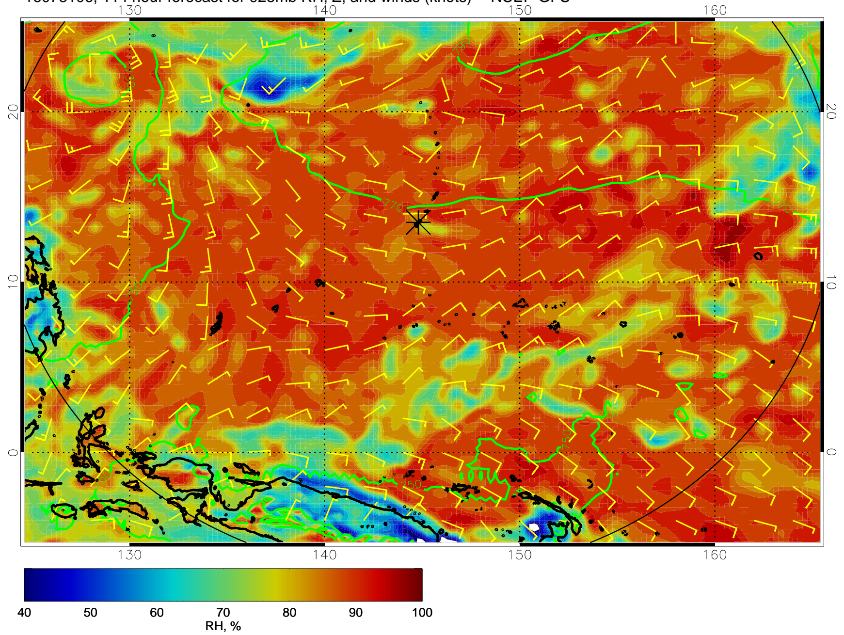
16073106, 114 hour forecast for 925mb RH, Z, and winds (knots) -- NCEP GFS
