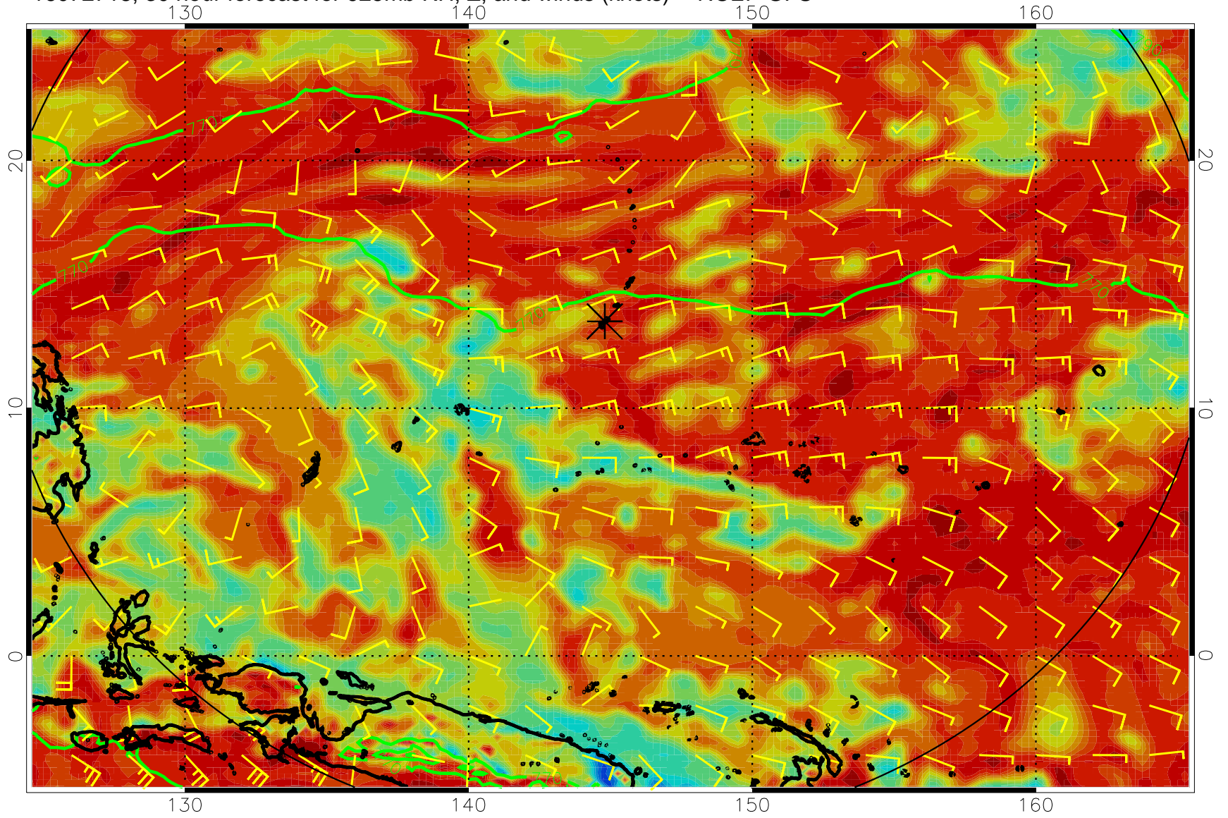
16072718, 30 hour forecast for 925mb RH, Z, and winds (knots) -- NCEP GFS
