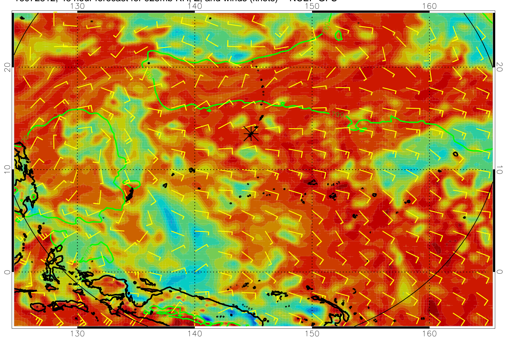
16072812, 48 hour forecast for 925mb RH, Z, and winds (knots) -- NCEP GFS
