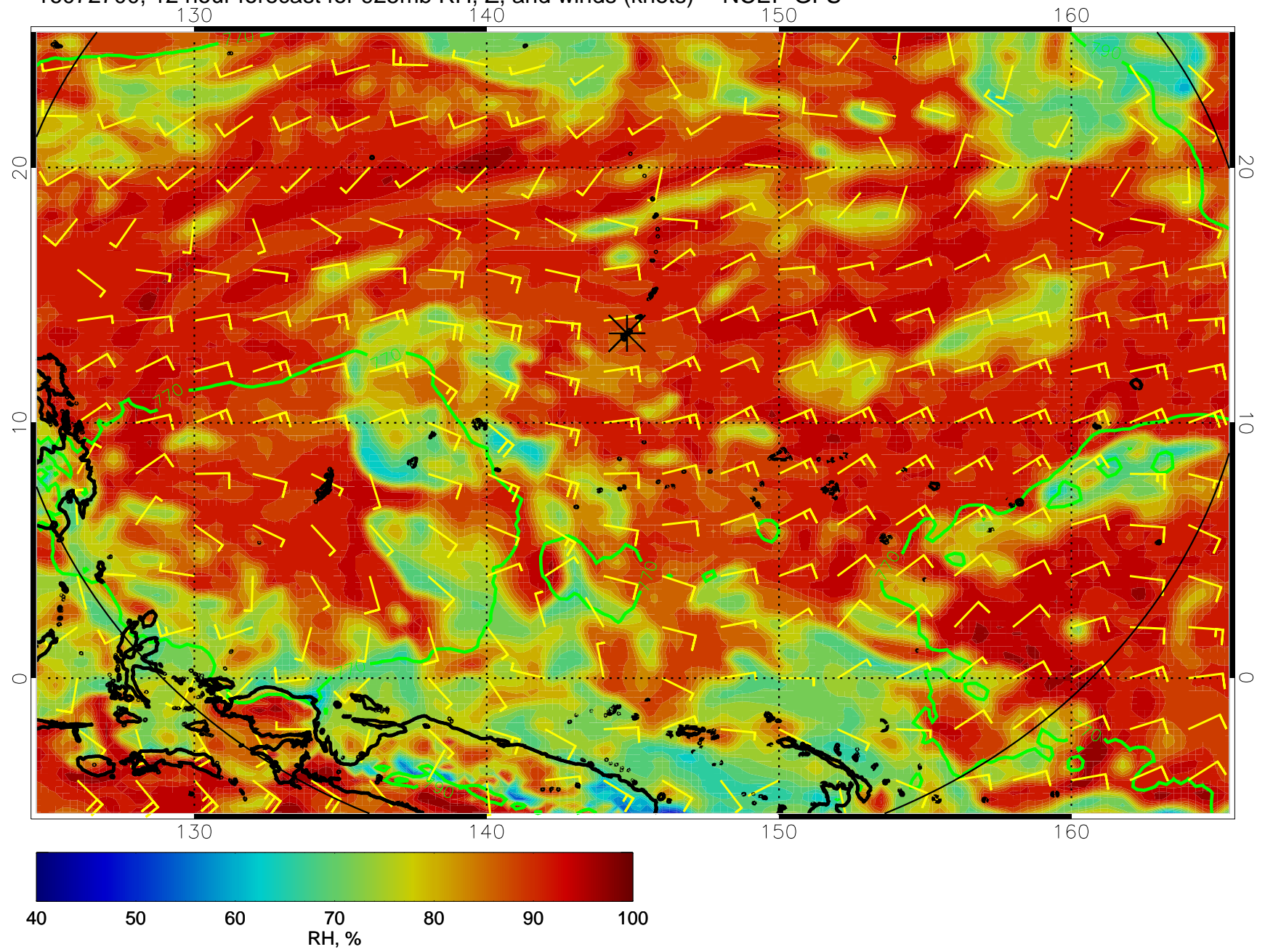
16072700, 12 hour forecast for 925mb RH, Z, and winds (knots) -- NCEP GFS
