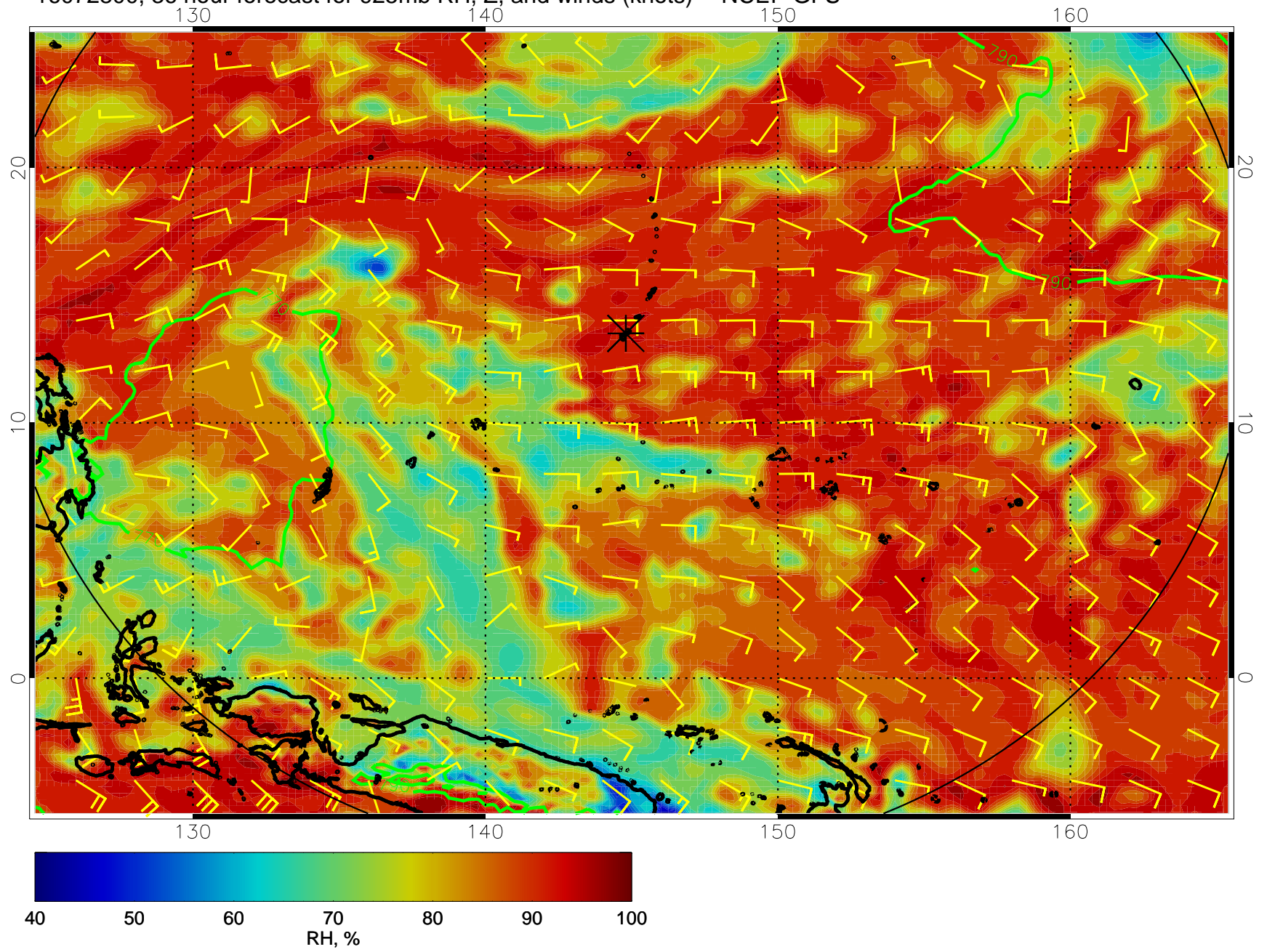
16072800, 36 hour forecast for 925mb RH, Z, and winds (knots) -- NCEP GFS
