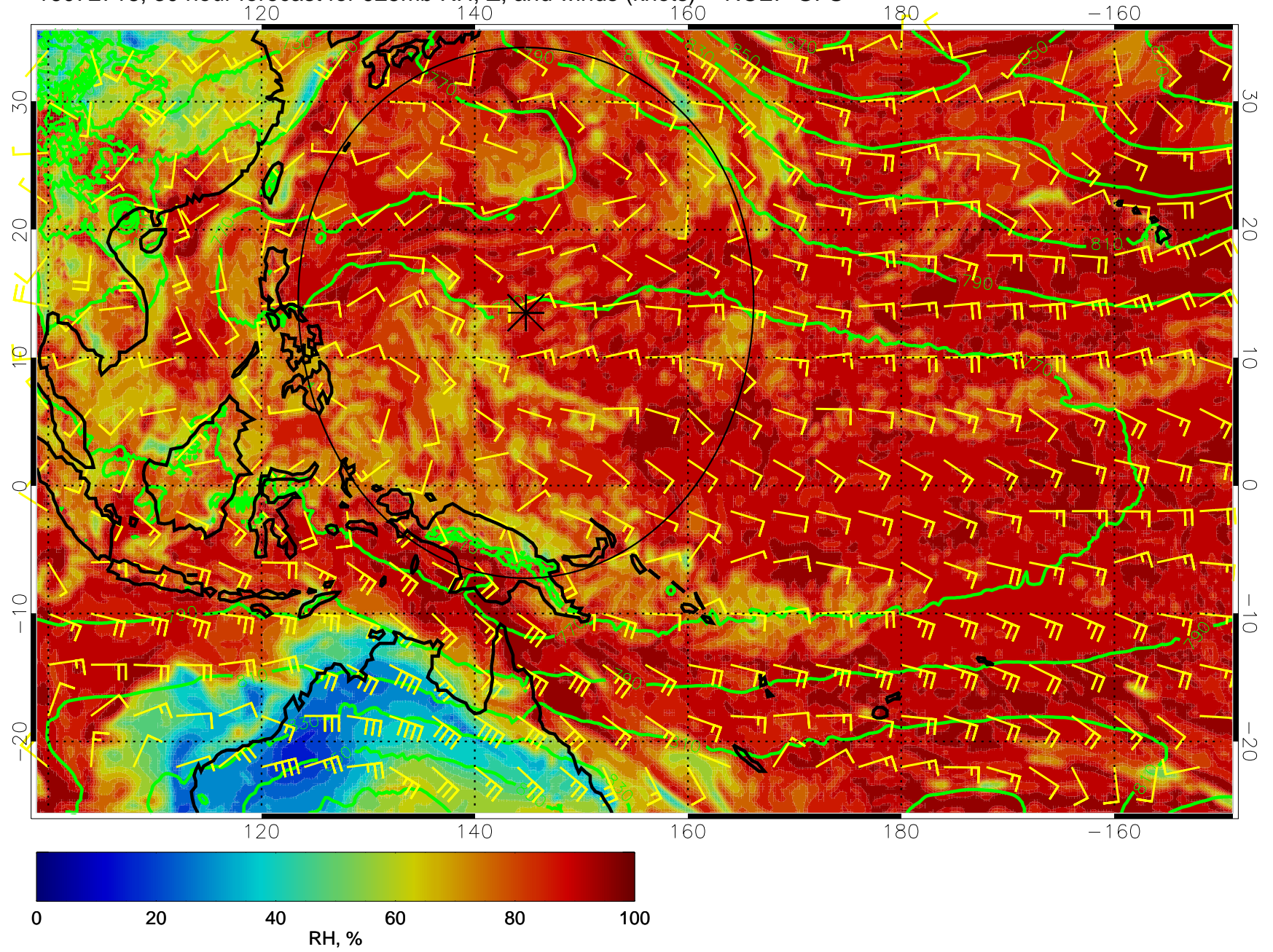
16072718, 30 hour forecast for 925mb RH, Z, and winds (knots) -- NCEP GFS
