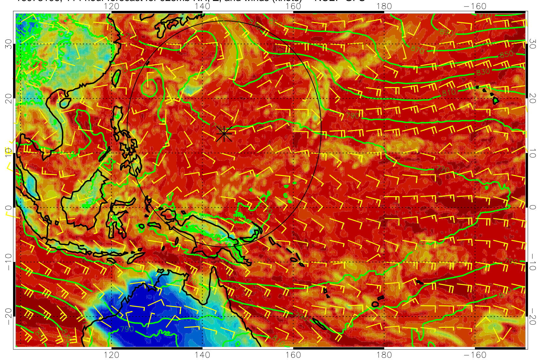
16073106, 114 hour forecast for 925mb RH, Z, and winds (knots) -- NCEP GFS
