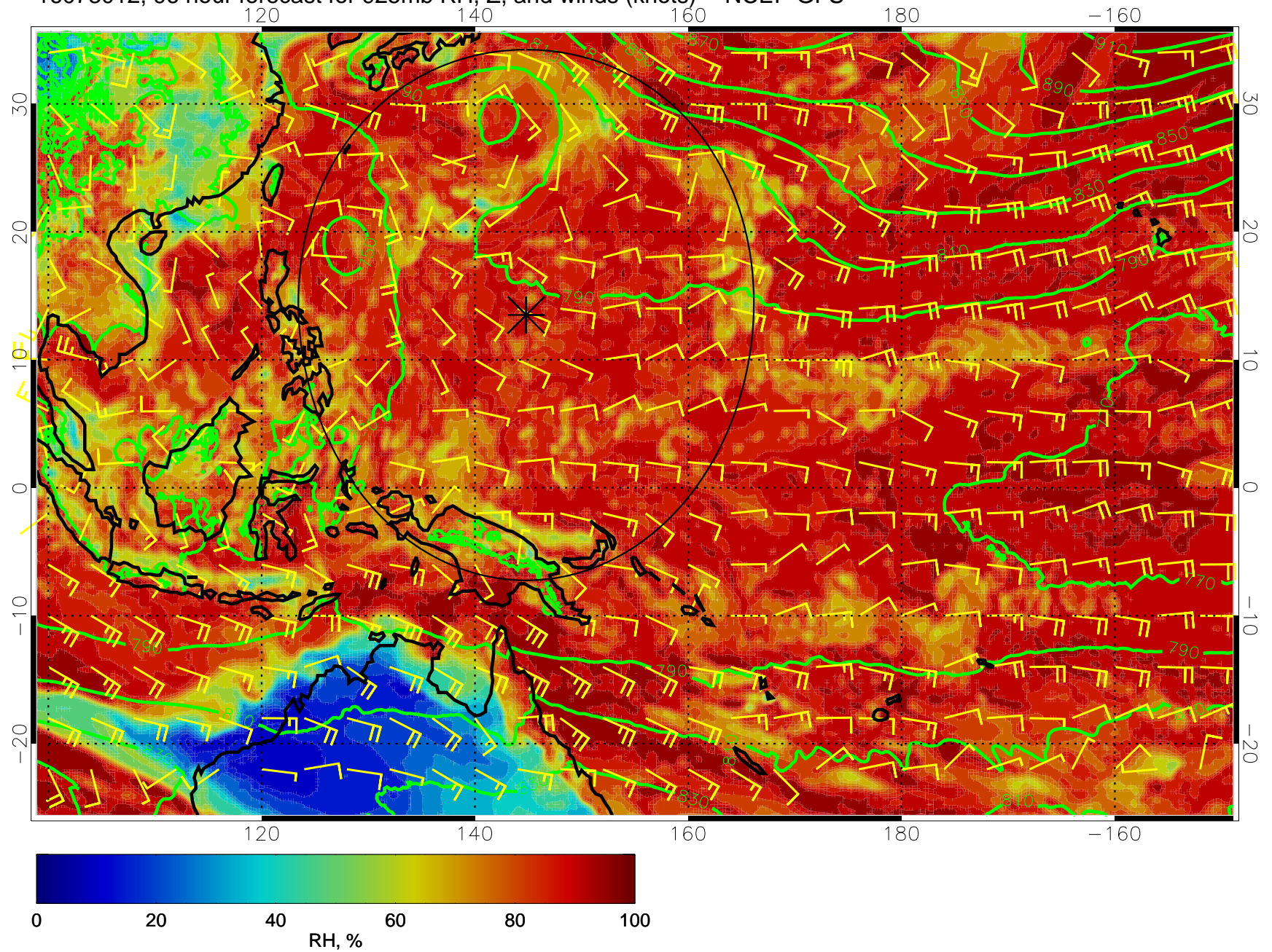
16073012, 96 hour forecast for 925mb RH, Z, and winds (knots) -- NCEP GFS
