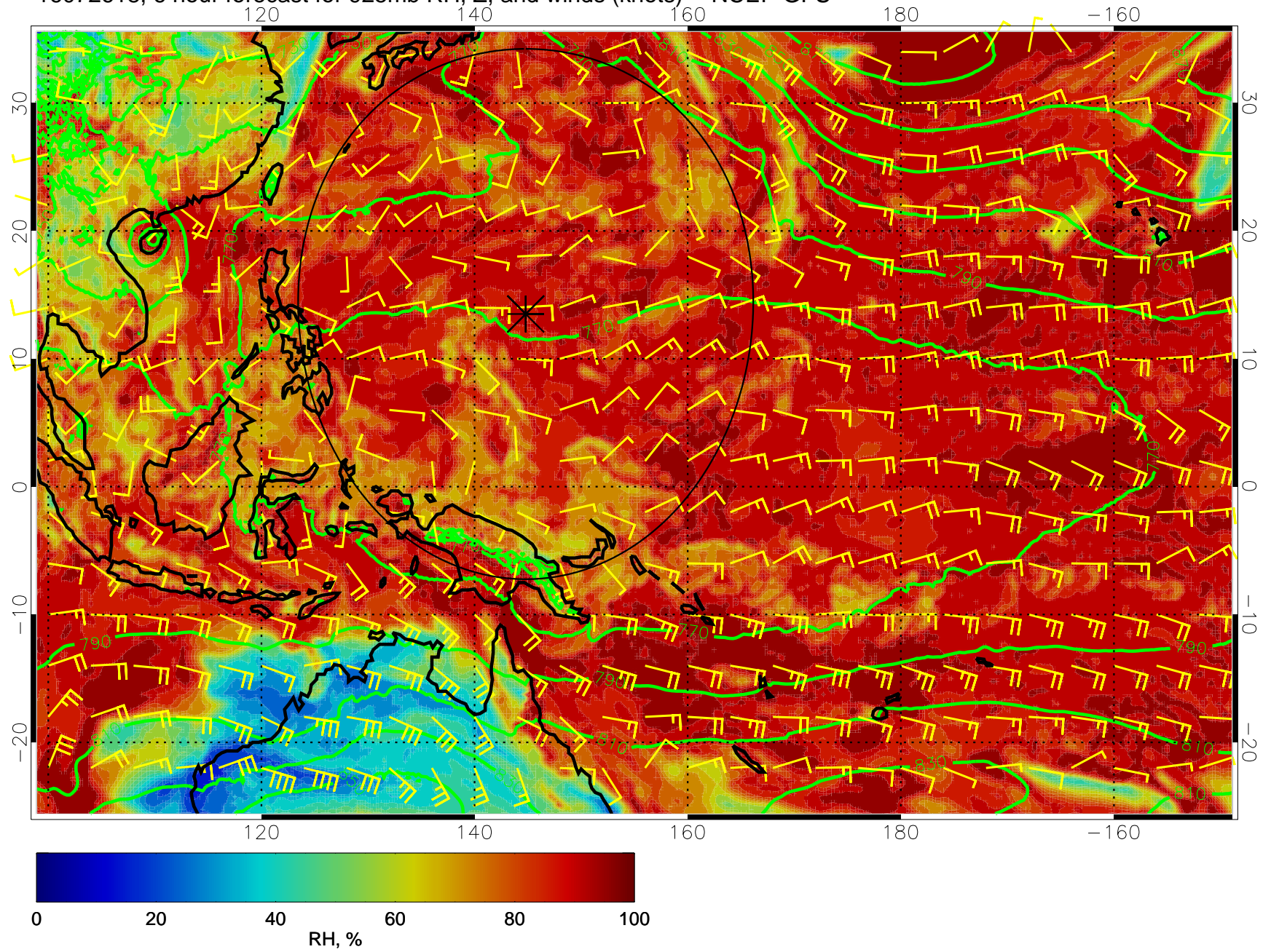
16072618, 6 hour forecast for 925mb RH, Z, and winds (knots) -- NCEP GFS
