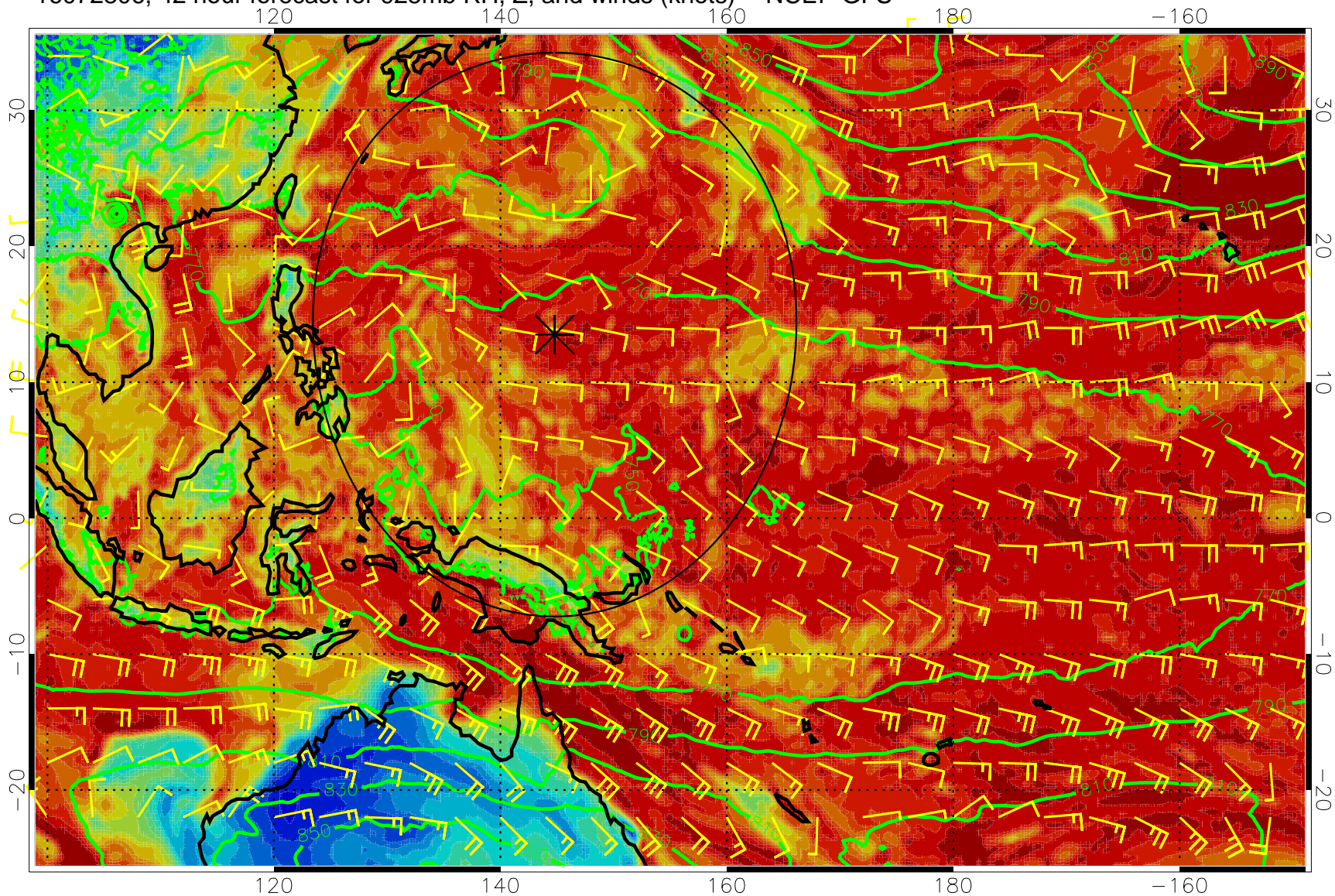
16072806, 42 hour forecast for 925mb RH, Z, and winds (knots) -- NCEP GFS
