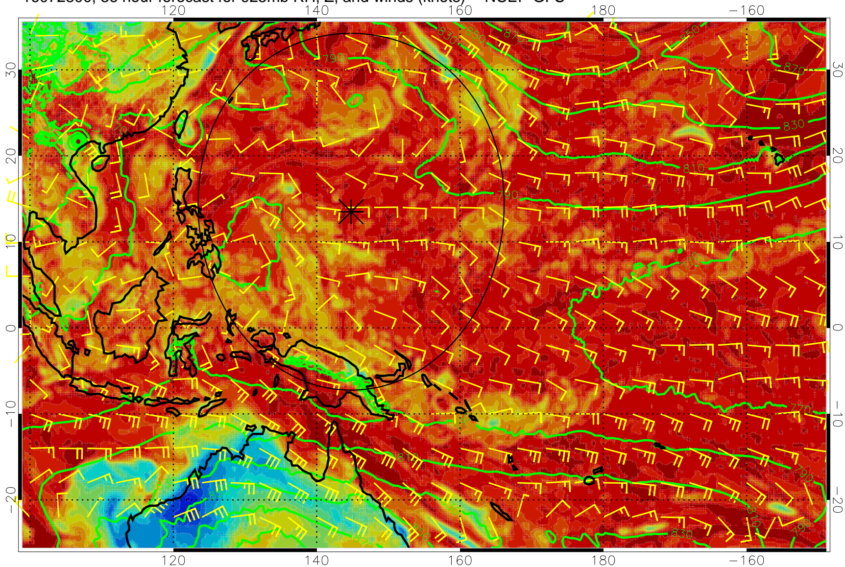
16072800, 36 hour forecast for 925mb RH, Z, and winds (knots) -- NCEP GFS
