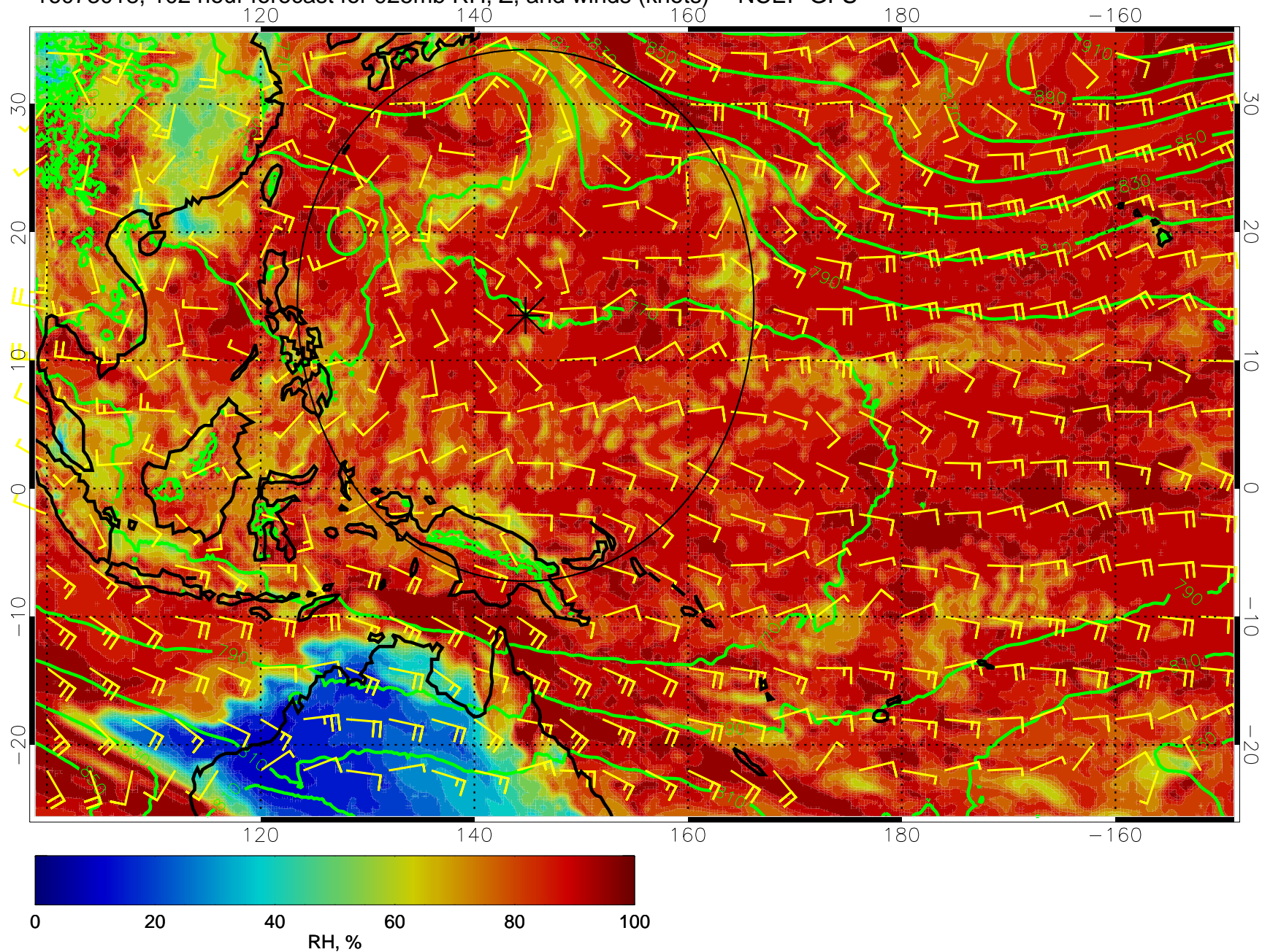
16073018, 102 hour forecast for 925mb RH, Z, and winds (knots) -- NCEP GFS
