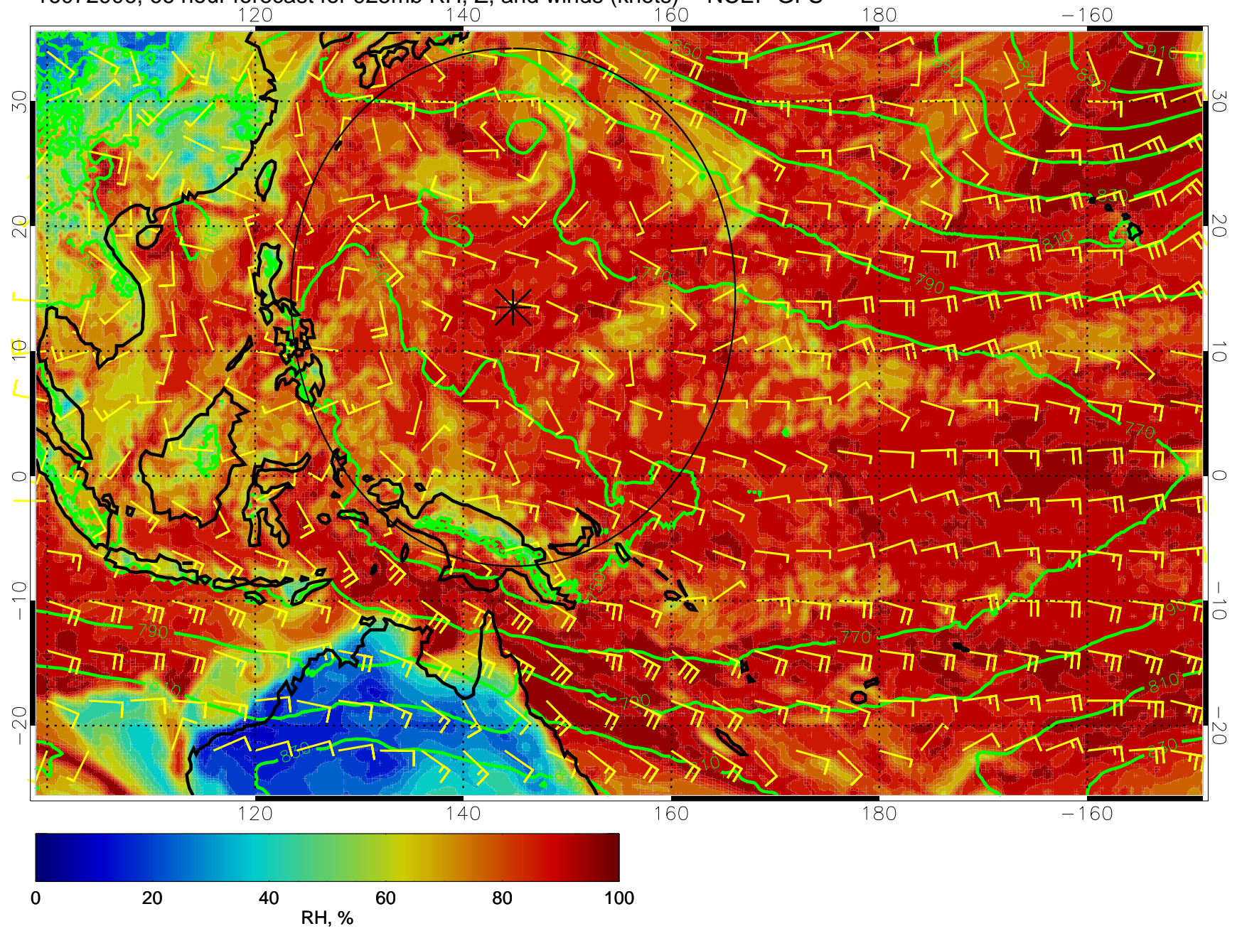
16072906, 66 hour forecast for 925mb RH, Z, and winds (knots) -- NCEP GFS
