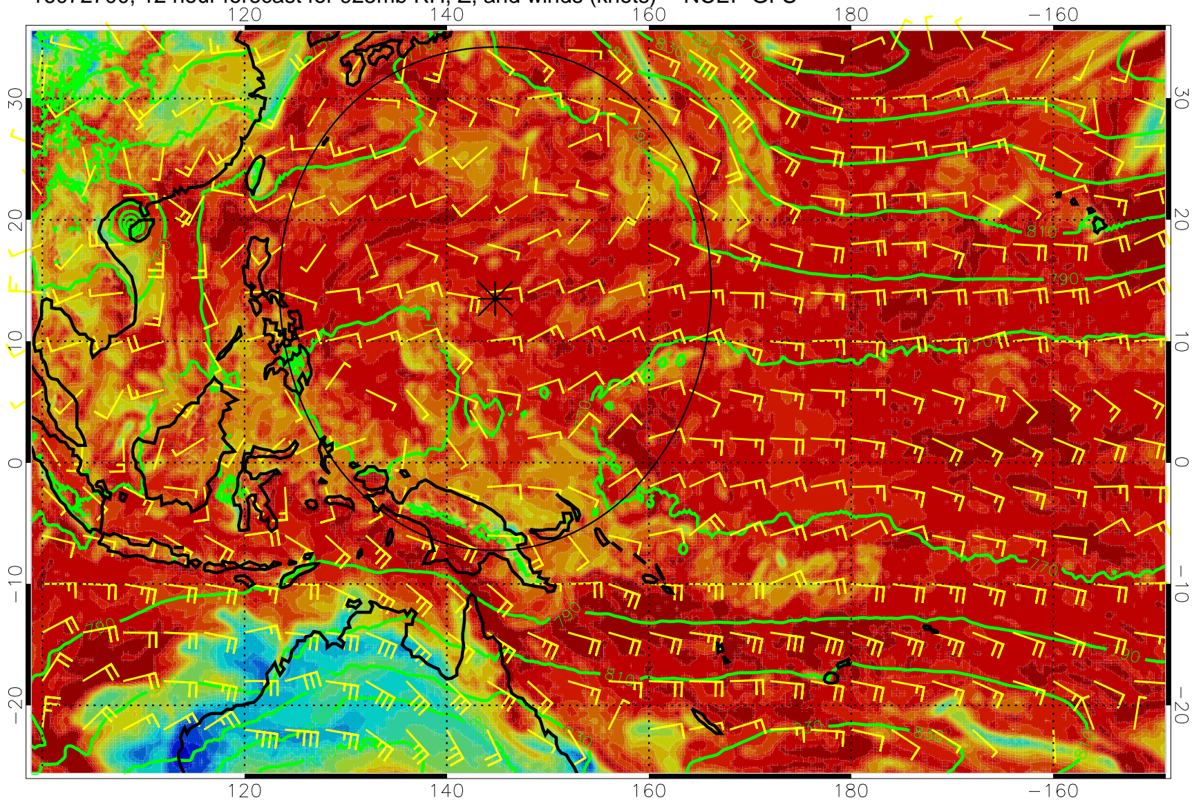
16072700, 12 hour forecast for 925mb RH, Z, and winds (knots) -- NCEP GFS
