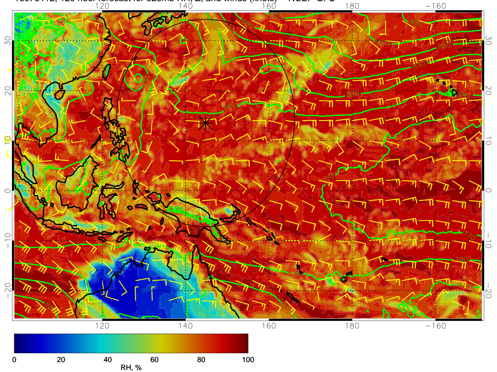
16073112, 120 hour forecast for 925mb RH, Z, and winds (knots) -- NCEP GFS
