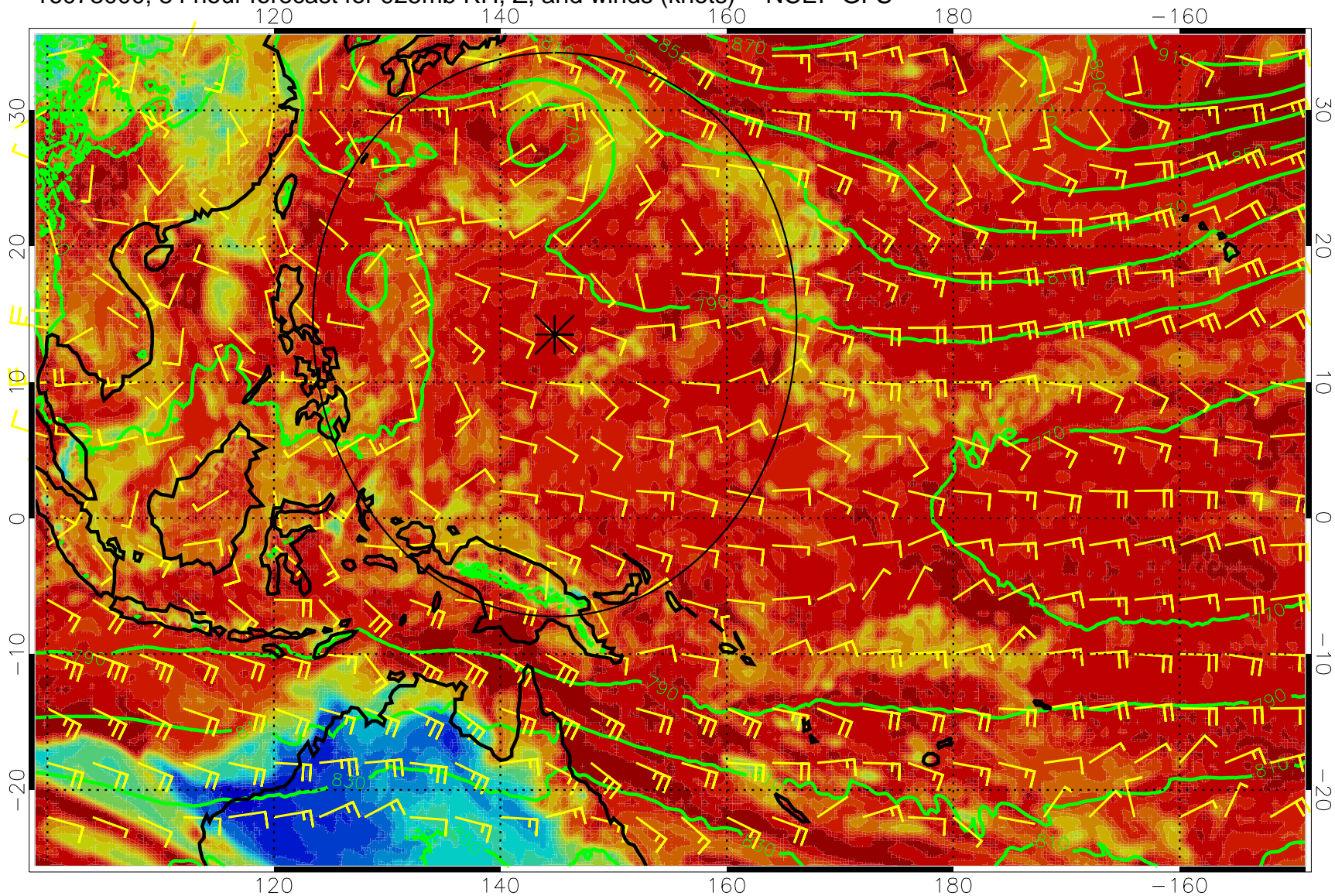
16073000, 84 hour forecast for 925mb RH, Z, and winds (knots) -- NCEP GFS
