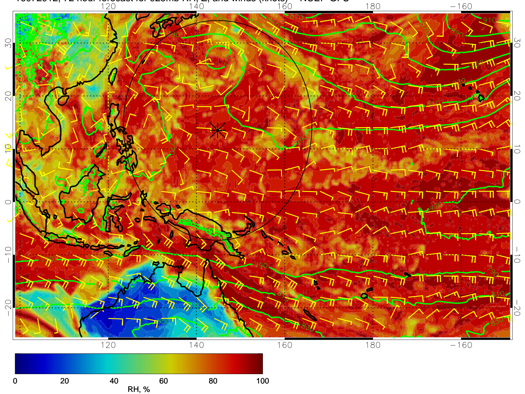
16072912, 72 hour forecast for 925mb RH, Z, and winds (knots) -- NCEP GFS
