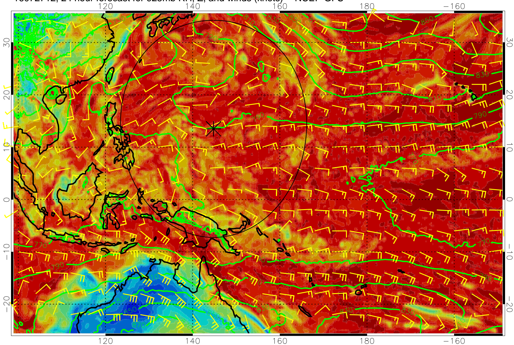
16072712, 24 hour forecast for 925mb RH, Z, and winds (knots) -- NCEP GFS
