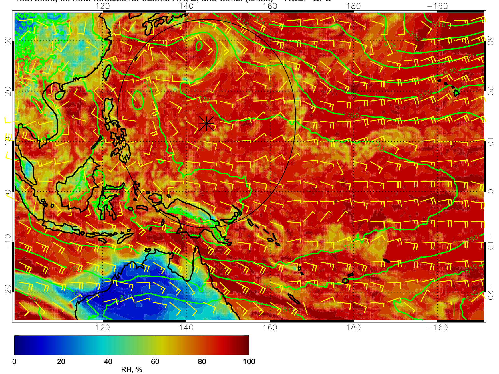
16073006, 90 hour forecast for 925mb RH, Z, and winds (knots) -- NCEP GFS
