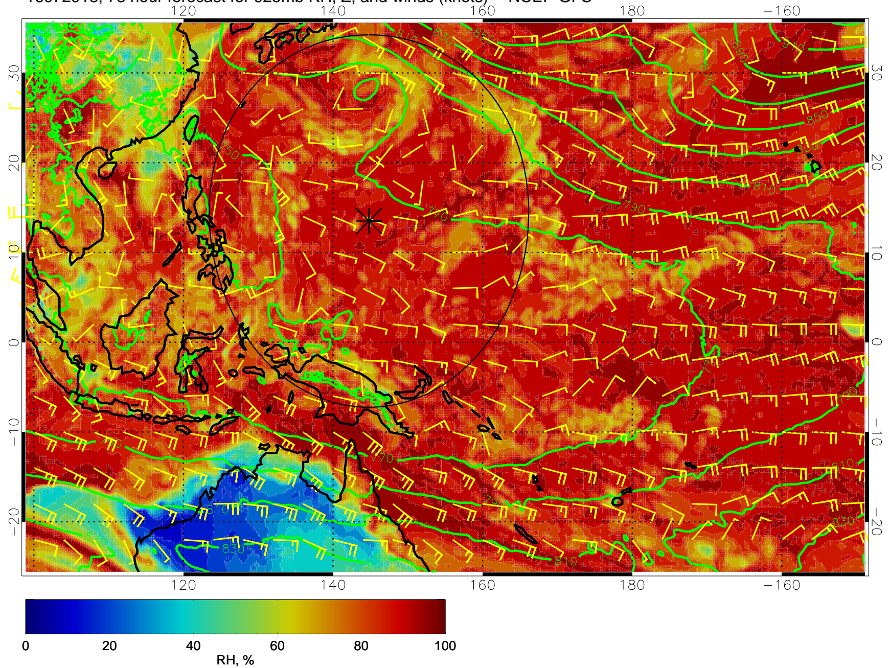
16072918, 78 hour forecast for 925mb RH, Z, and winds (knots) -- NCEP GFS
