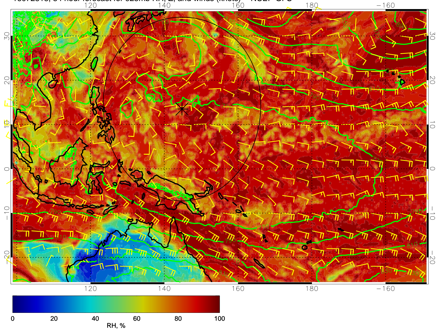
16072818, 54 hour forecast for 925mb RH, Z, and winds (knots) -- NCEP GFS
