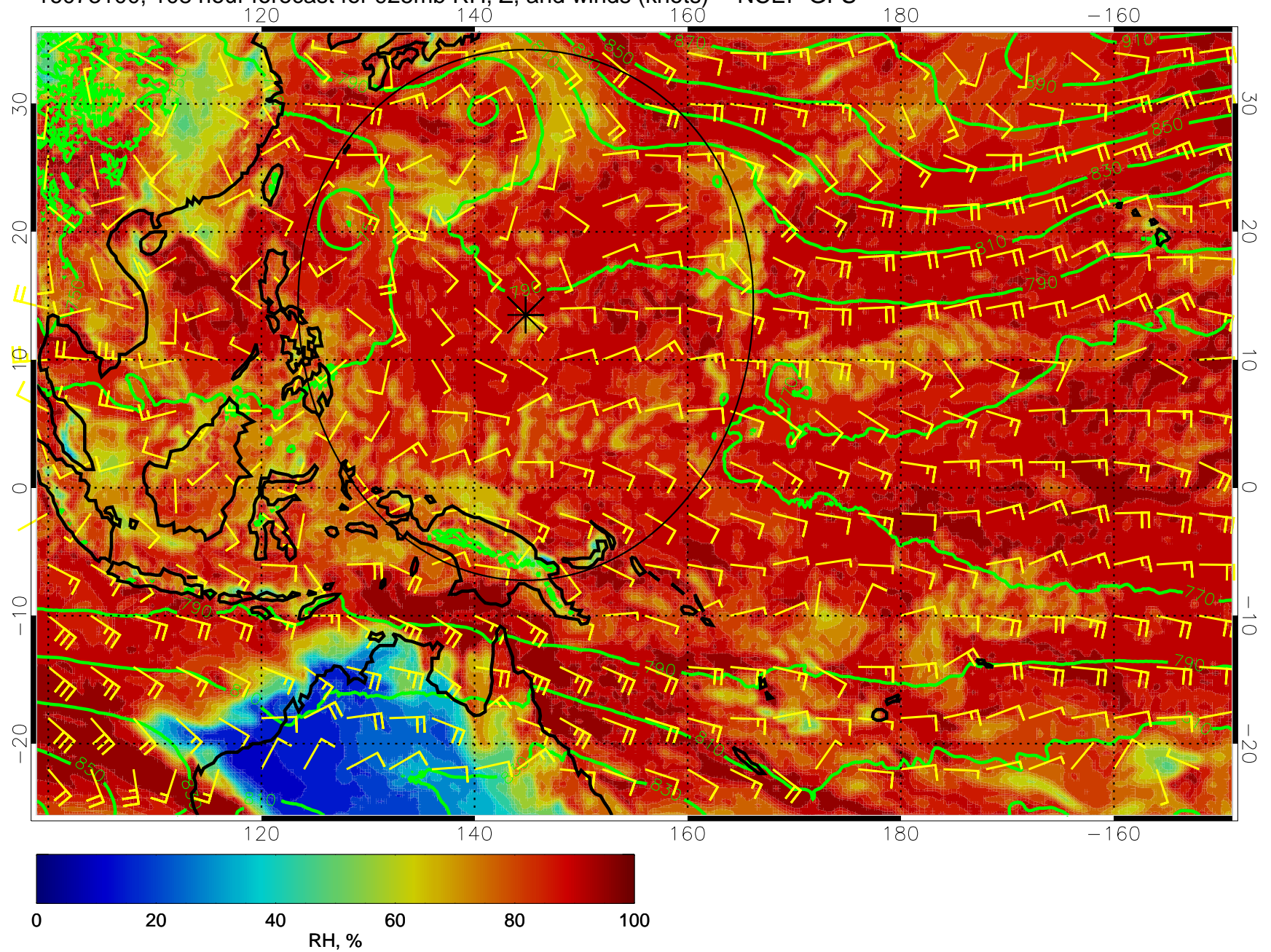
16073100, 108 hour forecast for 925mb RH, Z, and winds (knots) -- NCEP GFS
