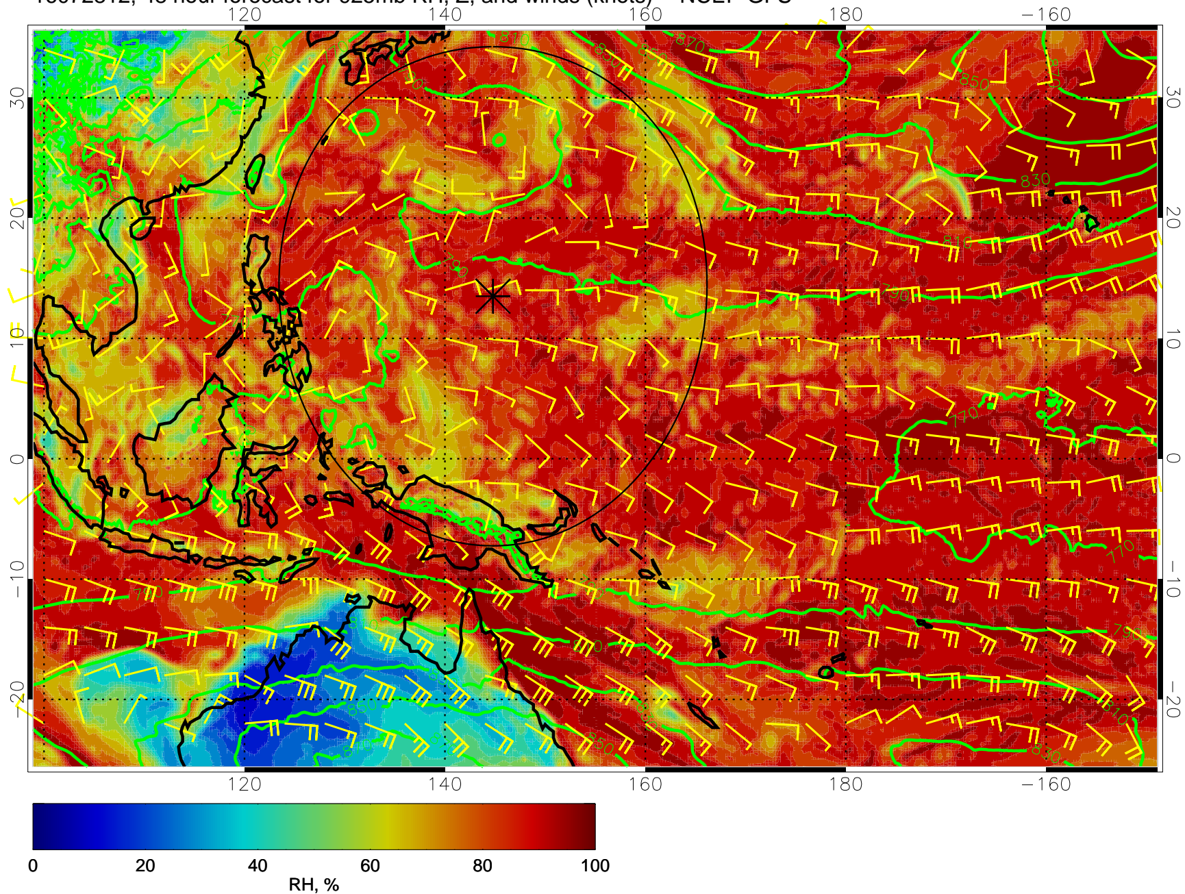
16072812, 48 hour forecast for 925mb RH, Z, and winds (knots) -- NCEP GFS
