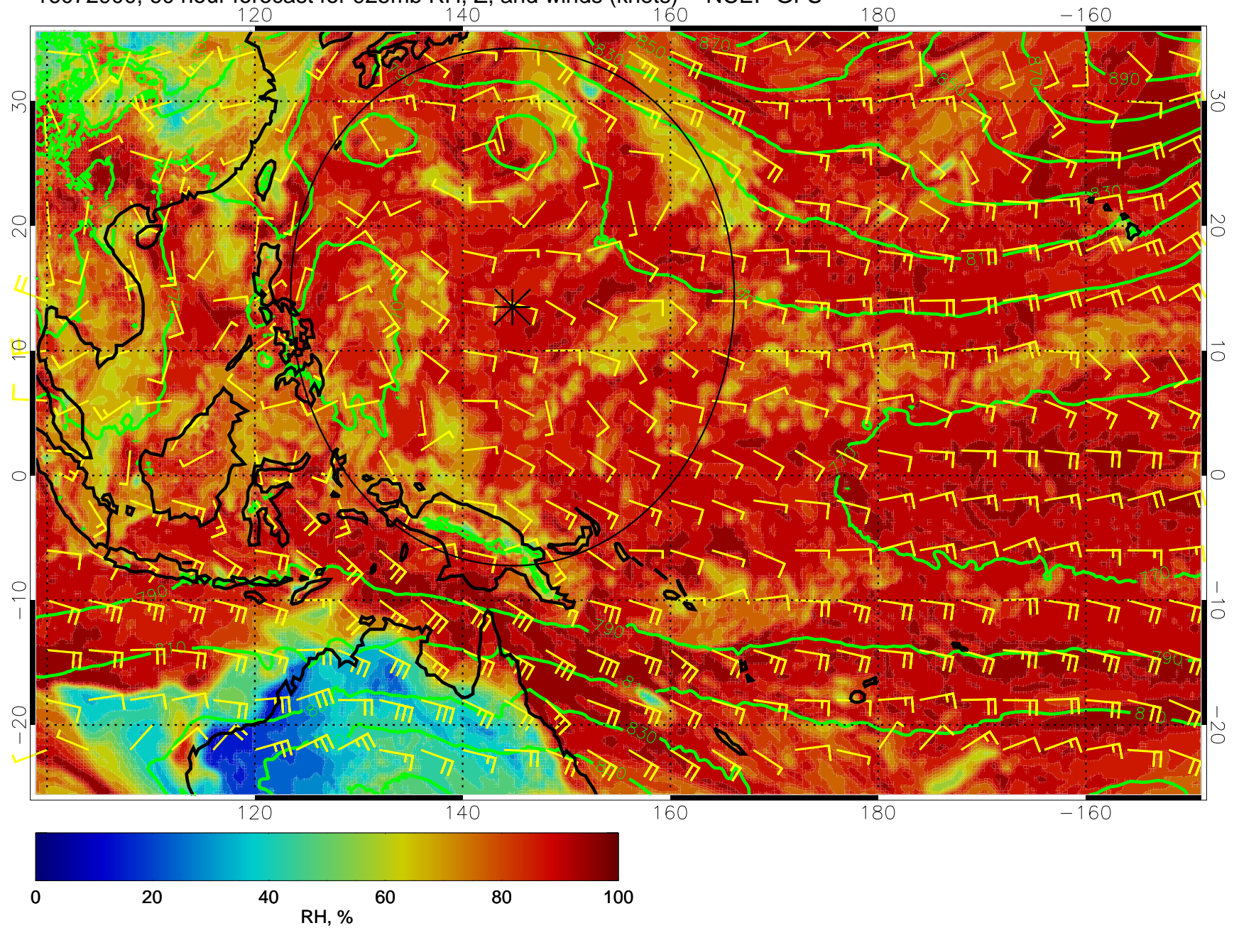
16072900, 60 hour forecast for 925mb RH, Z, and winds (knots) -- NCEP GFS
