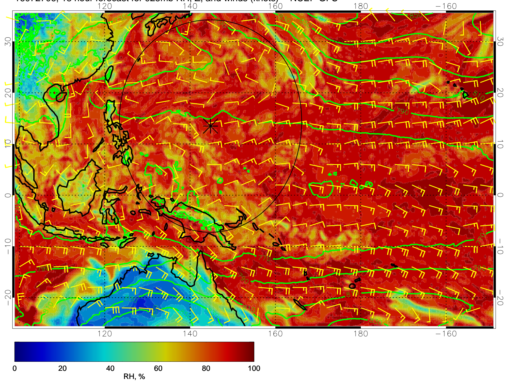
16072706, 18 hour forecast for 925mb RH, Z, and winds (knots) -- NCEP GFS
