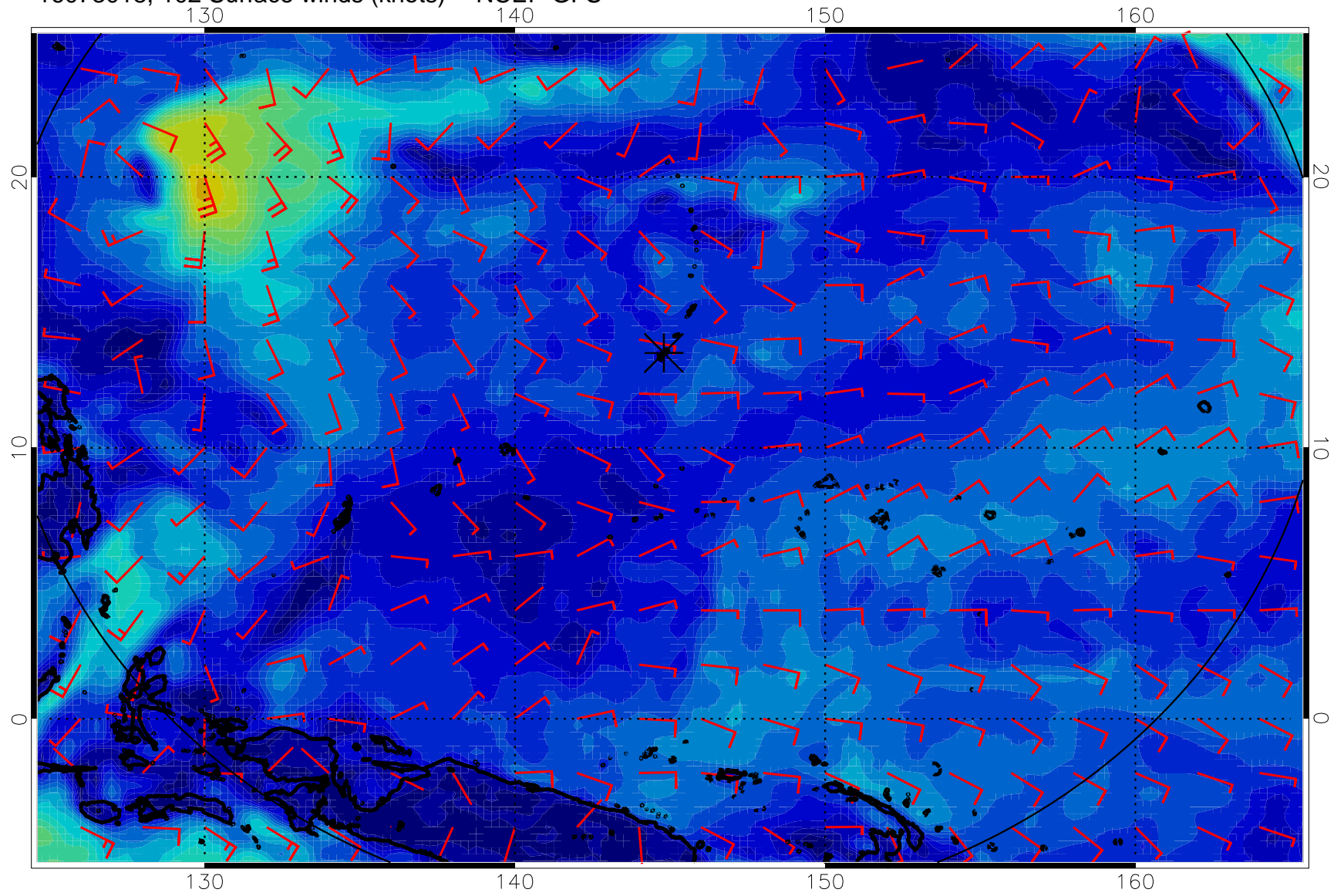
16073018, 102 Surface winds (knots) -- NCEP GFS
