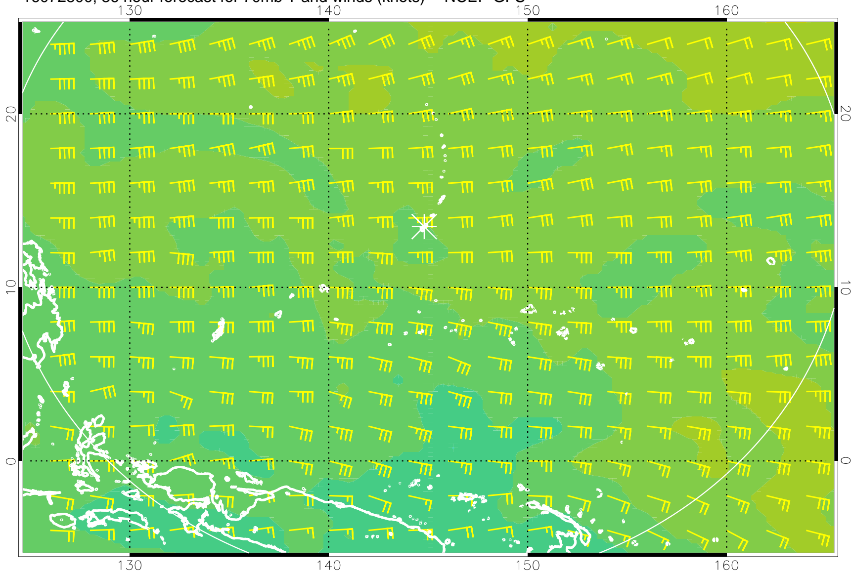
16072800, 36 hour forecast for 70mb T and winds (knots) -- NCEP GFS
