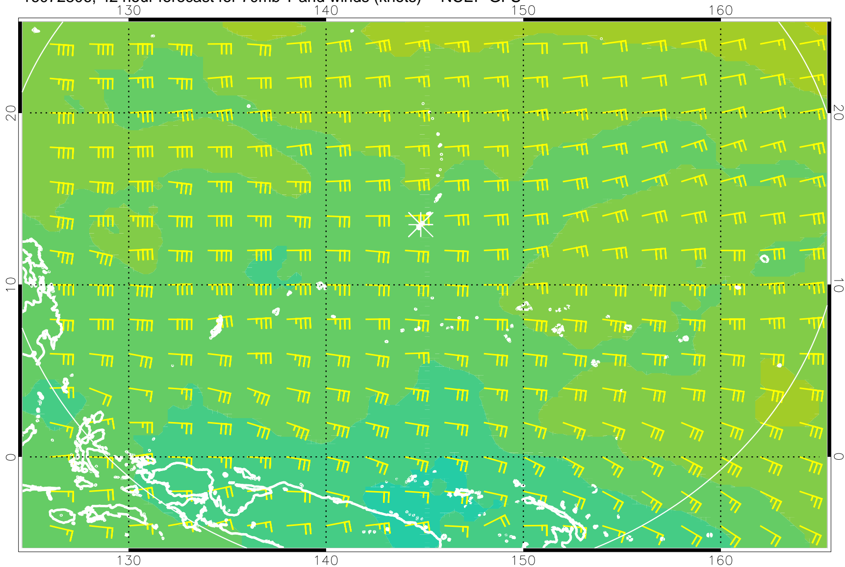
16072806, 42 hour forecast for 70mb T and winds (knots) -- NCEP GFS
