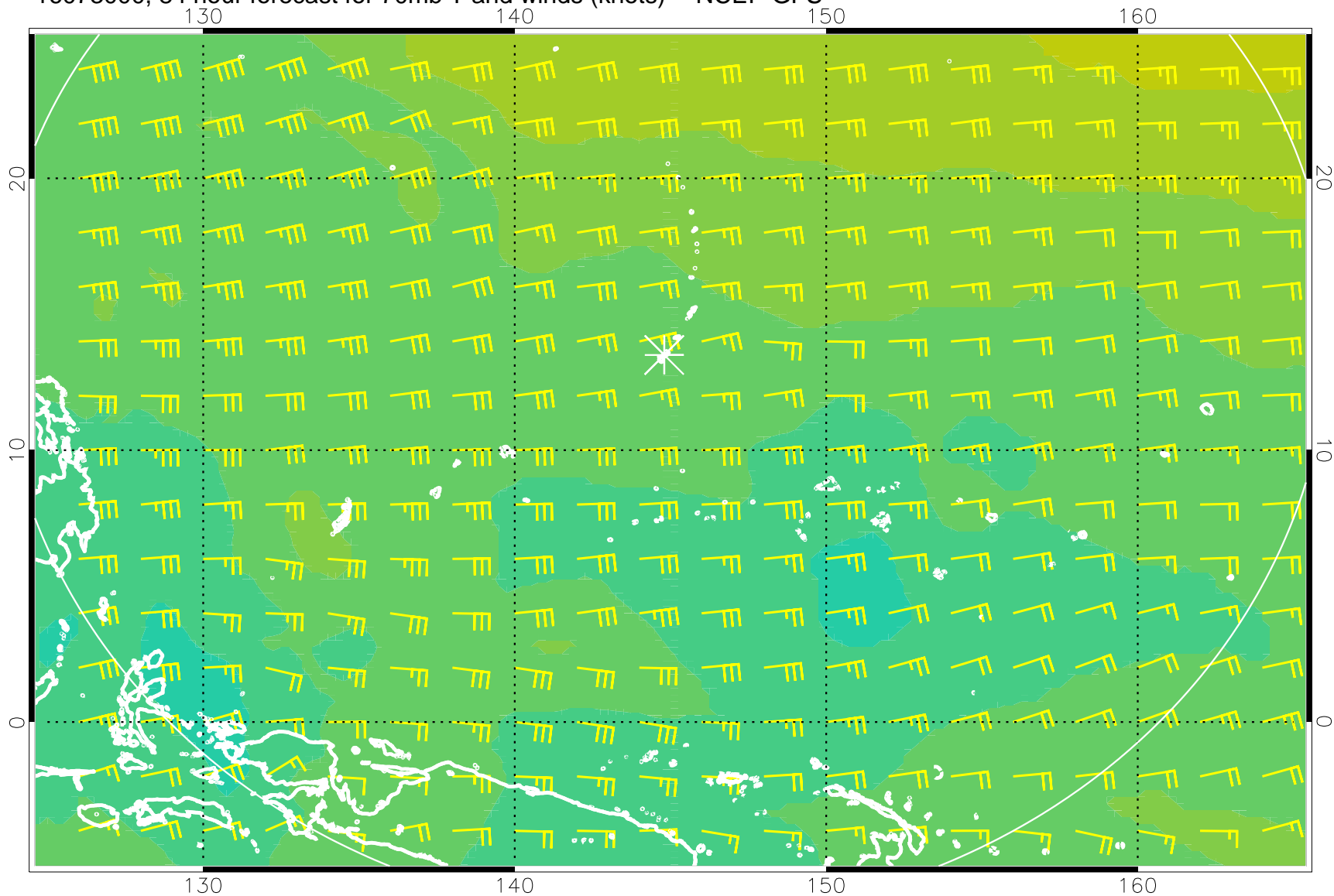
16073000, 84 hour forecast for 70mb T and winds (knots) -- NCEP GFS
