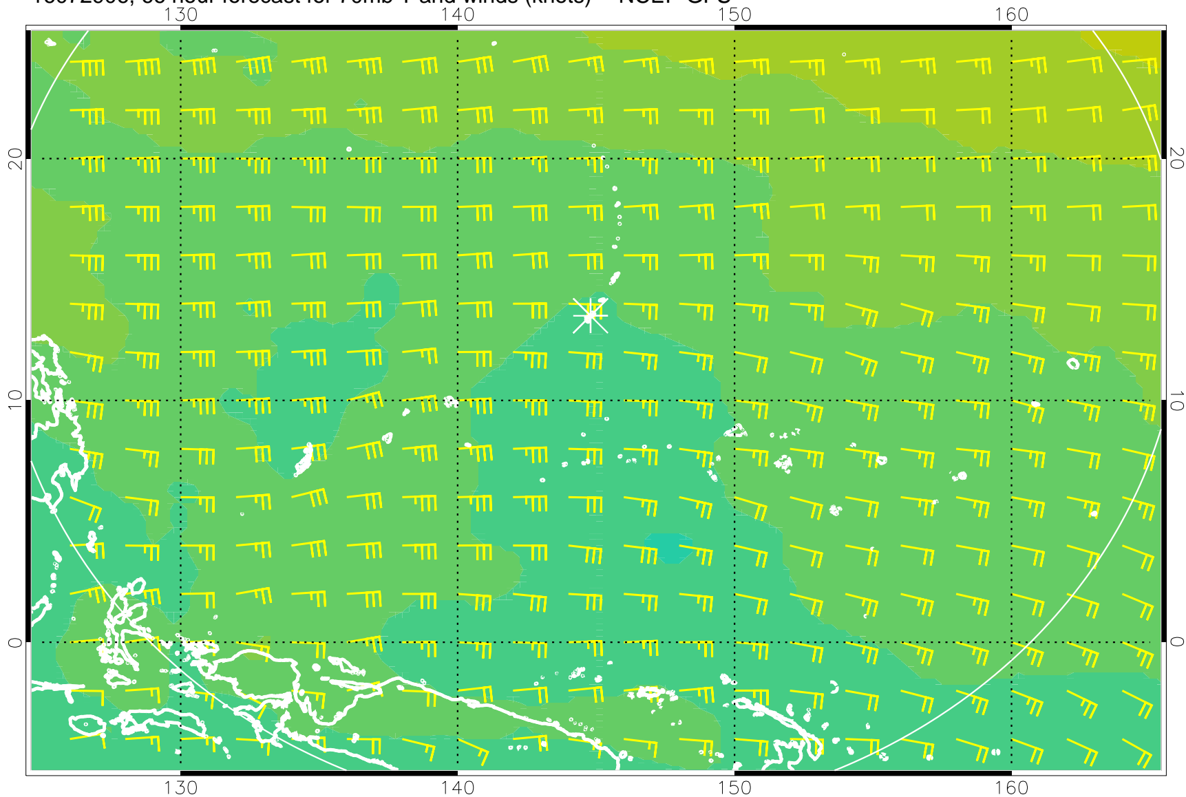
16072906, 66 hour forecast for 70mb T and winds (knots) -- NCEP GFS
