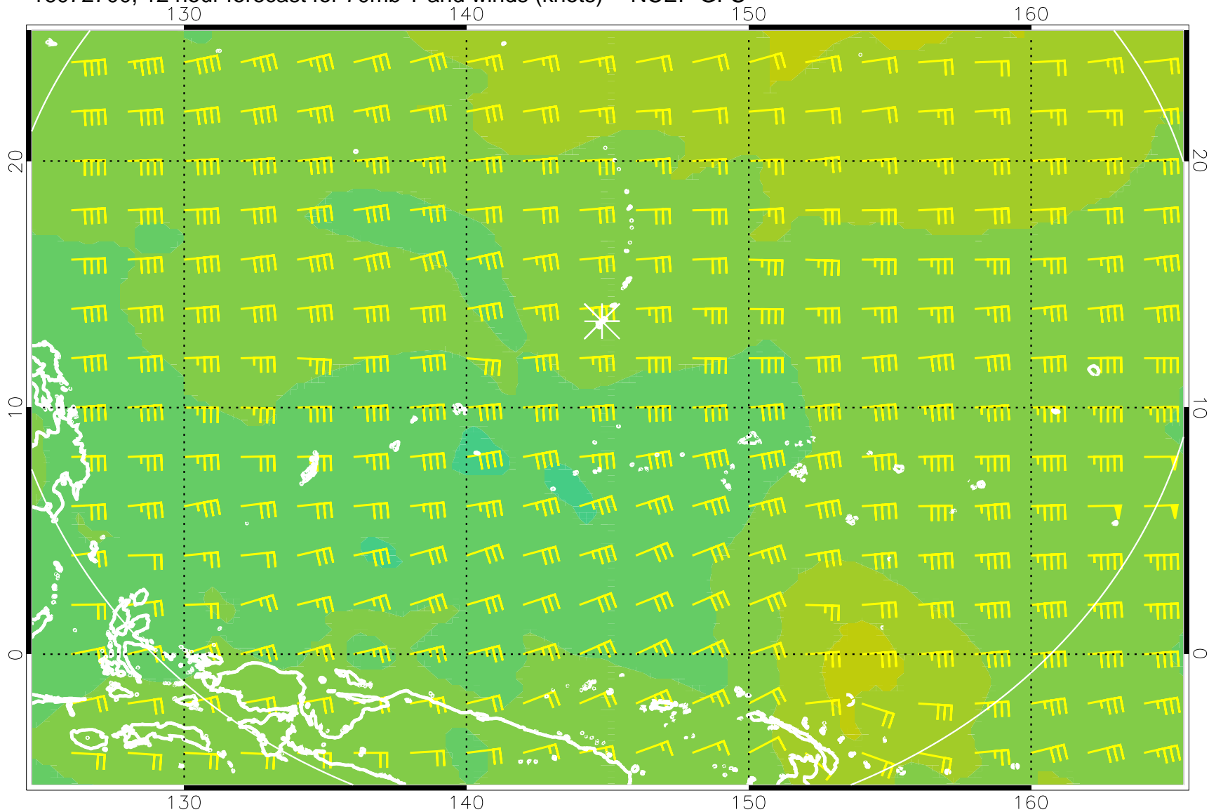
16072700, 12 hour forecast for 70mb T and winds (knots) -- NCEP GFS
