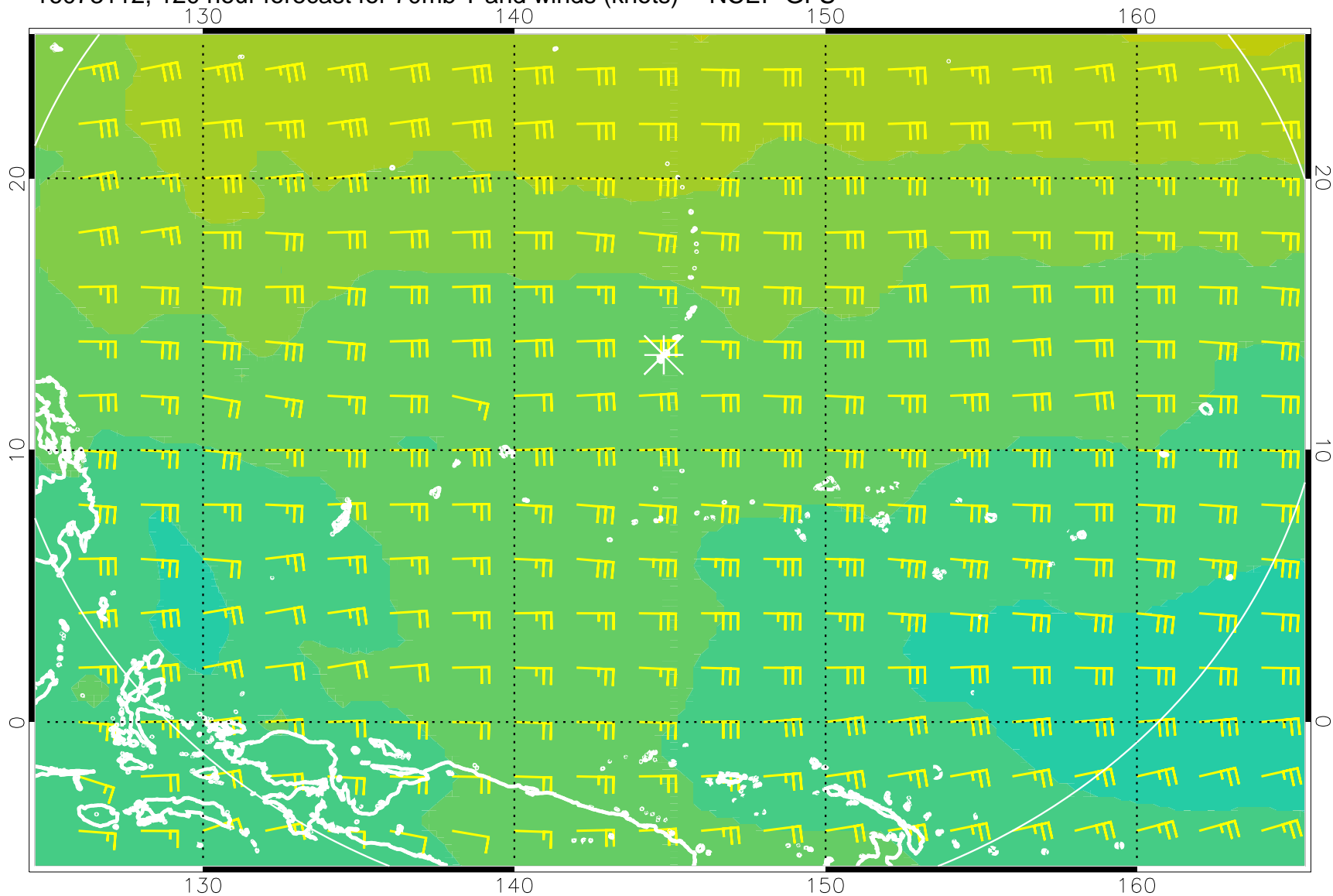
16073112, 120 hour forecast for 70mb T and winds (knots) -- NCEP GFS
