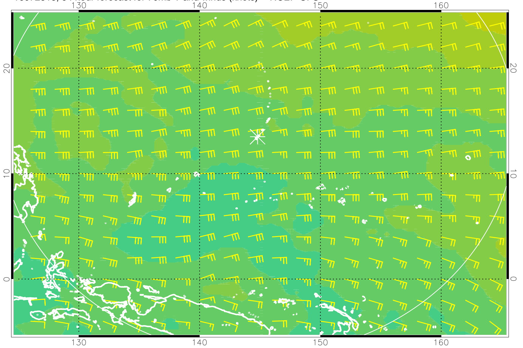
16072818, 54 hour forecast for 70mb T and winds (knots) -- NCEP GFS
