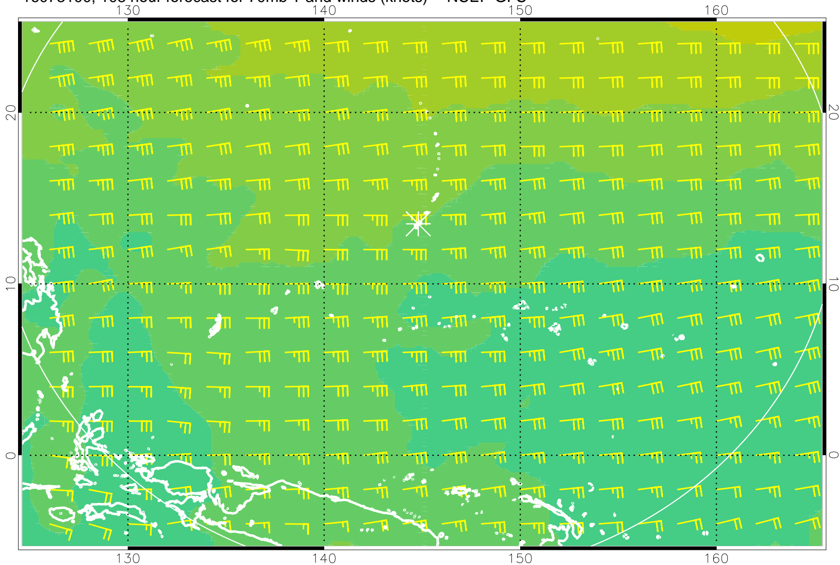
16073100, 108 hour forecast for 70mb T and winds (knots) -- NCEP GFS
