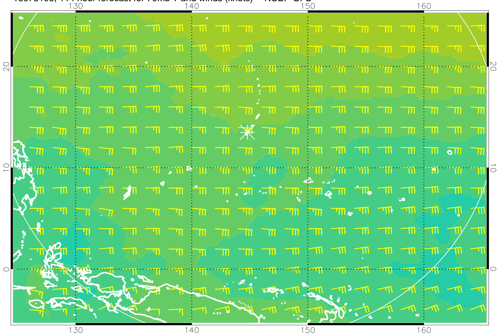
16073106, 114 hour forecast for 70mb T and winds (knots) -- NCEP GFS
