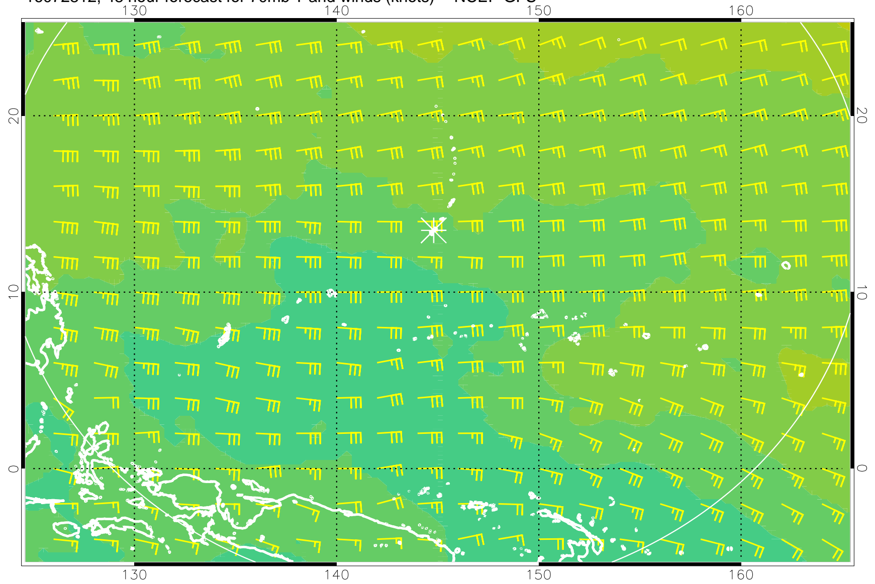
16072812, 48 hour forecast for 70mb T and winds (knots) -- NCEP GFS
