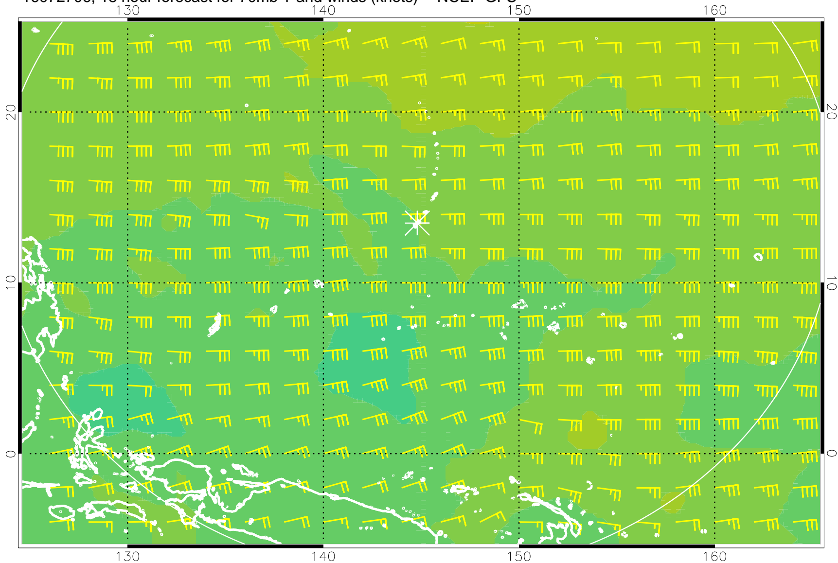
16072706, 18 hour forecast for 70mb T and winds (knots) -- NCEP GFS
