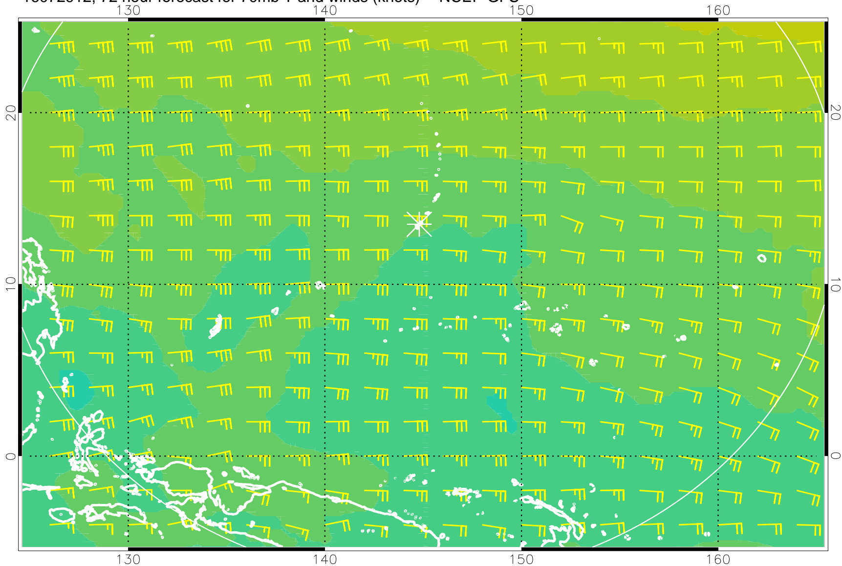
16072912, 72 hour forecast for 70mb T and winds (knots) -- NCEP GFS
