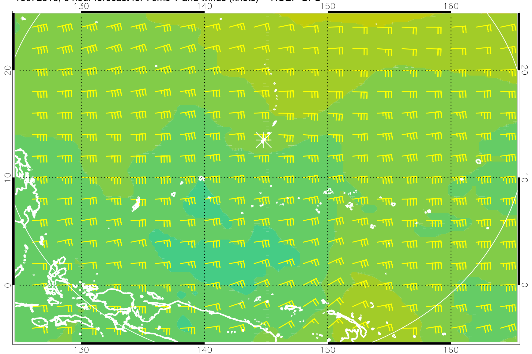
16072618, 6 hour forecast for 70mb T and winds (knots) -- NCEP GFS
