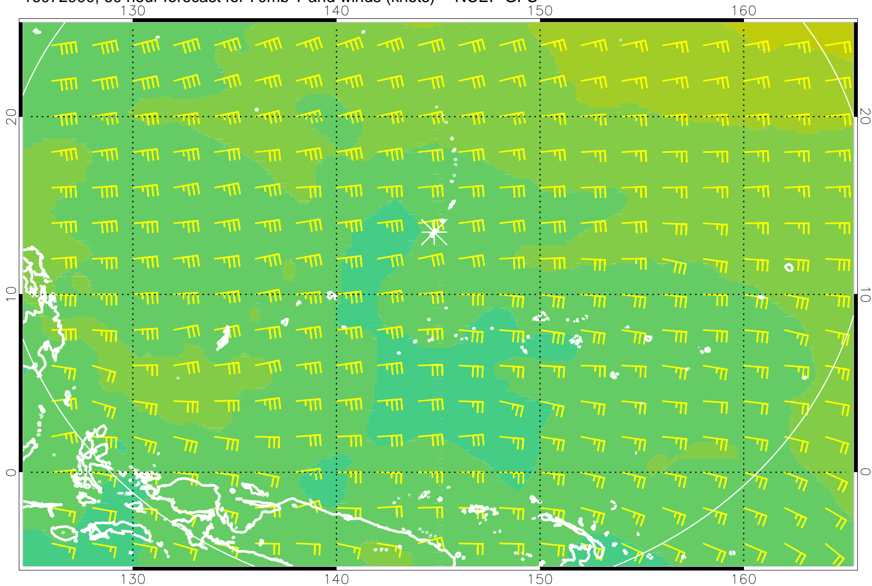
16072900, 60 hour forecast for 70mb T and winds (knots) -- NCEP GFS
