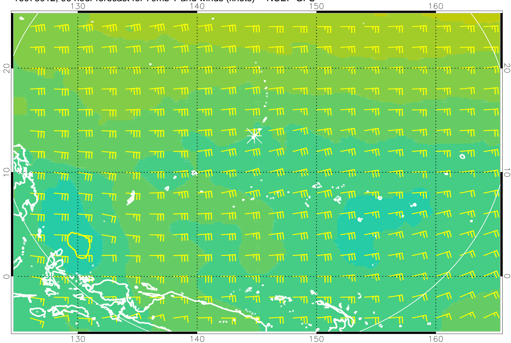
16073012, 96 hour forecast for 70mb T and winds (knots) -- NCEP GFS
