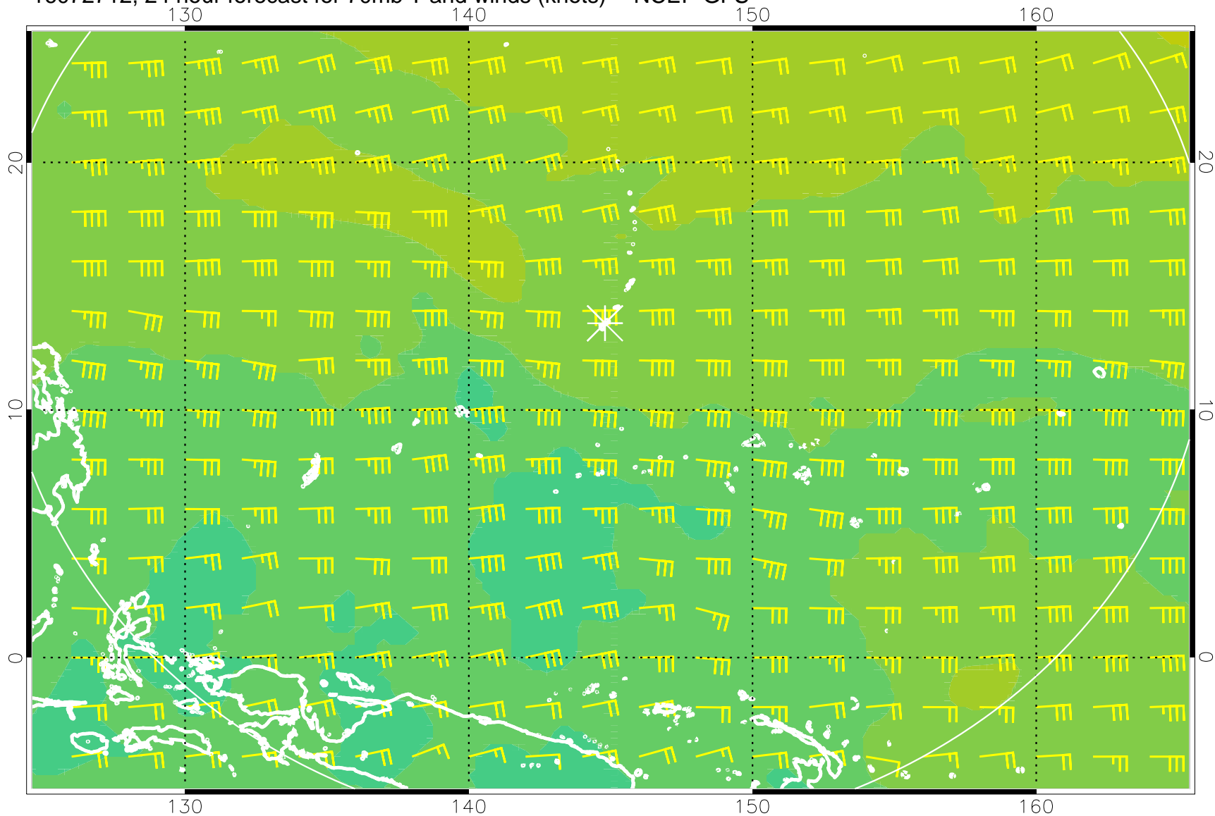
16072712, 24 hour forecast for 70mb T and winds (knots) -- NCEP GFS
