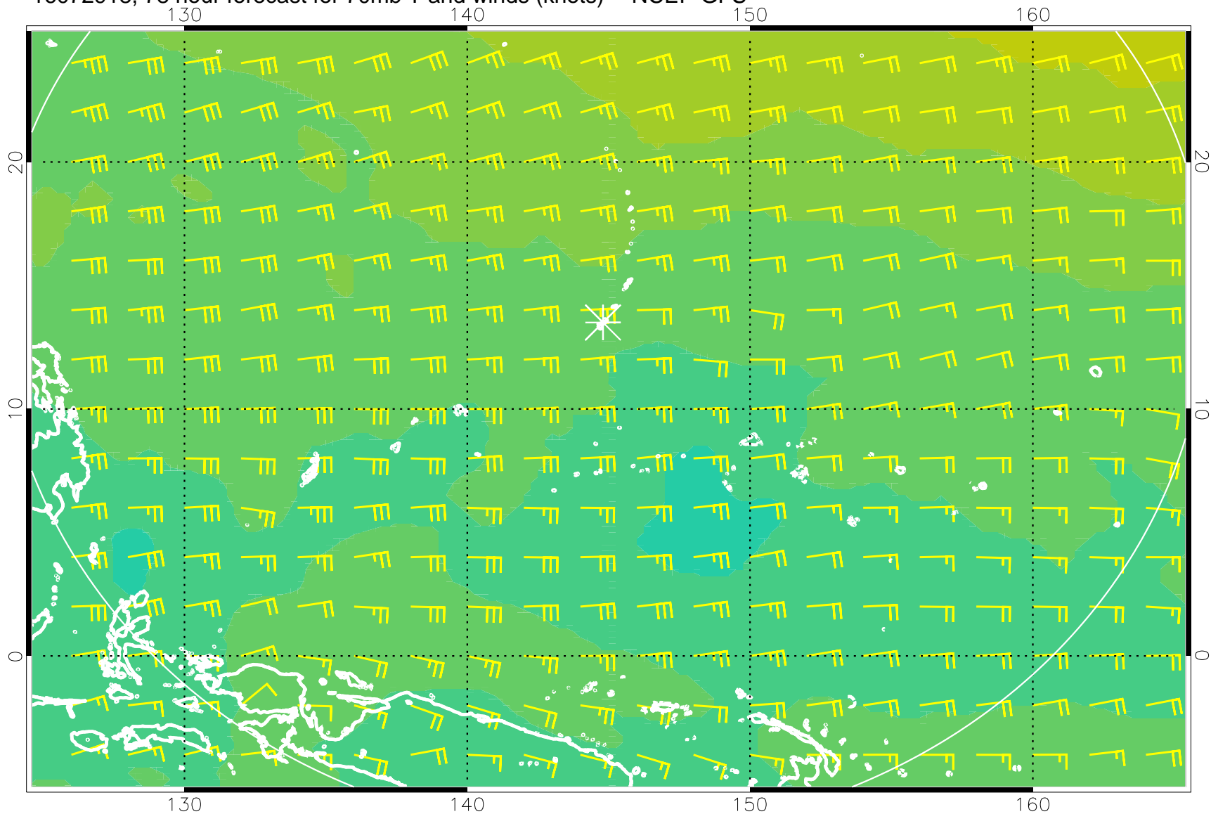
16072918, 78 hour forecast for 70mb T and winds (knots) -- NCEP GFS
