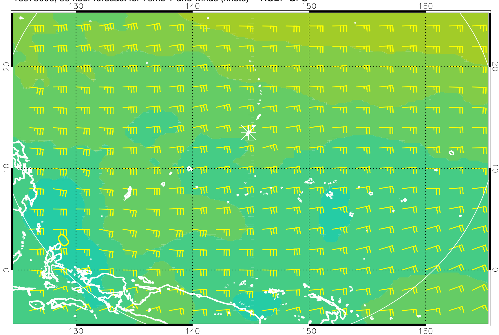
16073006, 90 hour forecast for 70mb T and winds (knots) -- NCEP GFS
