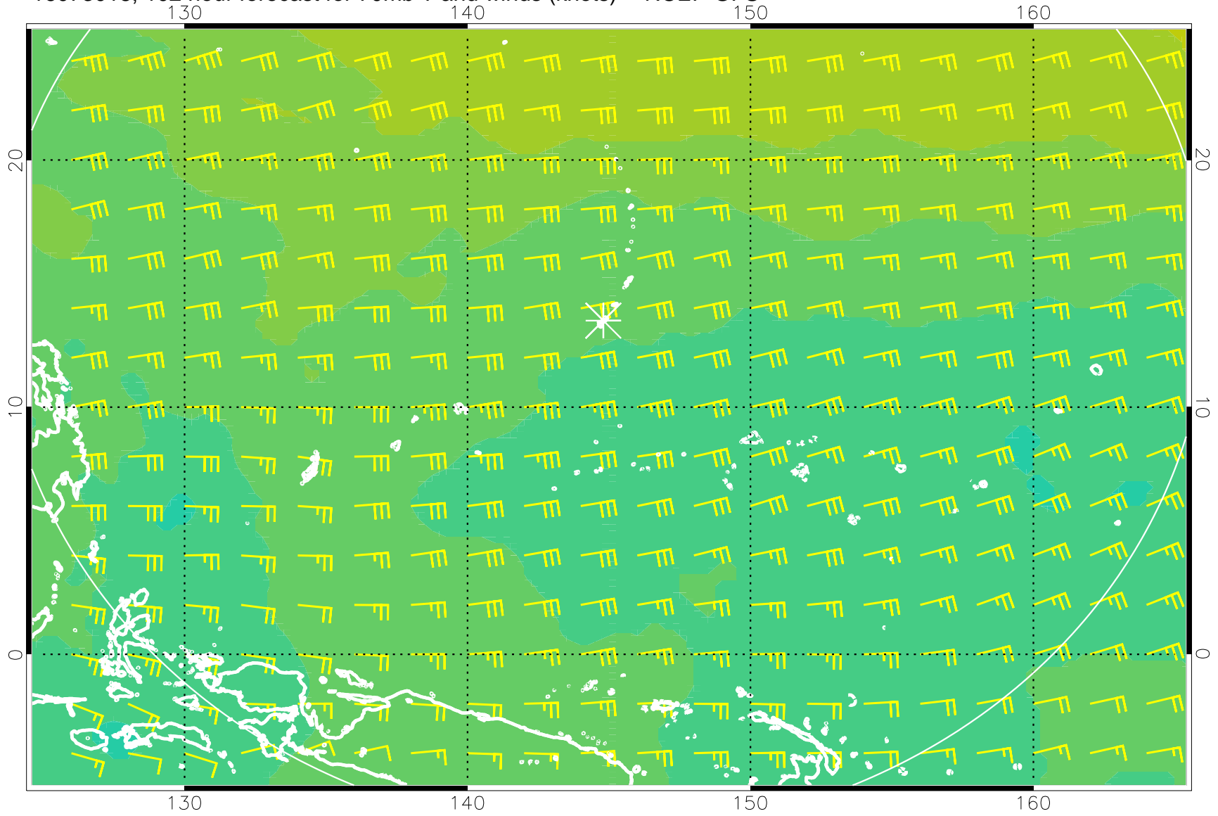
16073018, 102 hour forecast for 70mb T and winds (knots) -- NCEP GFS
