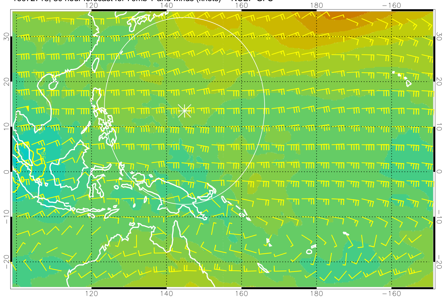
16072718, 30 hour forecast for 70mb T and winds (knots) -- NCEP GFS
