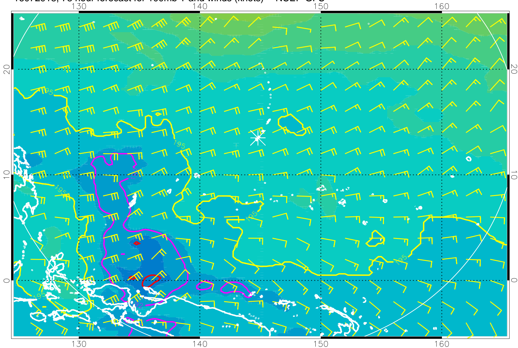
16072918, 78 hour forecast for 100mb T and winds (knots) -- NCEP GFS
