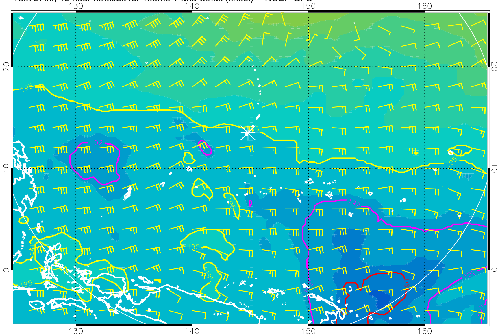
16072700, 12 hour forecast for 100mb T and winds (knots) -- NCEP GFS
