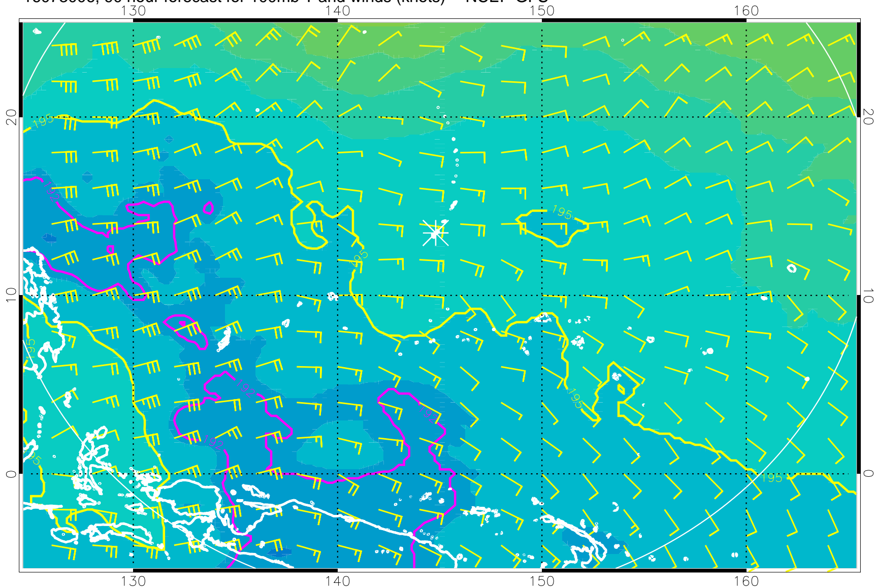
16073006, 90 hour forecast for 100mb T and winds (knots) -- NCEP GFS
