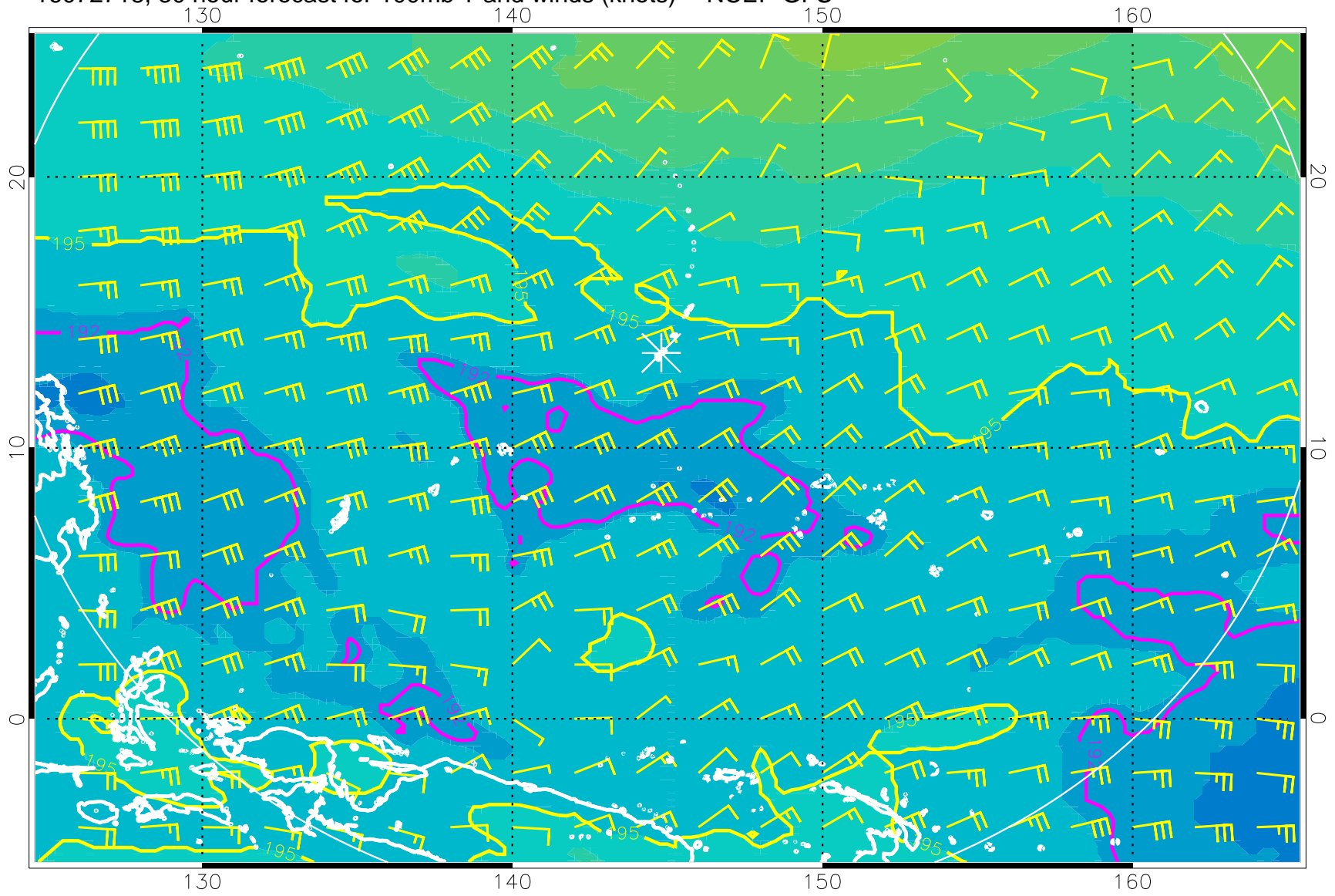
16072718, 30 hour forecast for 100mb T and winds (knots) -- NCEP GFS
