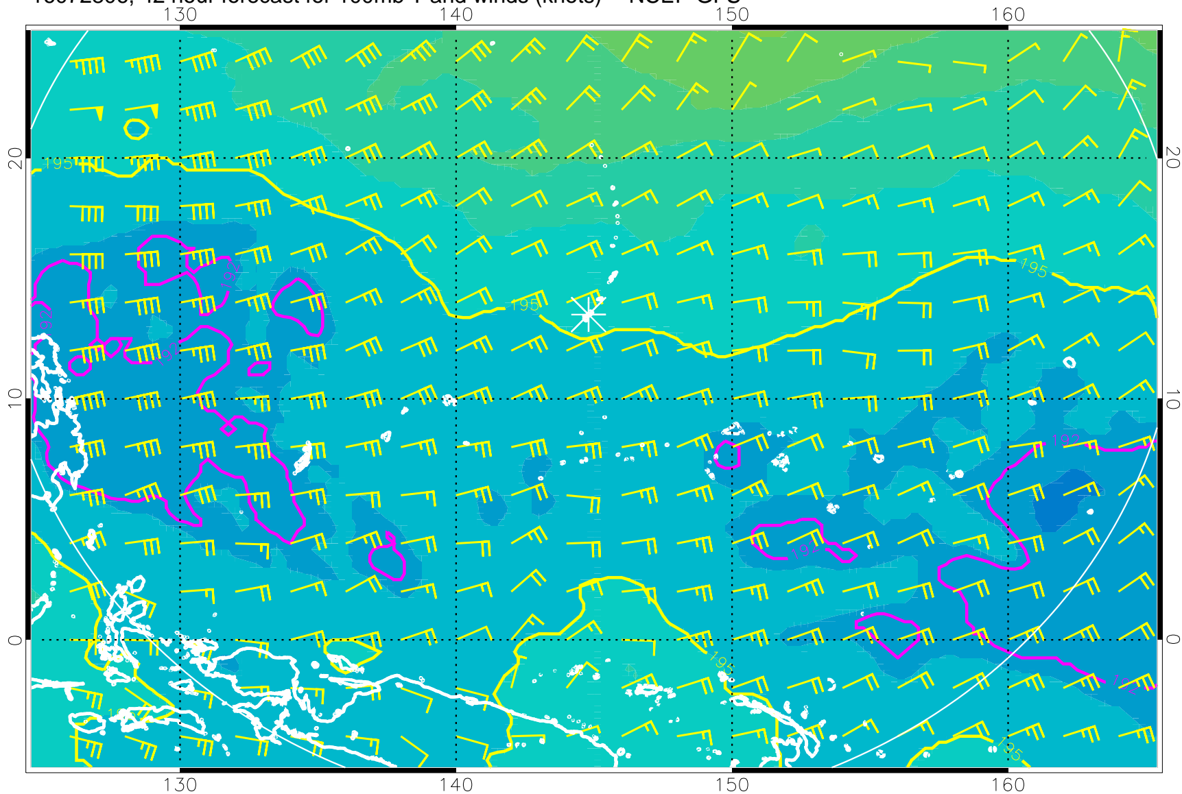
16072806, 42 hour forecast for 100mb T and winds (knots) -- NCEP GFS
