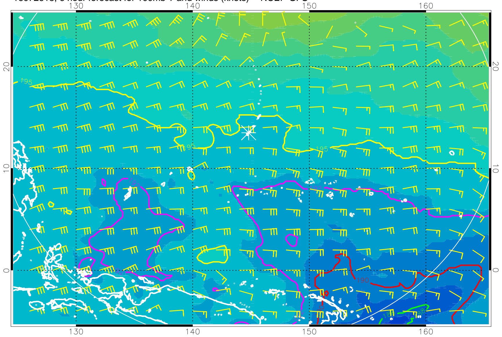
16072618, 6 hour forecast for 100mb T and winds (knots) -- NCEP GFS
