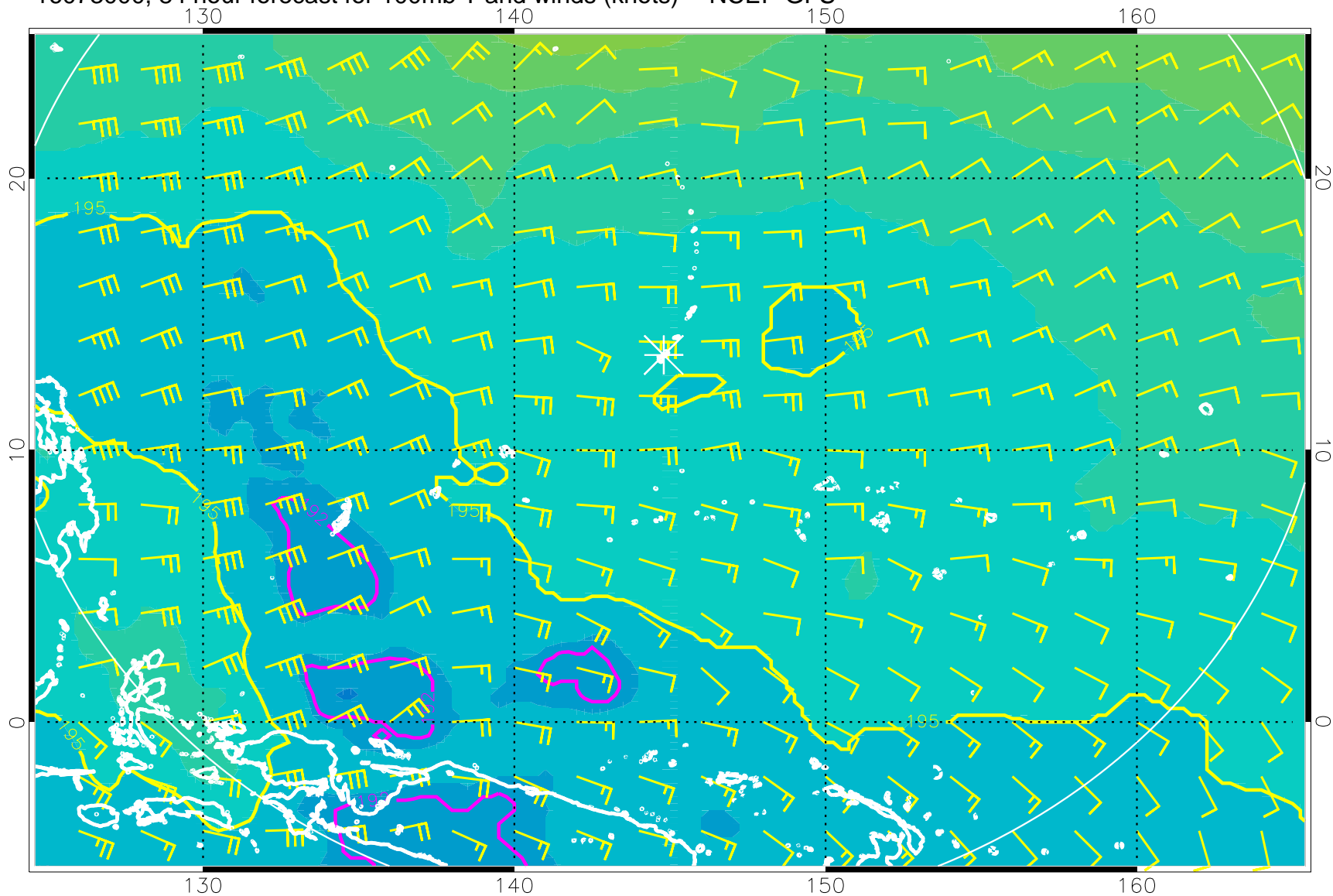
16073000, 84 hour forecast for 100mb T and winds (knots) -- NCEP GFS
