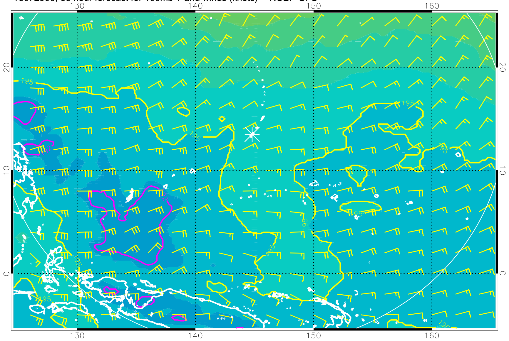
16072906, 66 hour forecast for 100mb T and winds (knots) -- NCEP GFS
