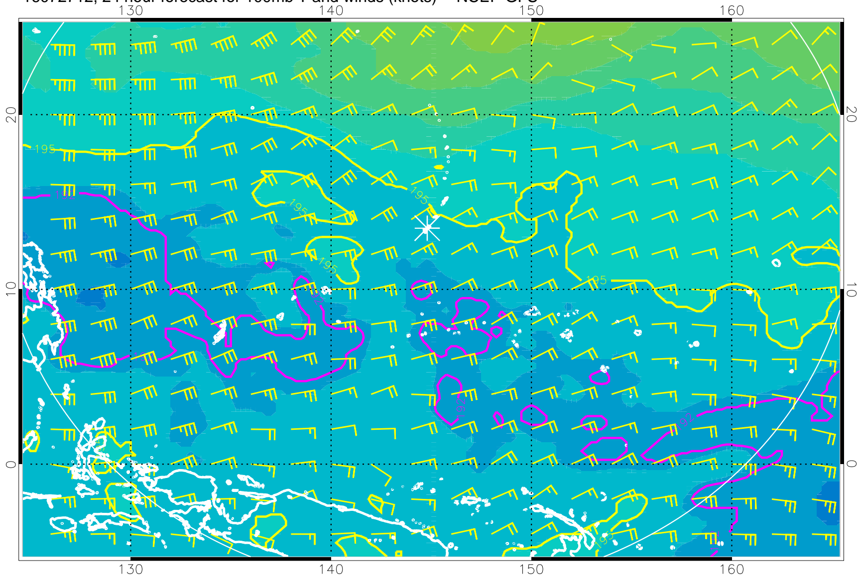
16072712, 24 hour forecast for 100mb T and winds (knots) -- NCEP GFS
