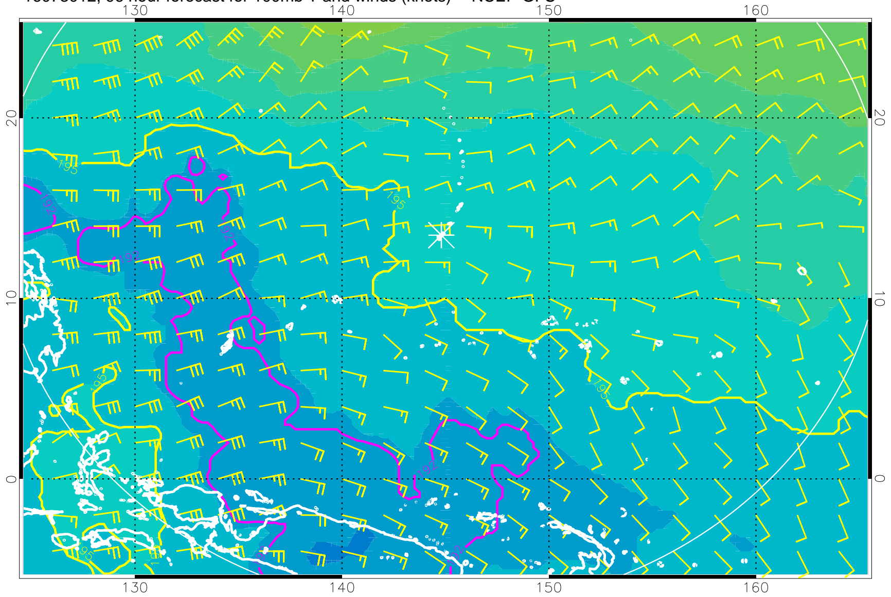
16073012, 96 hour forecast for 100mb T and winds (knots) -- NCEP GFS
