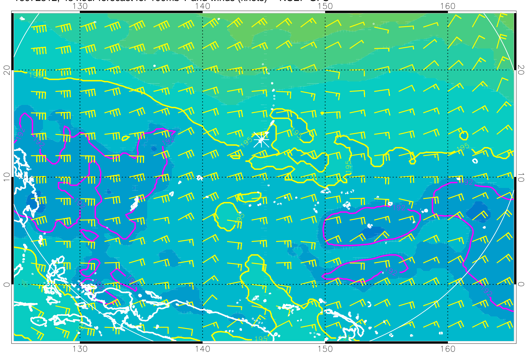
16072812, 48 hour forecast for 100mb T and winds (knots) -- NCEP GFS
