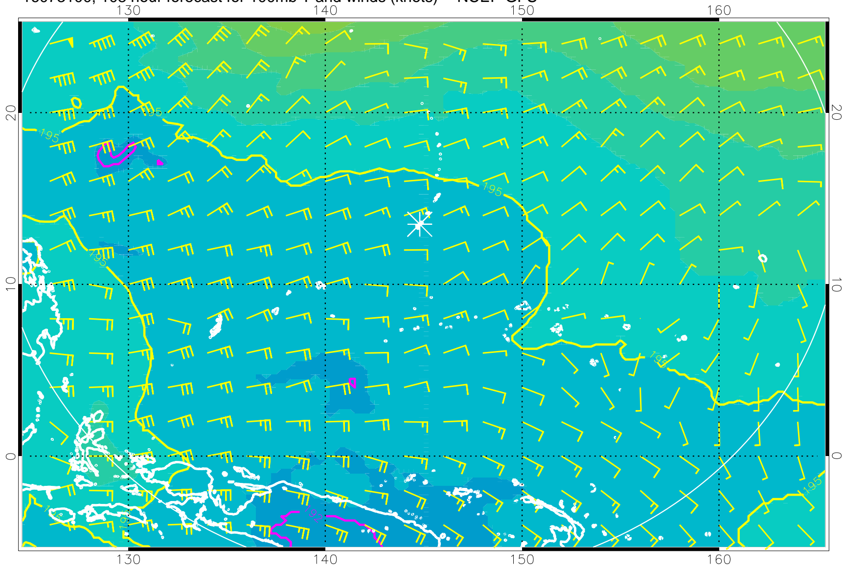
16073100, 108 hour forecast for 100mb T and winds (knots) -- NCEP GFS
