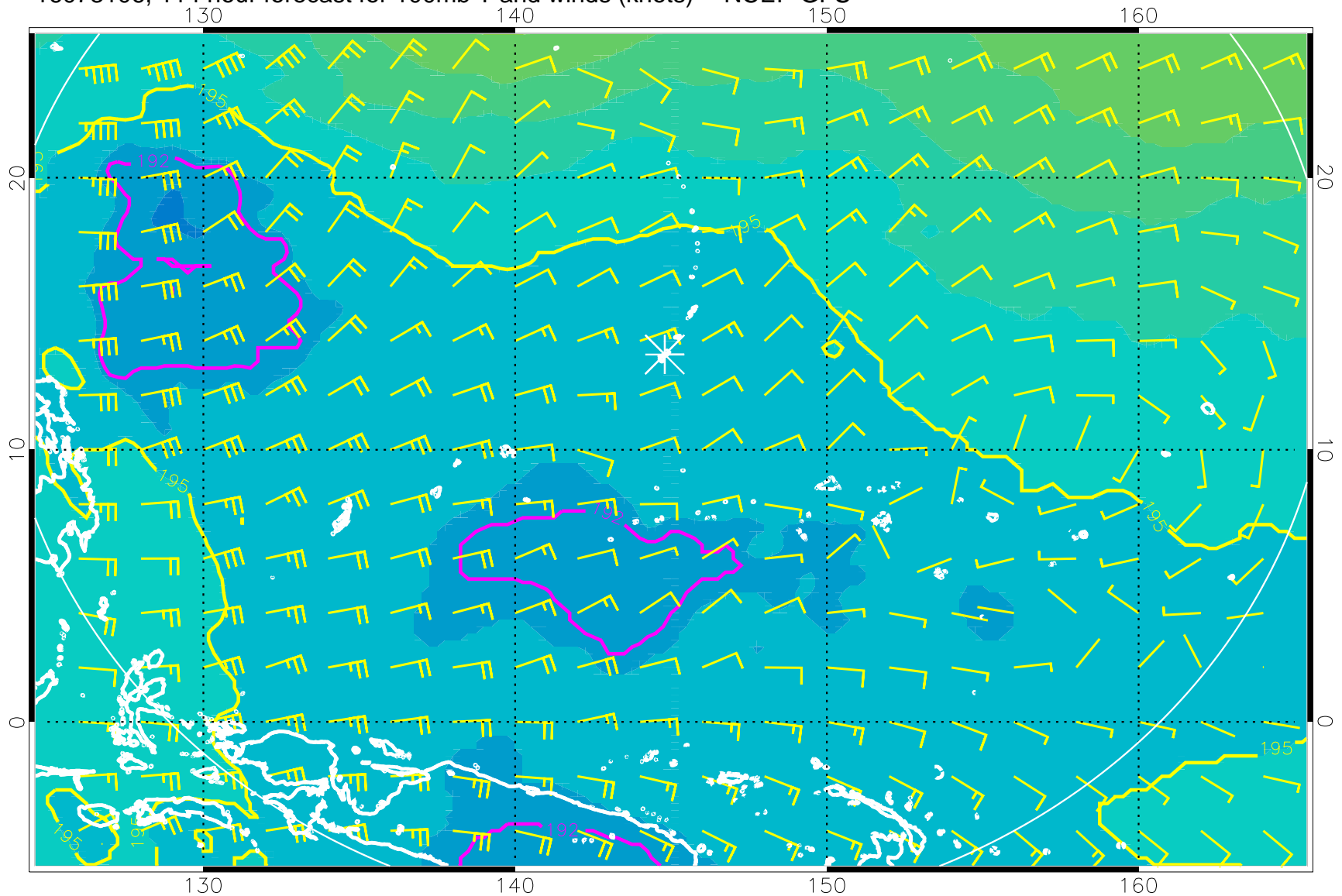
16073106, 114 hour forecast for 100mb T and winds (knots) -- NCEP GFS
