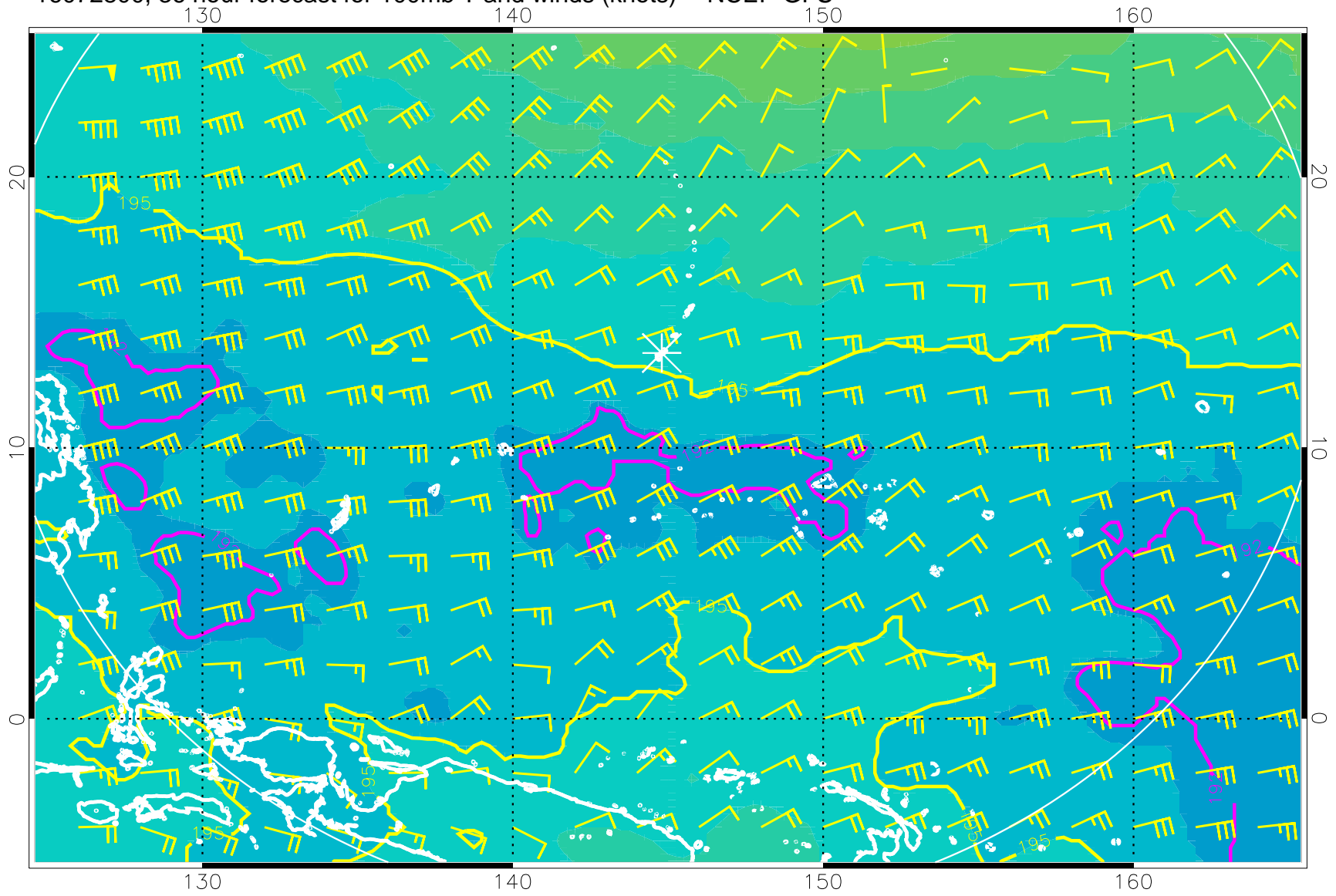
16072800, 36 hour forecast for 100mb T and winds (knots) -- NCEP GFS
