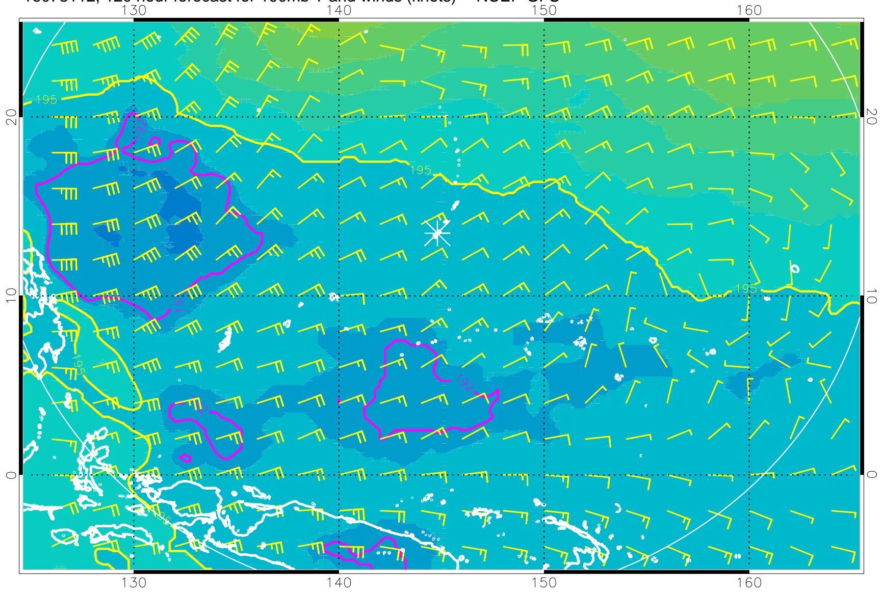
16073112, 120 hour forecast for 100mb T and winds (knots) -- NCEP GFS
