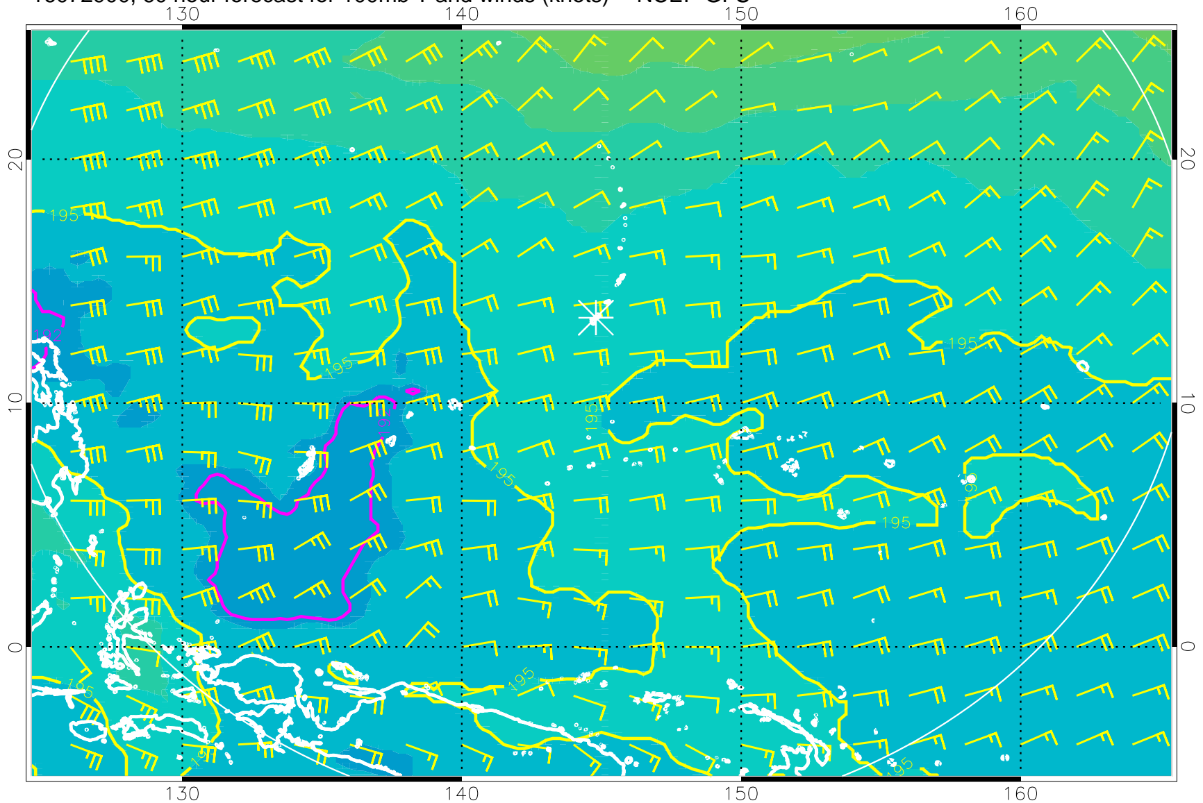
16072900, 60 hour forecast for 100mb T and winds (knots) -- NCEP GFS
