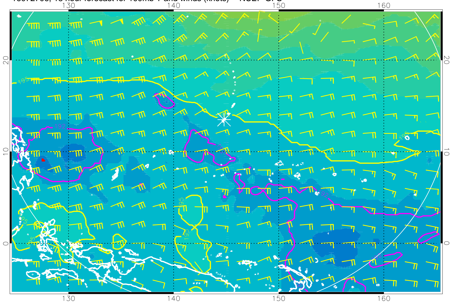
16072706, 18 hour forecast for 100mb T and winds (knots) -- NCEP GFS
