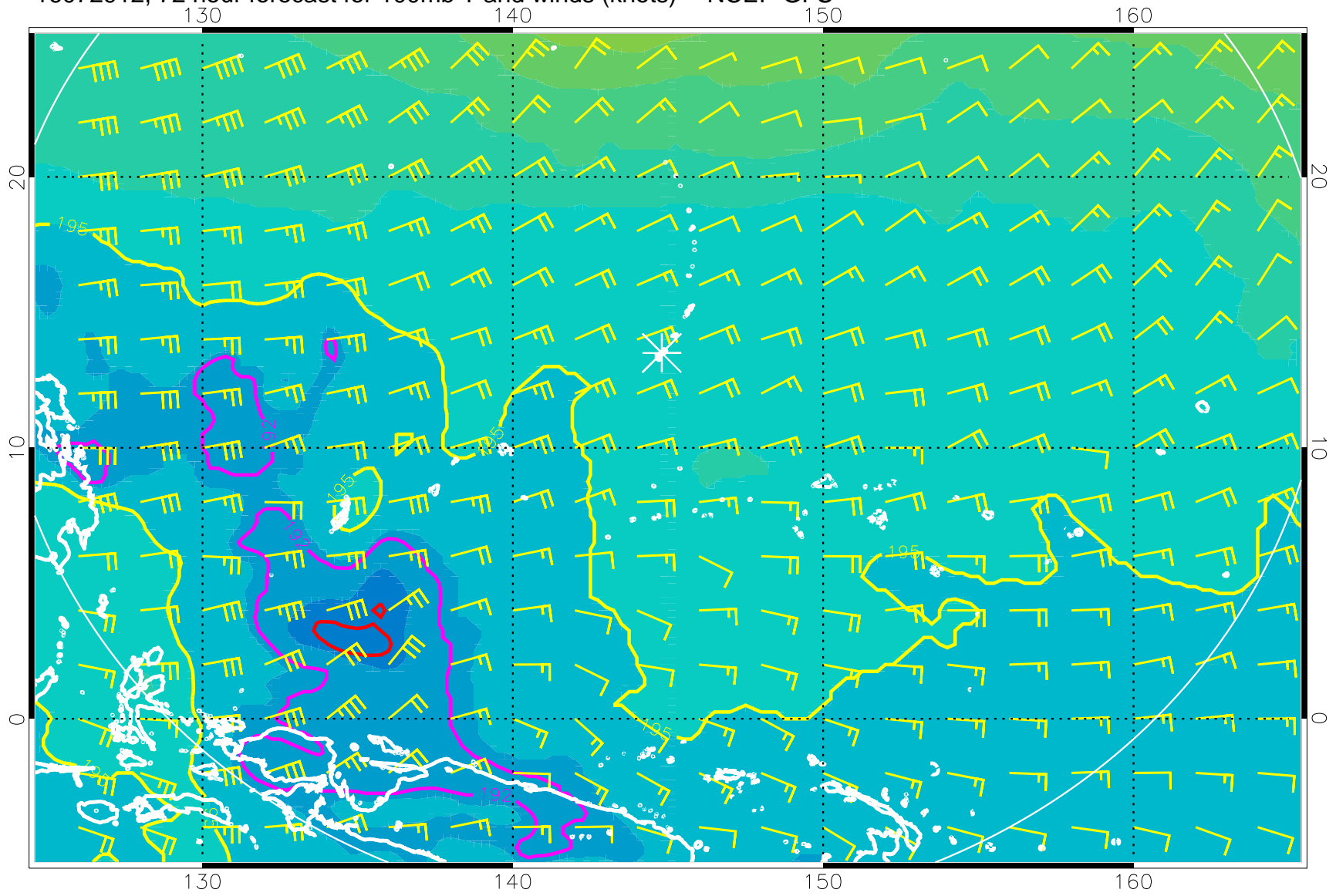
16072912, 72 hour forecast for 100mb T and winds (knots) -- NCEP GFS
