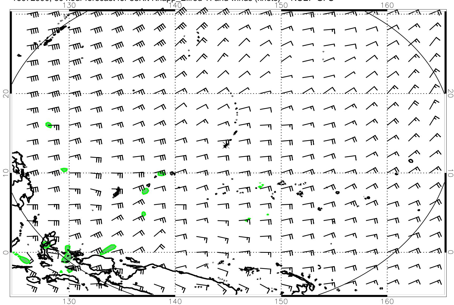
16072900, 60 hour forecast for 53Kft Knapp_Ellrod TI and winds (knots) -- NCEP GFS
