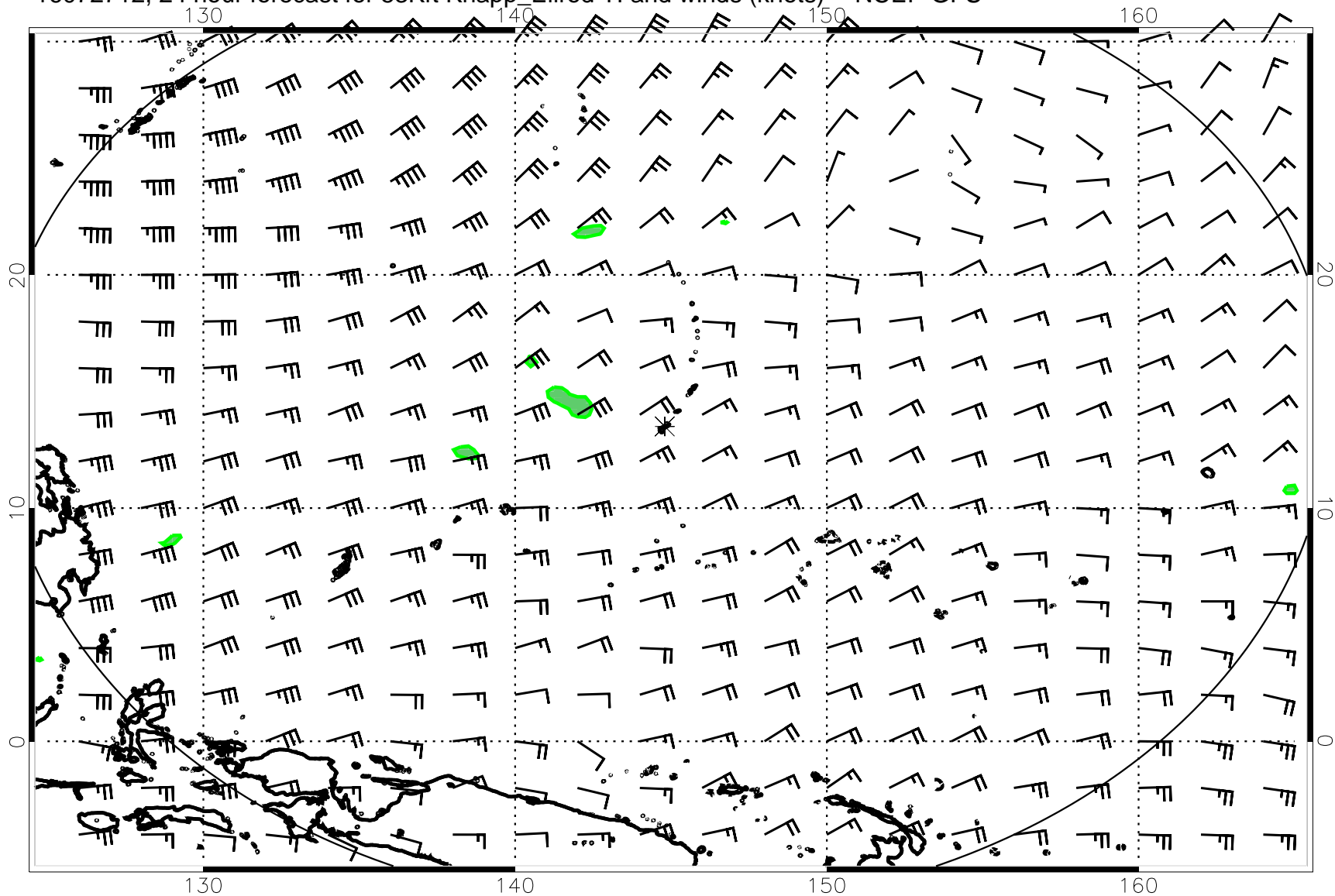
16072712, 24 hour forecast for 53Kft Knapp_Ellrod TI and winds (knots) -- NCEP GFS
