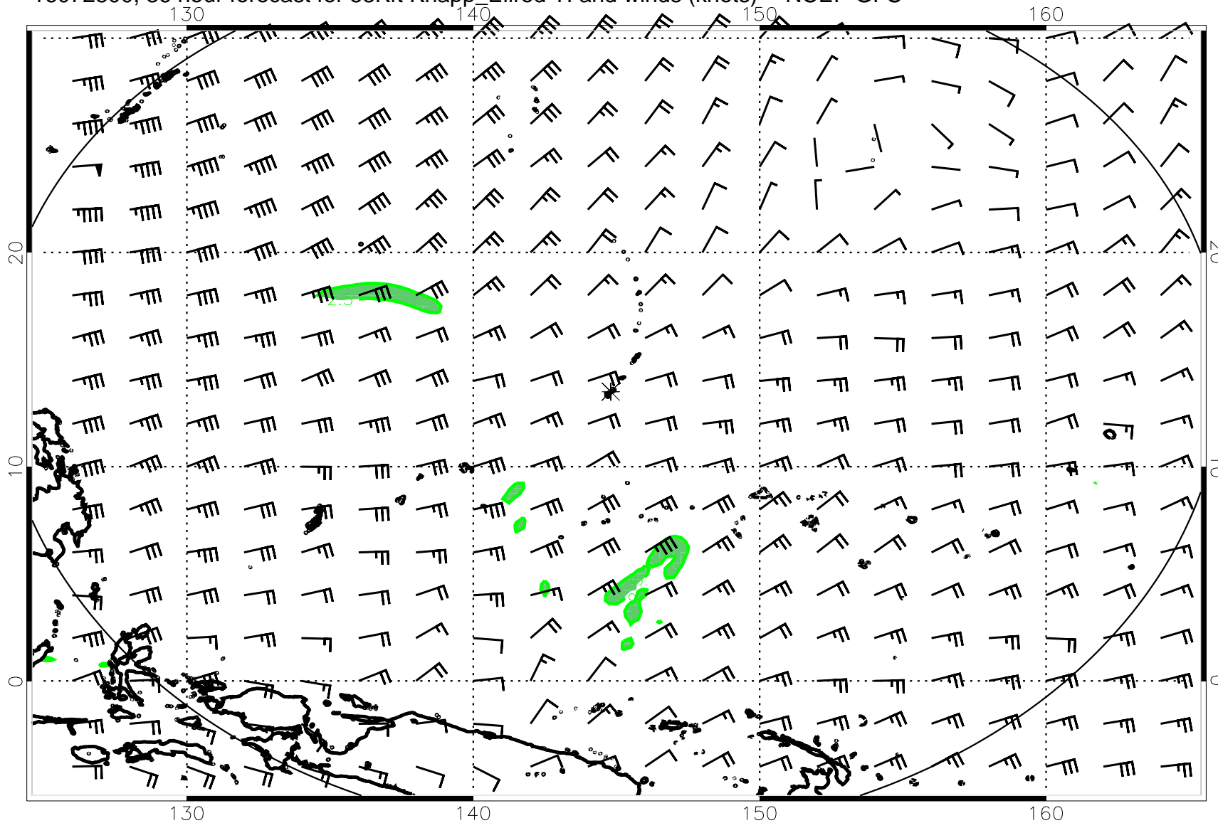
16072800, 36 hour forecast for 53Kft Knapp_Ellrod TI and winds (knots) -- NCEP GFS
