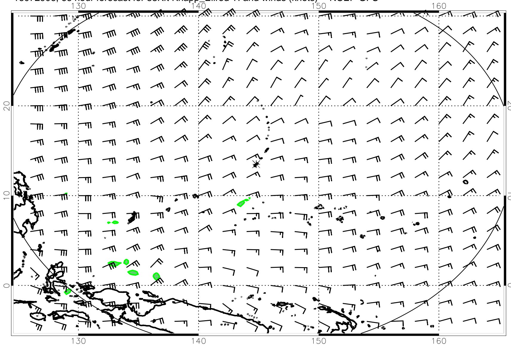
16072906, 66 hour forecast for 53Kft Knapp_Ellrod TI and winds (knots) -- NCEP GFS
