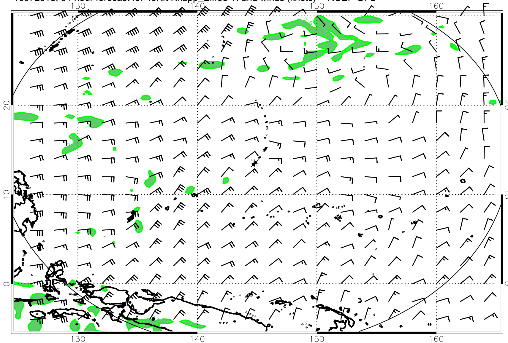
16072818, 54 hour forecast for 49Kft Knapp_Ellrod TI and winds (knots) -- NCEP GFS
