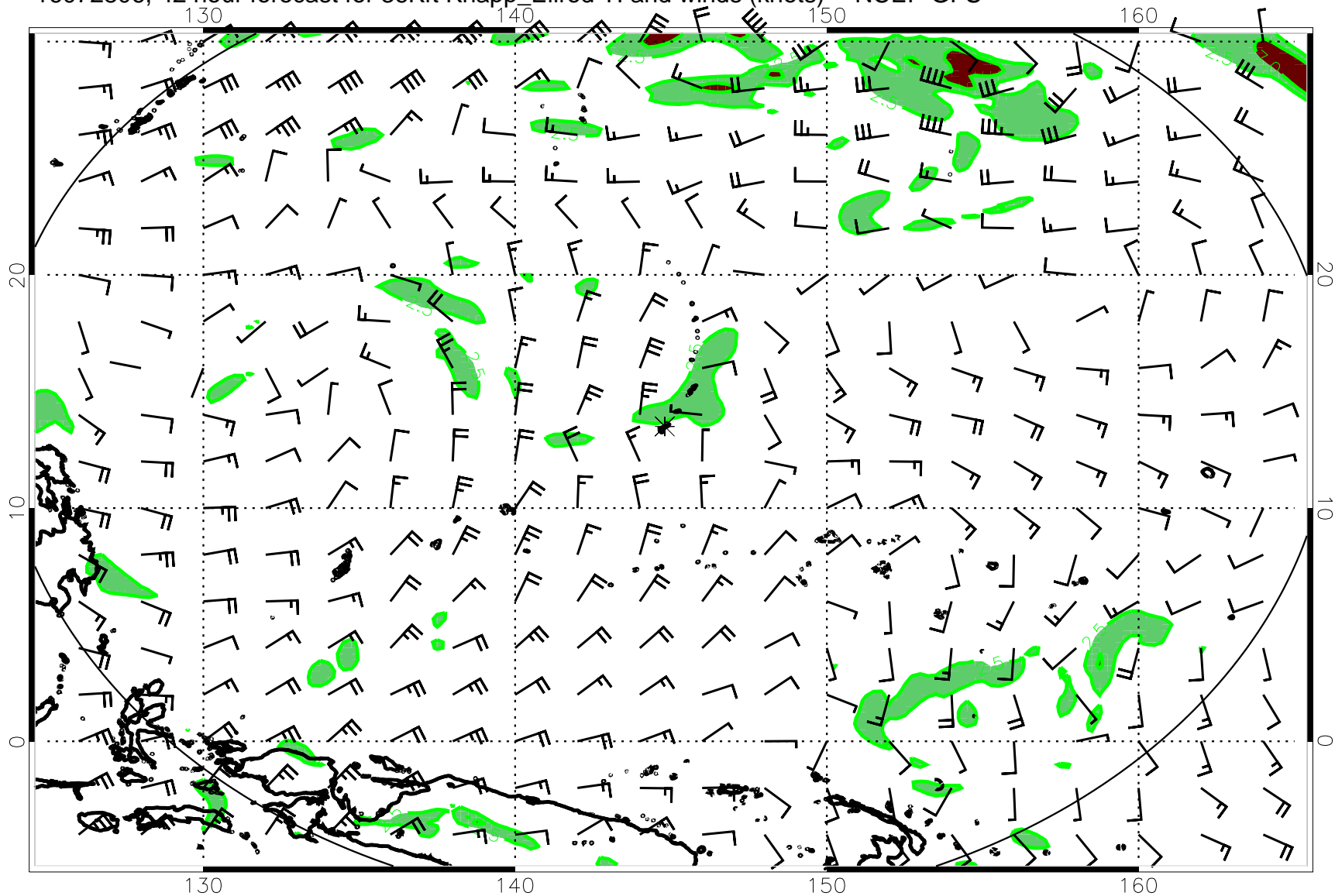
16072806, 42 hour forecast for 36Kft Knapp_Ellrod TI and winds (knots) -- NCEP GFS
