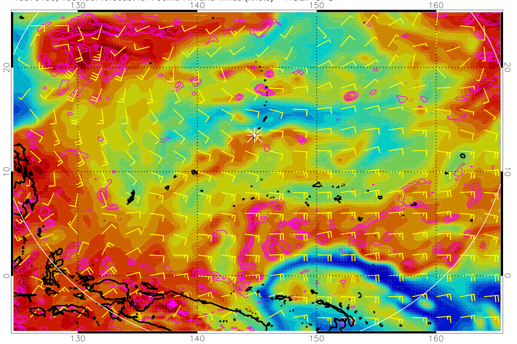
16073100, 108 hour forecast for 700mb RH and winds (knots) -- NCEP GFS
