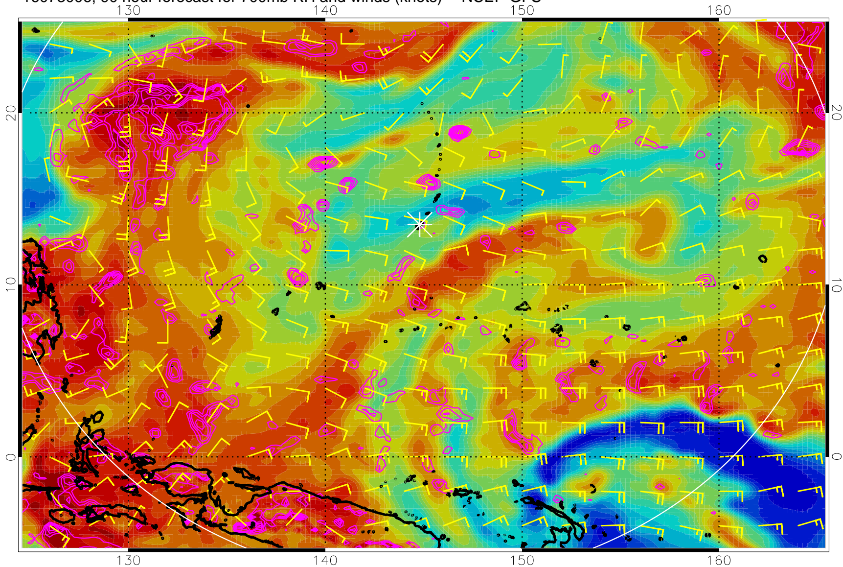
16073006, 90 hour forecast for 700mb RH and winds (knots) -- NCEP GFS
