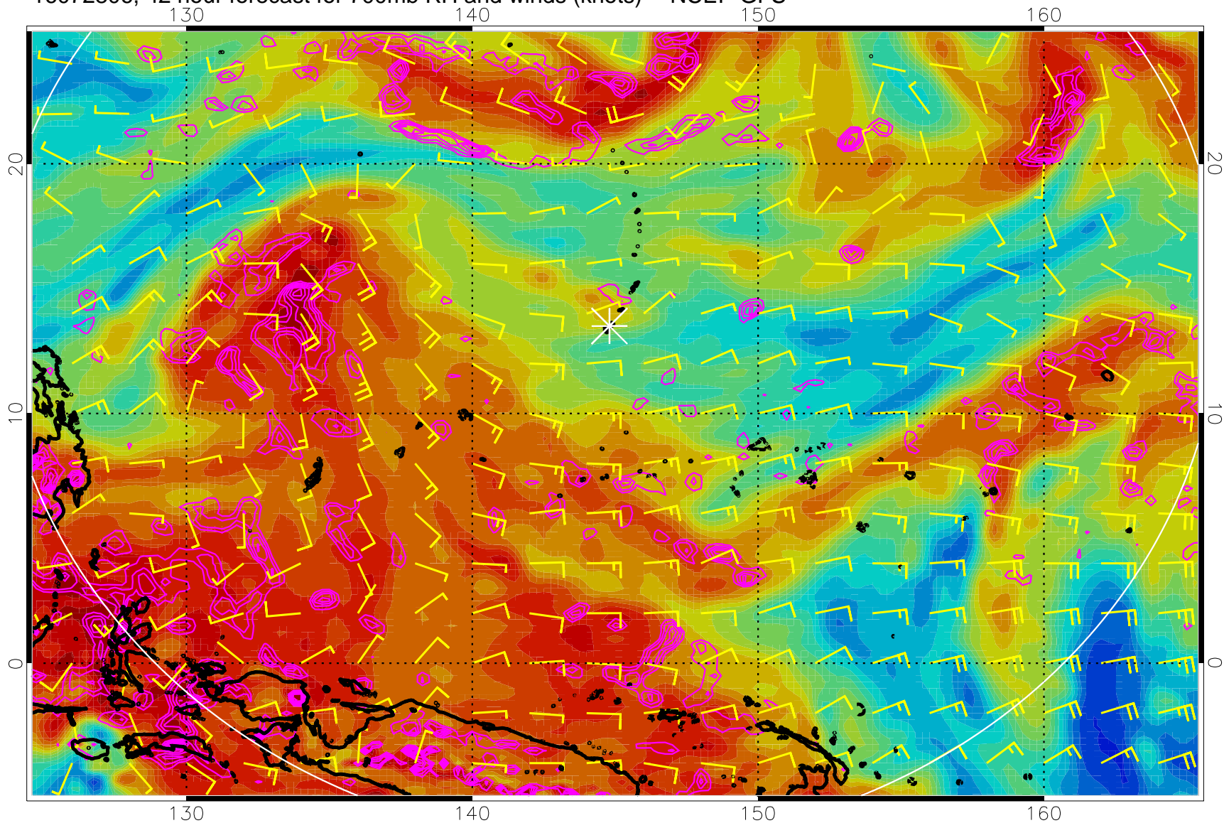
16072806, 42 hour forecast for 700mb RH and winds (knots) -- NCEP GFS
