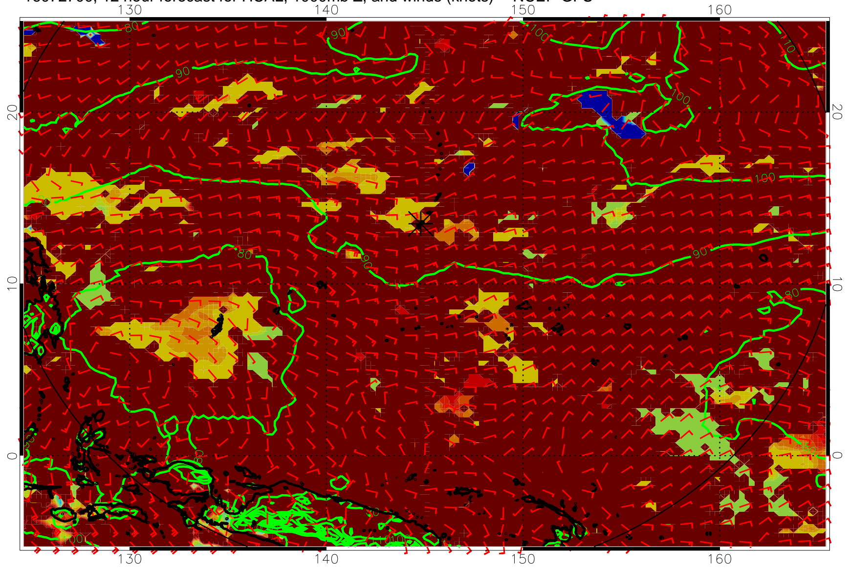
16072700, 12 hour forecast for HCAL, 1000mb Z, and winds (knots) -- NCEP GFS
