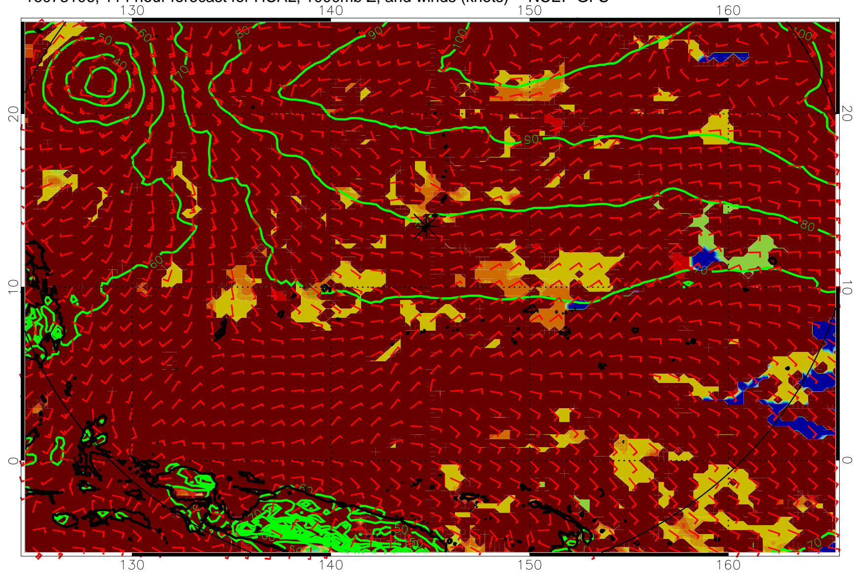
16073106, 114 hour forecast for HCAL, 1000mb Z, and winds (knots) -- NCEP GFS
