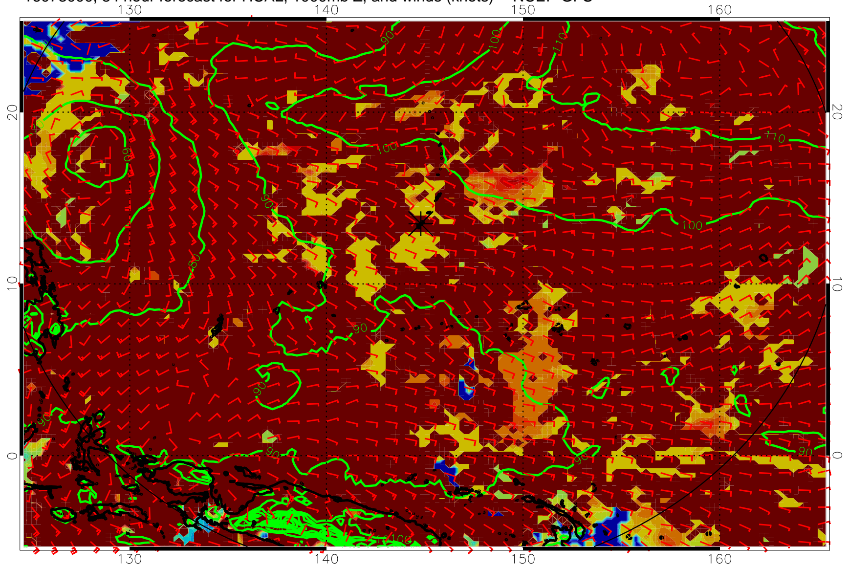
16073000, 84 hour forecast for HCAL, 1000mb Z, and winds (knots) -- NCEP GFS
