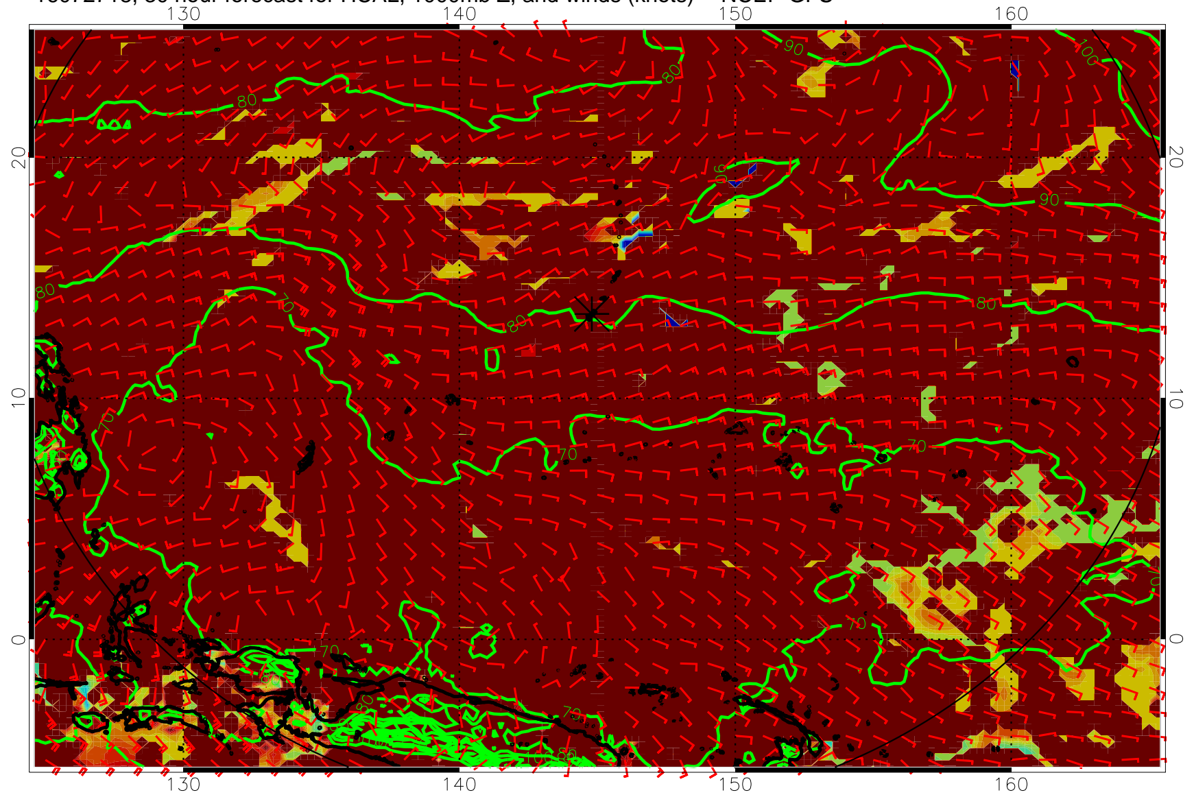
16072718, 30 hour forecast for HCAL, 1000mb Z, and winds (knots) -- NCEP GFS
