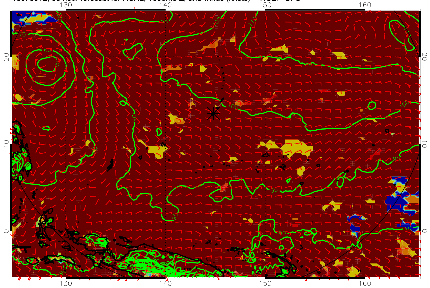
16073012, 96 hour forecast for HCAL, 1000mb Z, and winds (knots) -- NCEP GFS
