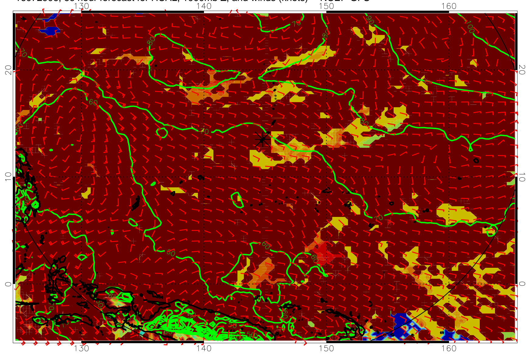
16072906, 66 hour forecast for HCAL, 1000mb Z, and winds (knots) -- NCEP GFS
