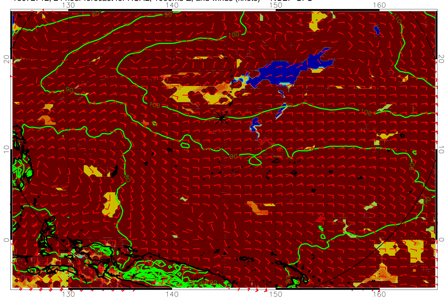
16072712, 24 hour forecast for HCAL, 1000mb Z, and winds (knots) -- NCEP GFS
