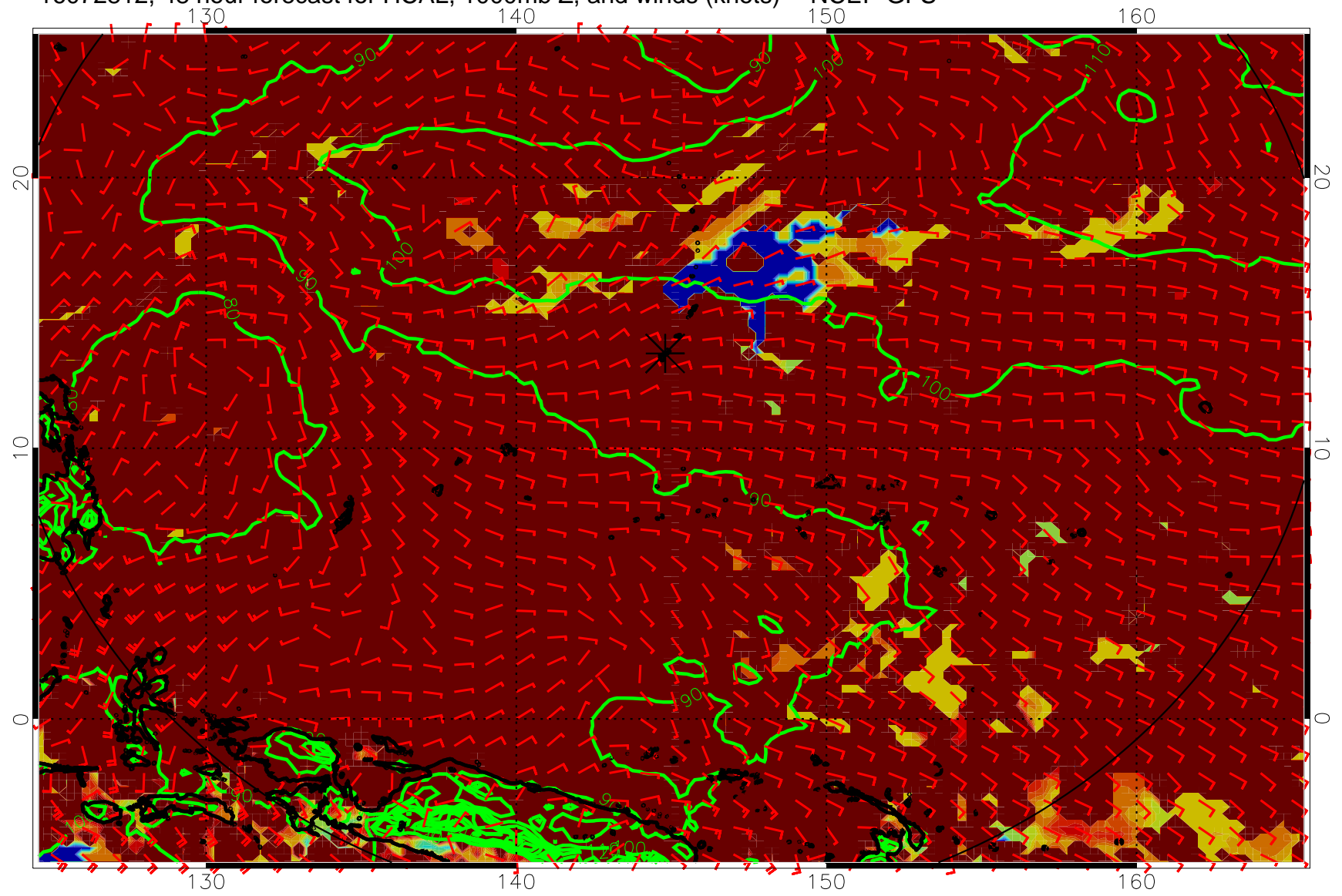
16072812, 48 hour forecast for HCAL, 1000mb Z, and winds (knots) -- NCEP GFS
