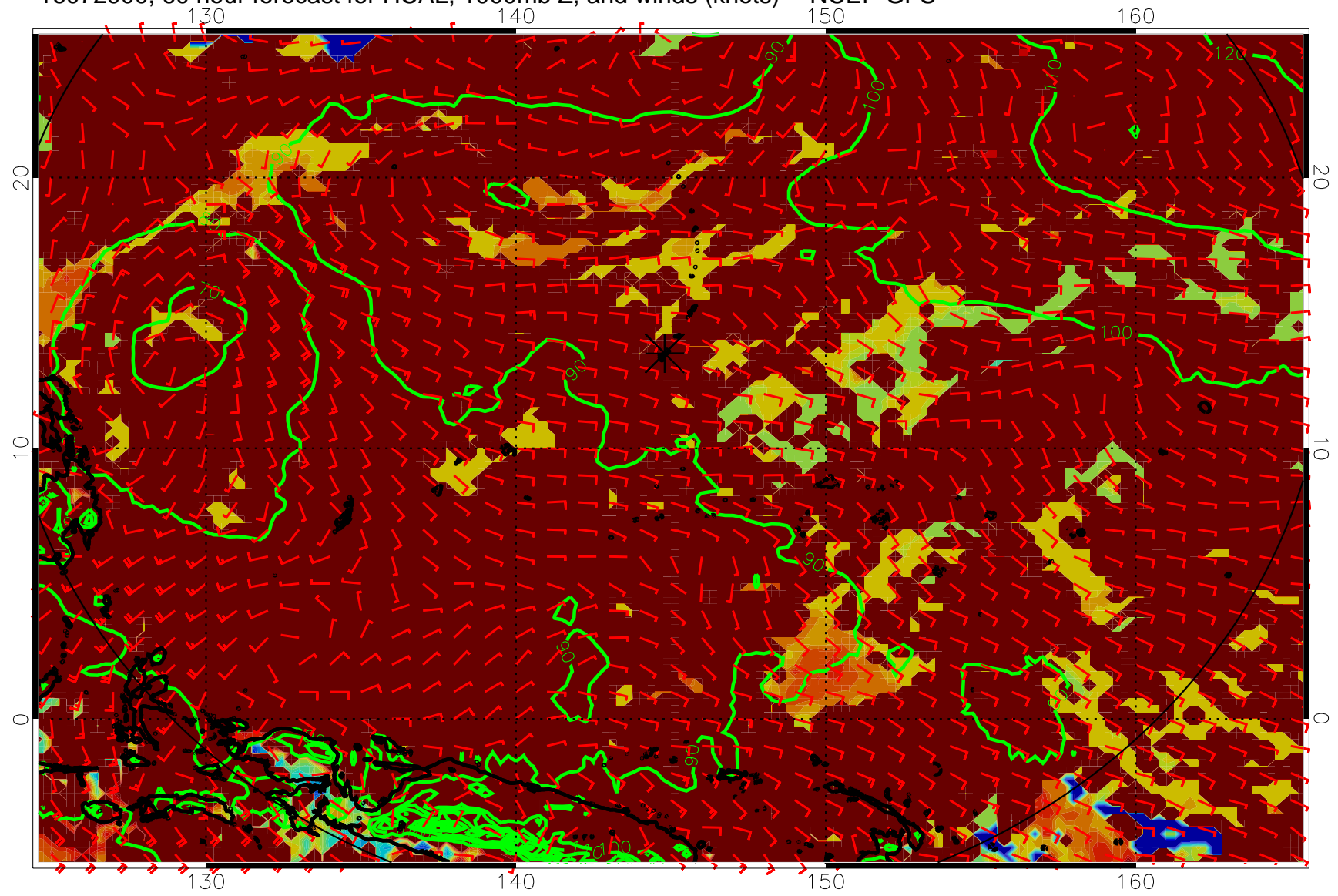
16072900, 60 hour forecast for HCAL, 1000mb Z, and winds (knots) -- NCEP GFS
