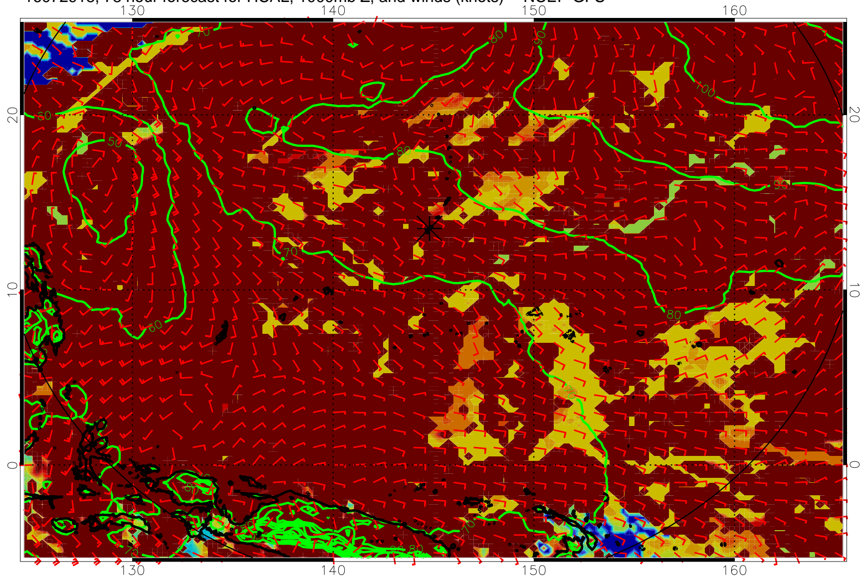
16072918, 78 hour forecast for HCAL, 1000mb Z, and winds (knots) -- NCEP GFS
