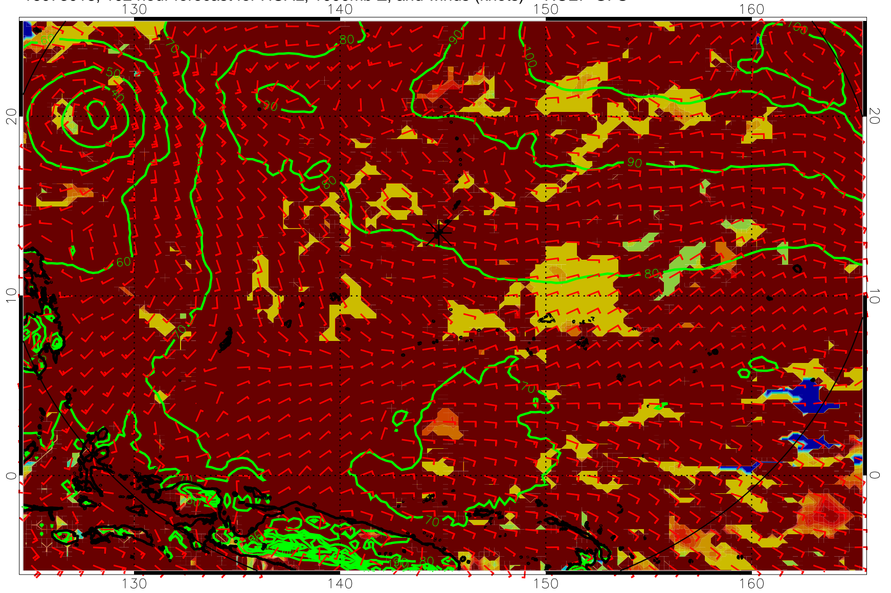
16073018, 102 hour forecast for HCAL, 1000mb Z, and winds (knots) -- NCEP GFS
