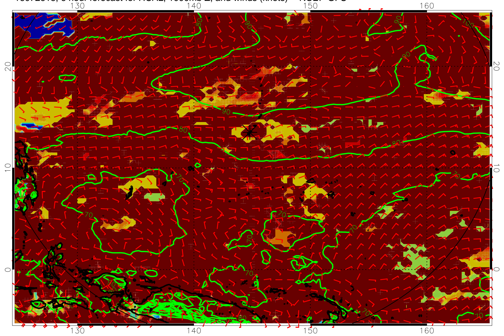
16072618, 6 hour forecast for HCAL, 1000mb Z, and winds (knots) -- NCEP GFS
