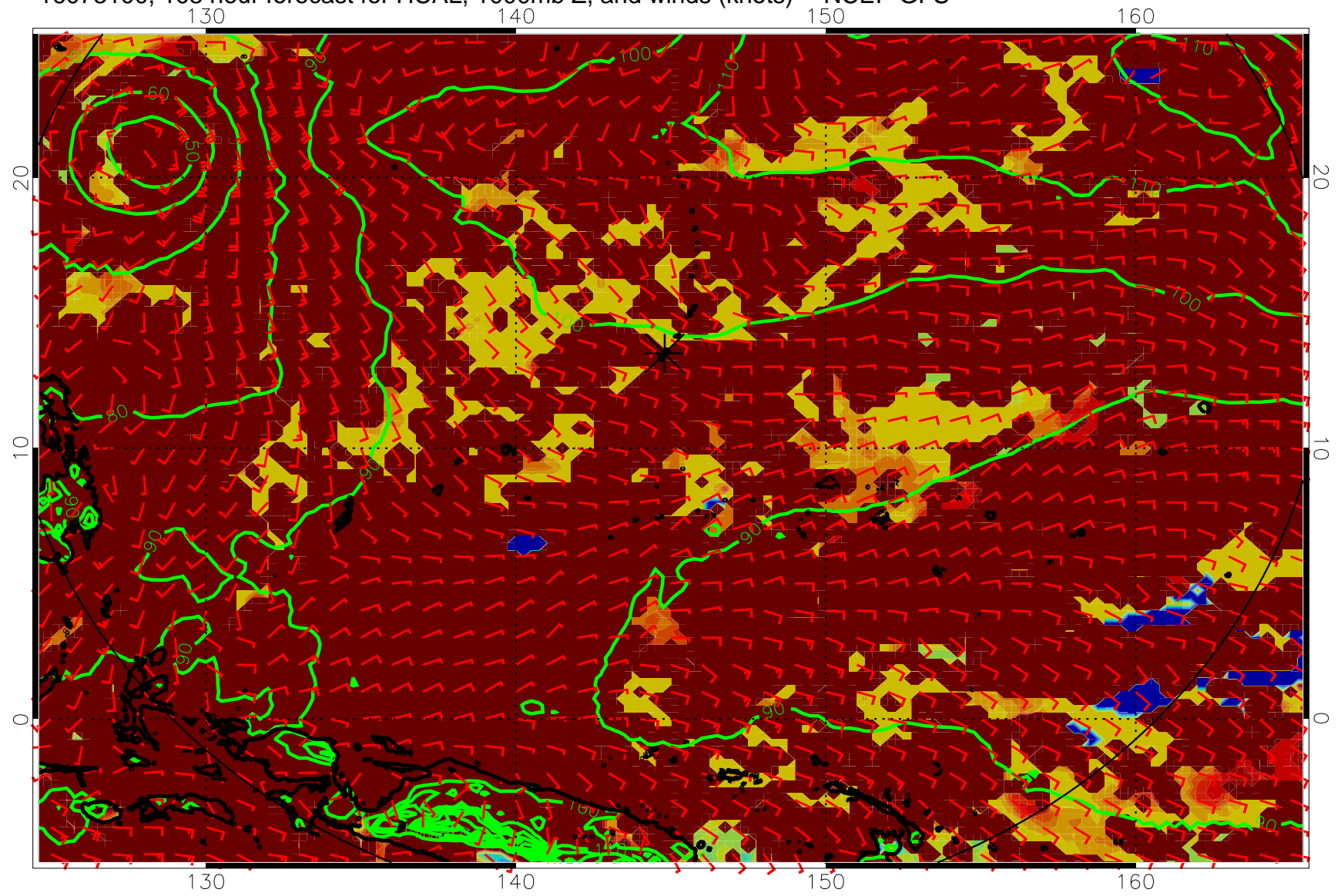
16073100, 108 hour forecast for HCAL, 1000mb Z, and winds (knots) -- NCEP GFS
