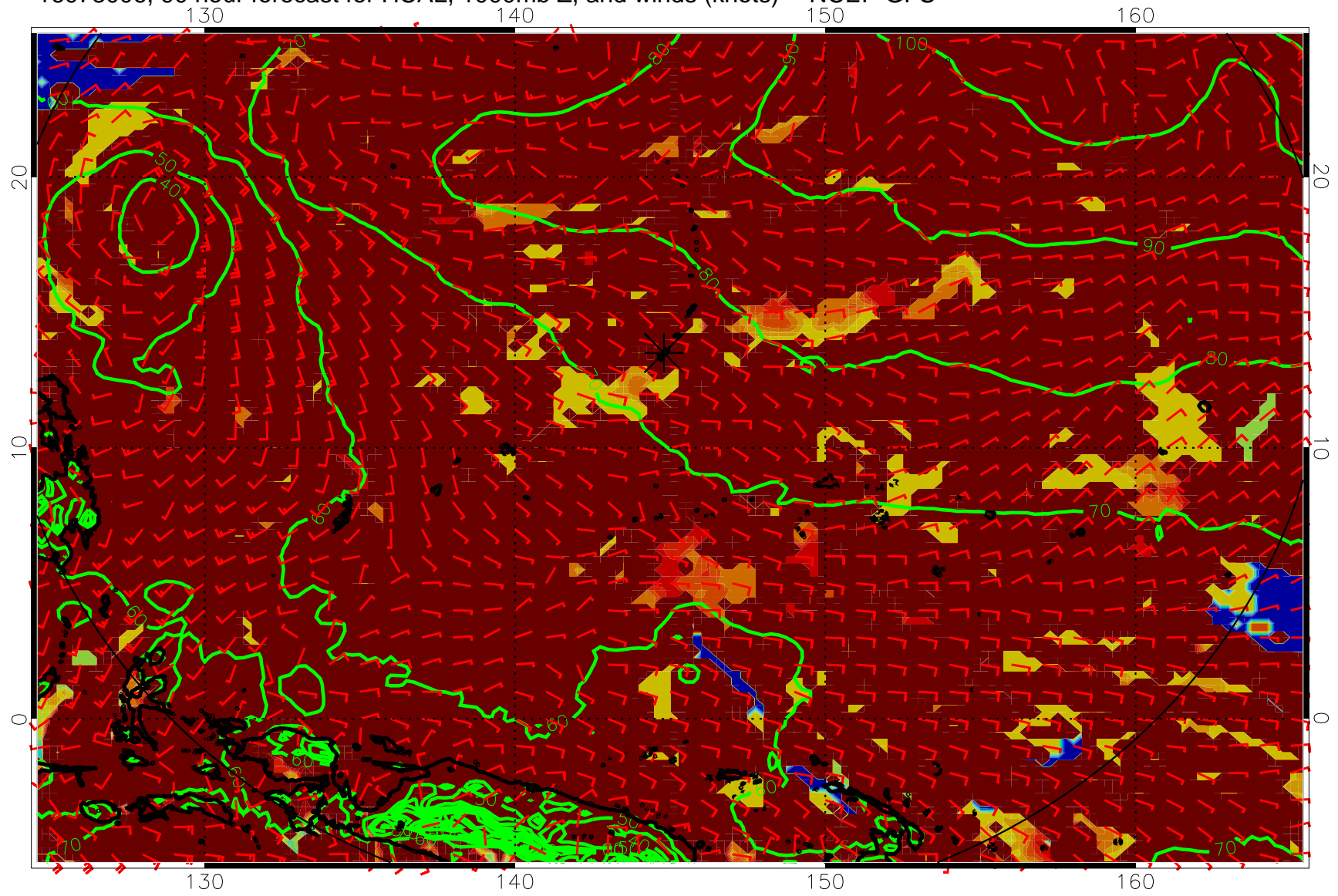
16073006, 90 hour forecast for HCAL, 1000mb Z, and winds (knots) -- NCEP GFS
