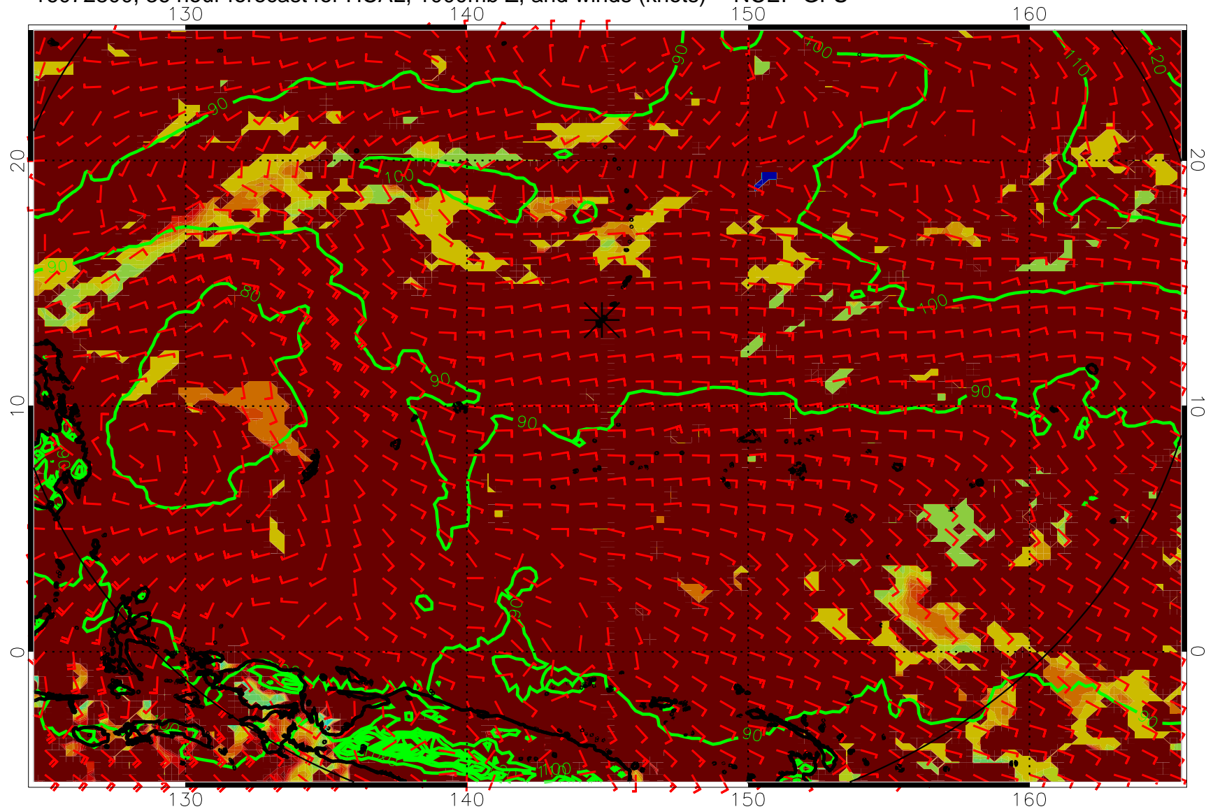
16072800, 36 hour forecast for HCAL, 1000mb Z, and winds (knots) -- NCEP GFS
