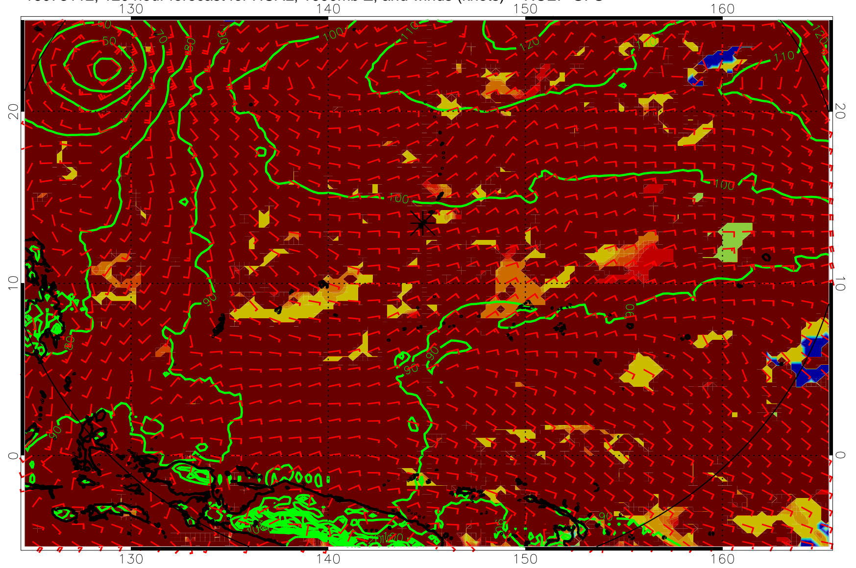
16073112, 120 hour forecast for HCAL, 1000mb Z, and winds (knots) -- NCEP GFS
