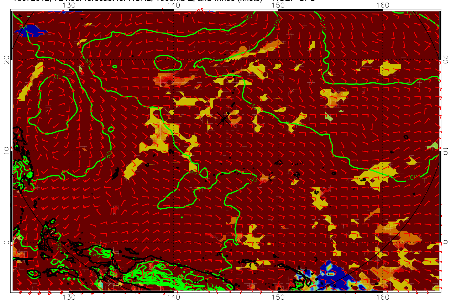
16072912, 72 hour forecast for HCAL, 1000mb Z, and winds (knots) -- NCEP GFS
