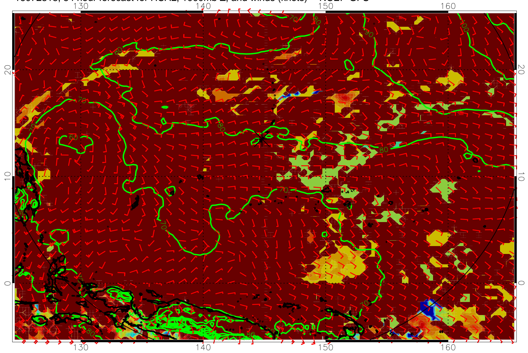
16072818, 54 hour forecast for HCAL, 1000mb Z, and winds (knots) -- NCEP GFS
