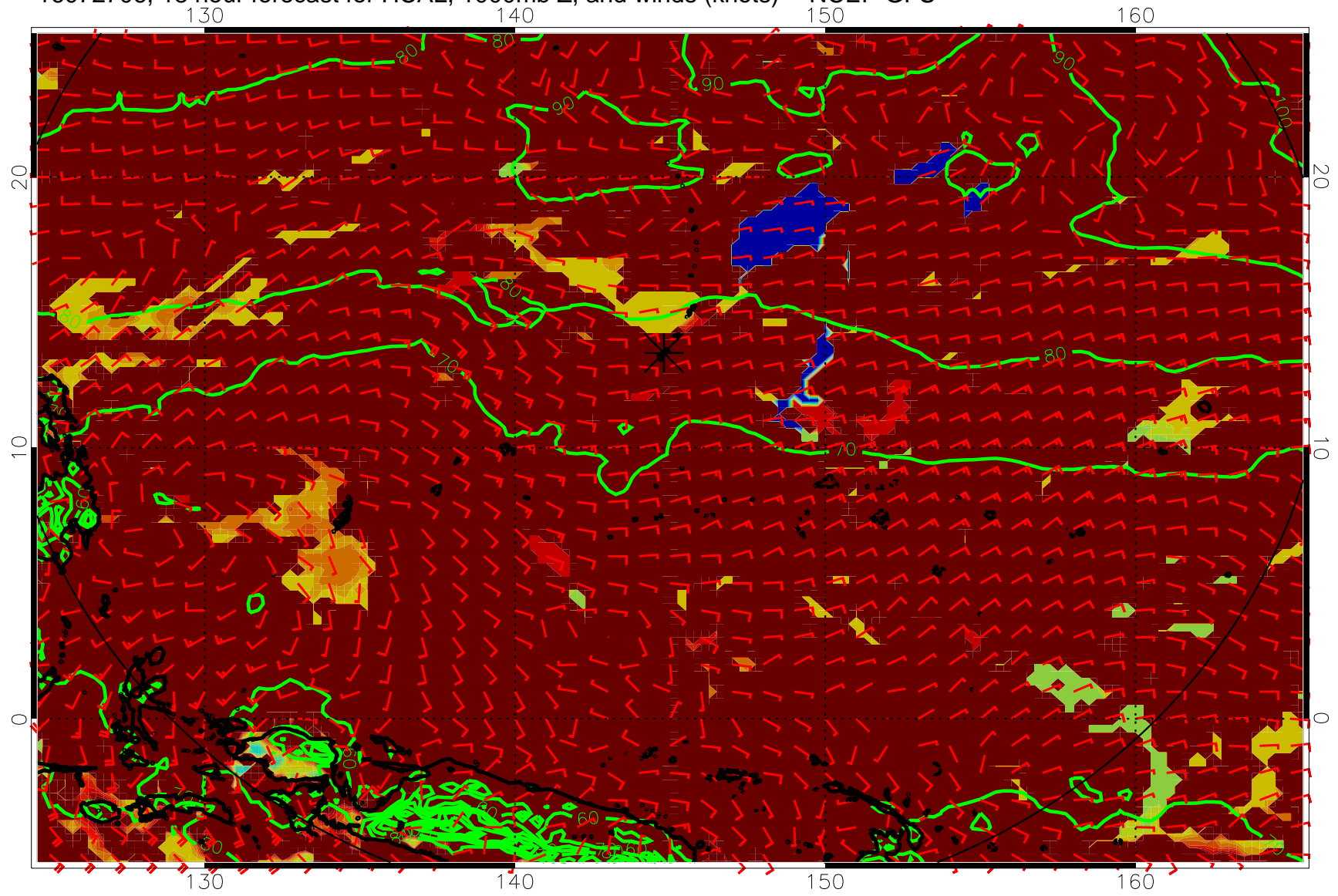
16072706, 18 hour forecast for HCAL, 1000mb Z, and winds (knots) -- NCEP GFS
