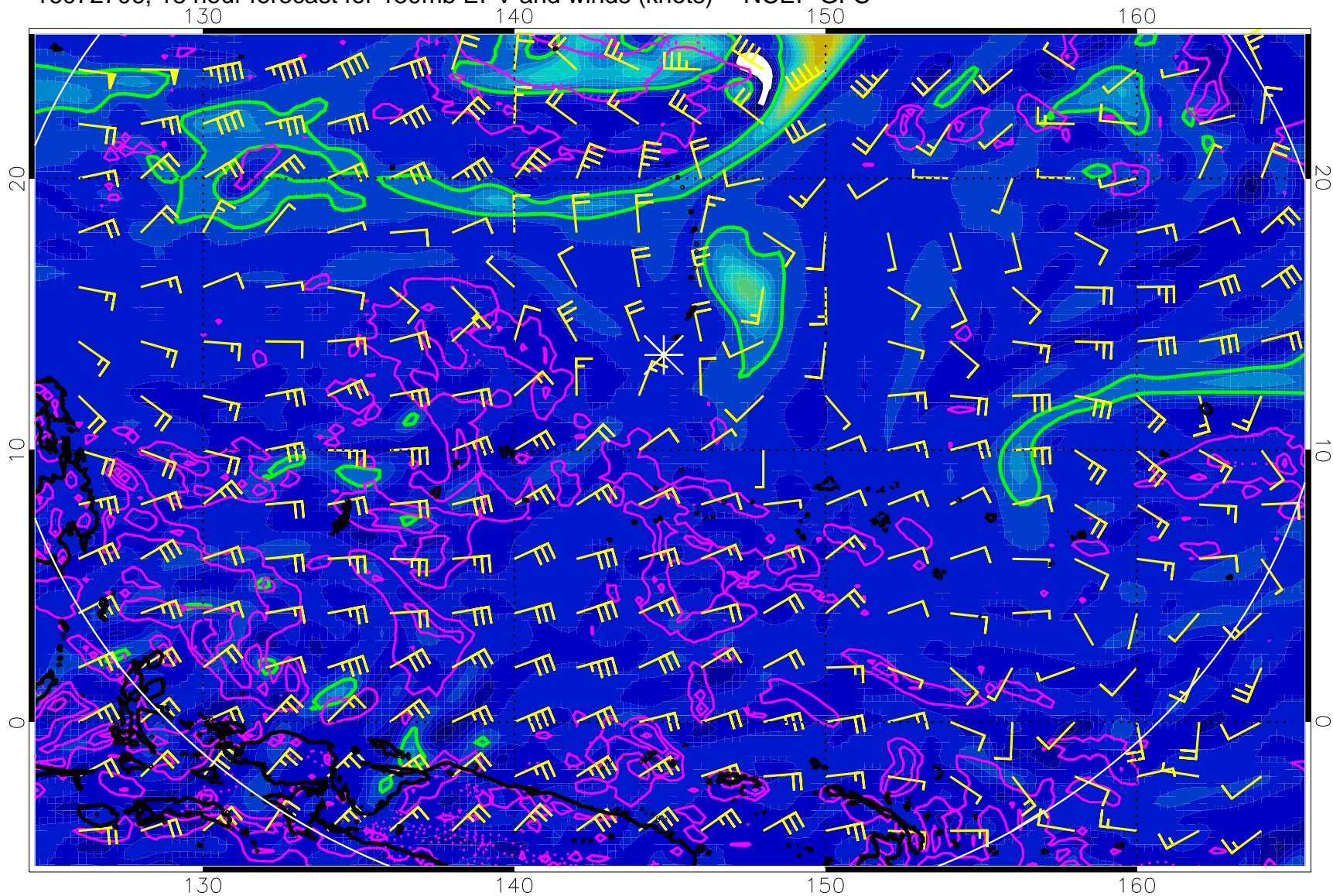
16072706, 18 hour forecast for 150mb EPV and winds (knots) -- NCEP GFS
