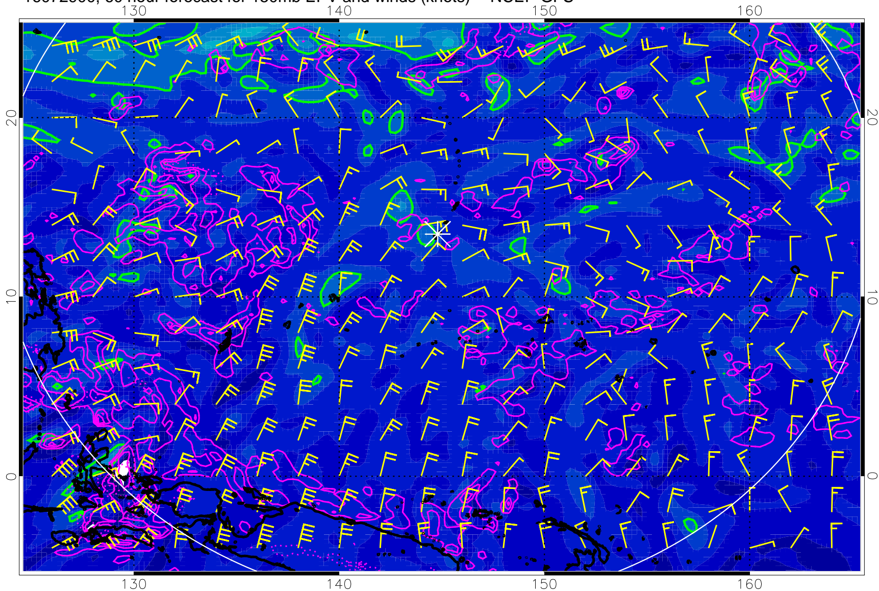
16072900, 60 hour forecast for 150mb EPV and winds (knots) -- NCEP GFS
