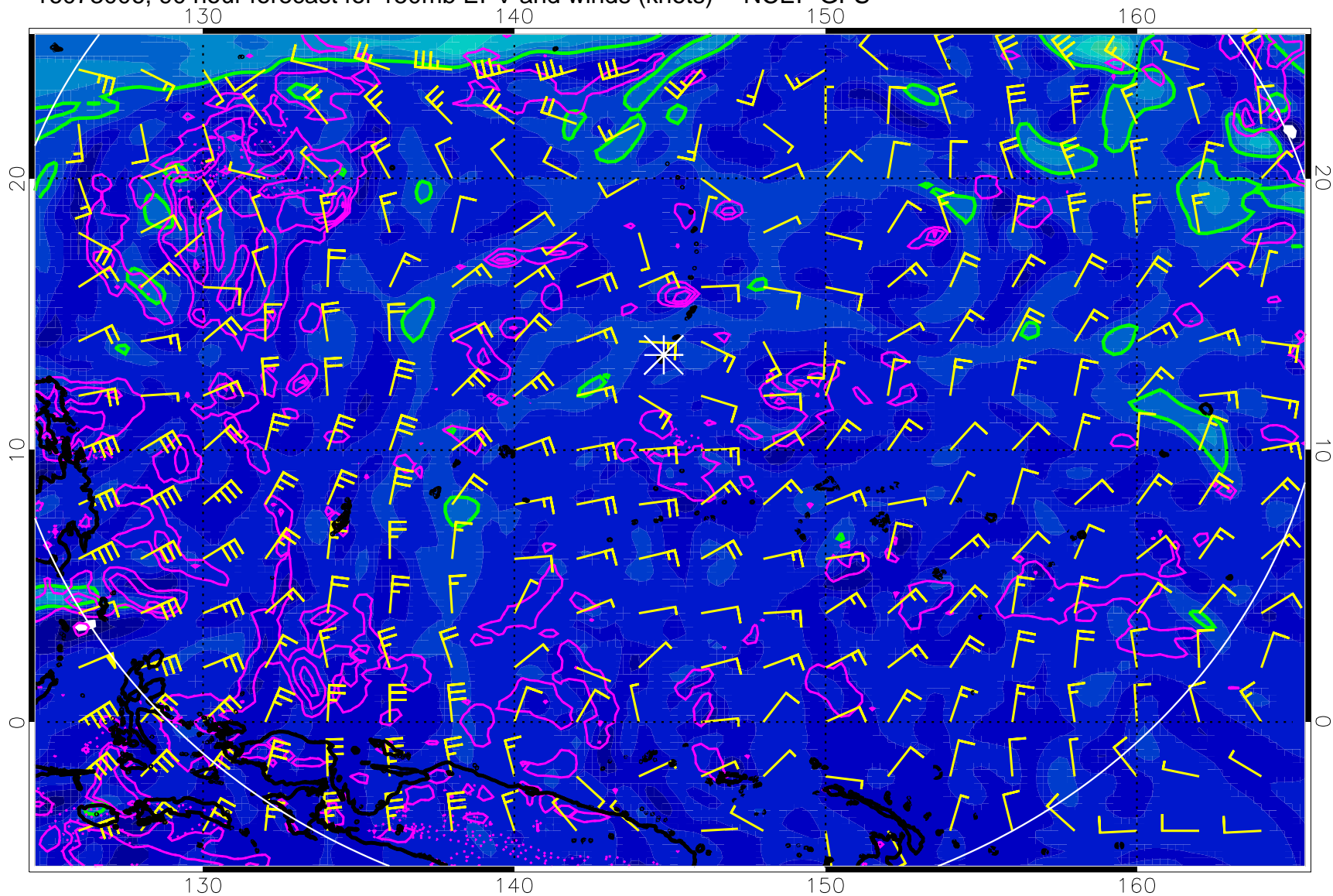
16073006, 90 hour forecast for 150mb EPV and winds (knots) -- NCEP GFS
