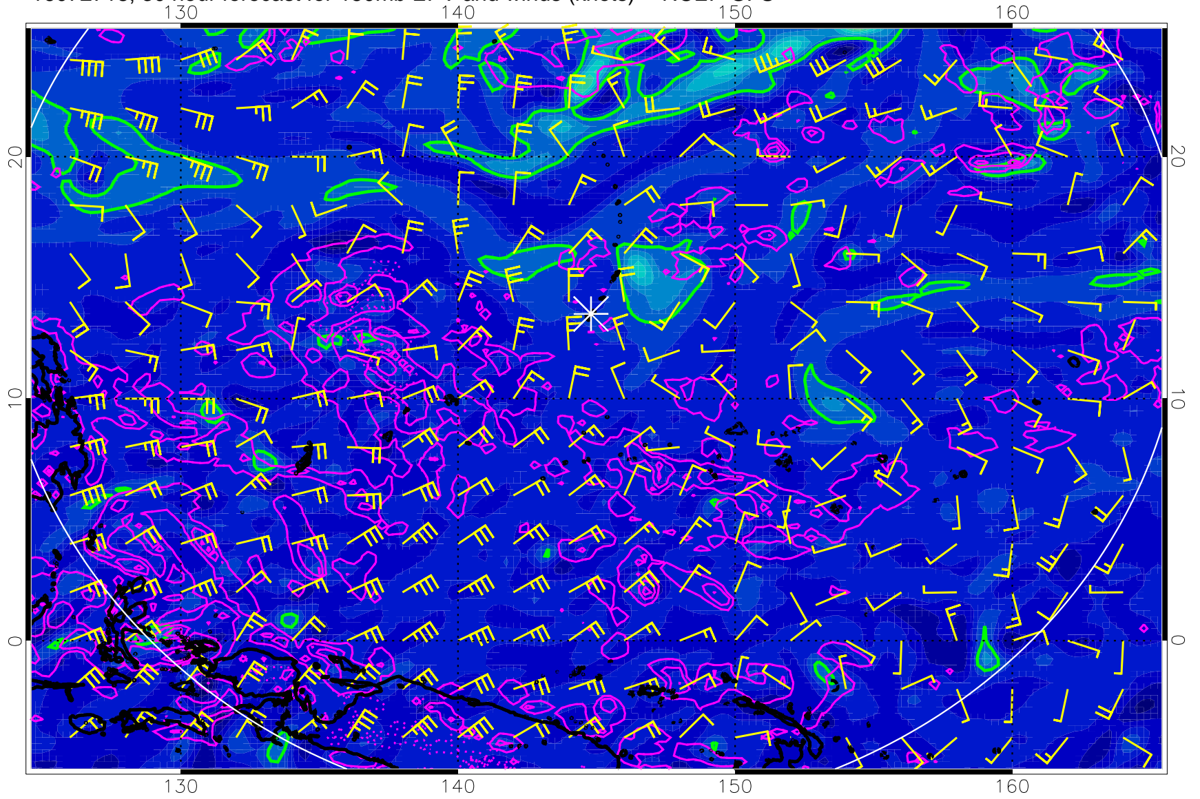
16072718, 30 hour forecast for 150mb EPV and winds (knots) -- NCEP GFS
