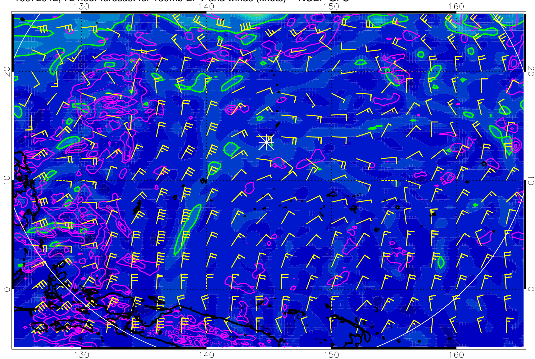
16072912, 72 hour forecast for 150mb EPV and winds (knots) -- NCEP GFS
