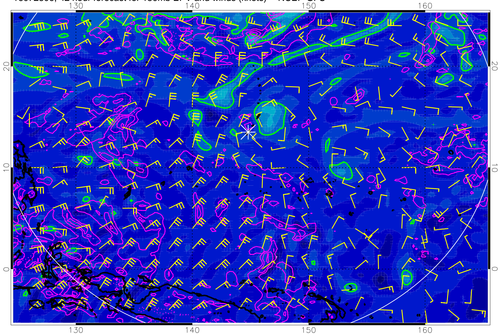
16072806, 42 hour forecast for 150mb EPV and winds (knots) -- NCEP GFS
