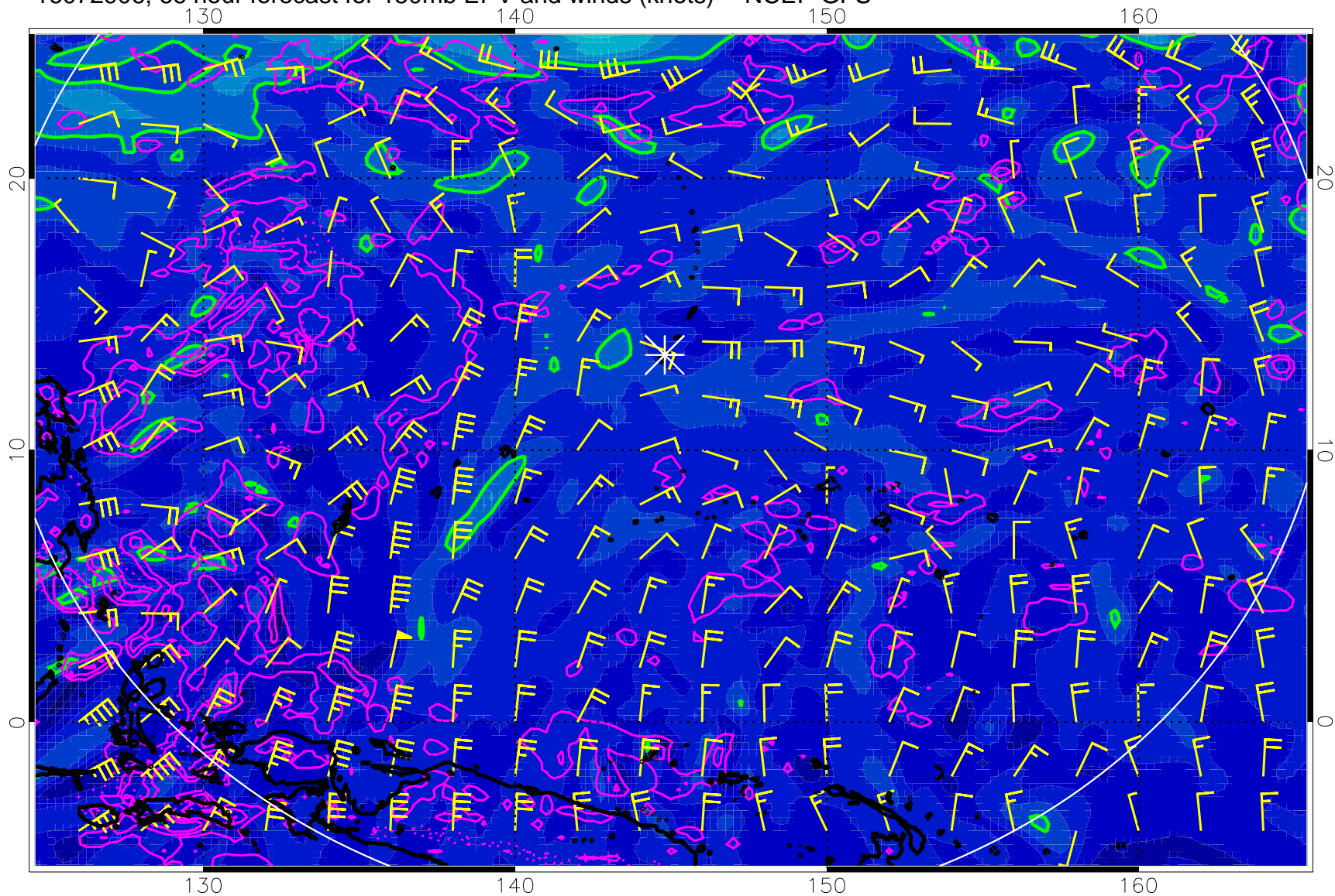
16072906, 66 hour forecast for 150mb EPV and winds (knots) -- NCEP GFS
