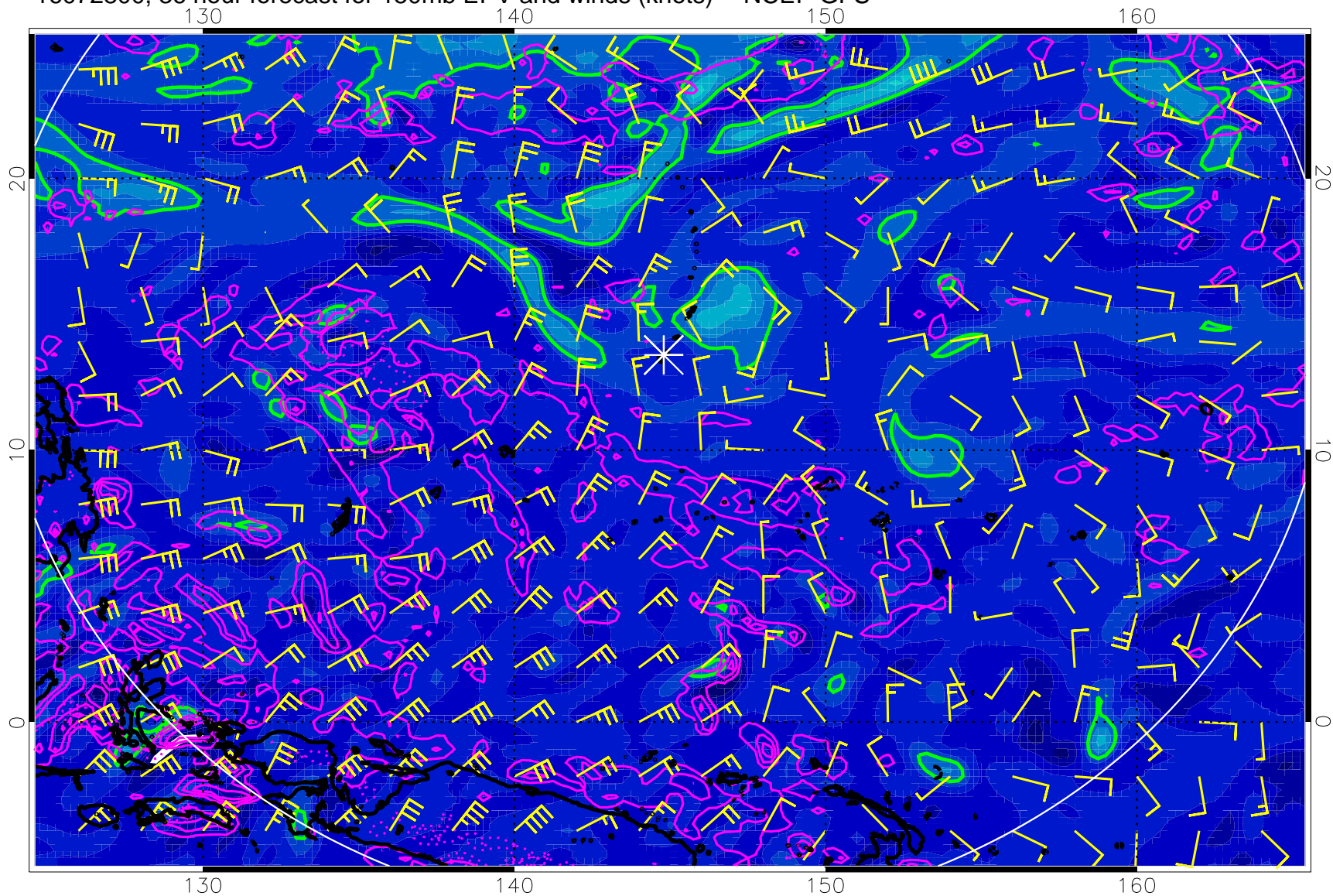
16072800, 36 hour forecast for 150mb EPV and winds (knots) -- NCEP GFS
