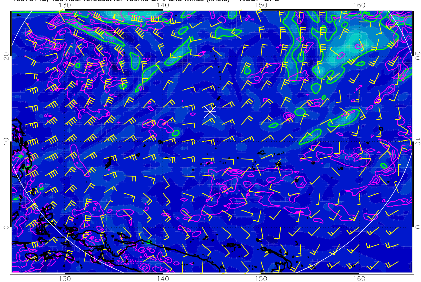
16073112, 120 hour forecast for 150mb EPV and winds (knots) -- NCEP GFS
