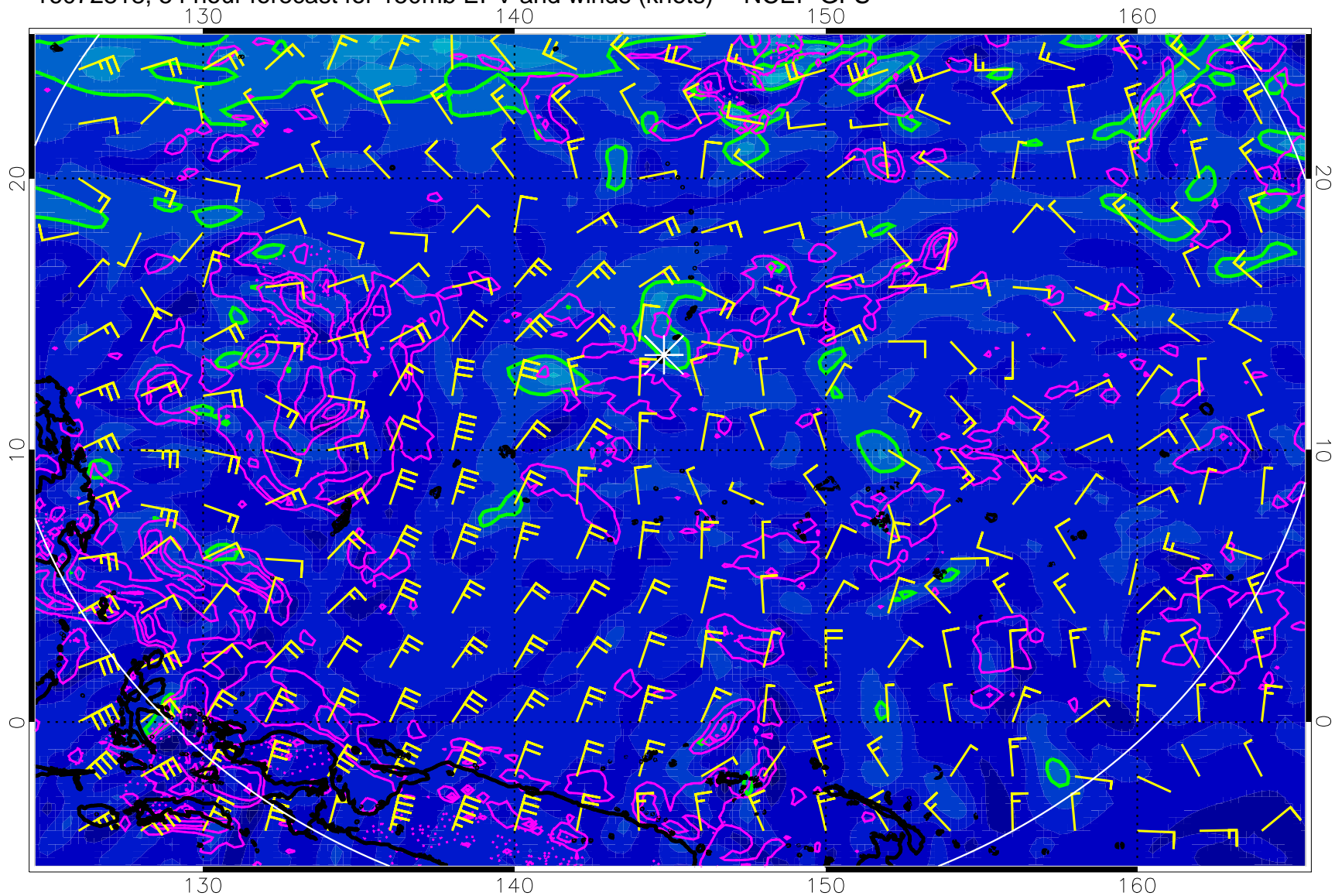
16072818, 54 hour forecast for 150mb EPV and winds (knots) -- NCEP GFS
