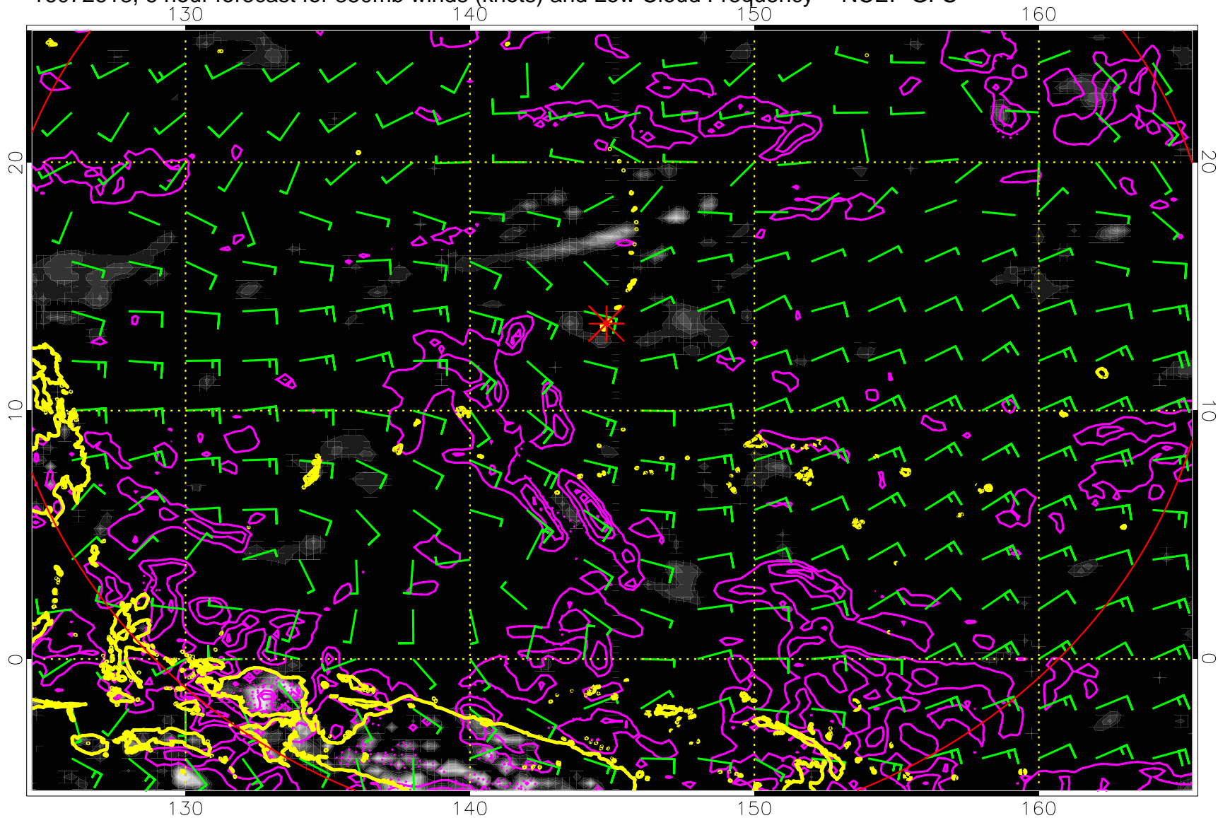
16072618, 6 hour forecast for 850mb winds (knots) and Low Cloud Frequency -- NCEP GFS
