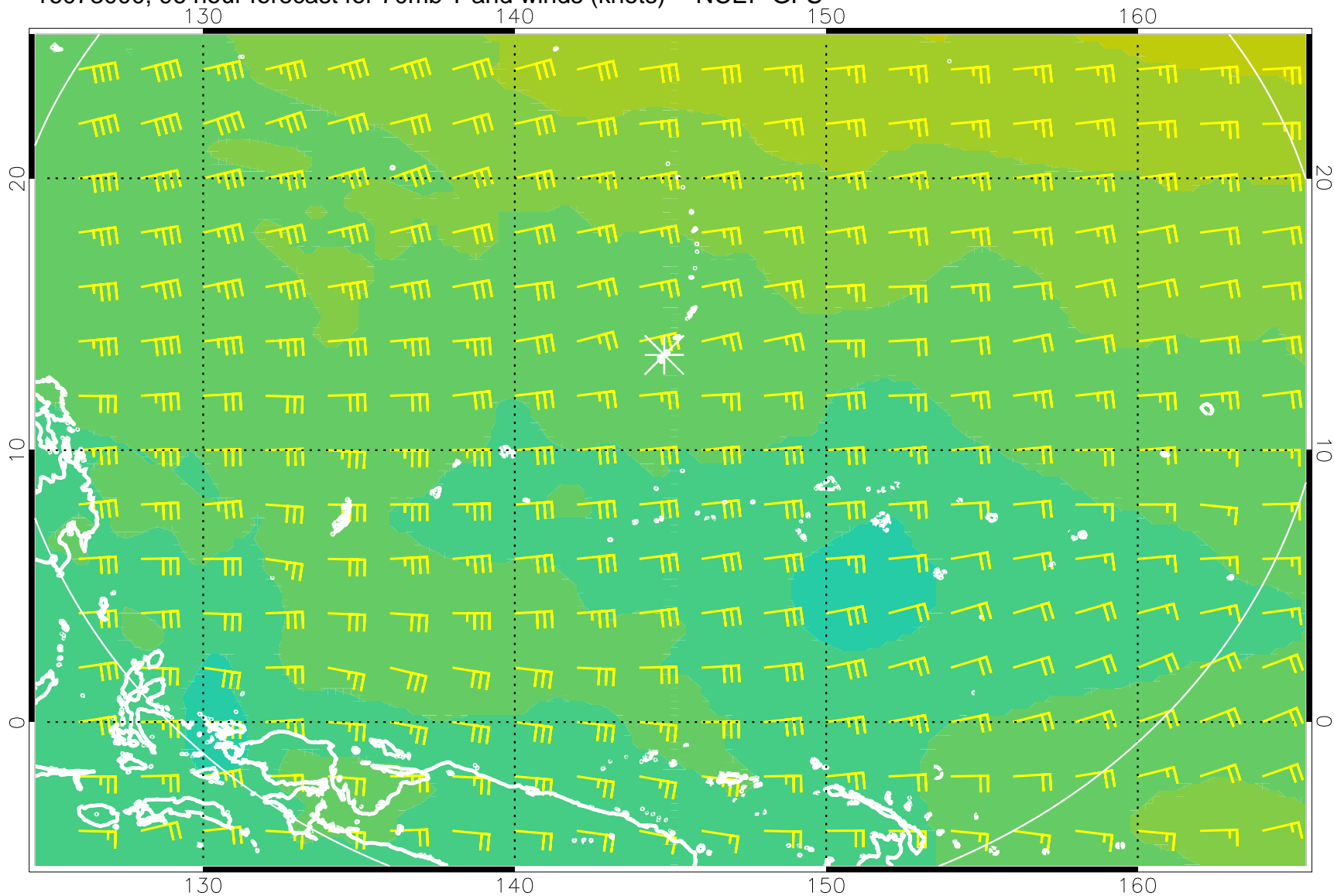
16073000, 96 hour forecast for 70mb T and winds (knots) -- NCEP GFS
