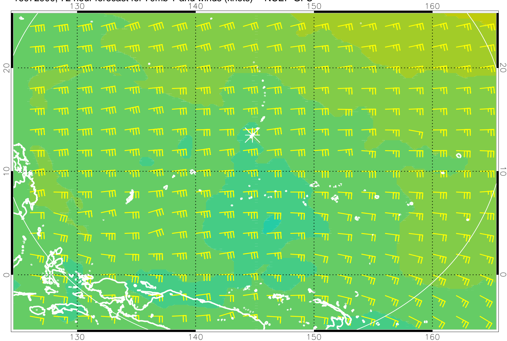
16072900, 72 hour forecast for 70mb T and winds (knots) -- NCEP GFS
