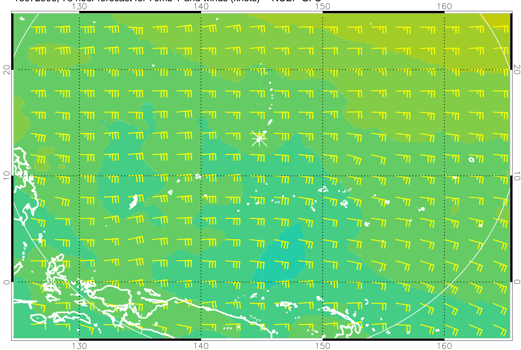
16072906, 78 hour forecast for 70mb T and winds (knots) -- NCEP GFS
