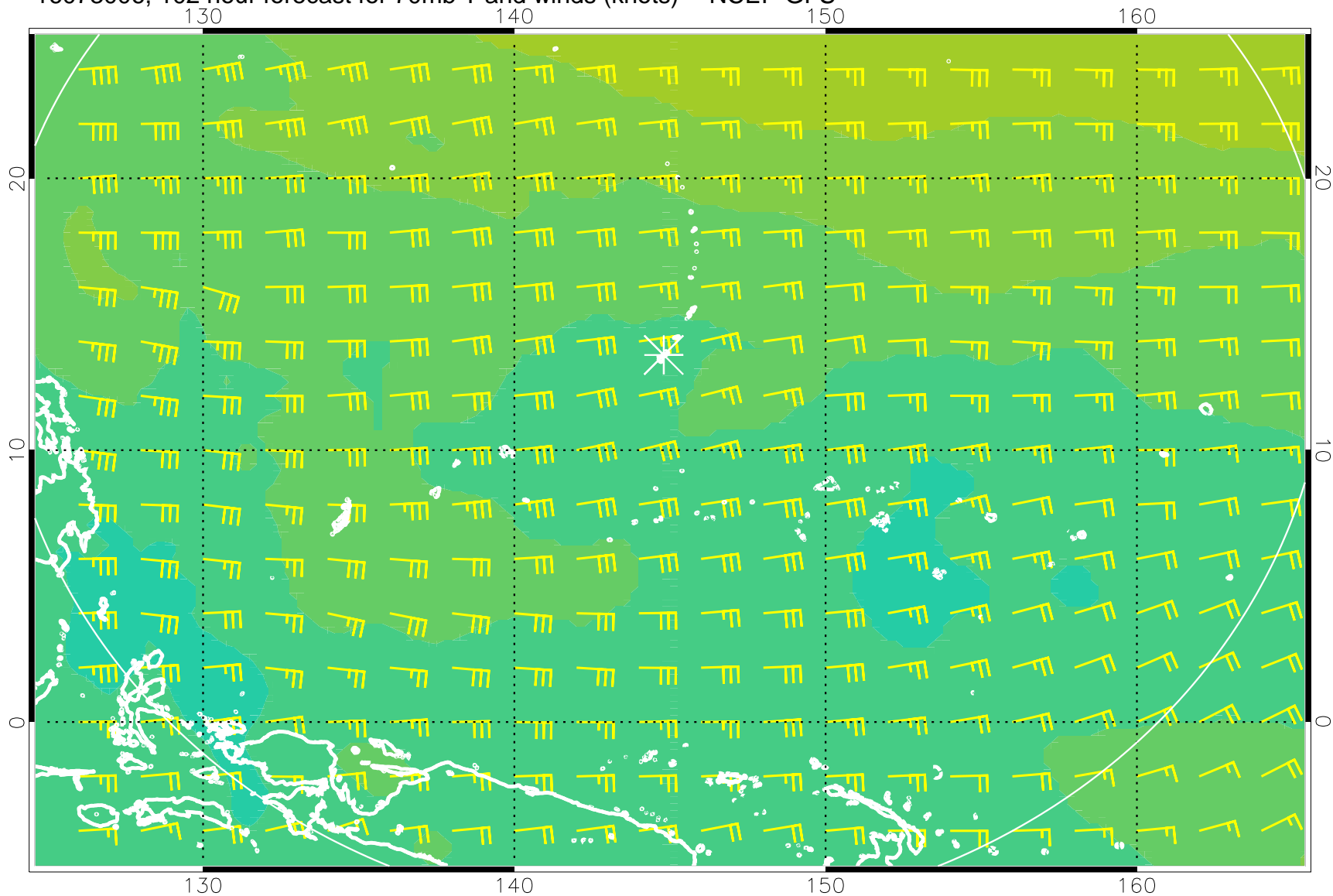
16073006, 102 hour forecast for 70mb T and winds (knots) -- NCEP GFS
