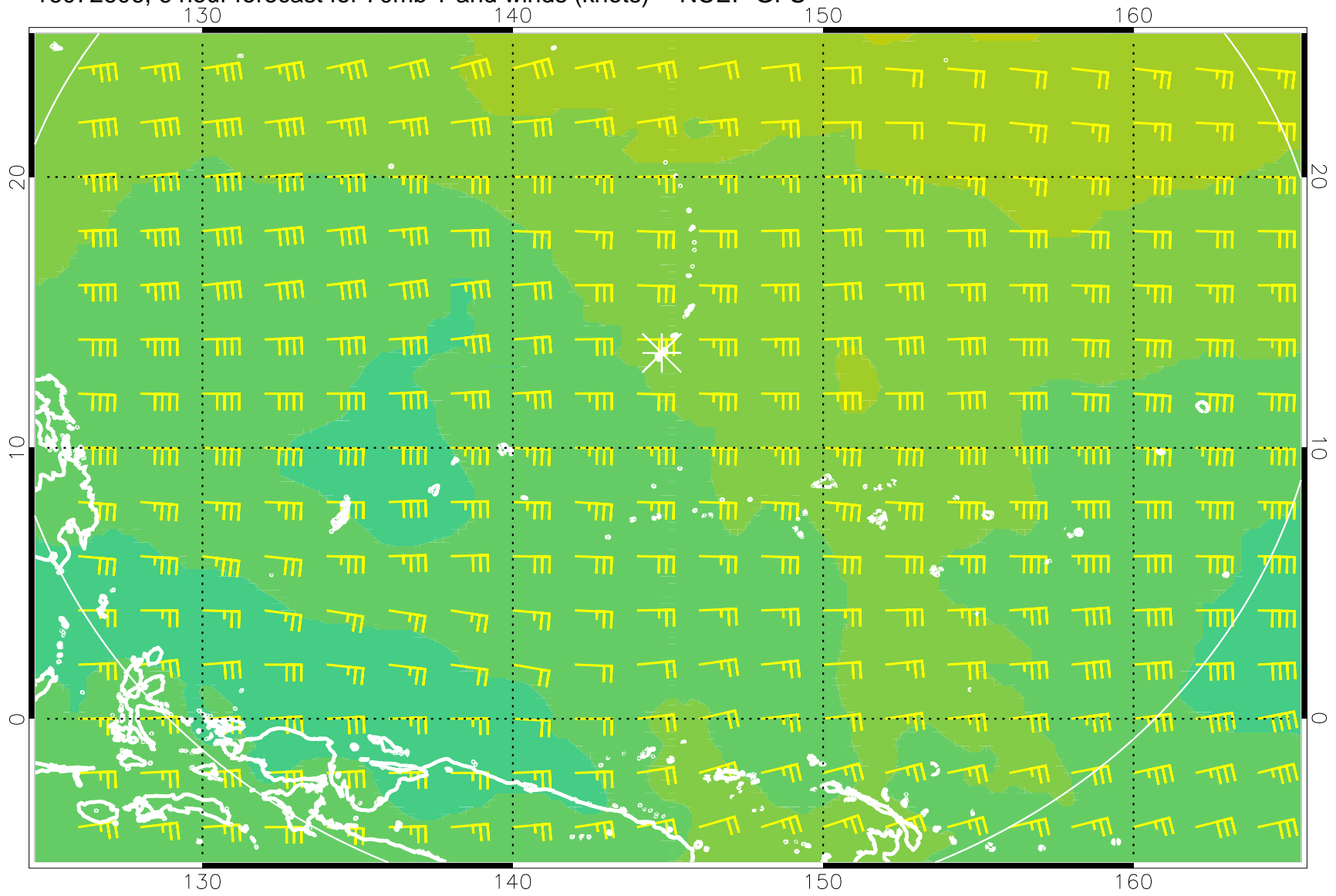
16072606, 6 hour forecast for 70mb T and winds (knots) -- NCEP GFS
