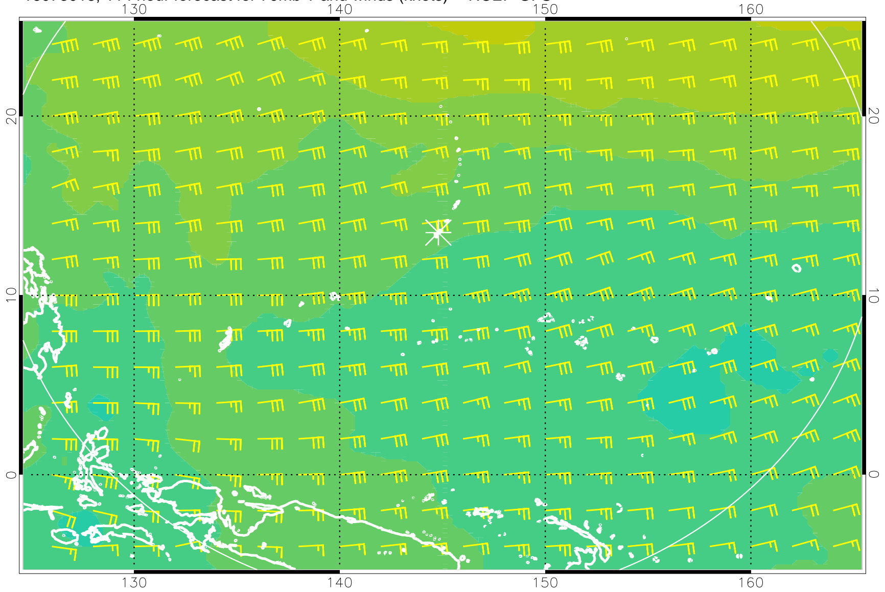
16073018, 114 hour forecast for 70mb T and winds (knots) -- NCEP GFS
