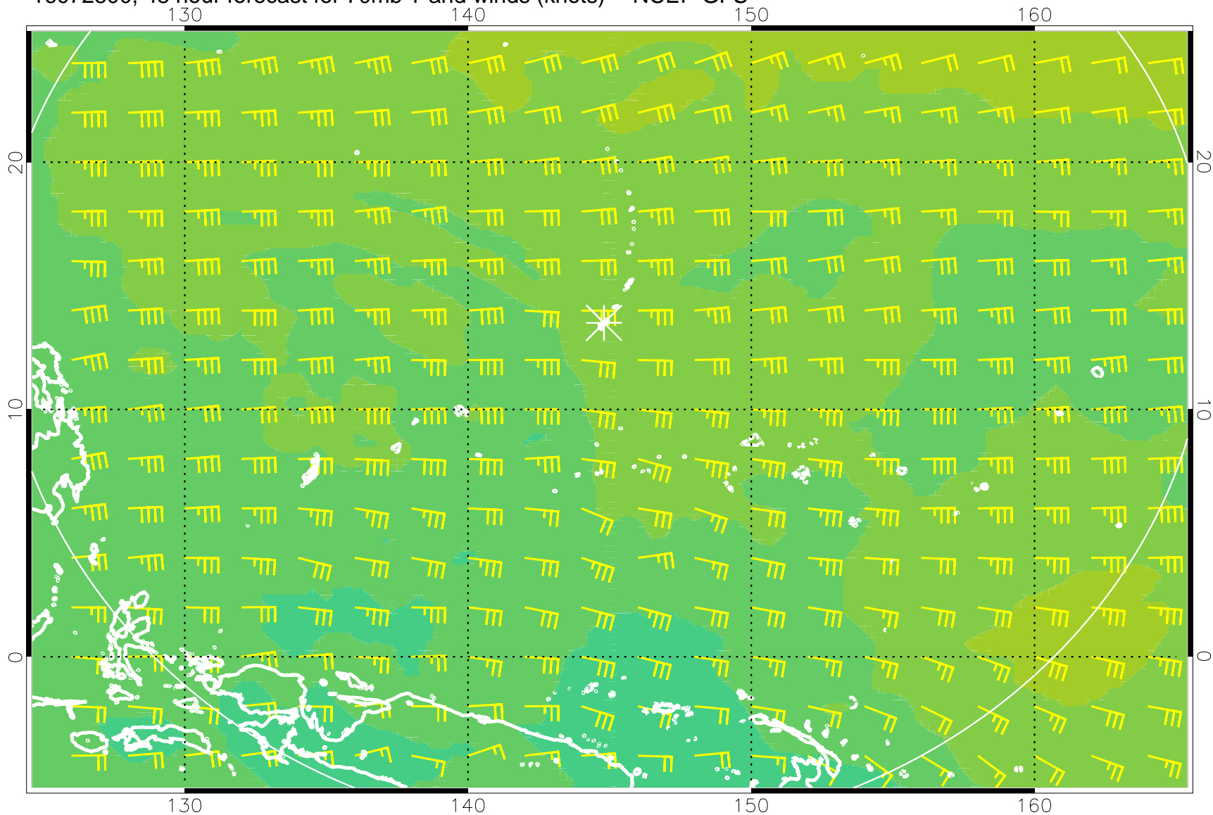
16072800, 48 hour forecast for 70mb T and winds (knots) -- NCEP GFS
