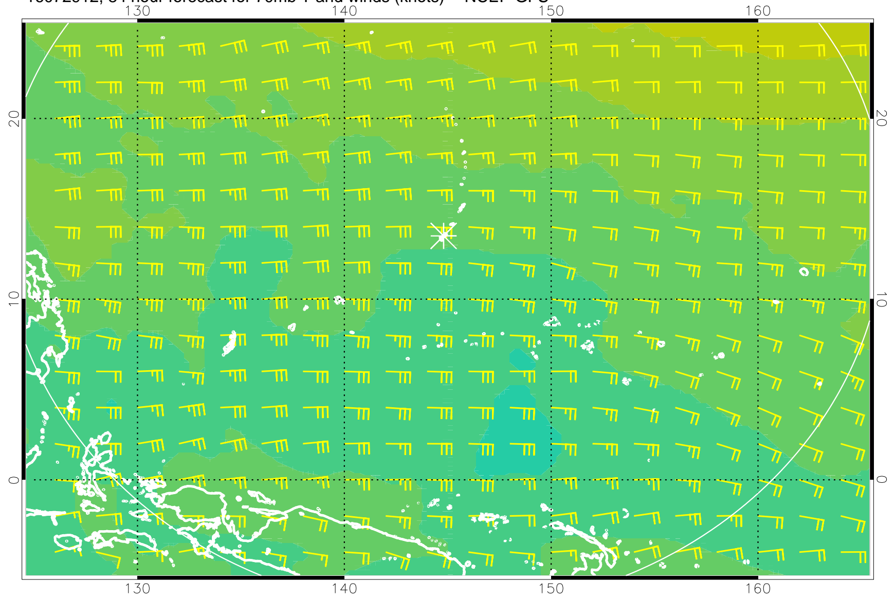
16072912, 84 hour forecast for 70mb T and winds (knots) -- NCEP GFS
