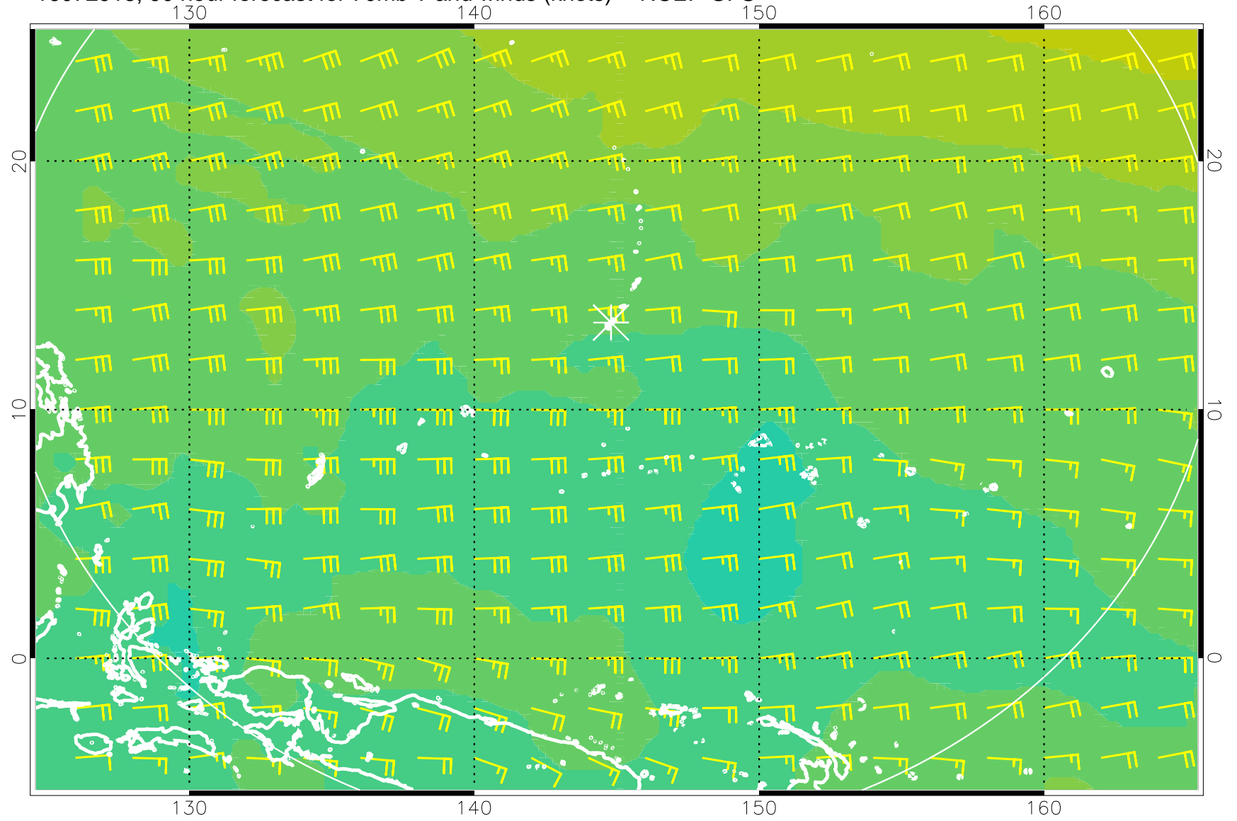
16072918, 90 hour forecast for 70mb T and winds (knots) -- NCEP GFS
