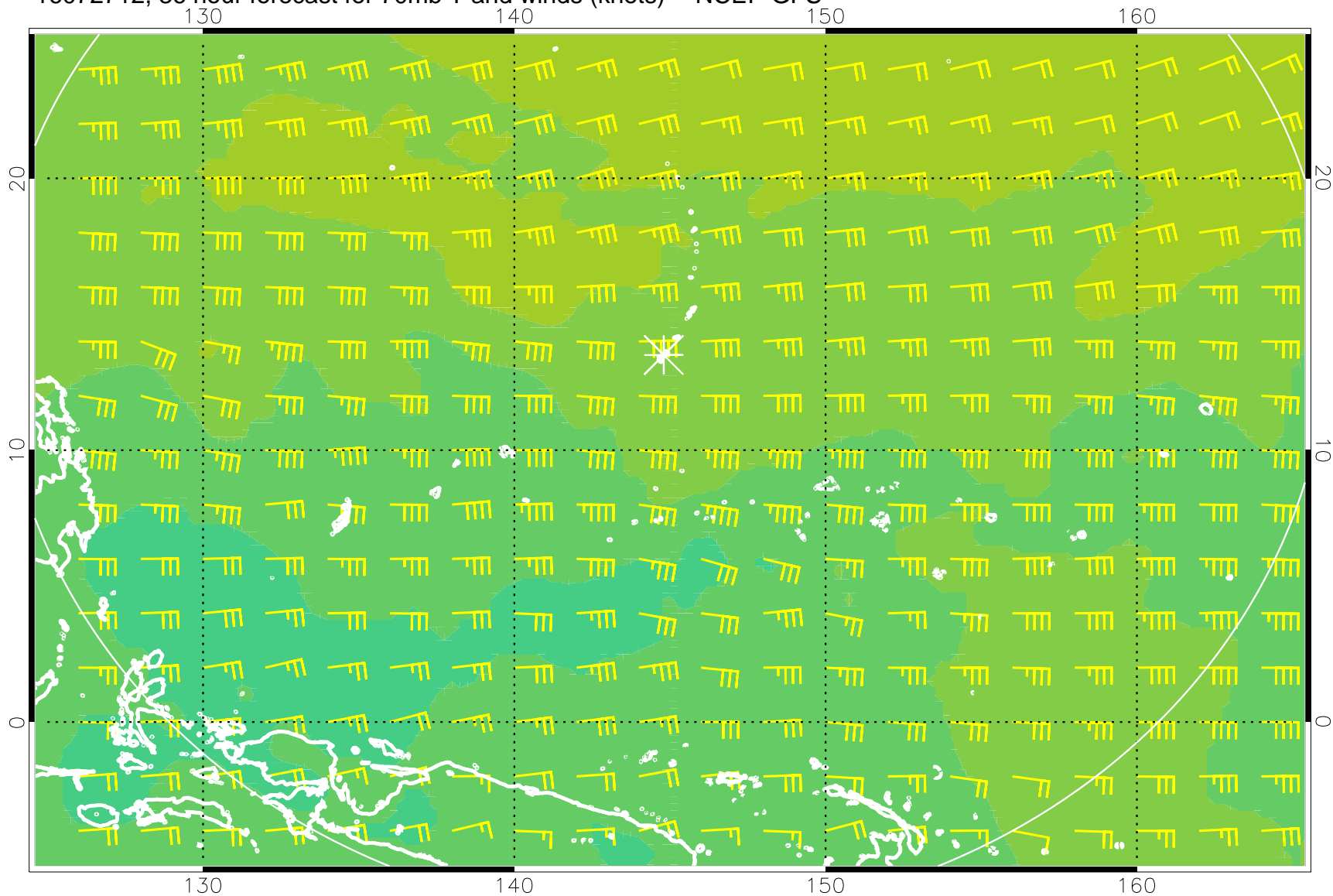
16072712, 36 hour forecast for 70mb T and winds (knots) -- NCEP GFS
