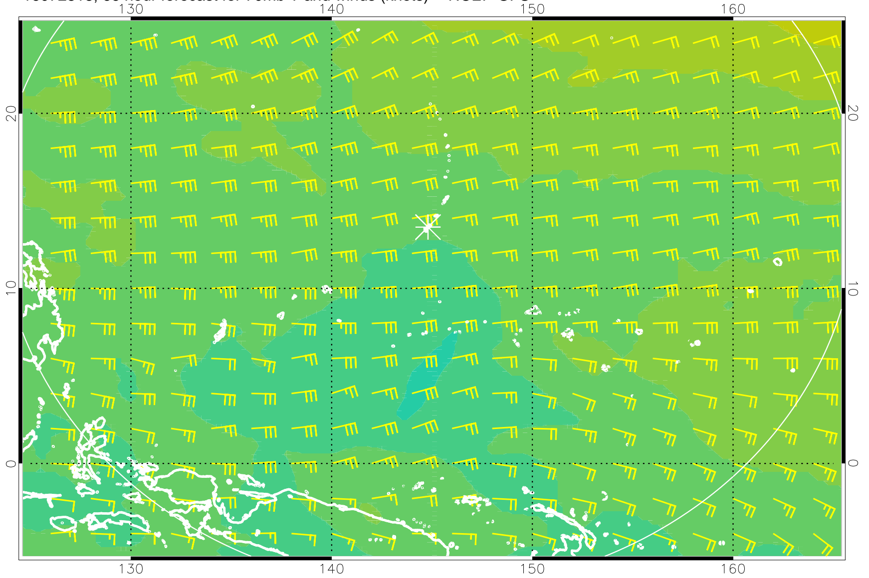
16072818, 66 hour forecast for 70mb T and winds (knots) -- NCEP GFS
