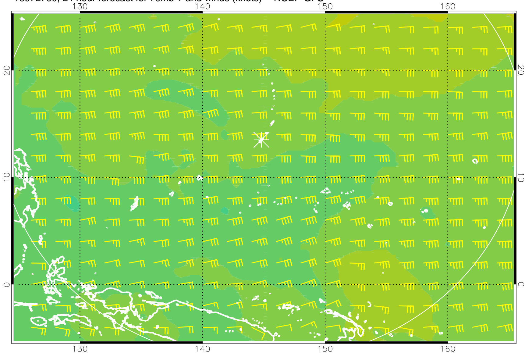
16072700, 24 hour forecast for 70mb T and winds (knots) -- NCEP GFS
