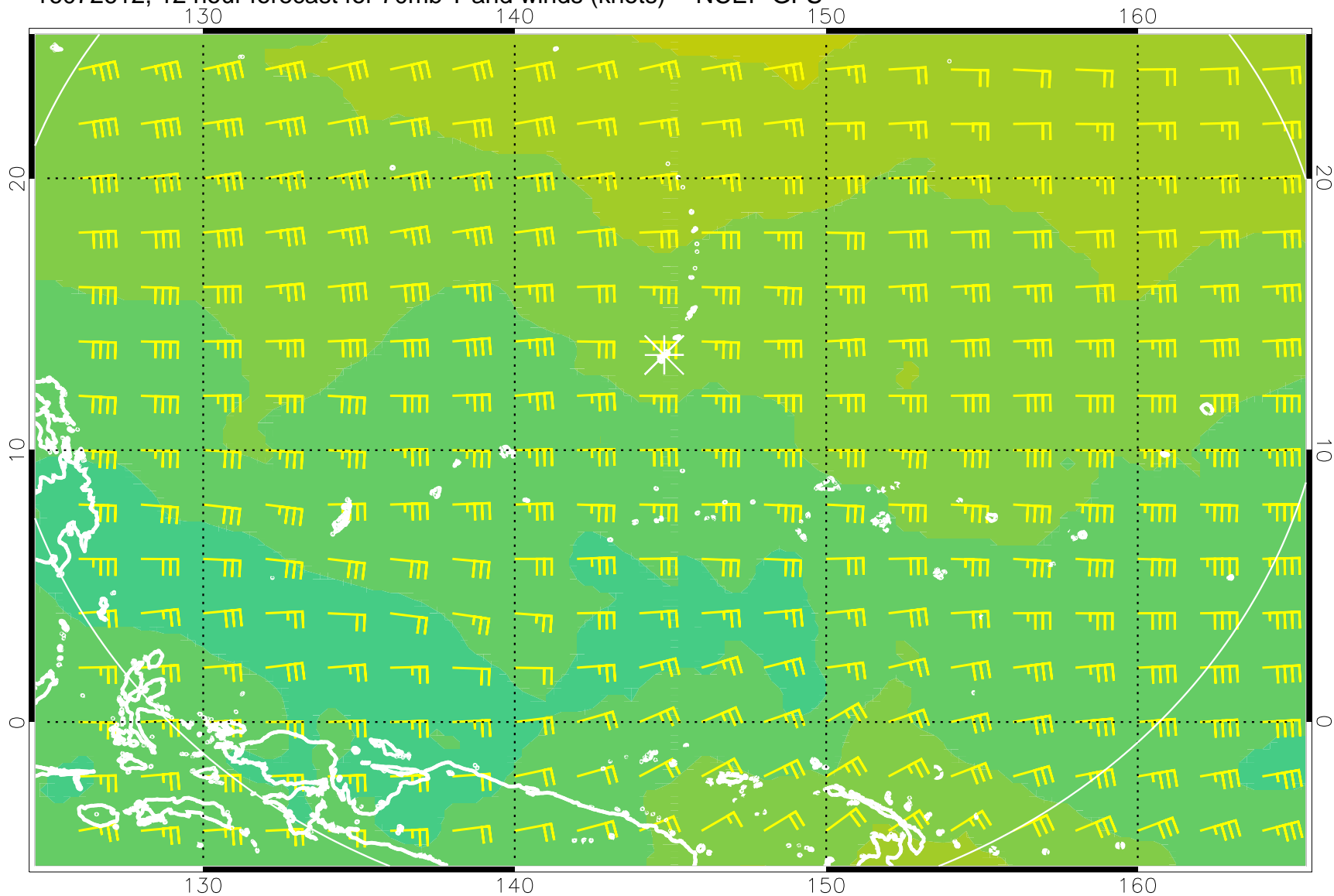
16072612, 12 hour forecast for 70mb T and winds (knots) -- NCEP GFS
