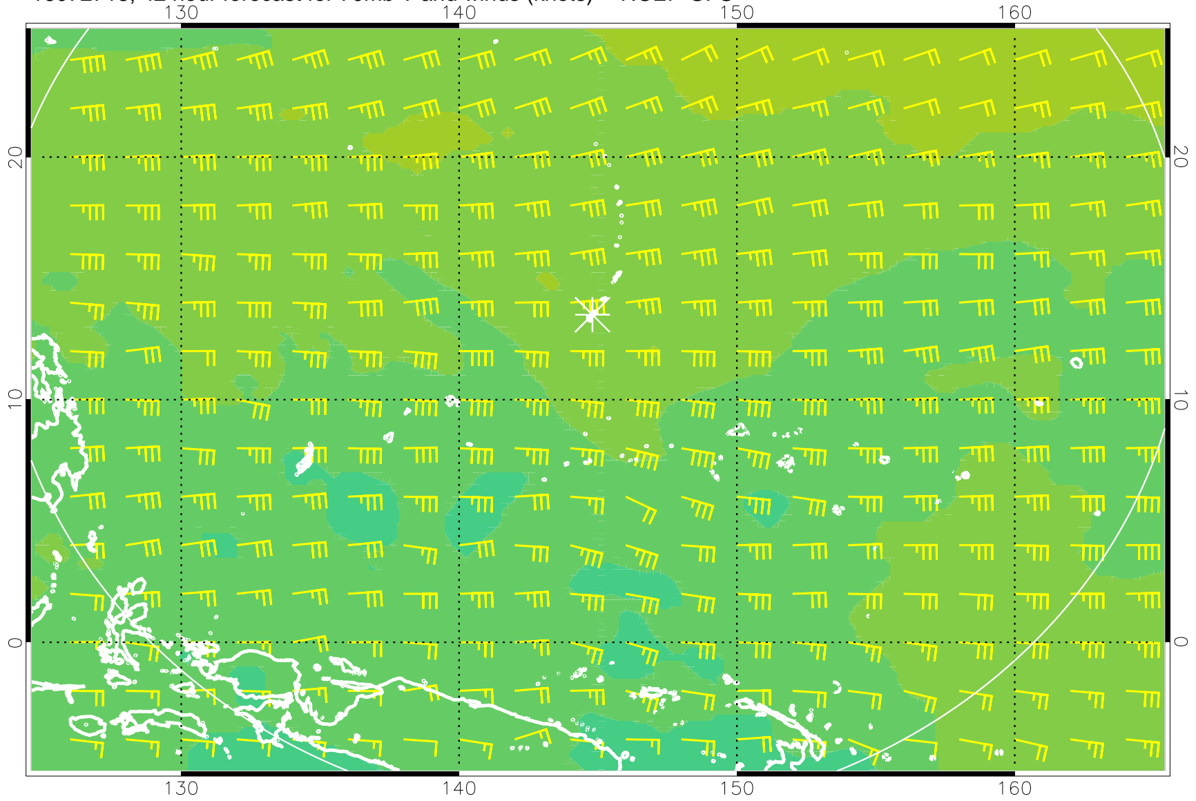
16072718, 42 hour forecast for 70mb T and winds (knots) -- NCEP GFS
