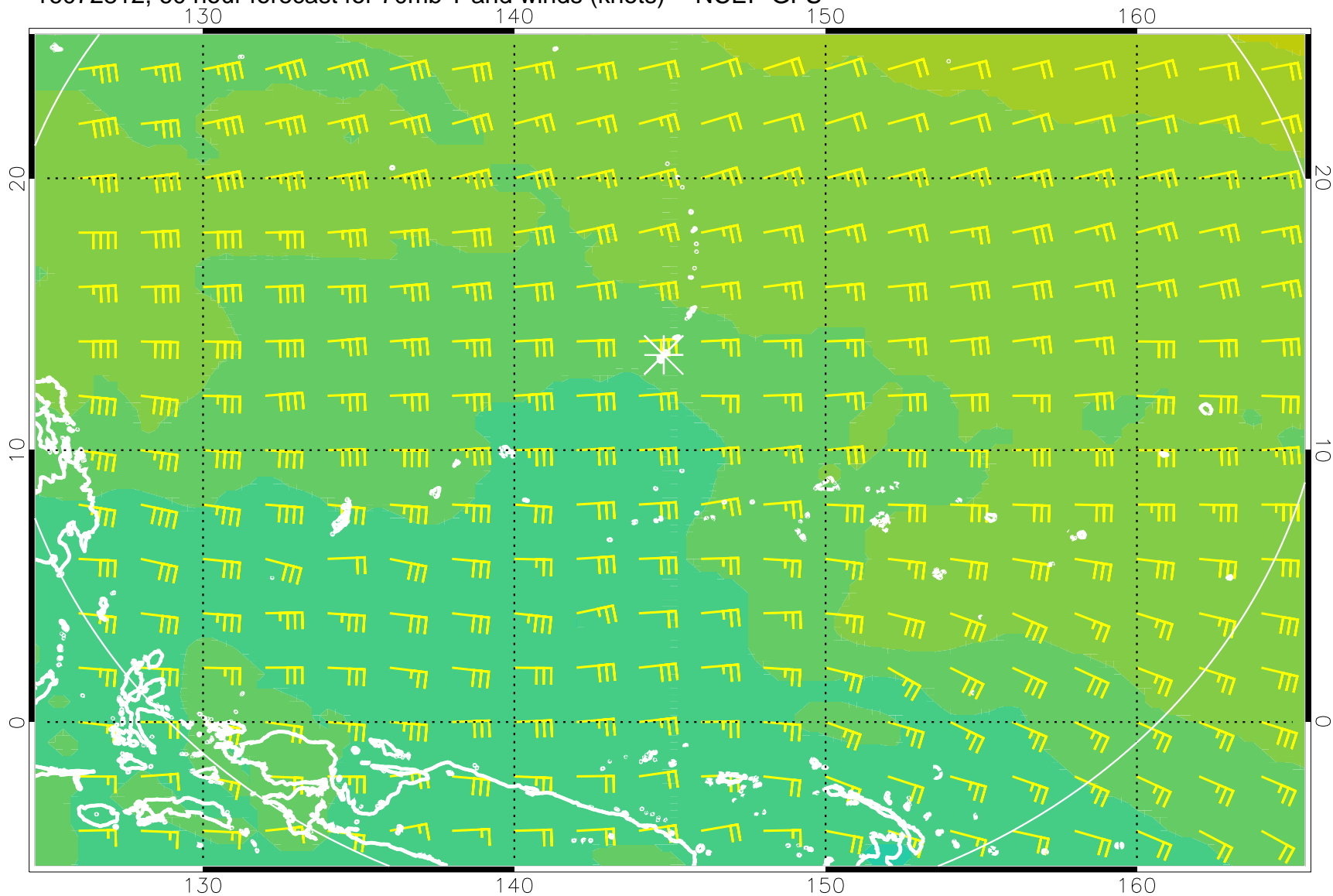
16072812, 60 hour forecast for 70mb T and winds (knots) -- NCEP GFS
