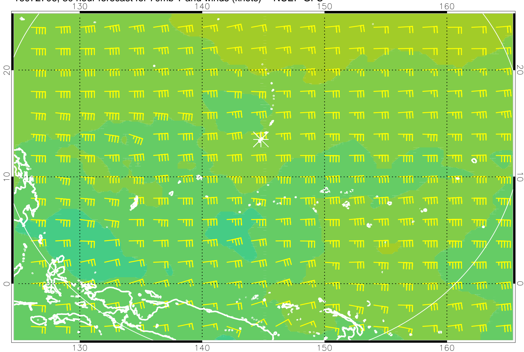
16072706, 30 hour forecast for 70mb T and winds (knots) -- NCEP GFS
