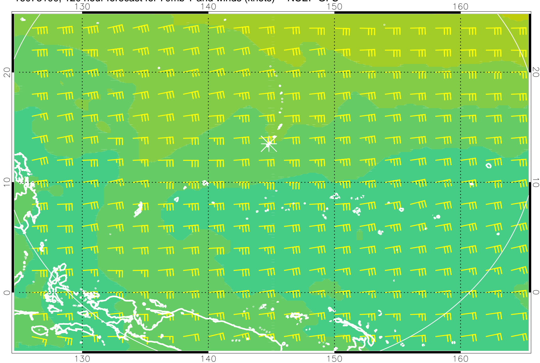
16073100, 120 hour forecast for 70mb T and winds (knots) -- NCEP GFS
