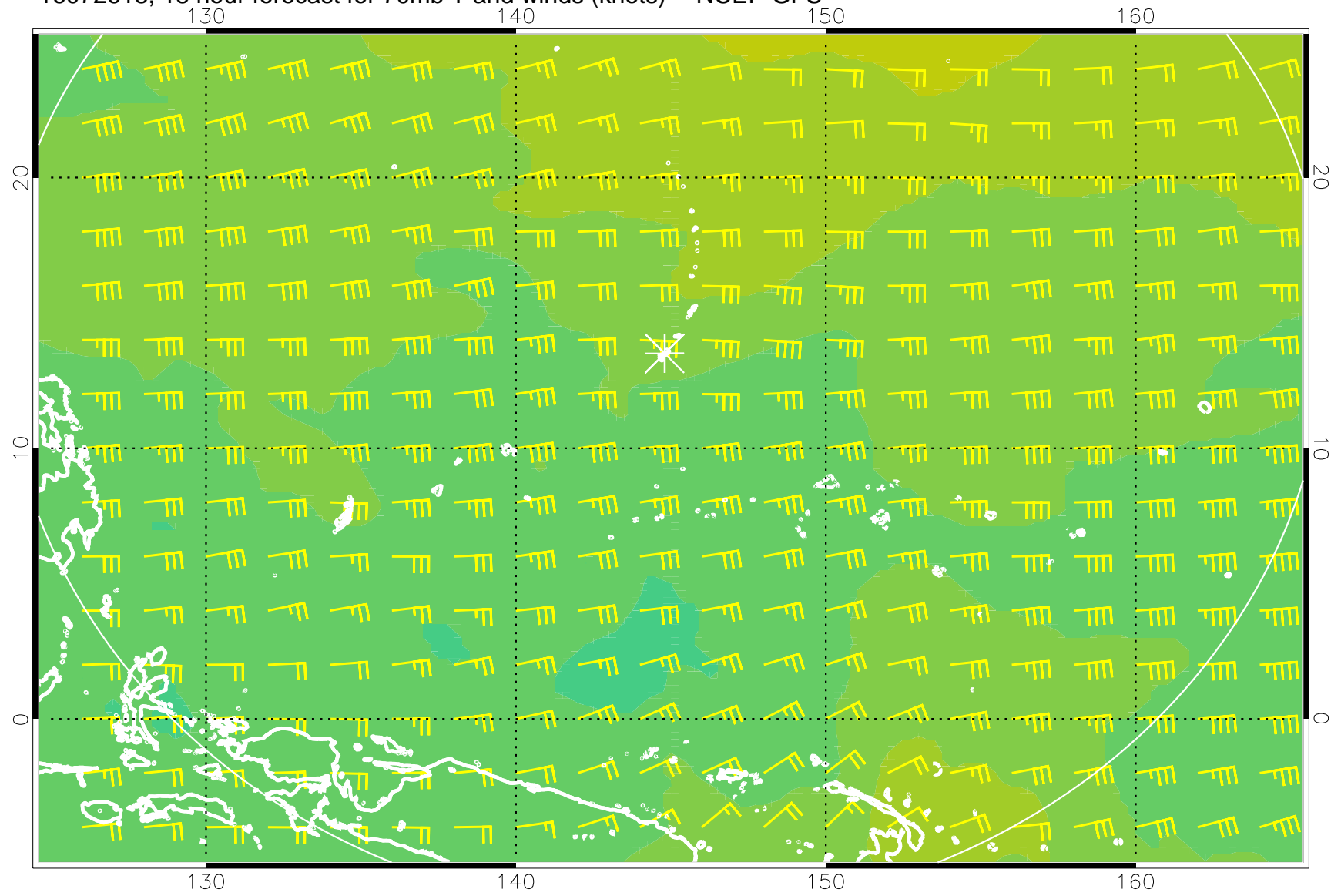
16072618, 18 hour forecast for 70mb T and winds (knots) -- NCEP GFS
