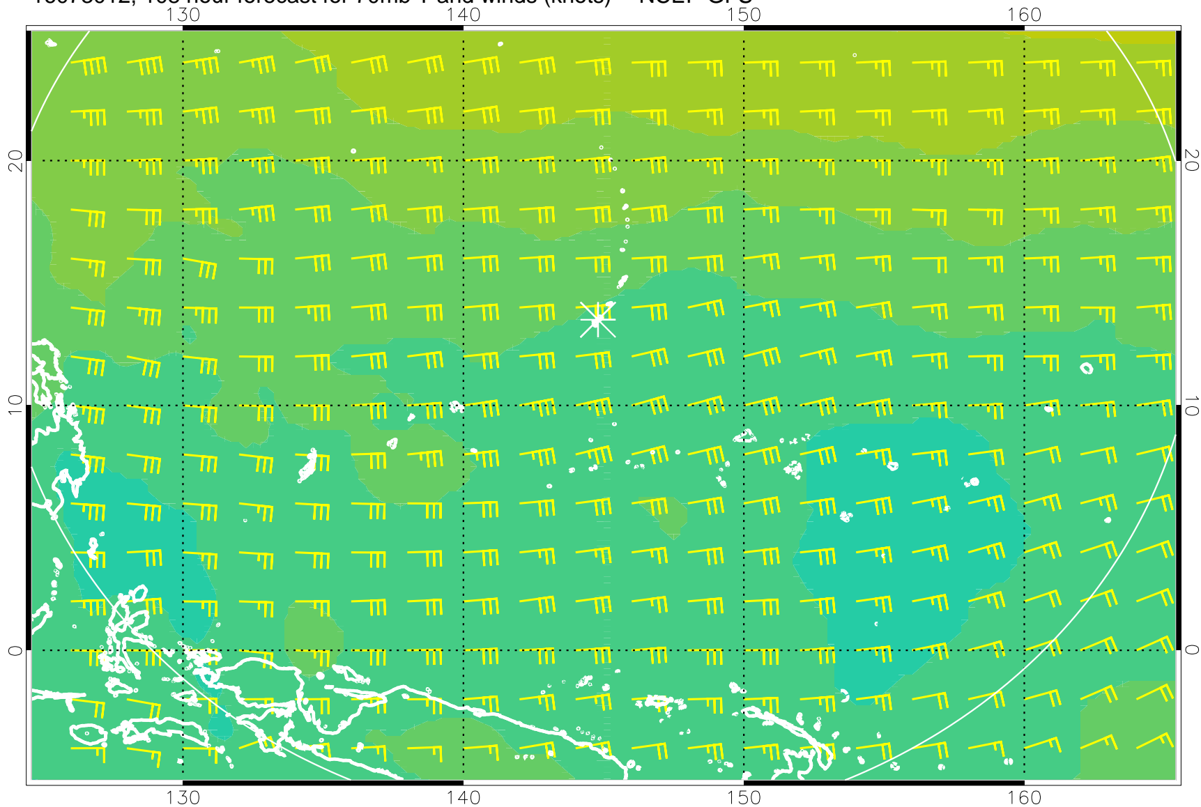
16073012, 108 hour forecast for 70mb T and winds (knots) -- NCEP GFS
