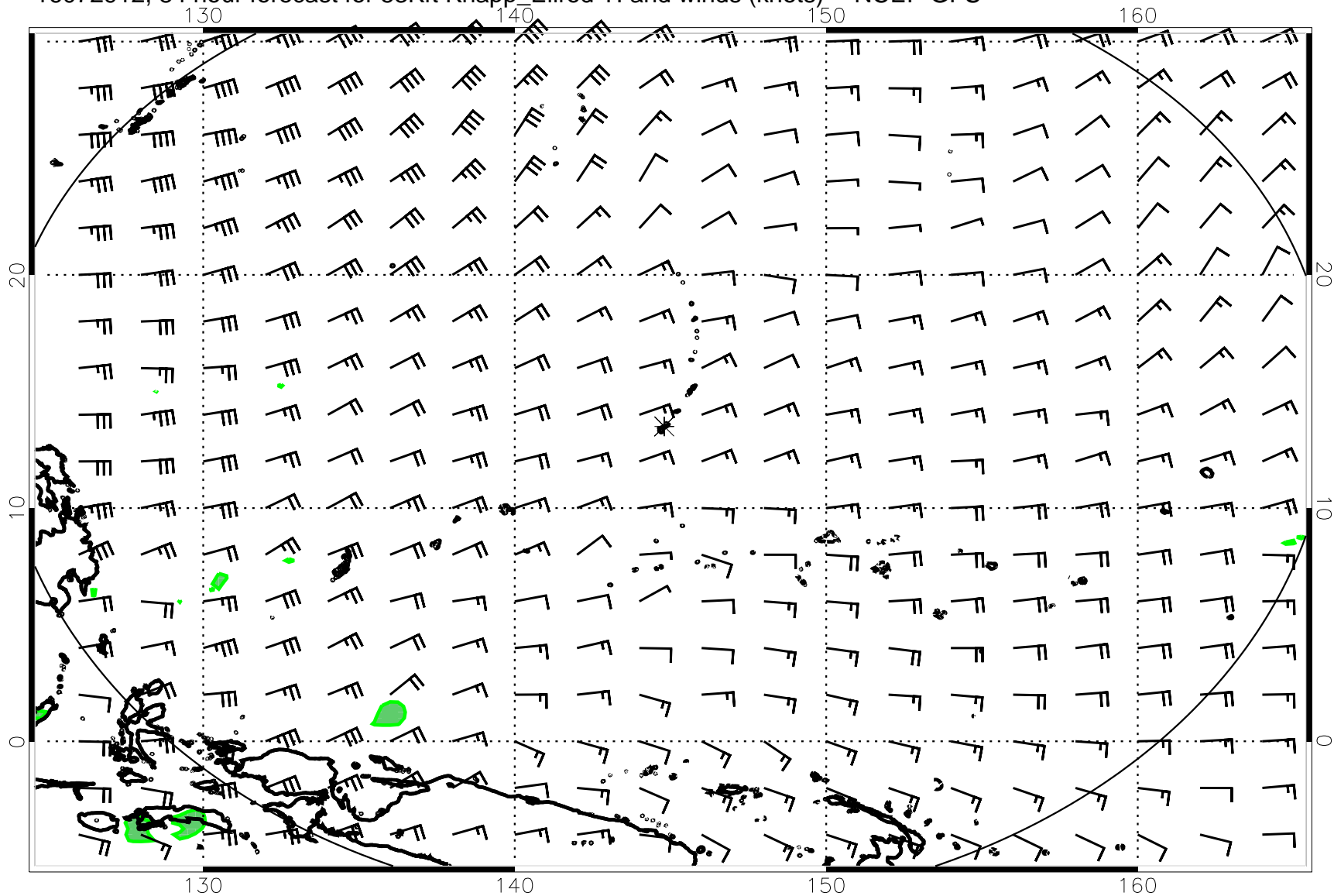
16072912, 84 hour forecast for 53Kft Knapp_Ellrod TI and winds (knots) -- NCEP GFS
