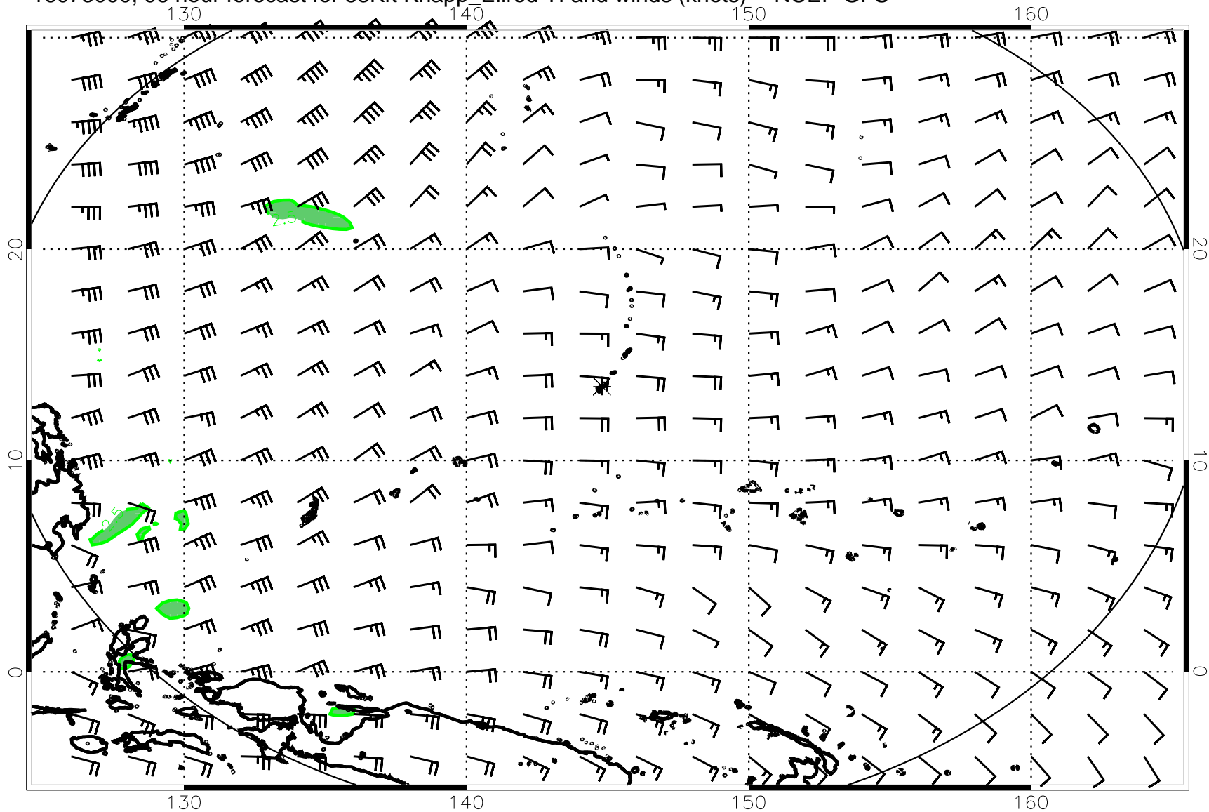
16073000, 96 hour forecast for 53Kft Knapp_Ellrod TI and winds (knots) -- NCEP GFS
