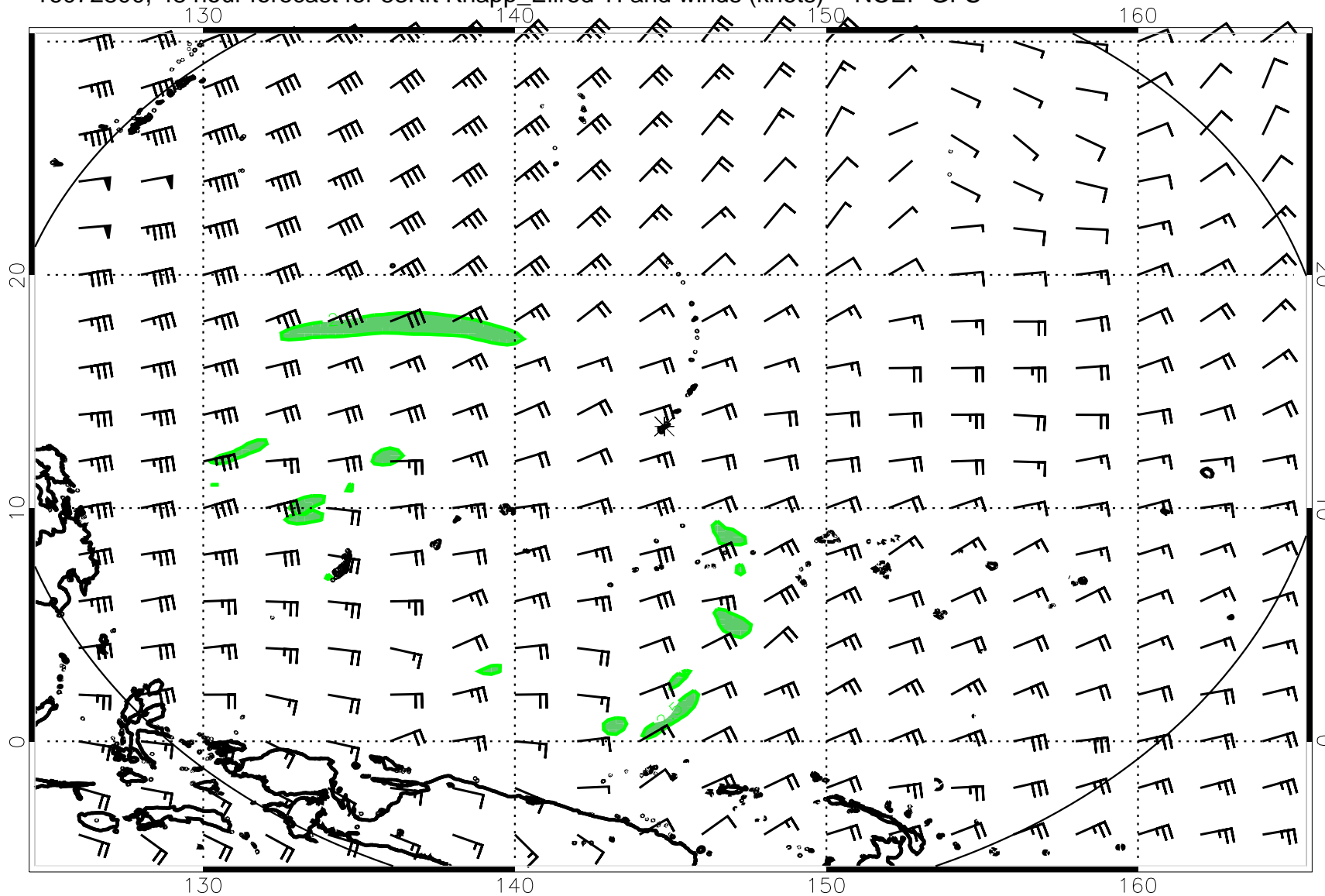
16072800, 48 hour forecast for 53Kft Knapp_Ellrod TI and winds (knots) -- NCEP GFS
