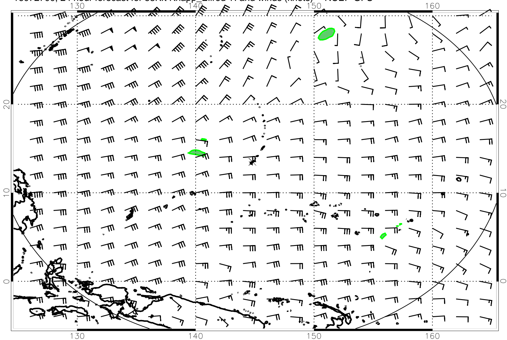
16072700, 24 hour forecast for 53Kft Knapp_Ellrod TI and winds (knots) -- NCEP GFS
