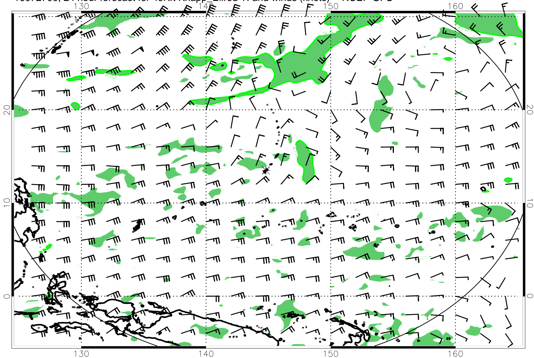
16072700, 24 hour forecast for 49Kft Knapp_Ellrod TI and winds (knots) -- NCEP GFS
