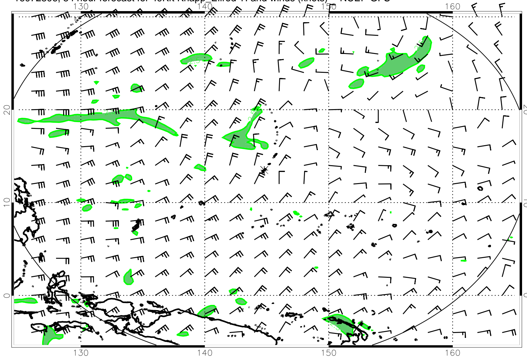
16072806, 54 hour forecast for 49Kft Knapp_Ellrod TI and winds (knots) -- NCEP GFS
