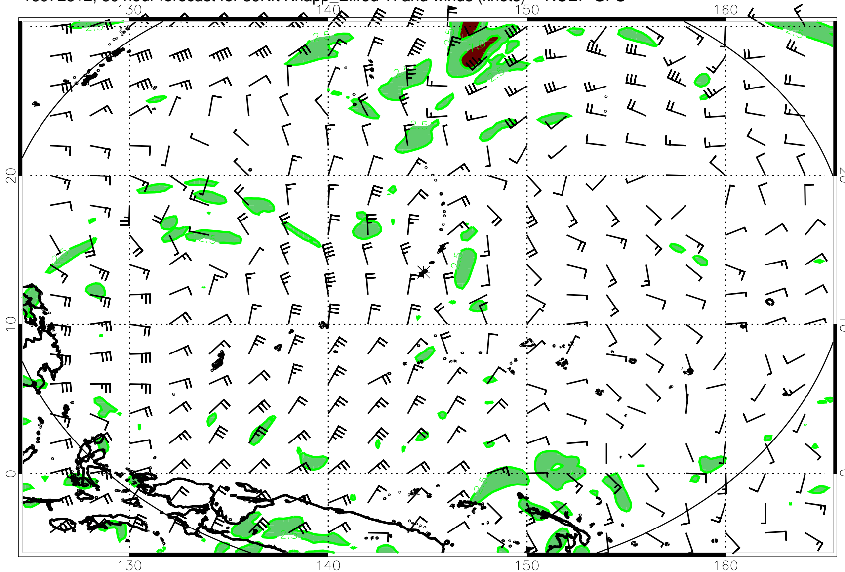
16072812, 60 hour forecast for 39Kft Knapp_Ellrod TI and winds (knots) -- NCEP GFS
