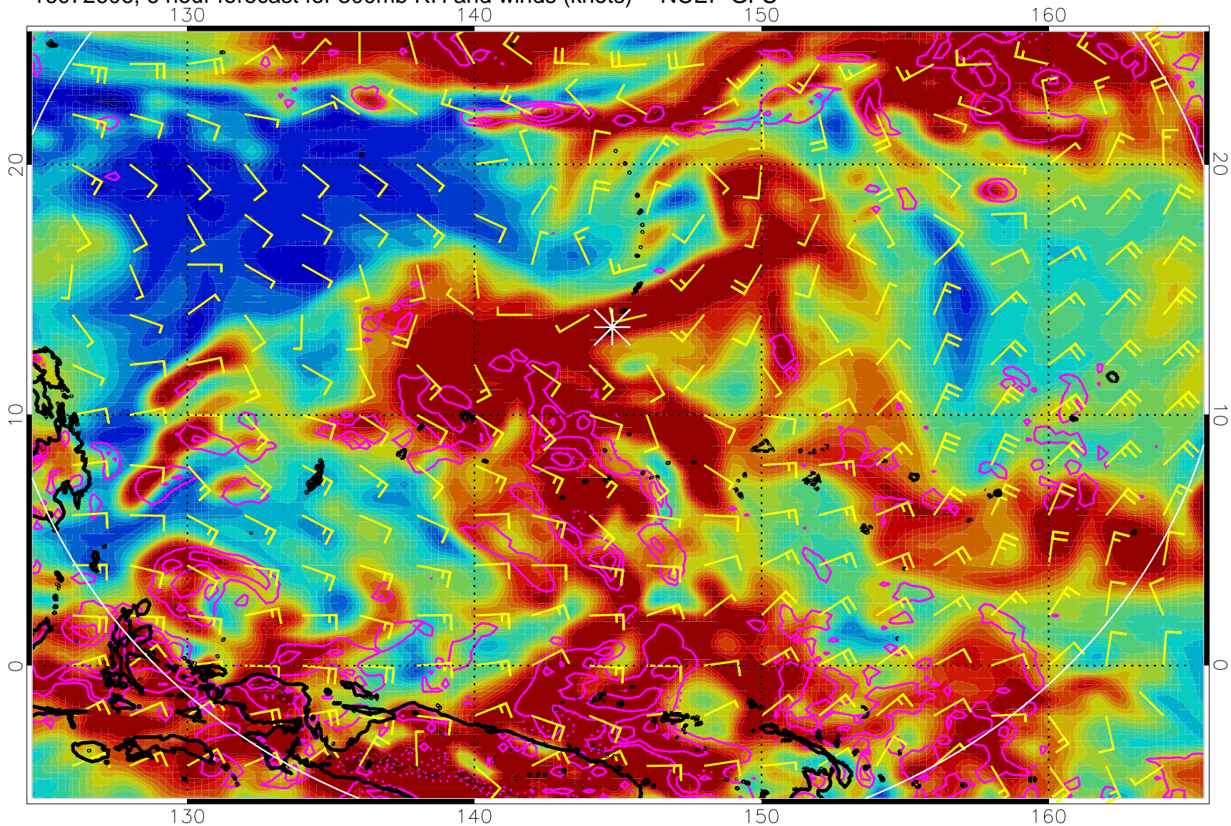
16072606, 6 hour forecast for 300mb RH and winds (knots) -- NCEP GFS
