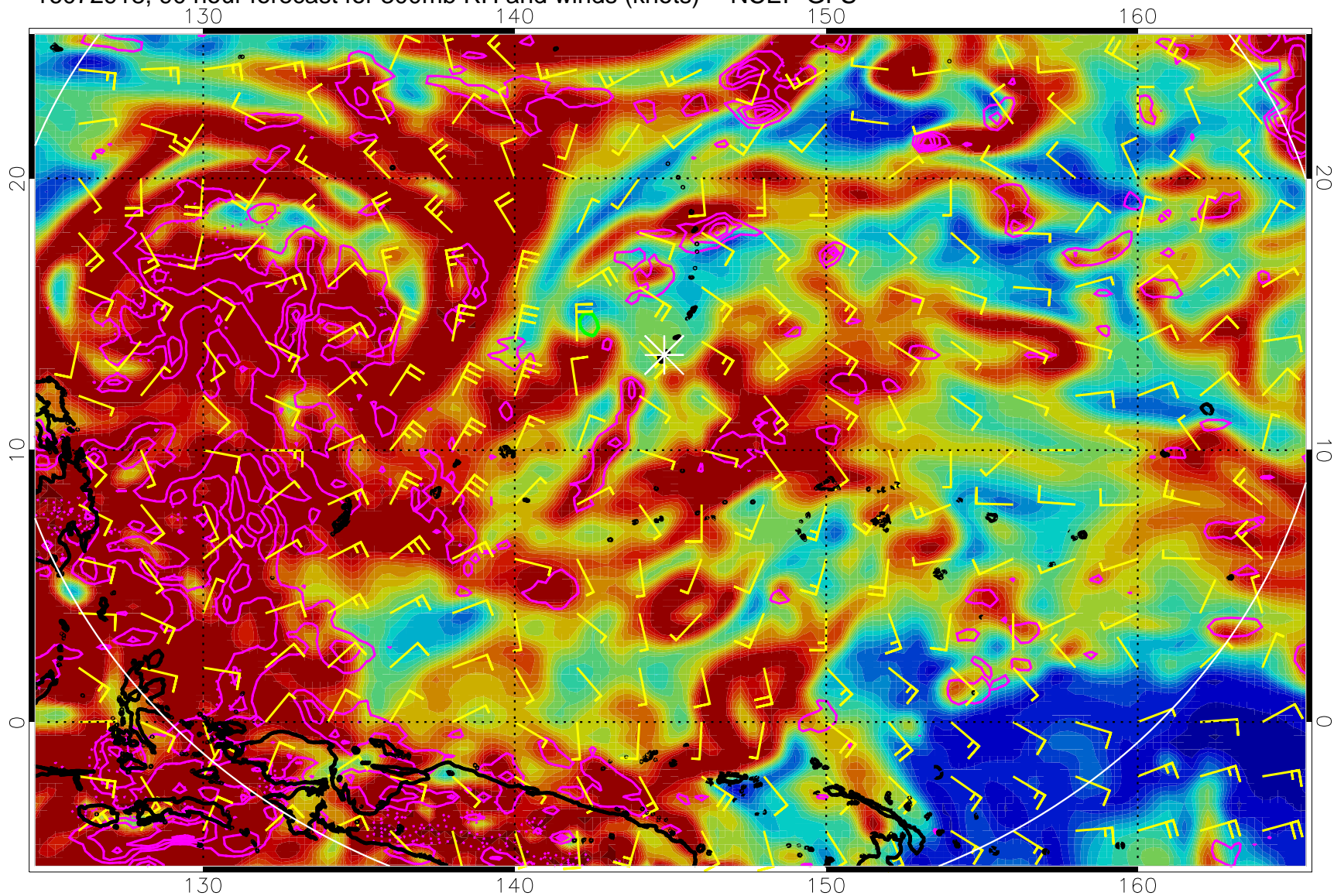
16072918, 90 hour forecast for 300mb RH and winds (knots) -- NCEP GFS
