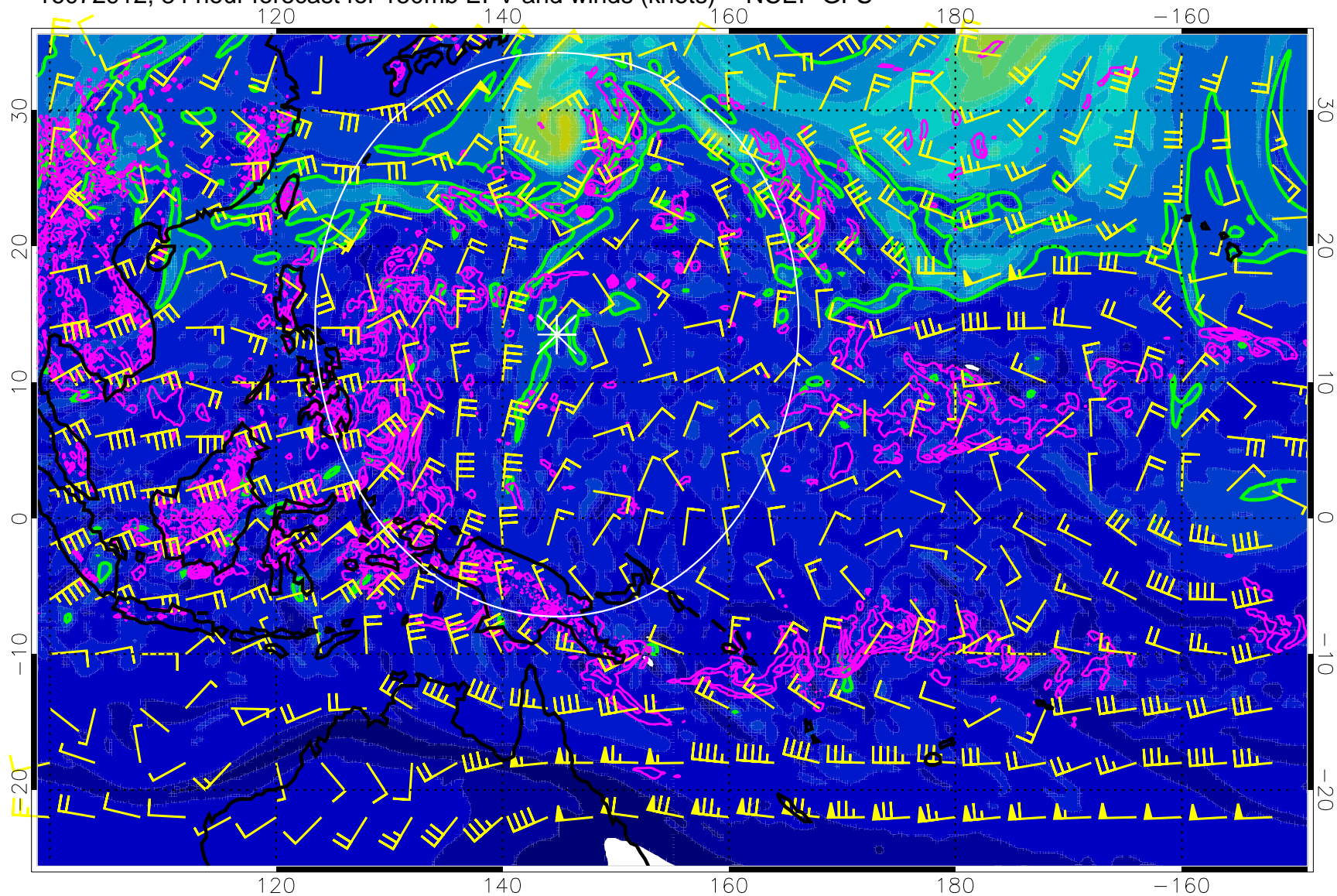
16072912, 84 hour forecast for 150mb EPV and winds (knots) -- NCEP GFS
