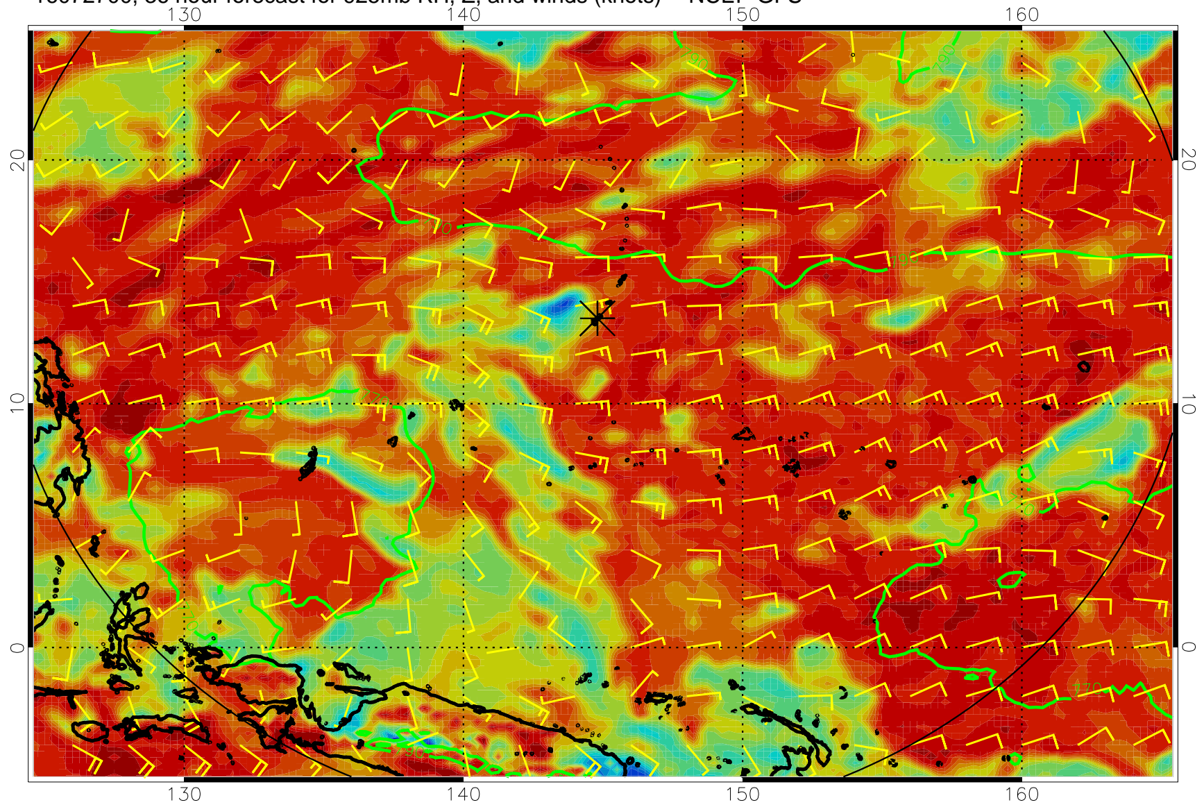
16072700, 36 hour forecast for 925mb RH, Z, and winds (knots) -- NCEP GFS
