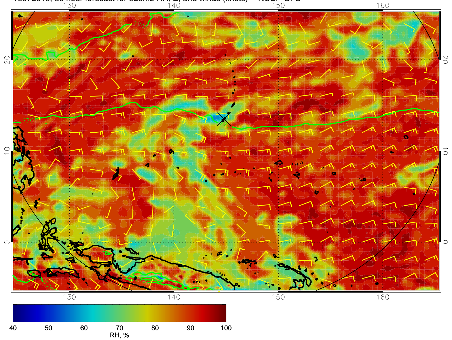
16072618, 30 hour forecast for 925mb RH, Z, and winds (knots) -- NCEP GFS
