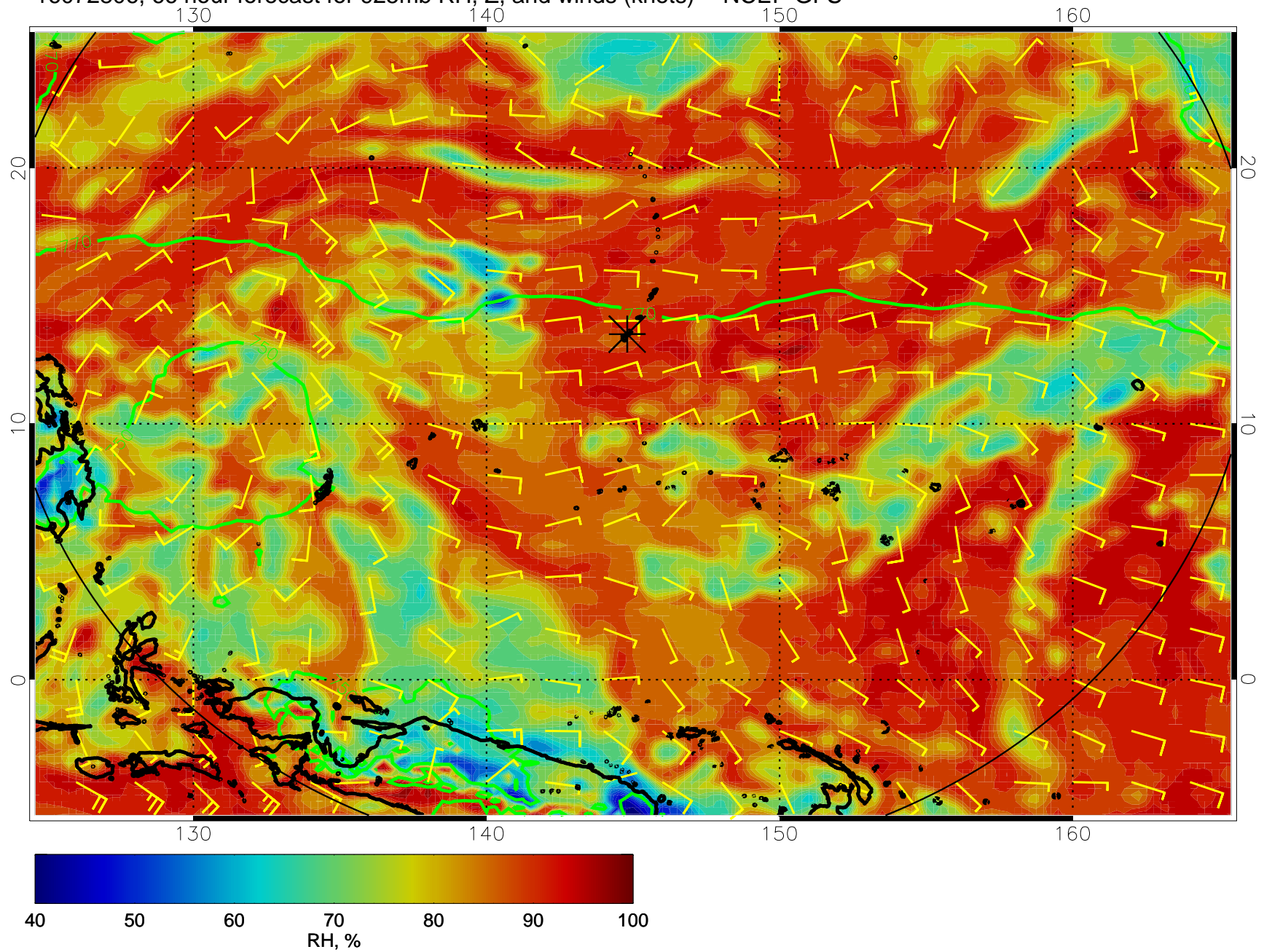
16072806, 66 hour forecast for 925mb RH, Z, and winds (knots) -- NCEP GFS
