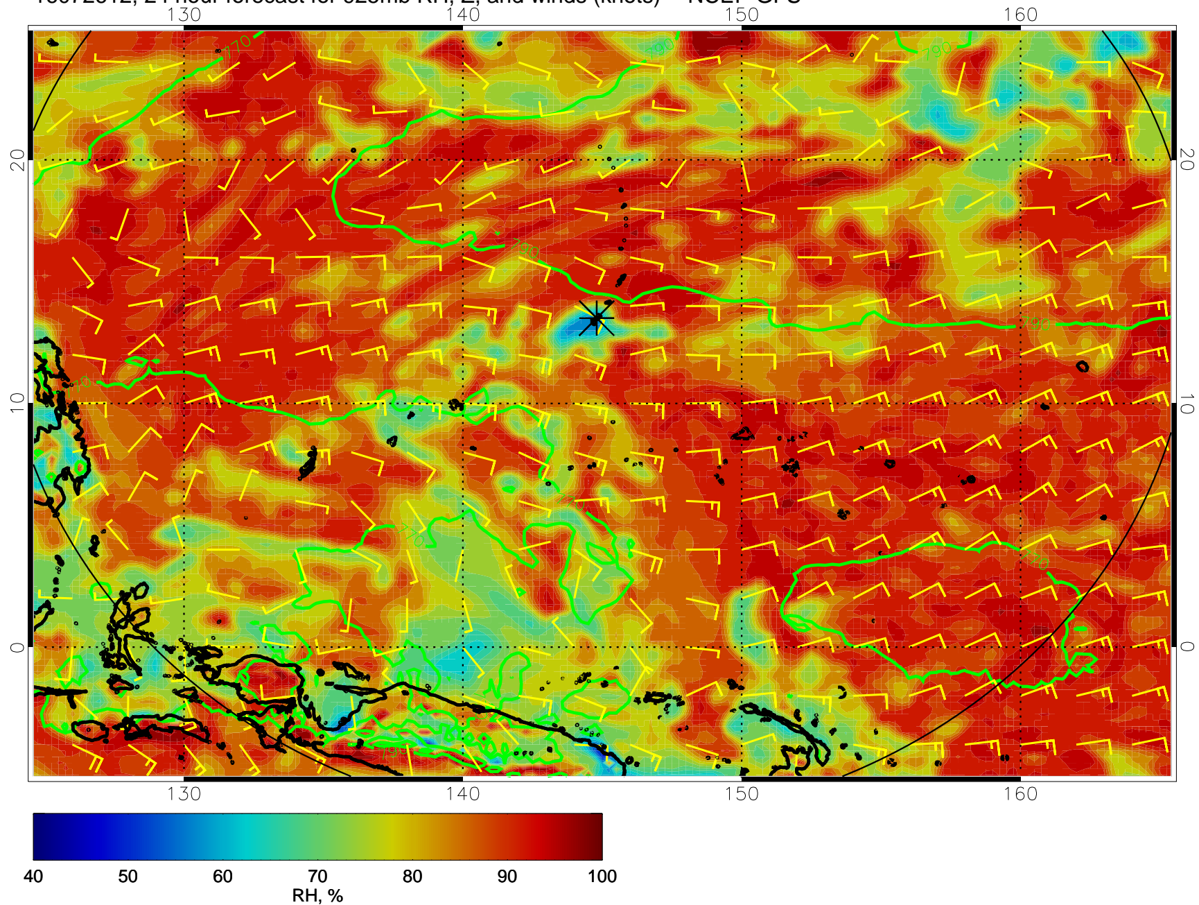
16072612, 24 hour forecast for 925mb RH, Z, and winds (knots) -- NCEP GFS
