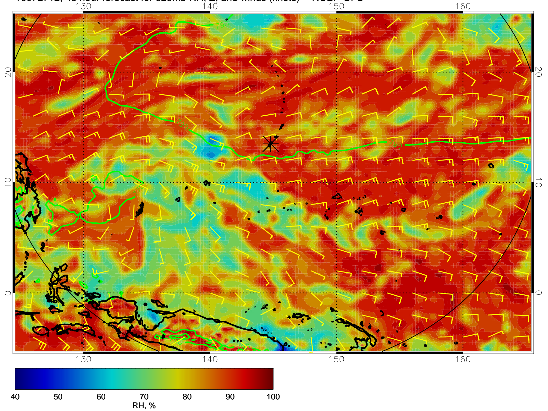
16072712, 48 hour forecast for 925mb RH, Z, and winds (knots) -- NCEP GFS
