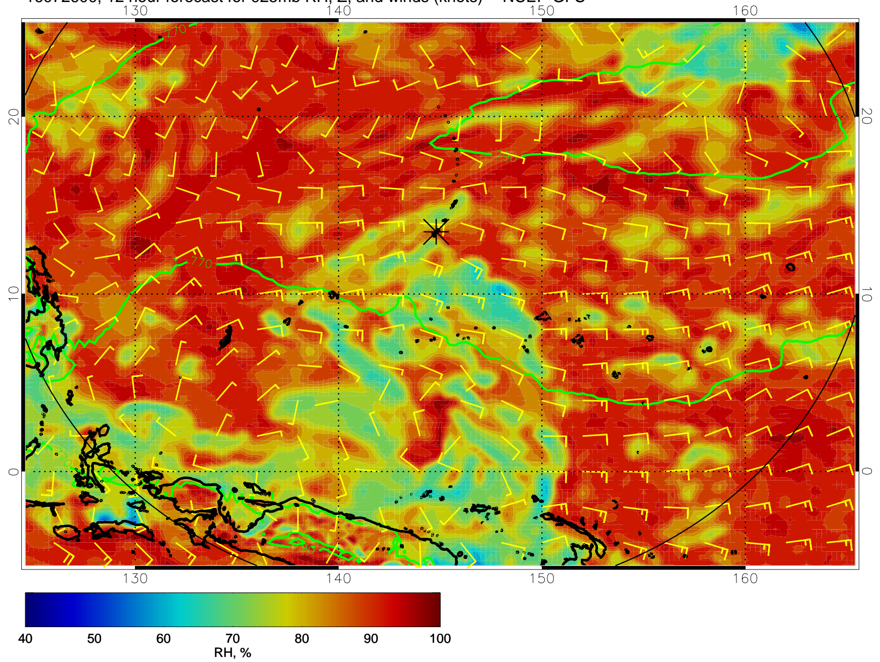
16072600, 12 hour forecast for 925mb RH, Z, and winds (knots) -- NCEP GFS
