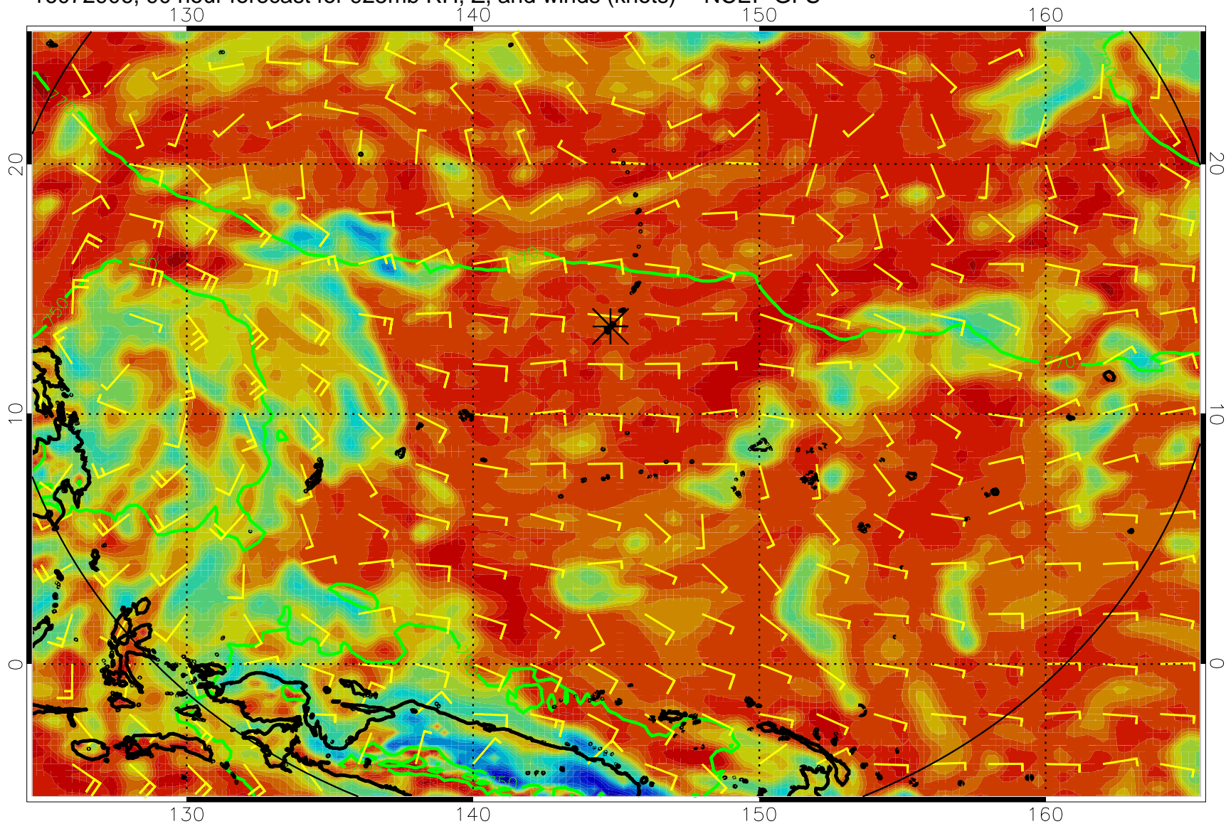
16072906, 90 hour forecast for 925mb RH, Z, and winds (knots) -- NCEP GFS
