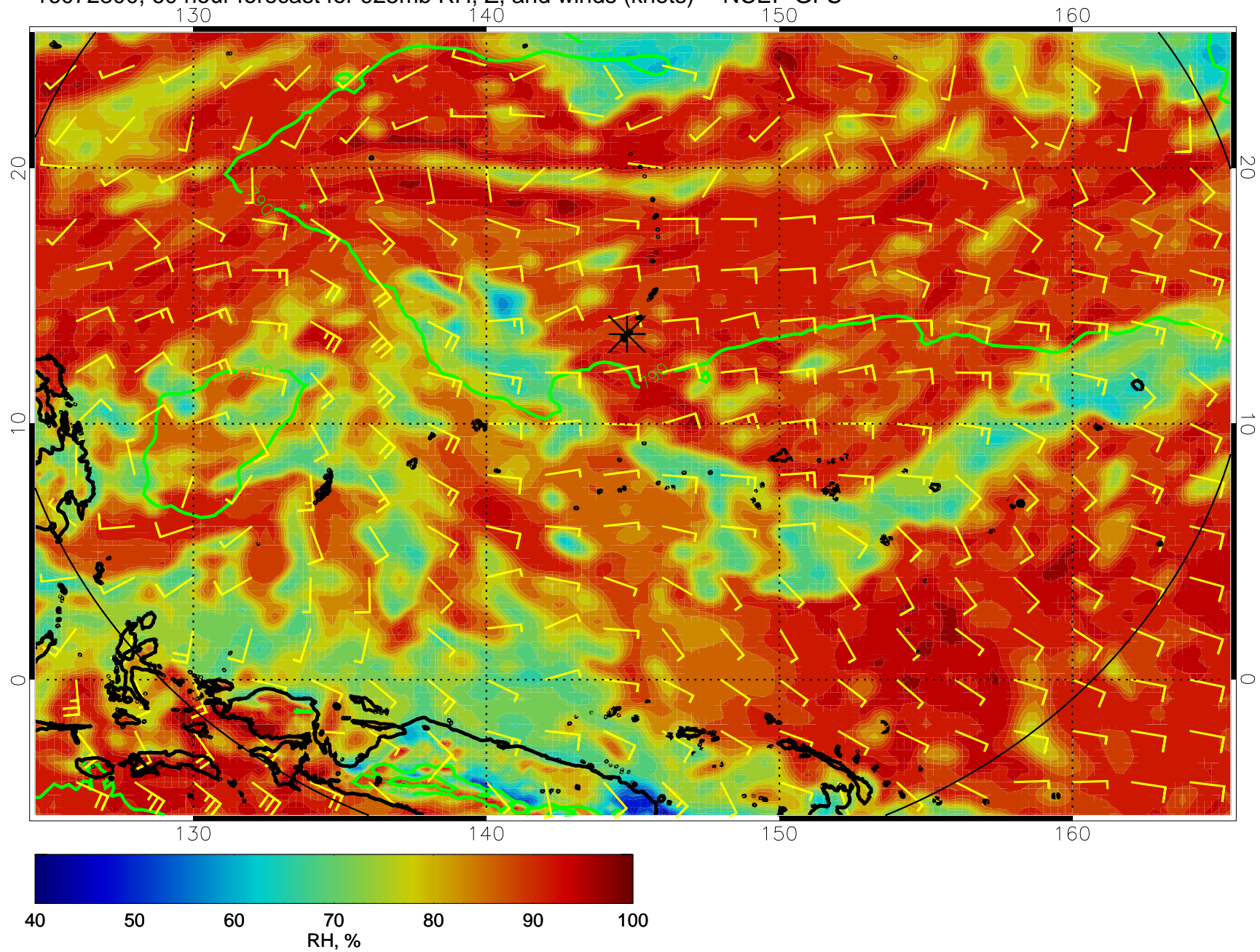
16072800, 60 hour forecast for 925mb RH, Z, and winds (knots) -- NCEP GFS
