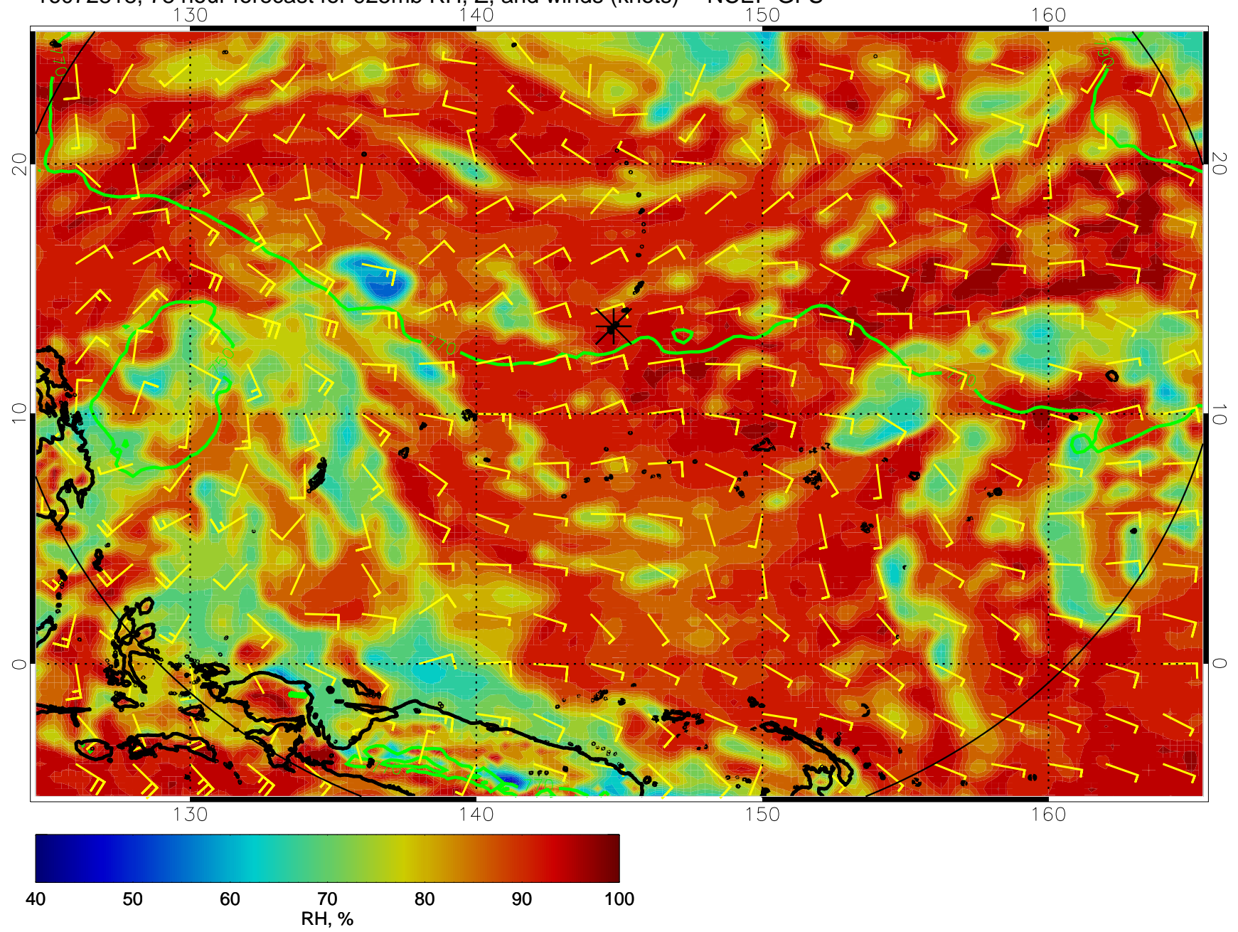
16072818, 78 hour forecast for 925mb RH, Z, and winds (knots) -- NCEP GFS
