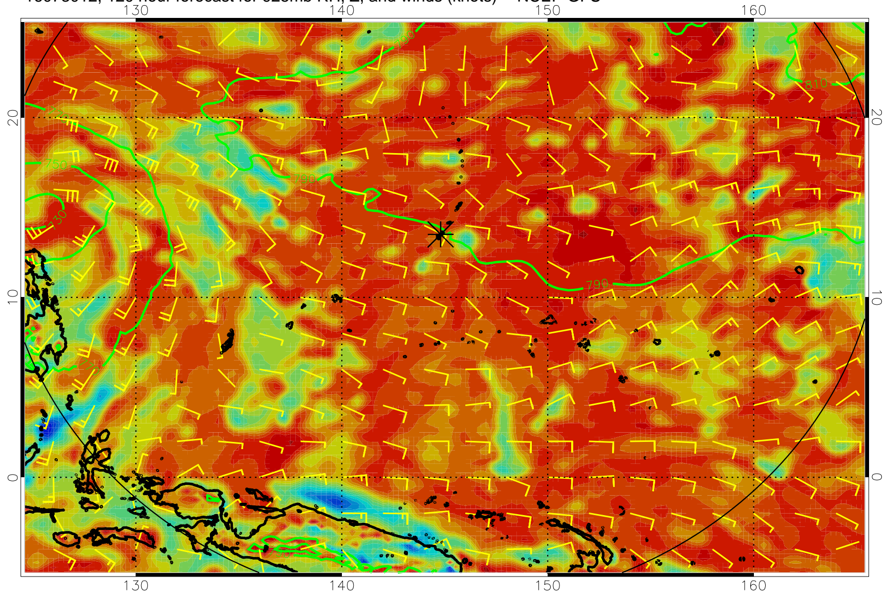
16073012, 120 hour forecast for 925mb RH, Z, and winds (knots) -- NCEP GFS
