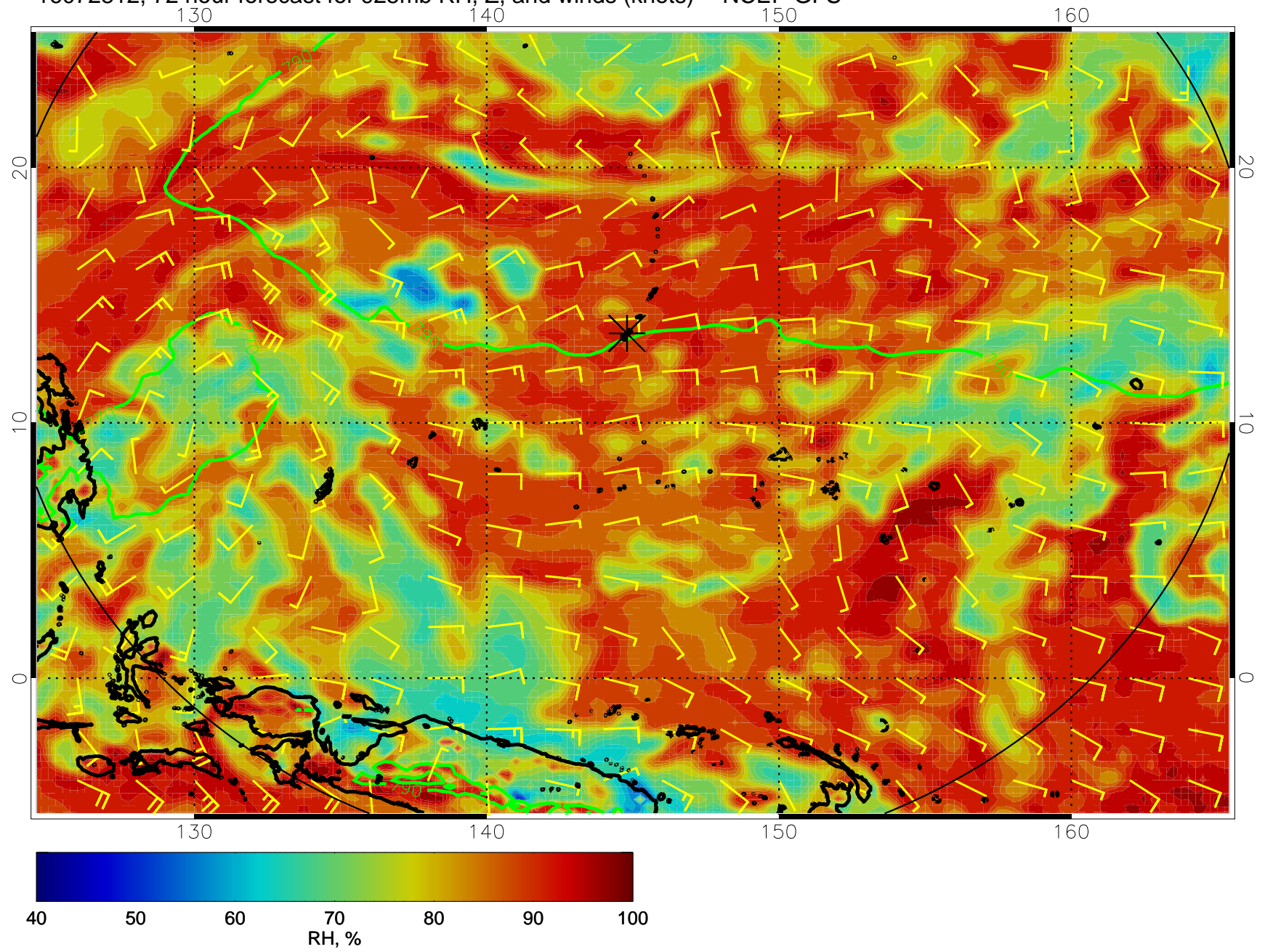
16072812, 72 hour forecast for 925mb RH, Z, and winds (knots) -- NCEP GFS
