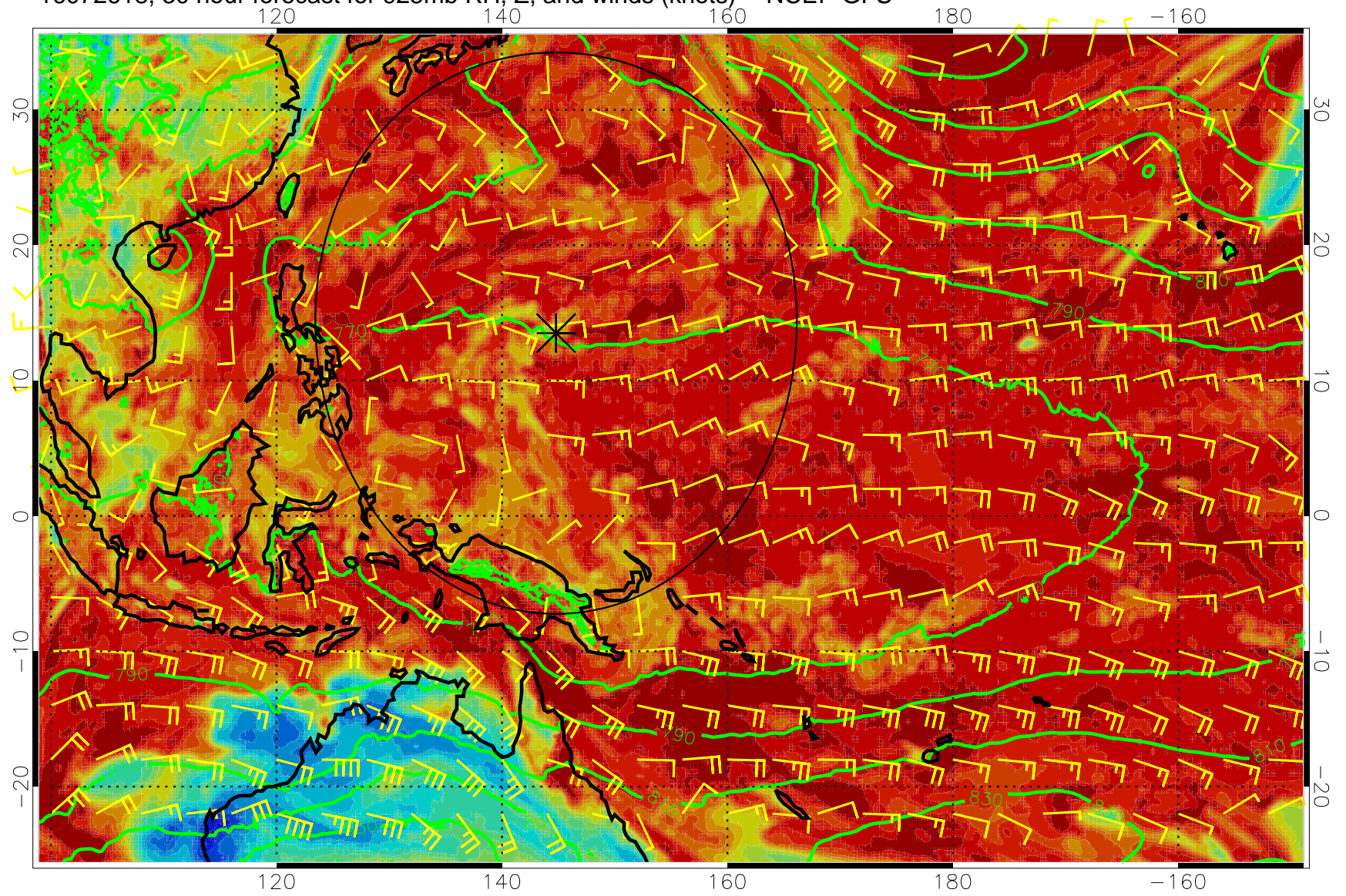
16072618, 30 hour forecast for 925mb RH, Z, and winds (knots) -- NCEP GFS
