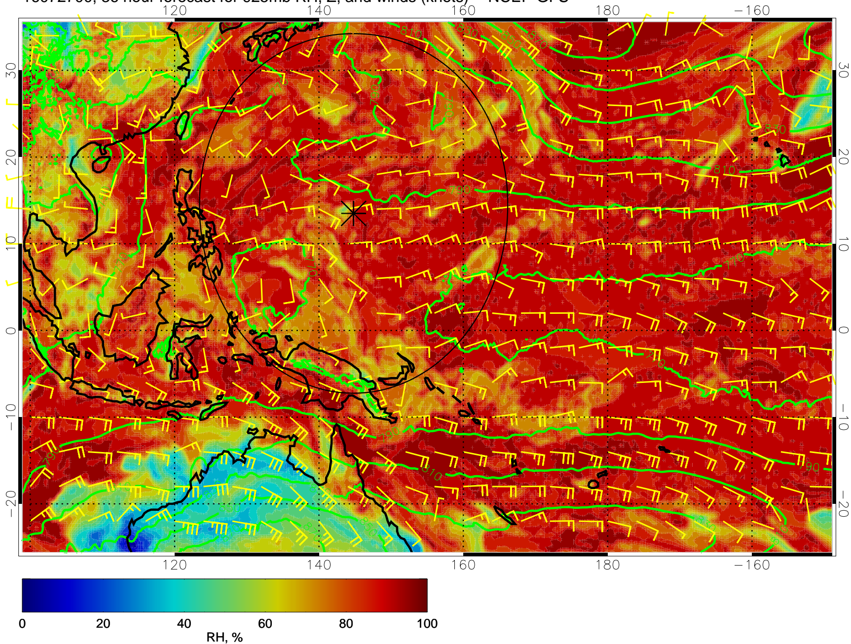
16072700, 36 hour forecast for 925mb RH, Z, and winds (knots) -- NCEP GFS
