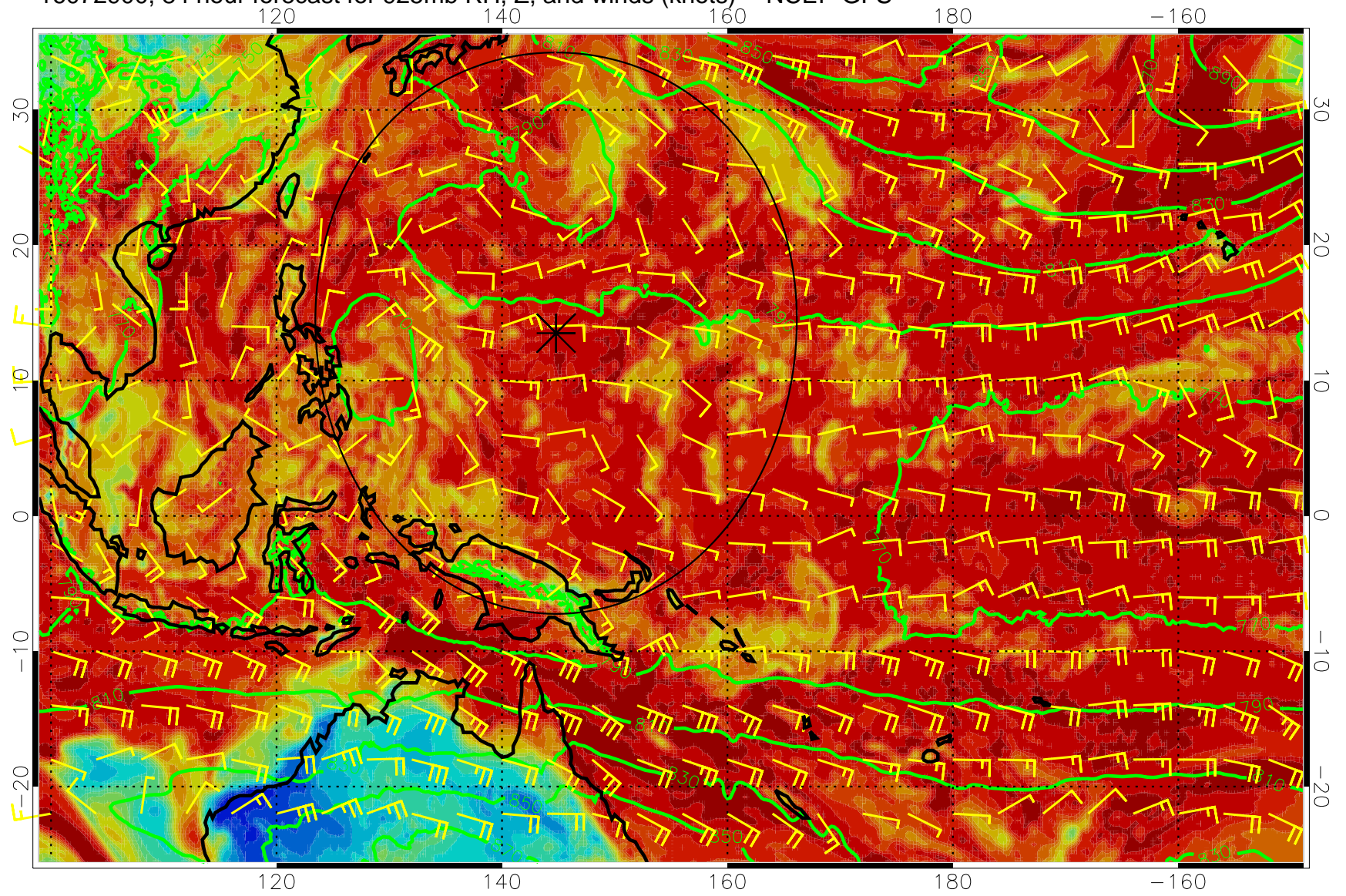
16072900, 84 hour forecast for 925mb RH, Z, and winds (knots) -- NCEP GFS
