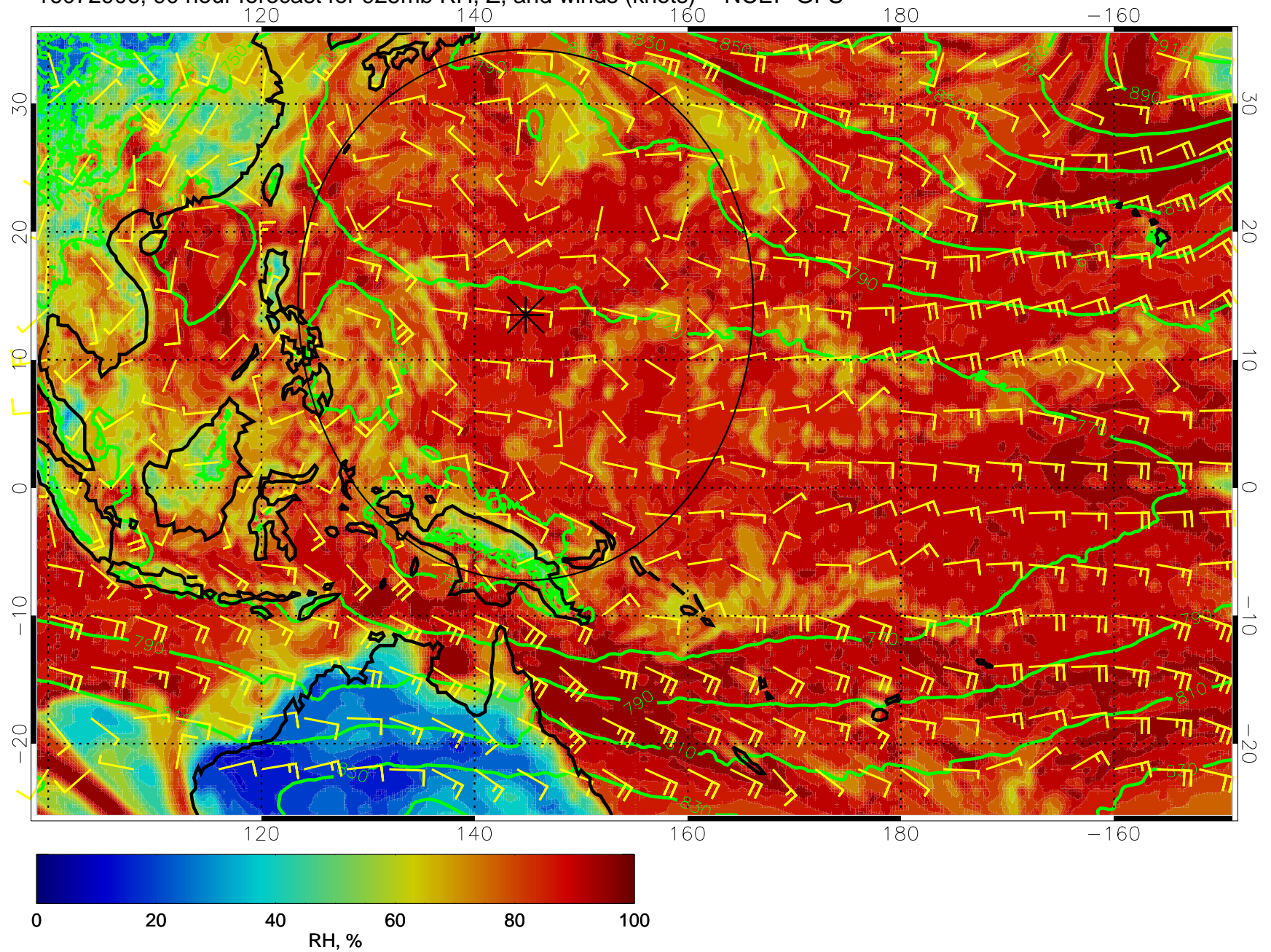
16072906, 90 hour forecast for 925mb RH, Z, and winds (knots) -- NCEP GFS
