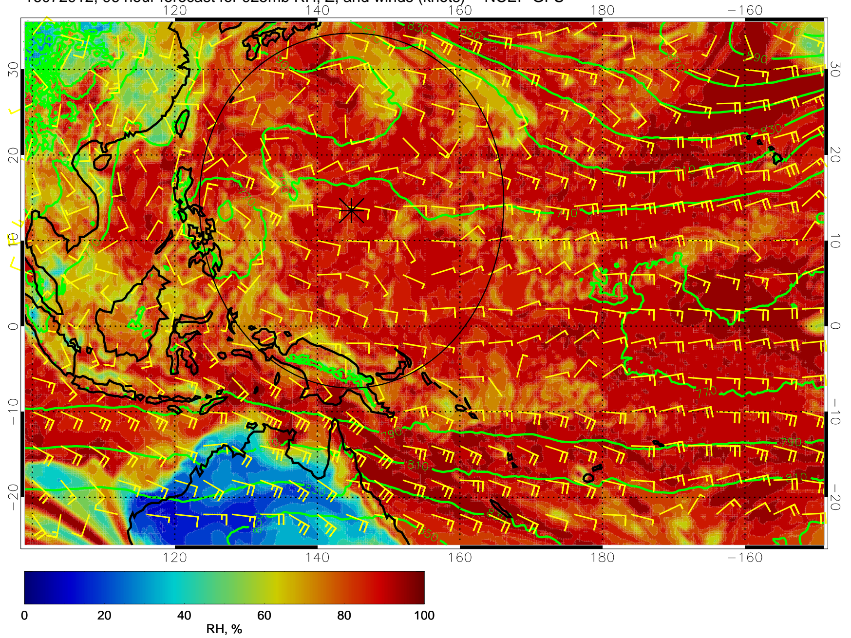
16072912, 96 hour forecast for 925mb RH, Z, and winds (knots) -- NCEP GFS
