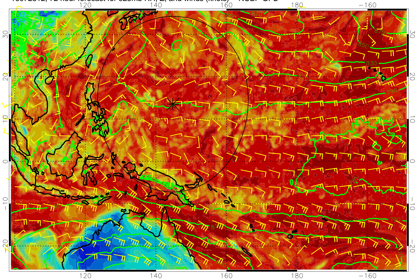
16072812, 72 hour forecast for 925mb RH, Z, and winds (knots) -- NCEP GFS
