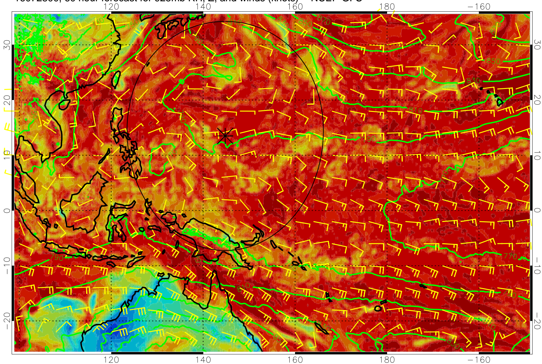
16072800, 60 hour forecast for 925mb RH, Z, and winds (knots) -- NCEP GFS
