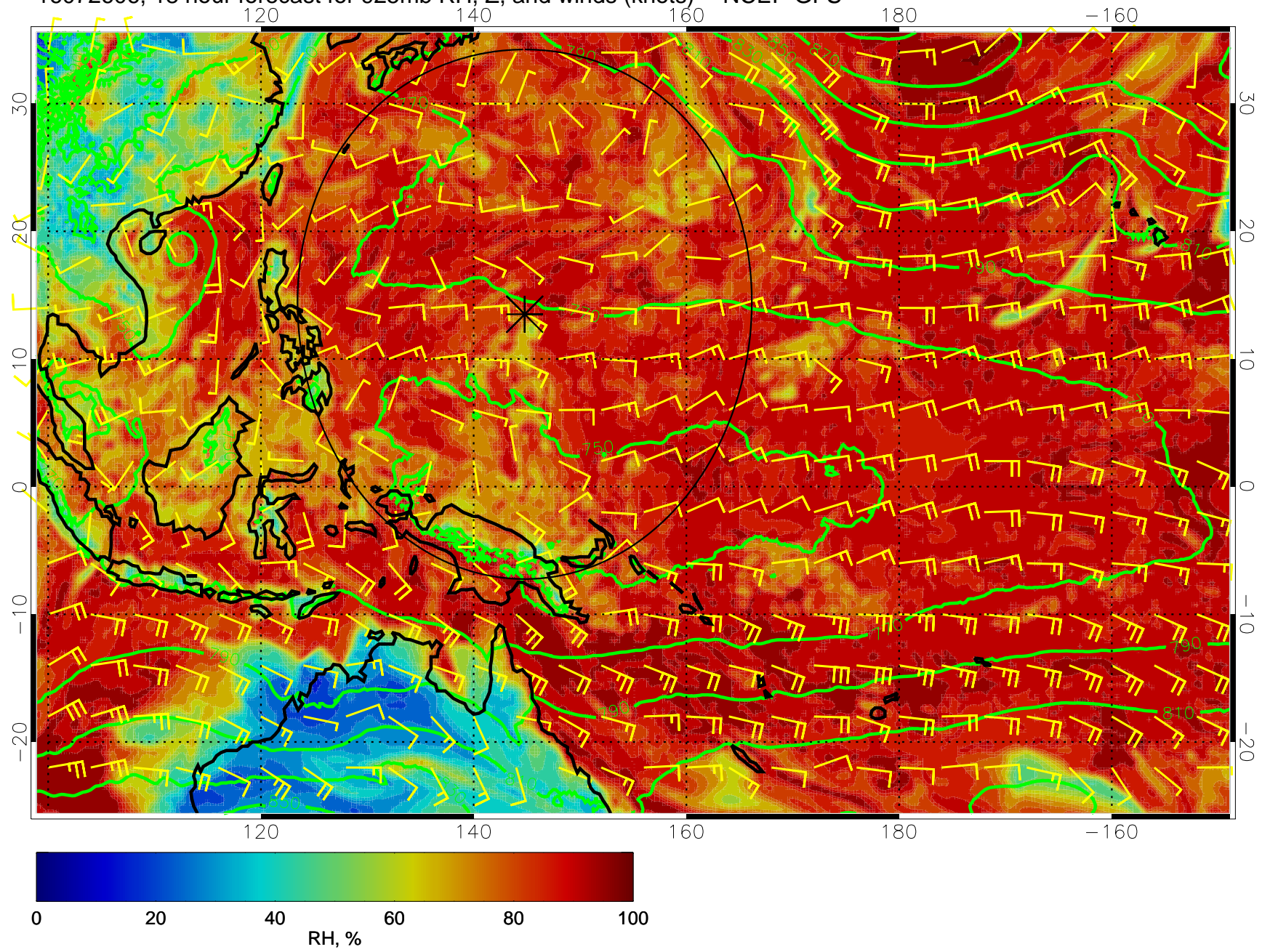
16072606, 18 hour forecast for 925mb RH, Z, and winds (knots) -- NCEP GFS
