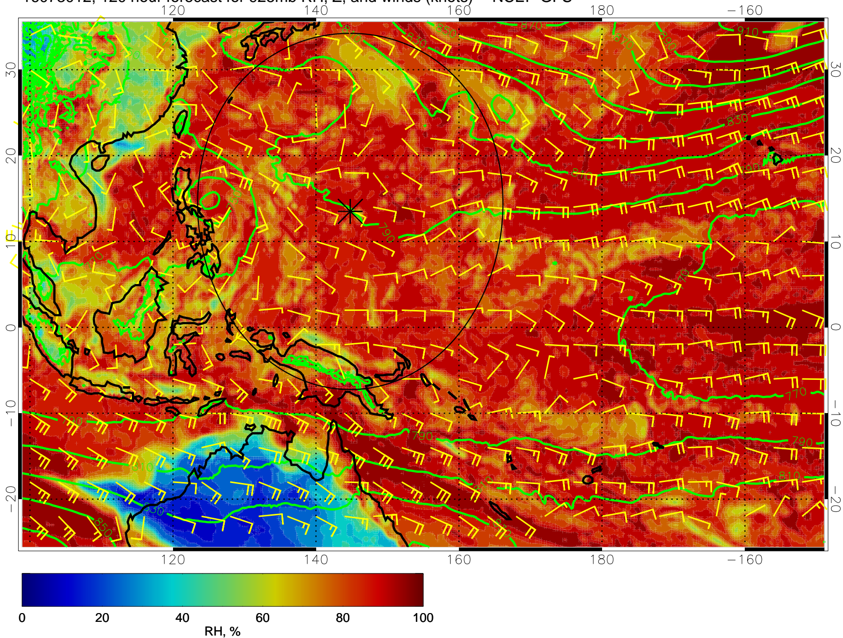
16073012, 120 hour forecast for 925mb RH, Z, and winds (knots) -- NCEP GFS
