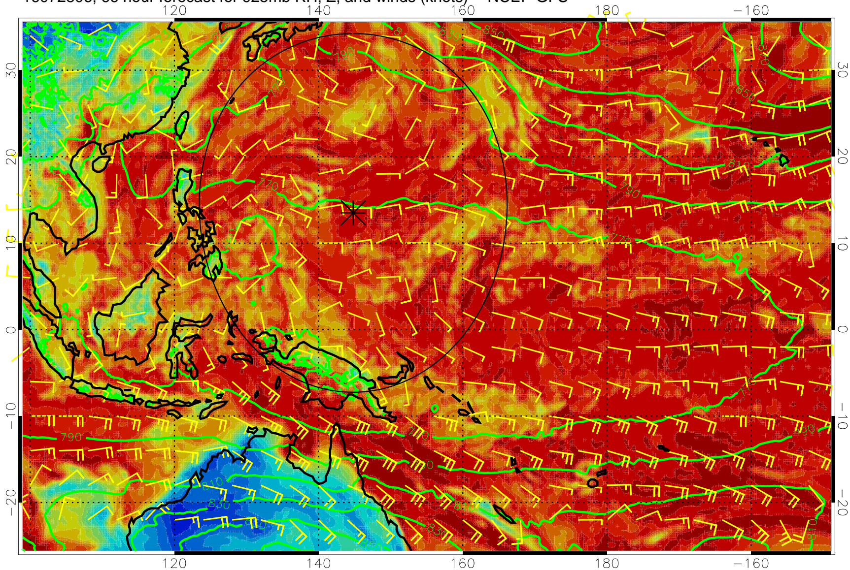
16072806, 66 hour forecast for 925mb RH, Z, and winds (knots) -- NCEP GFS
