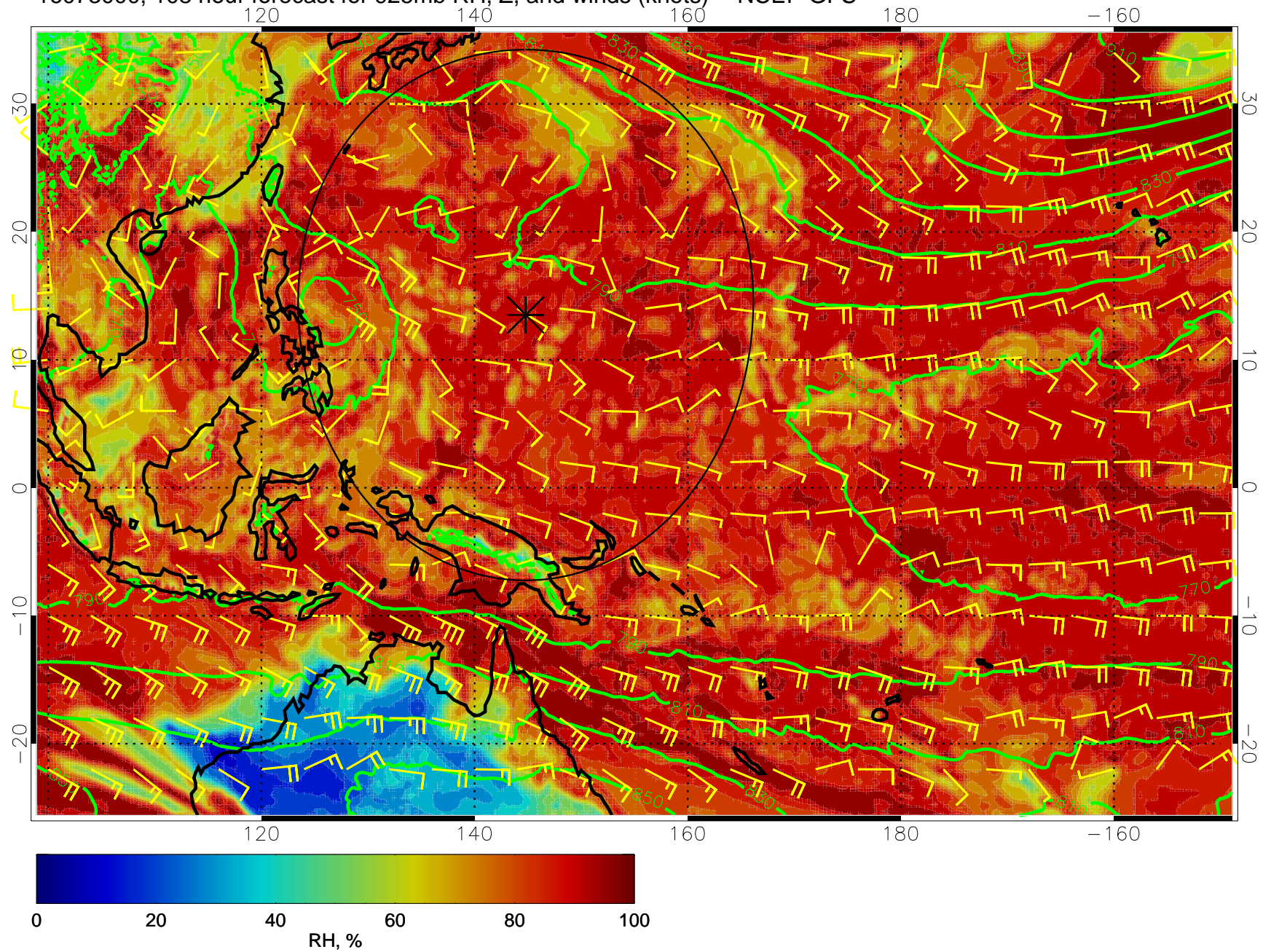
16073000, 108 hour forecast for 925mb RH, Z, and winds (knots) -- NCEP GFS
