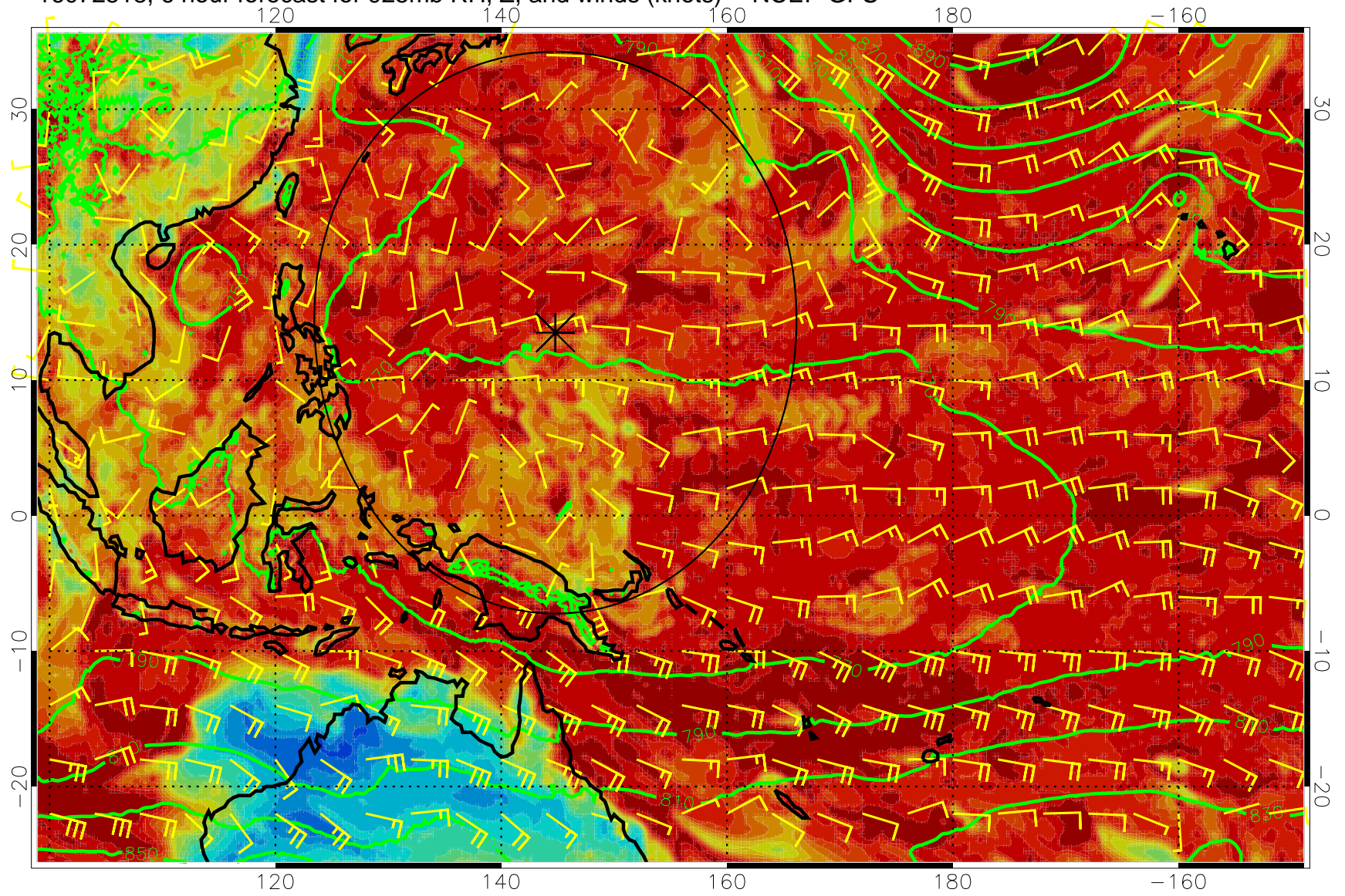
16072518, 6 hour forecast for 925mb RH, Z, and winds (knots) -- NCEP GFS
