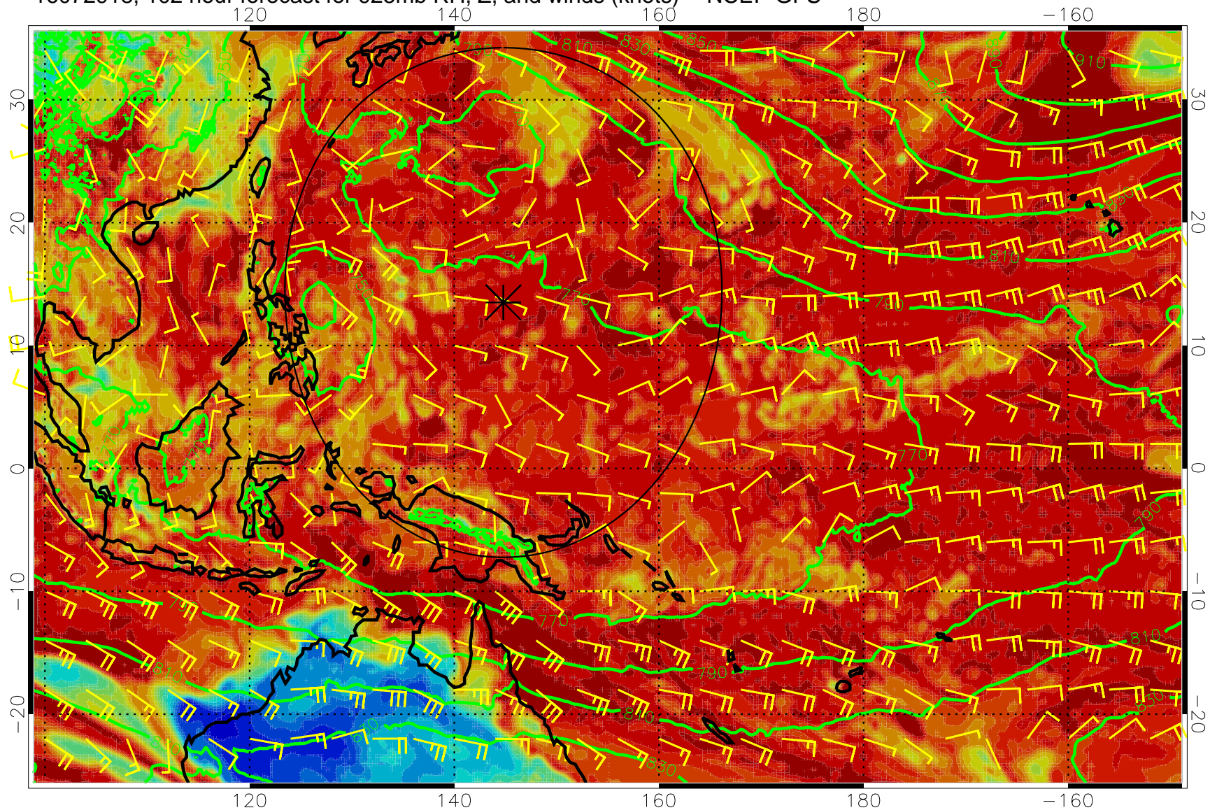
16072918, 102 hour forecast for 925mb RH, Z, and winds (knots) -- NCEP GFS
