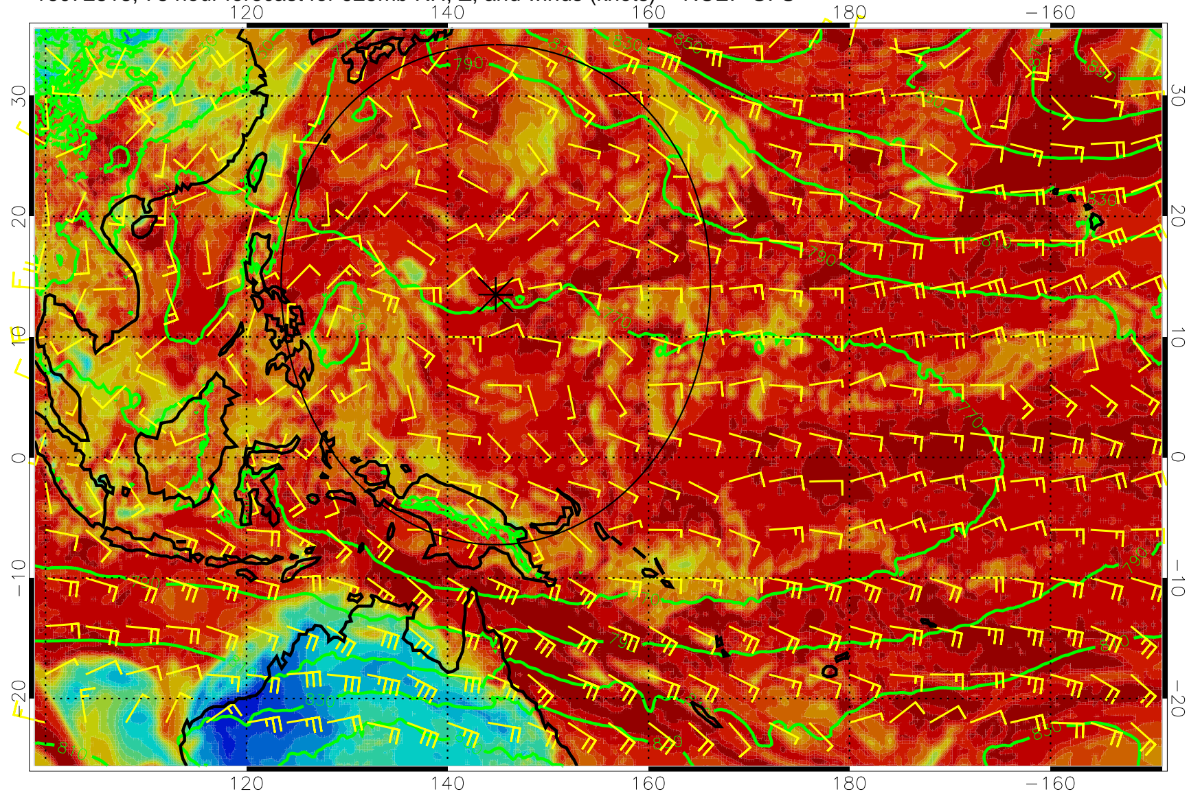
16072818, 78 hour forecast for 925mb RH, Z, and winds (knots) -- NCEP GFS
