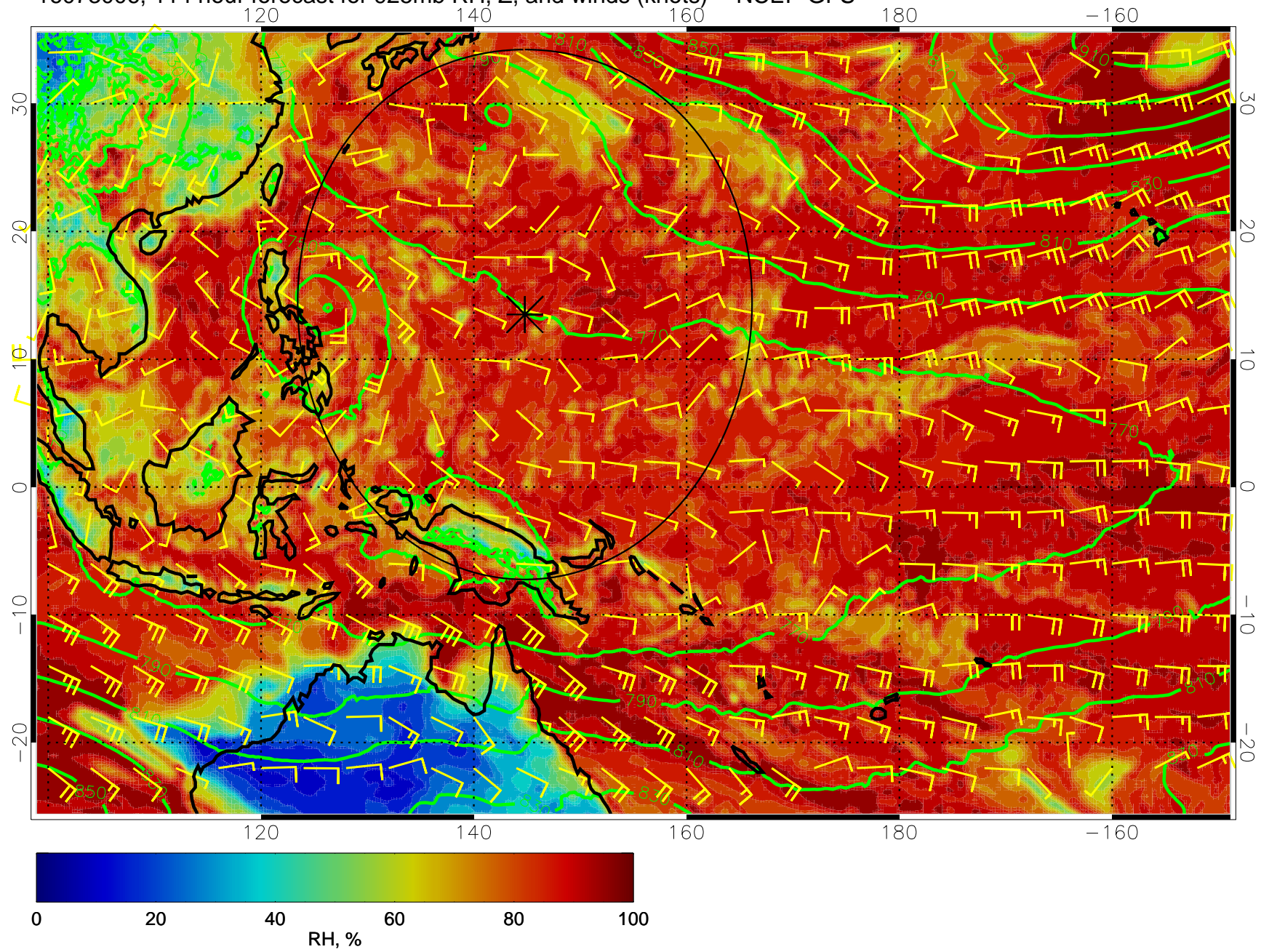
16073006, 114 hour forecast for 925mb RH, Z, and winds (knots) -- NCEP GFS
