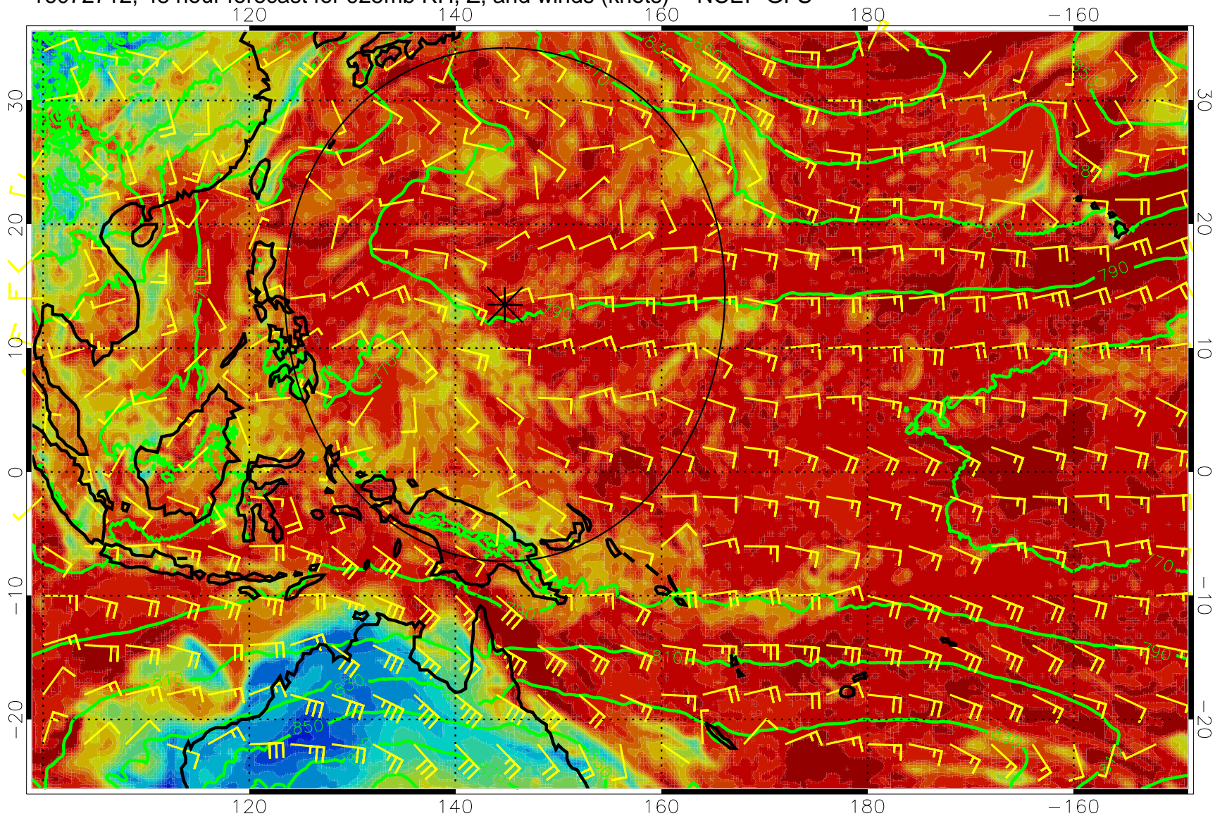
16072712, 48 hour forecast for 925mb RH, Z, and winds (knots) -- NCEP GFS
