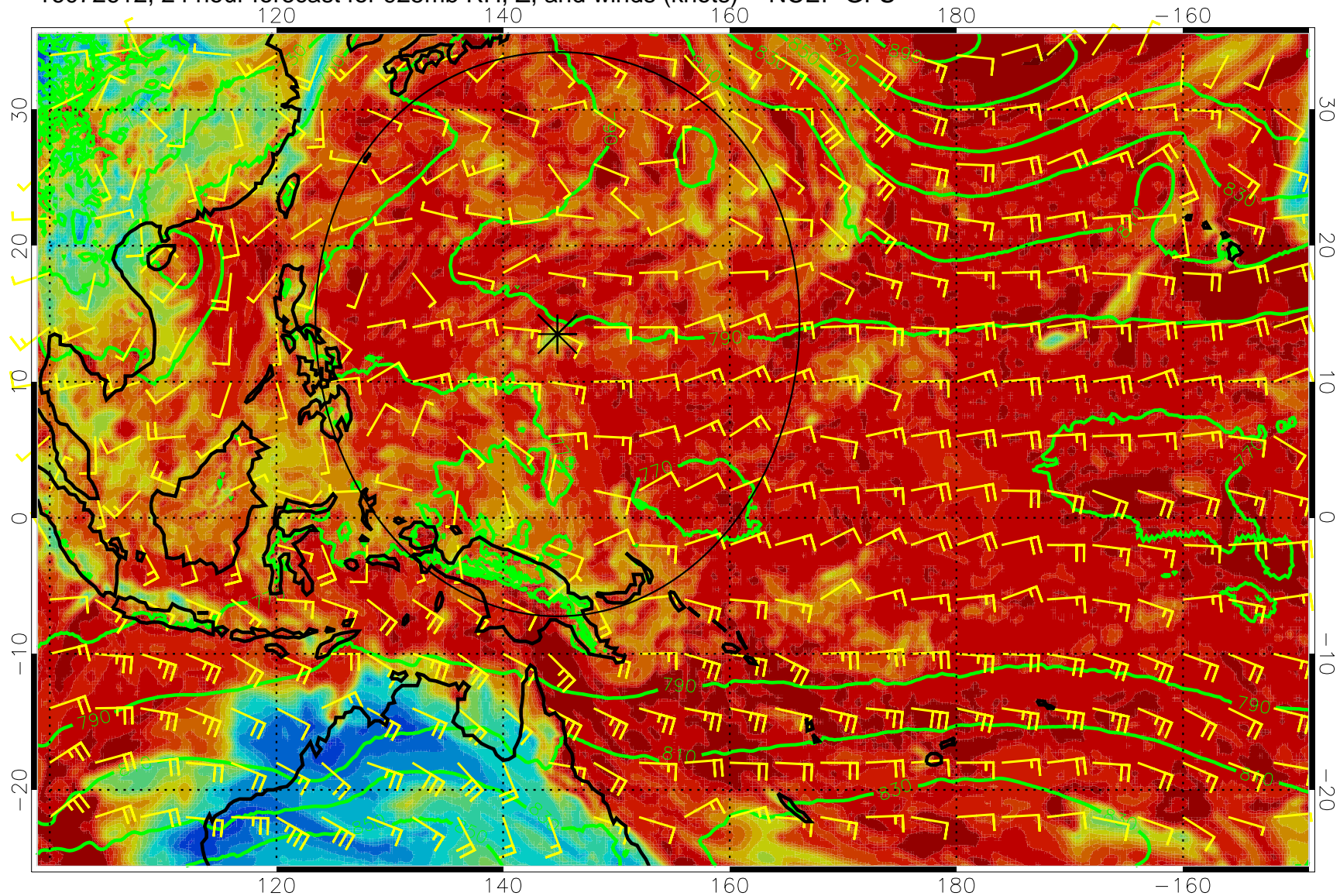
16072612, 24 hour forecast for 925mb RH, Z, and winds (knots) -- NCEP GFS
