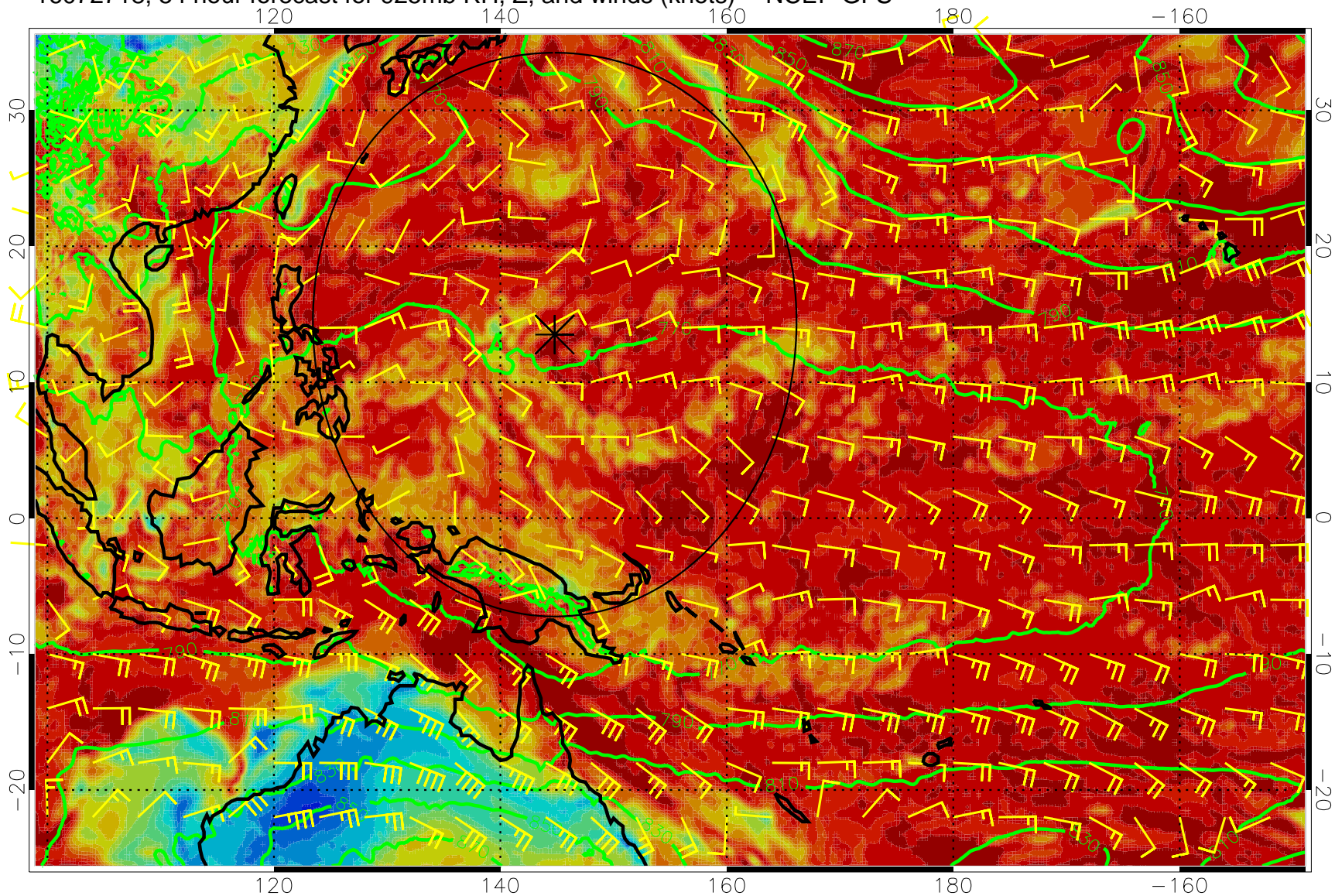
16072718, 54 hour forecast for 925mb RH, Z, and winds (knots) -- NCEP GFS
