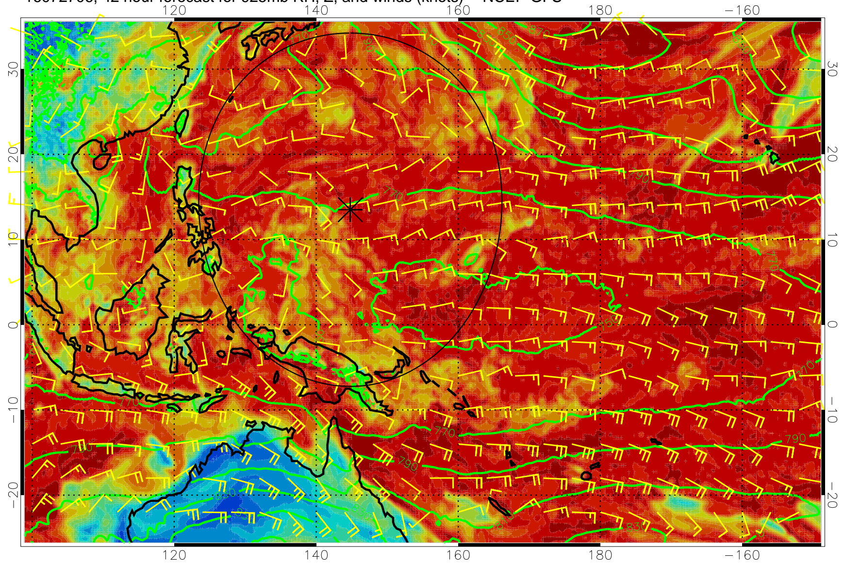
16072706, 42 hour forecast for 925mb RH, Z, and winds (knots) -- NCEP GFS
