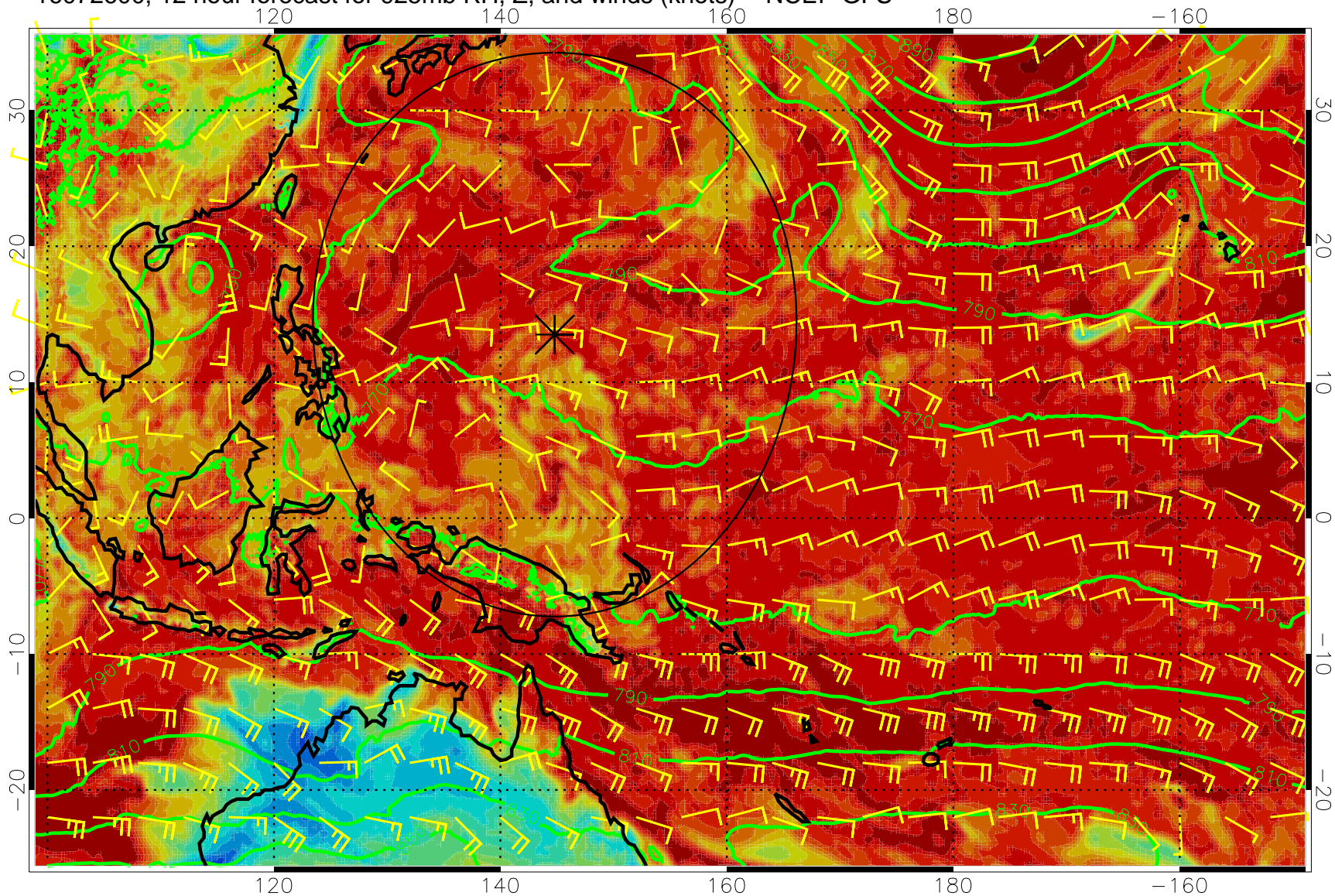
16072600, 12 hour forecast for 925mb RH, Z, and winds (knots) -- NCEP GFS
