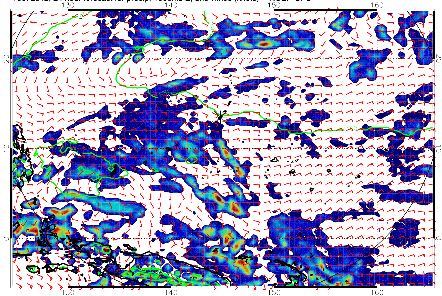
16072612, 24 hour forecast for precip, 1000mb Z, and winds (knots) -- NCEP GFS
