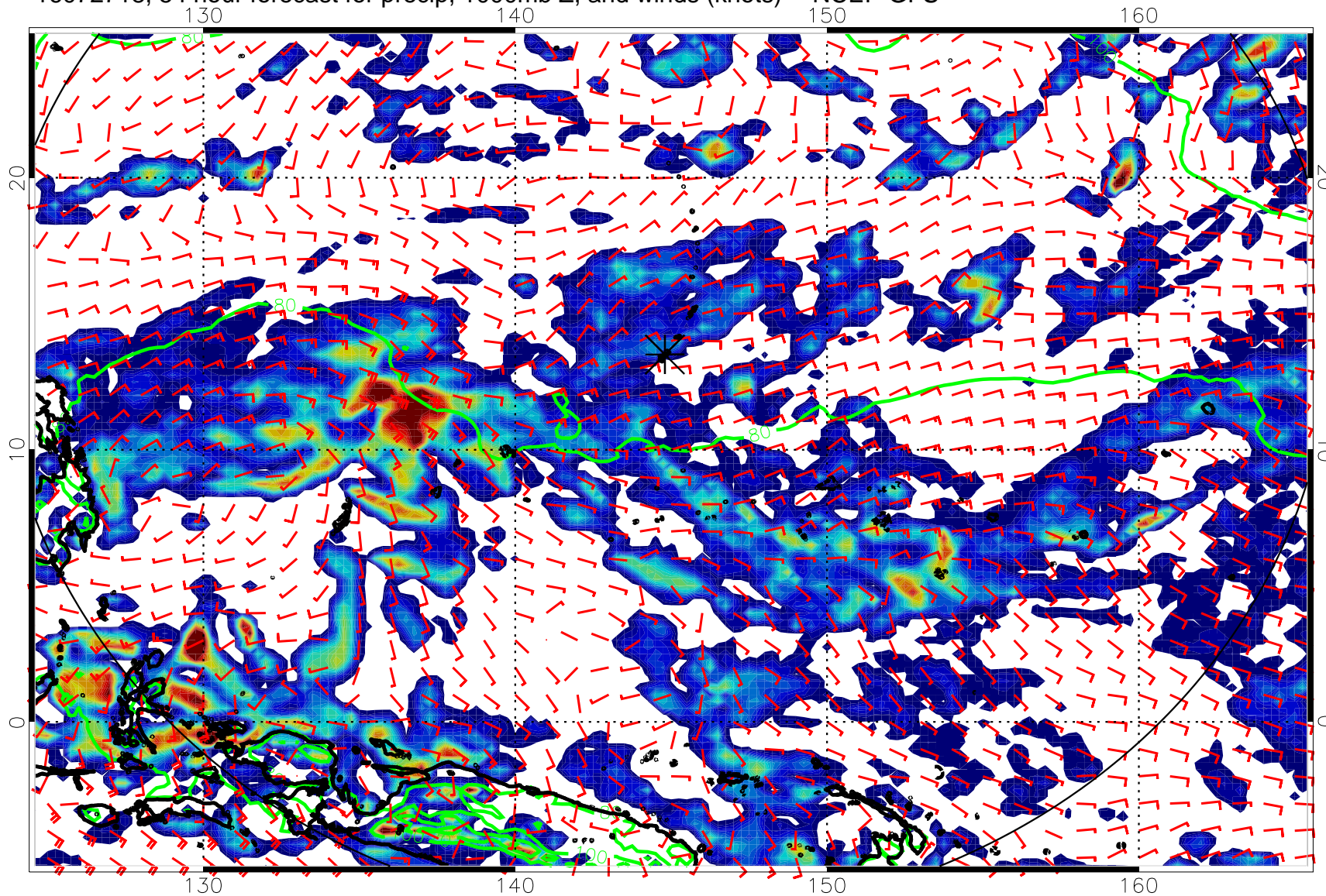
16072718, 54 hour forecast for precip, 1000mb Z, and winds (knots) -- NCEP GFS
