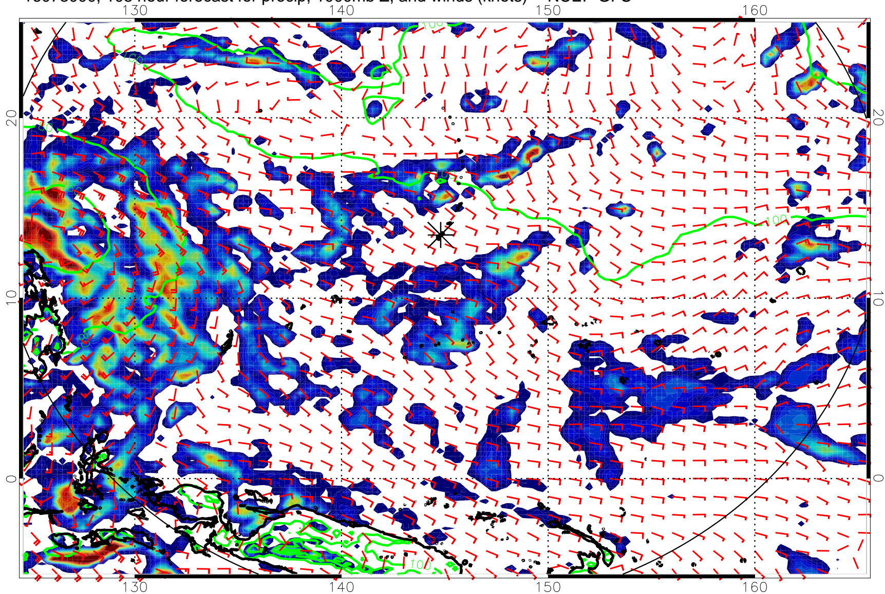
16073000, 108 hour forecast for precip, 1000mb Z, and winds (knots) -- NCEP GFS
