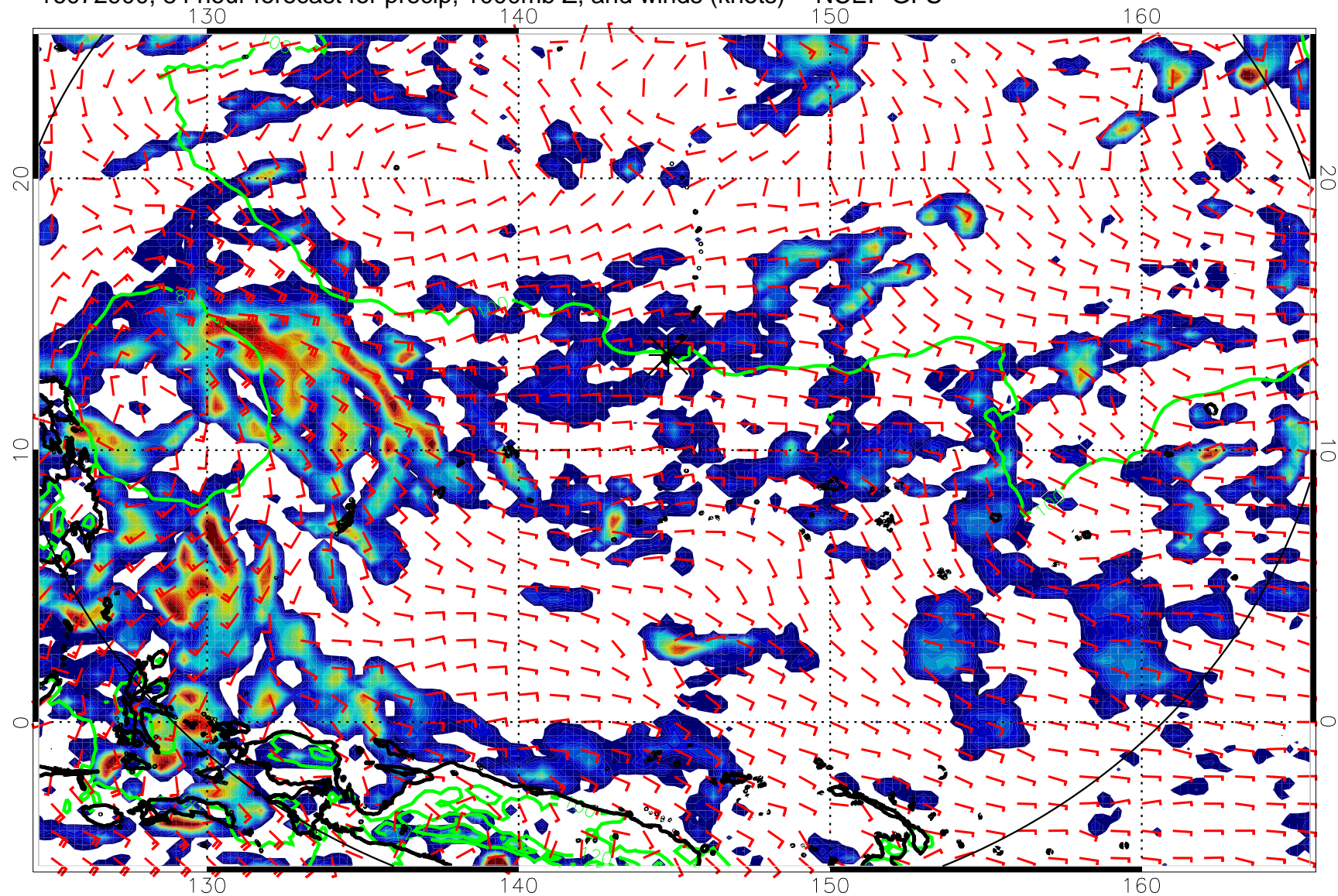
16072900, 84 hour forecast for precip, 1000mb Z, and winds (knots) -- NCEP GFS
