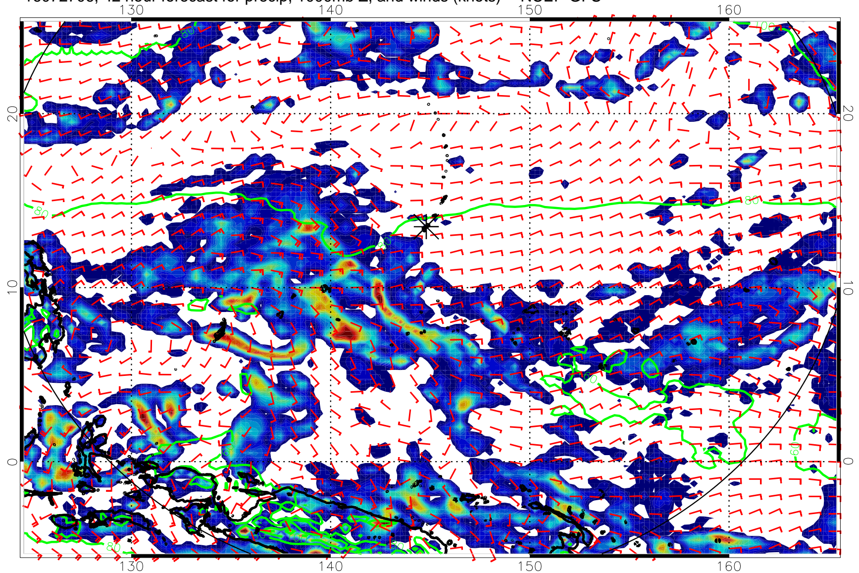
16072706, 42 hour forecast for precip, 1000mb Z, and winds (knots) -- NCEP GFS
