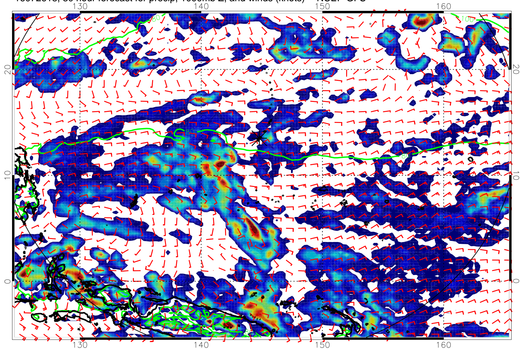
16072618, 30 hour forecast for precip, 1000mb Z, and winds (knots) -- NCEP GFS
