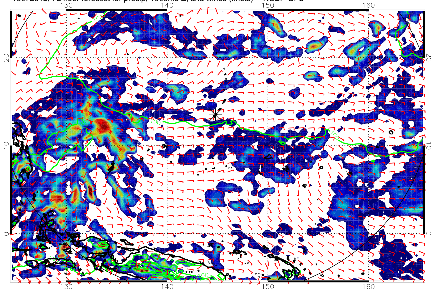
16072812, 72 hour forecast for precip, 1000mb Z, and winds (knots) -- NCEP GFS
