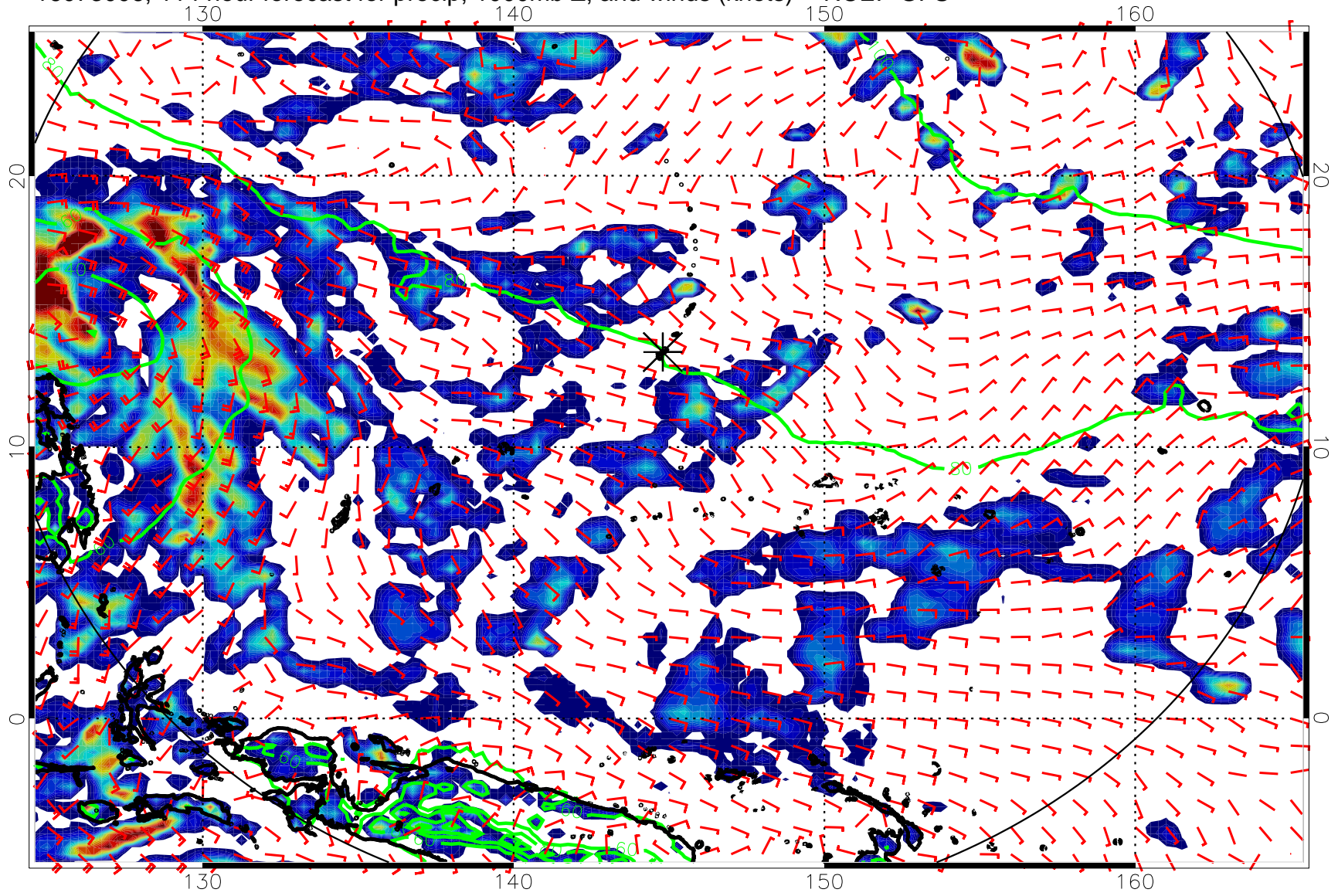
16073006, 114 hour forecast for precip, 1000mb Z, and winds (knots) -- NCEP GFS
