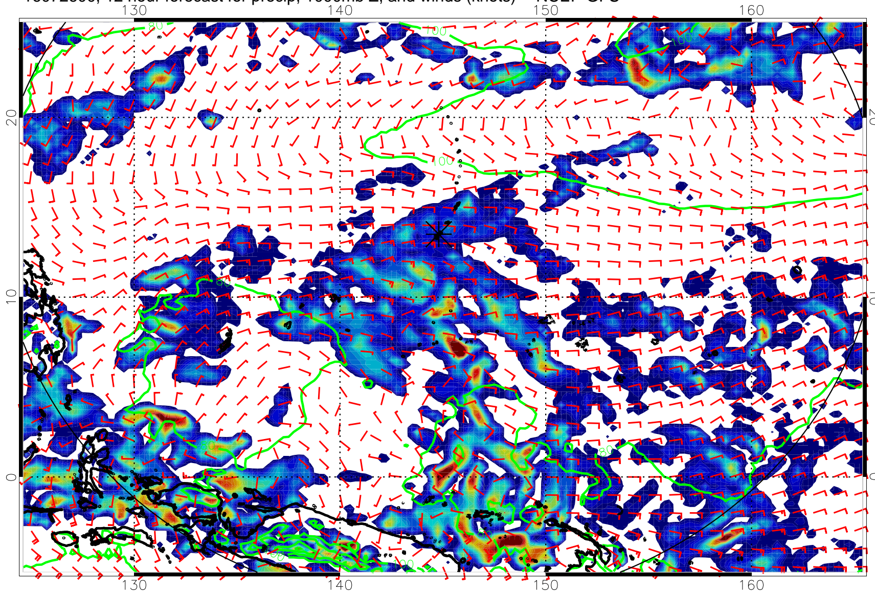
16072600, 12 hour forecast for precip, 1000mb Z, and winds (knots) -- NCEP GFS
