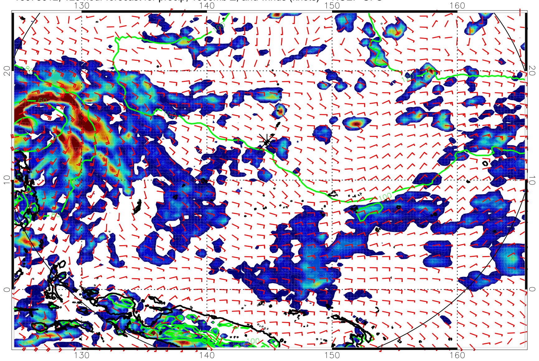
16073012, 120 hour forecast for precip, 1000mb Z, and winds (knots) -- NCEP GFS
