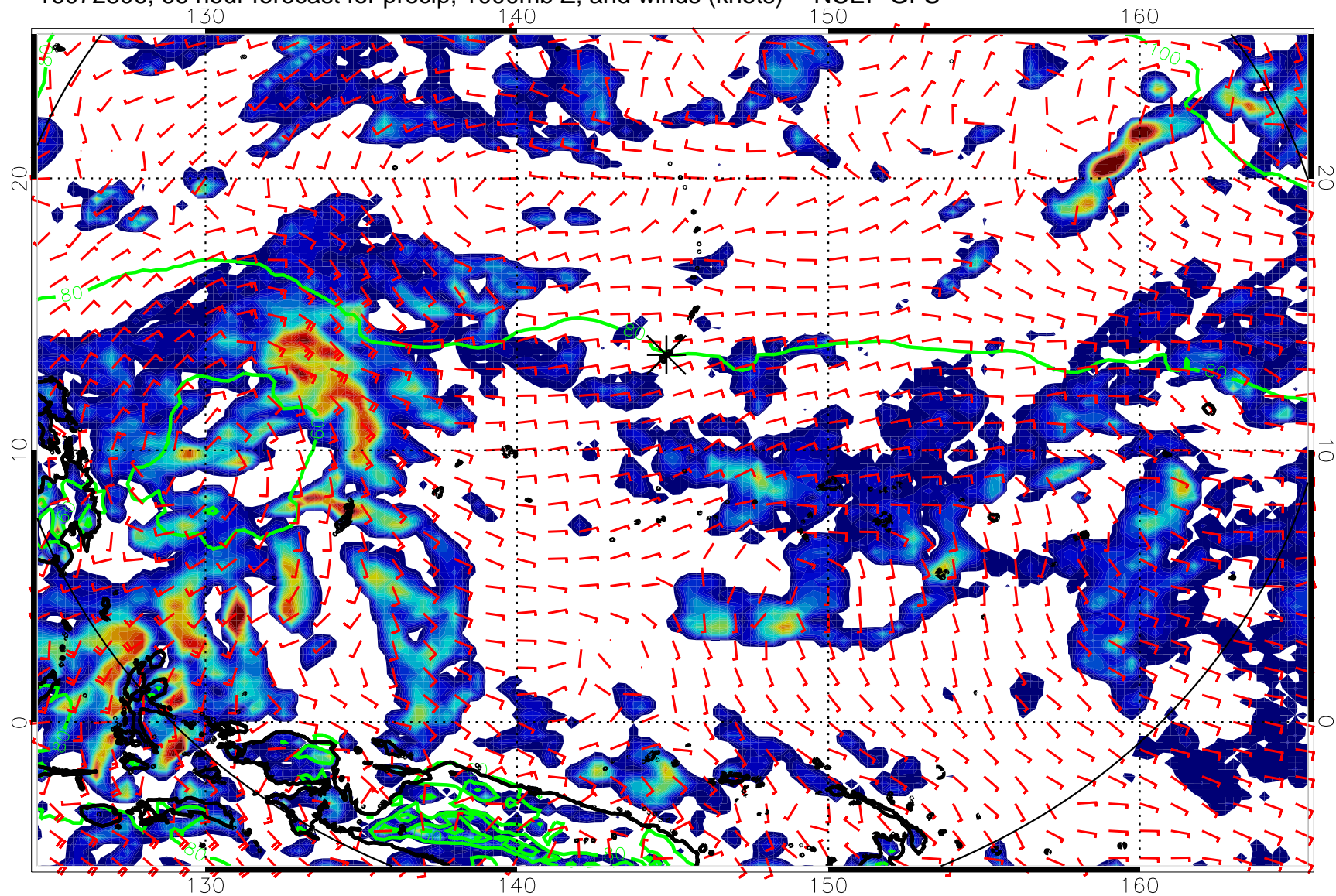
16072806, 66 hour forecast for precip, 1000mb Z, and winds (knots) -- NCEP GFS
