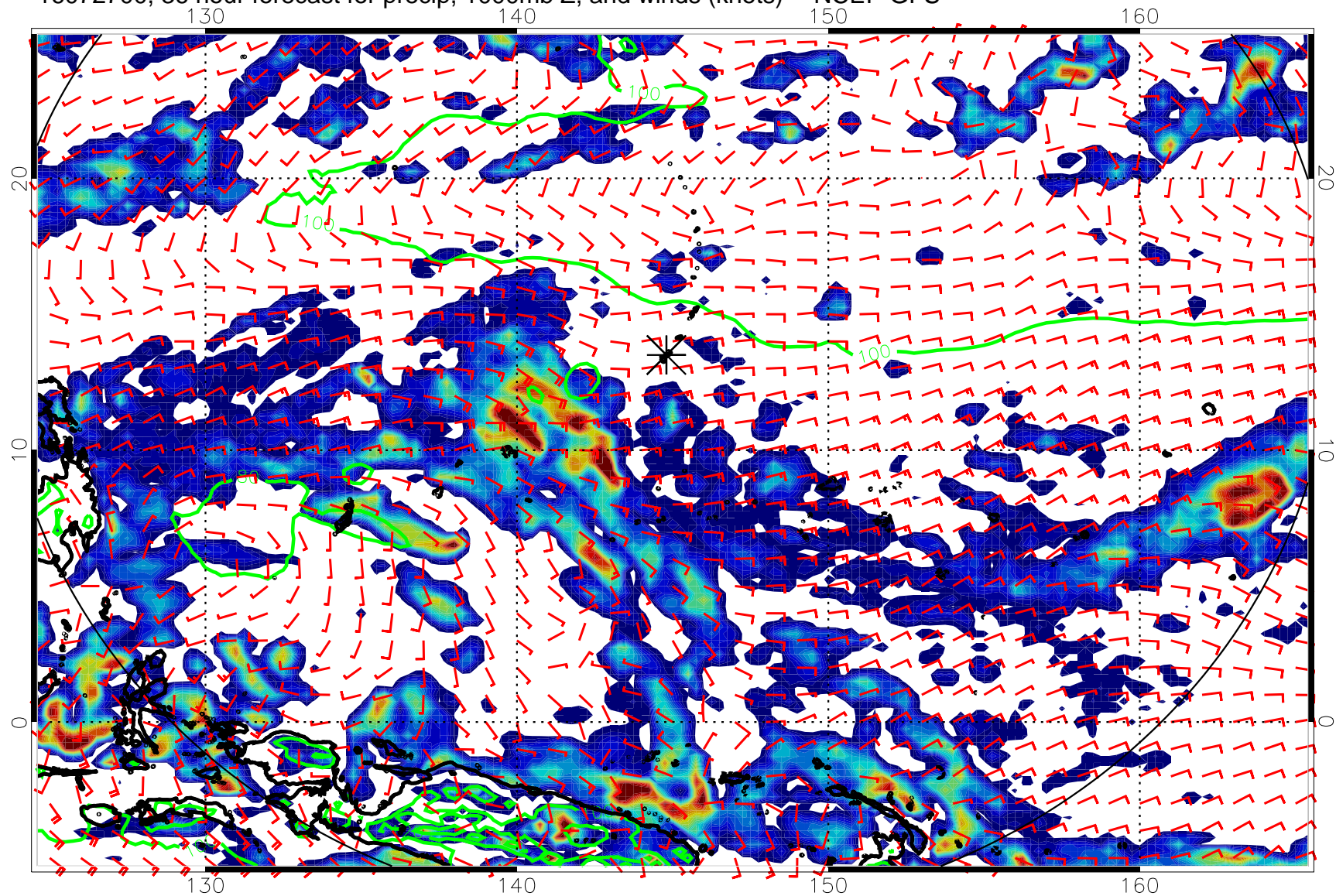
16072700, 36 hour forecast for precip, 1000mb Z, and winds (knots) -- NCEP GFS
