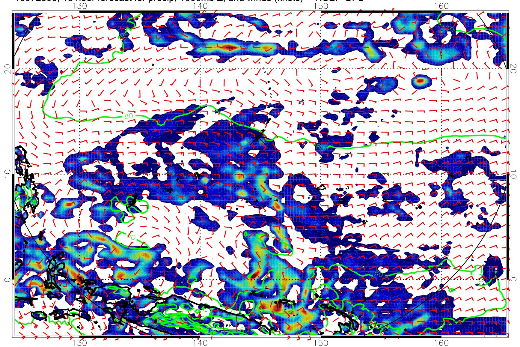
16072606, 18 hour forecast for precip, 1000mb Z, and winds (knots) -- NCEP GFS
