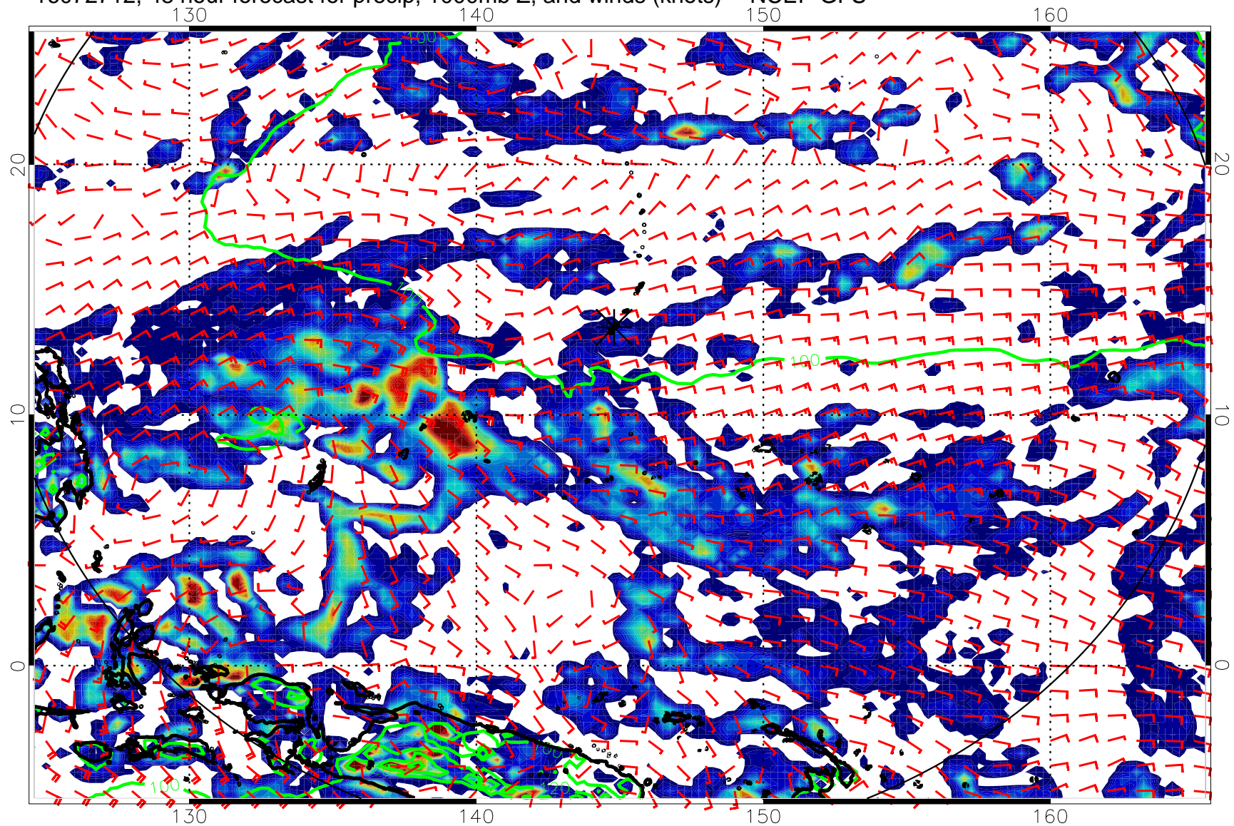
16072712, 48 hour forecast for precip, 1000mb Z, and winds (knots) -- NCEP GFS
