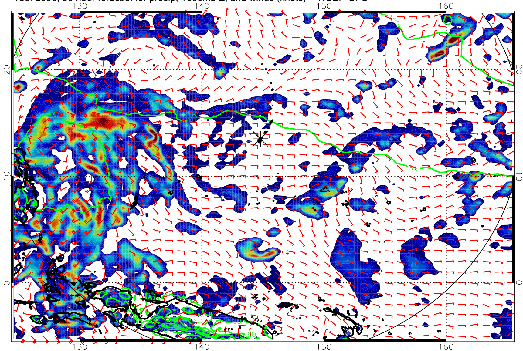
16072906, 90 hour forecast for precip, 1000mb Z, and winds (knots) -- NCEP GFS
