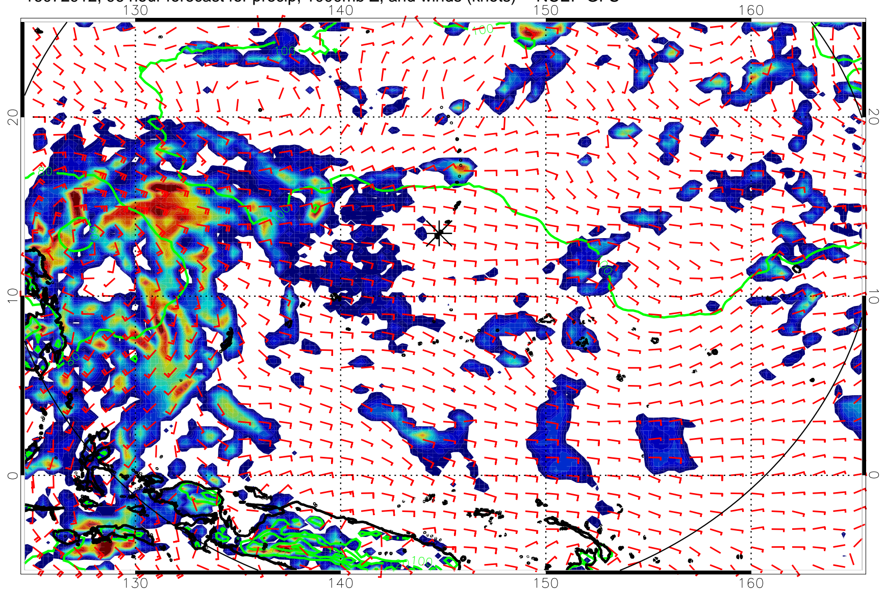
16072912, 96 hour forecast for precip, 1000mb Z, and winds (knots) -- NCEP GFS
