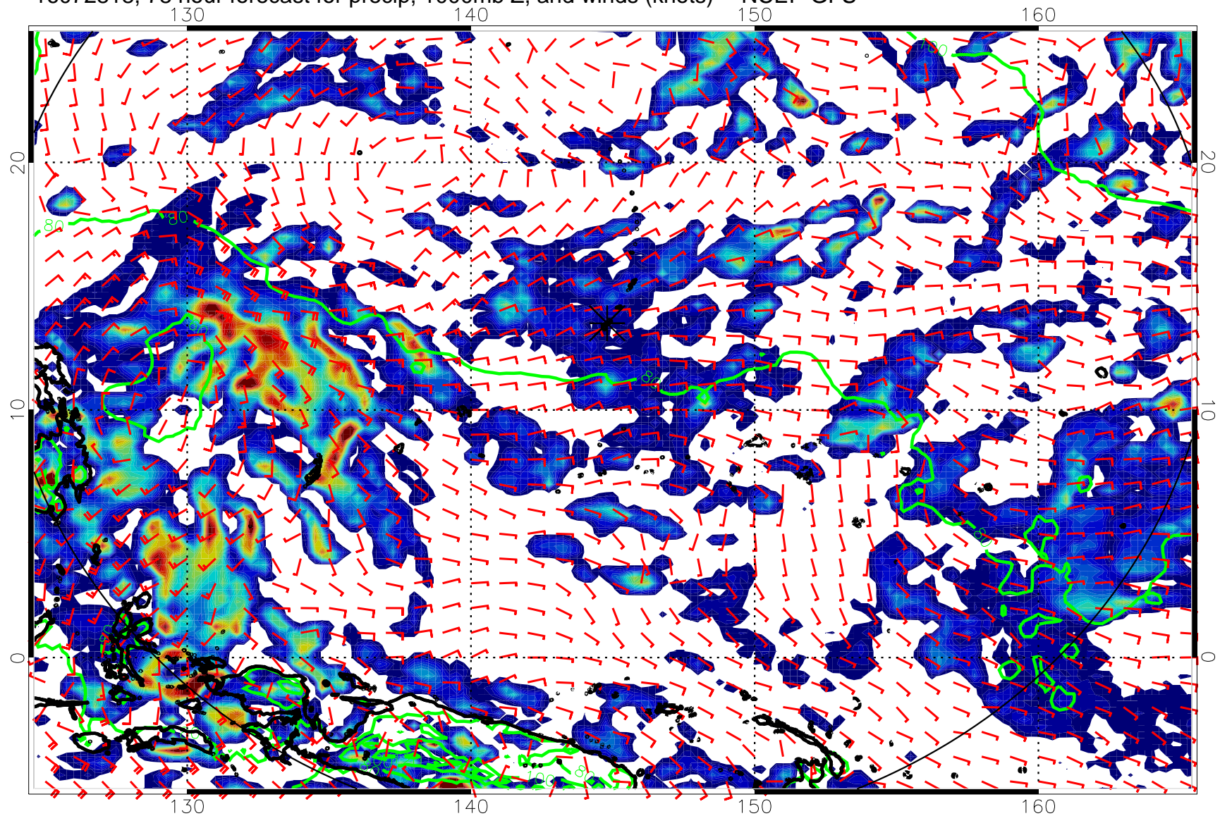
16072818, 78 hour forecast for precip, 1000mb Z, and winds (knots) -- NCEP GFS
