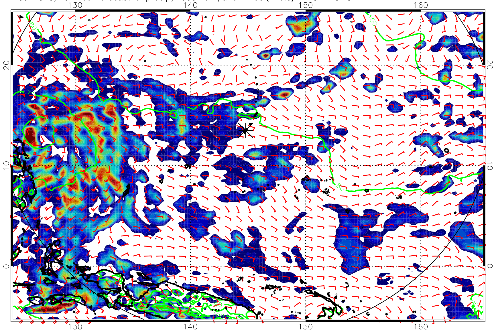
16072918, 102 hour forecast for precip, 1000mb Z, and winds (knots) -- NCEP GFS
