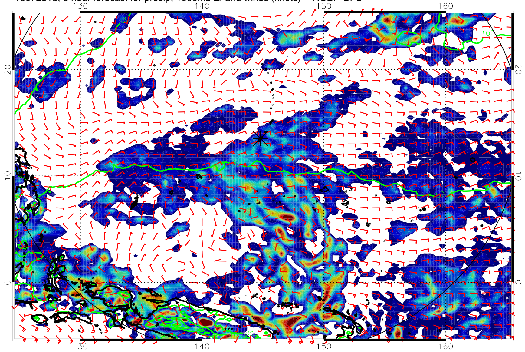
16072518, 6 hour forecast for precip, 1000mb Z, and winds (knots) -- NCEP GFS
