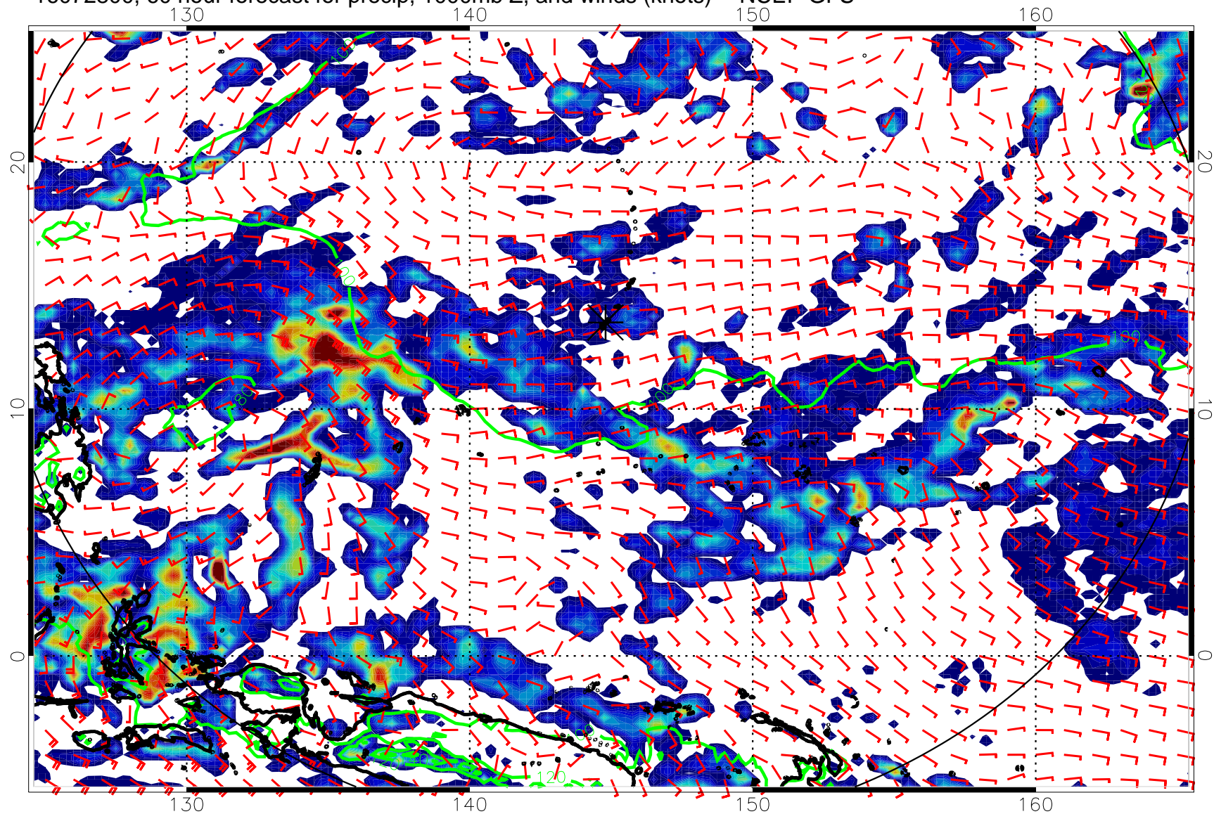
16072800, 60 hour forecast for precip, 1000mb Z, and winds (knots) -- NCEP GFS
