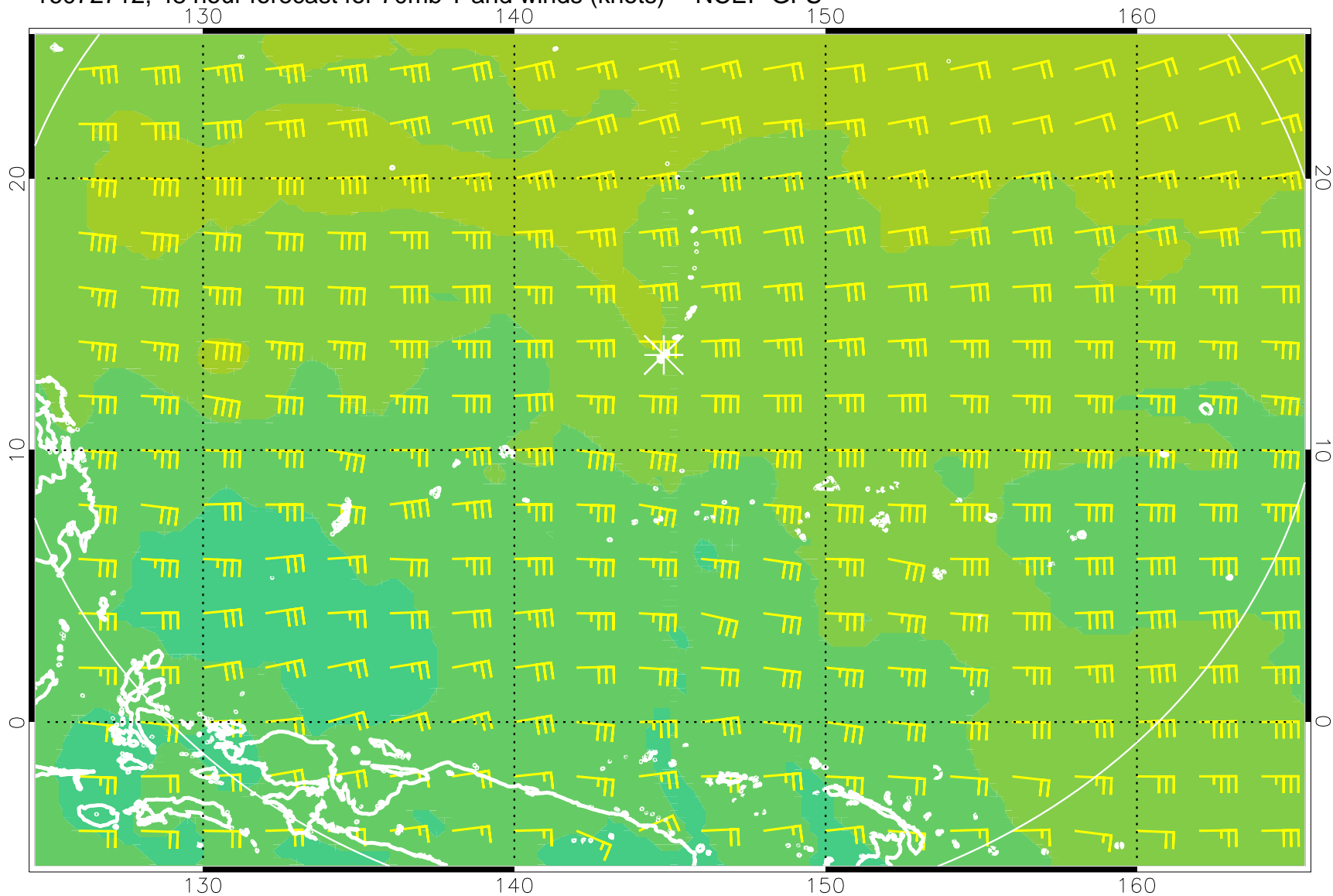
16072712, 48 hour forecast for 70mb T and winds (knots) -- NCEP GFS
