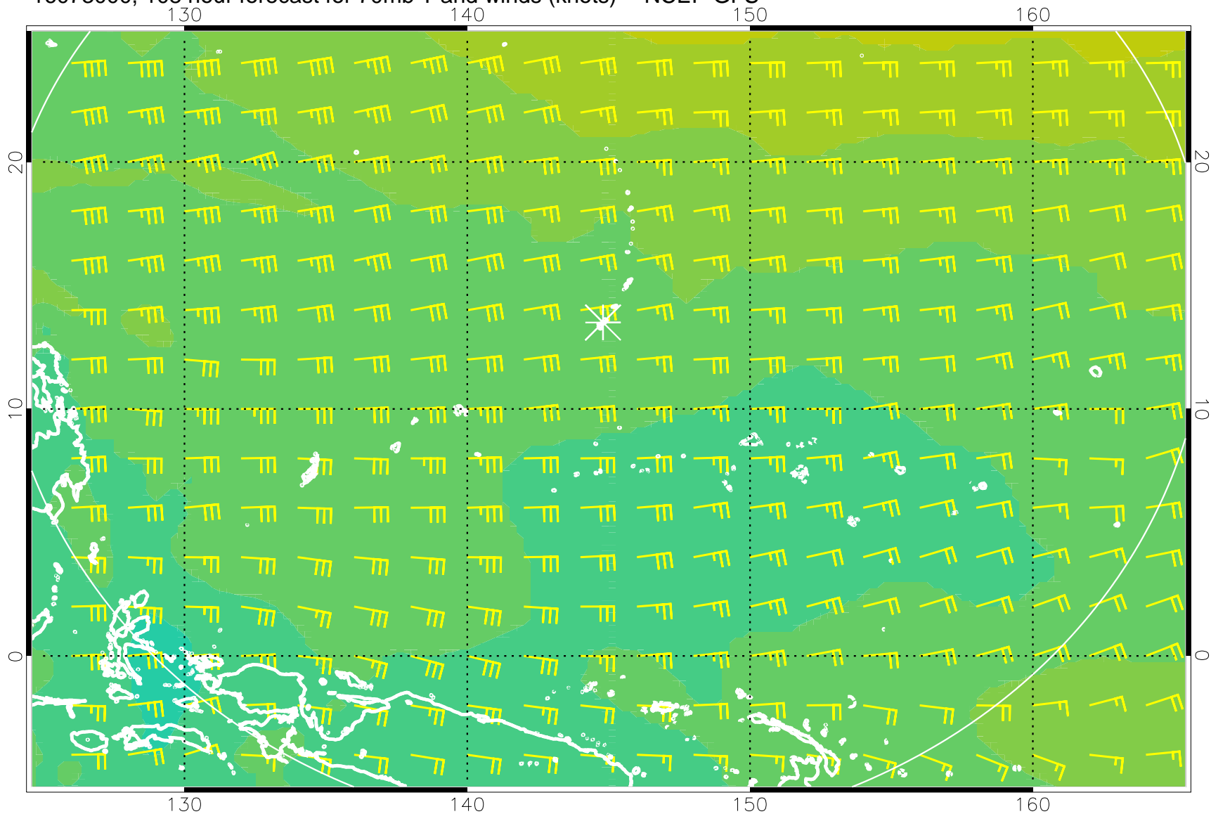
16073000, 108 hour forecast for 70mb T and winds (knots) -- NCEP GFS
