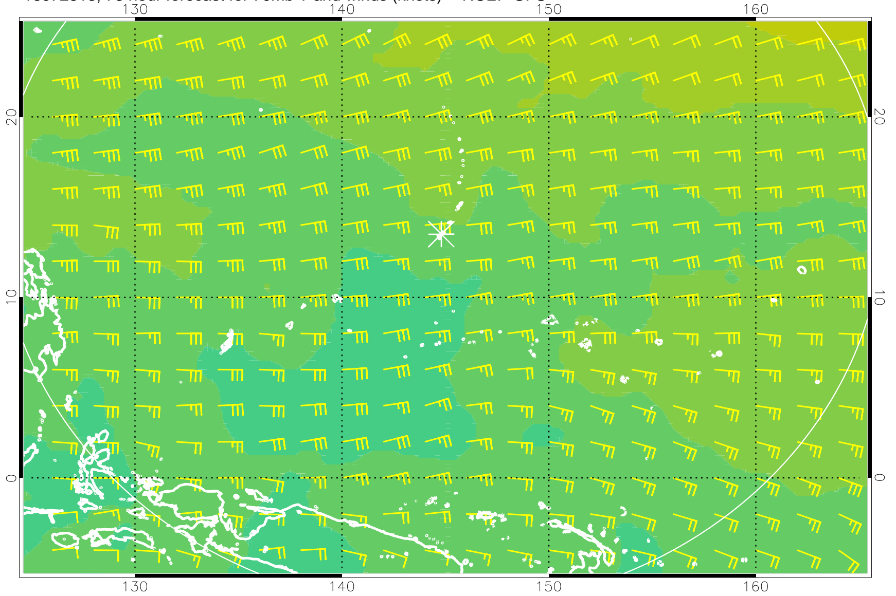
16072818, 78 hour forecast for 70mb T and winds (knots) -- NCEP GFS
