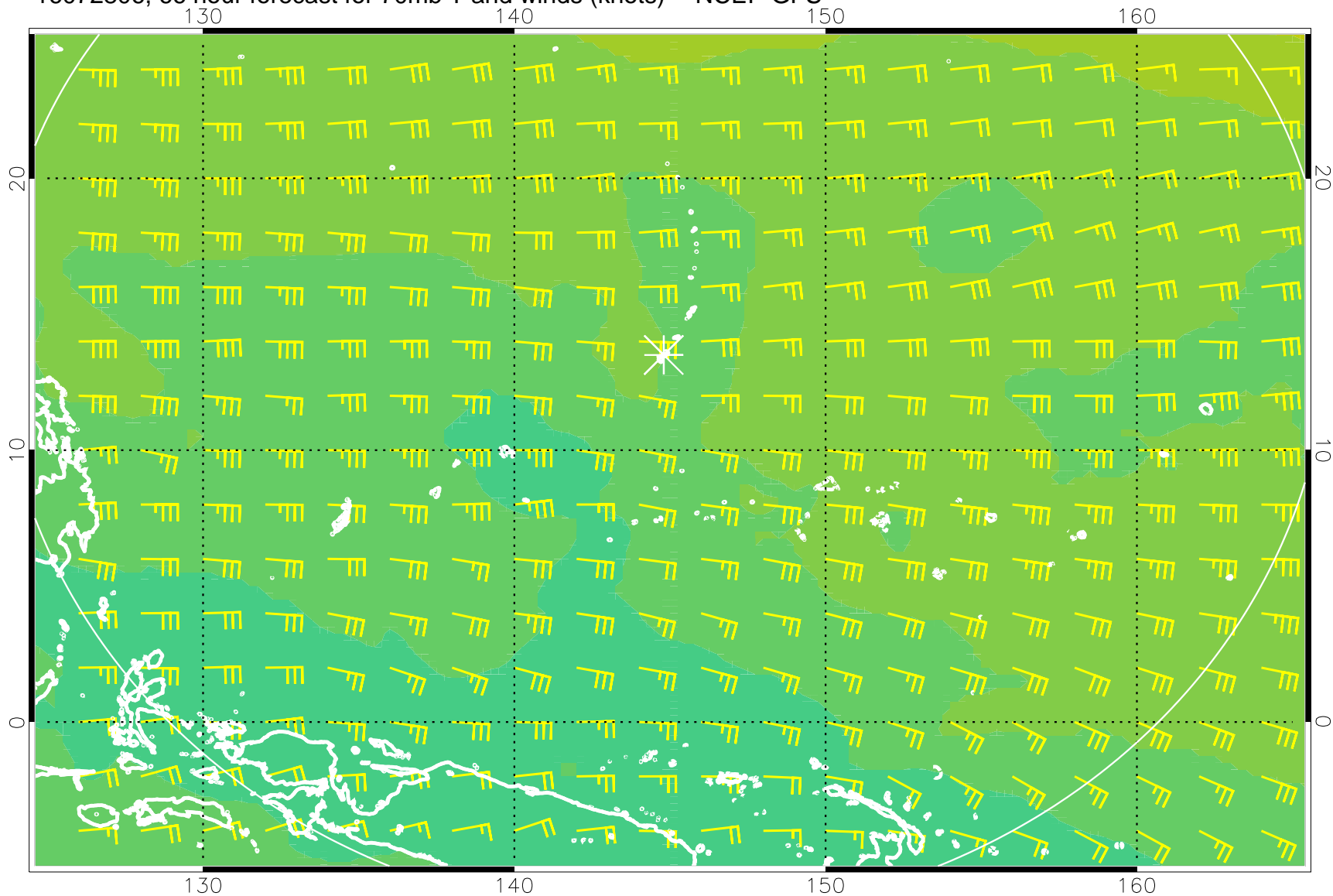
16072806, 66 hour forecast for 70mb T and winds (knots) -- NCEP GFS
