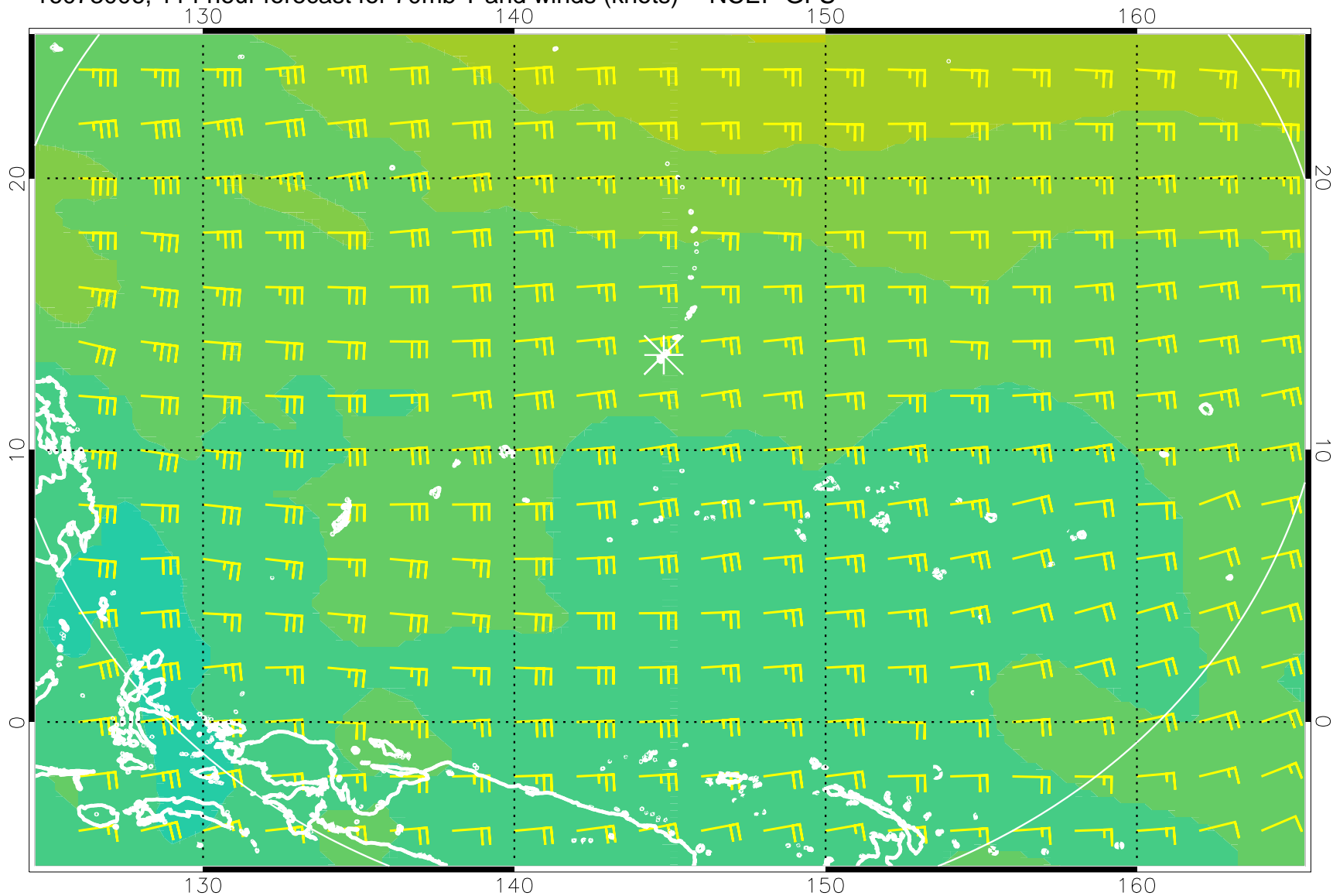
16073006, 114 hour forecast for 70mb T and winds (knots) -- NCEP GFS
