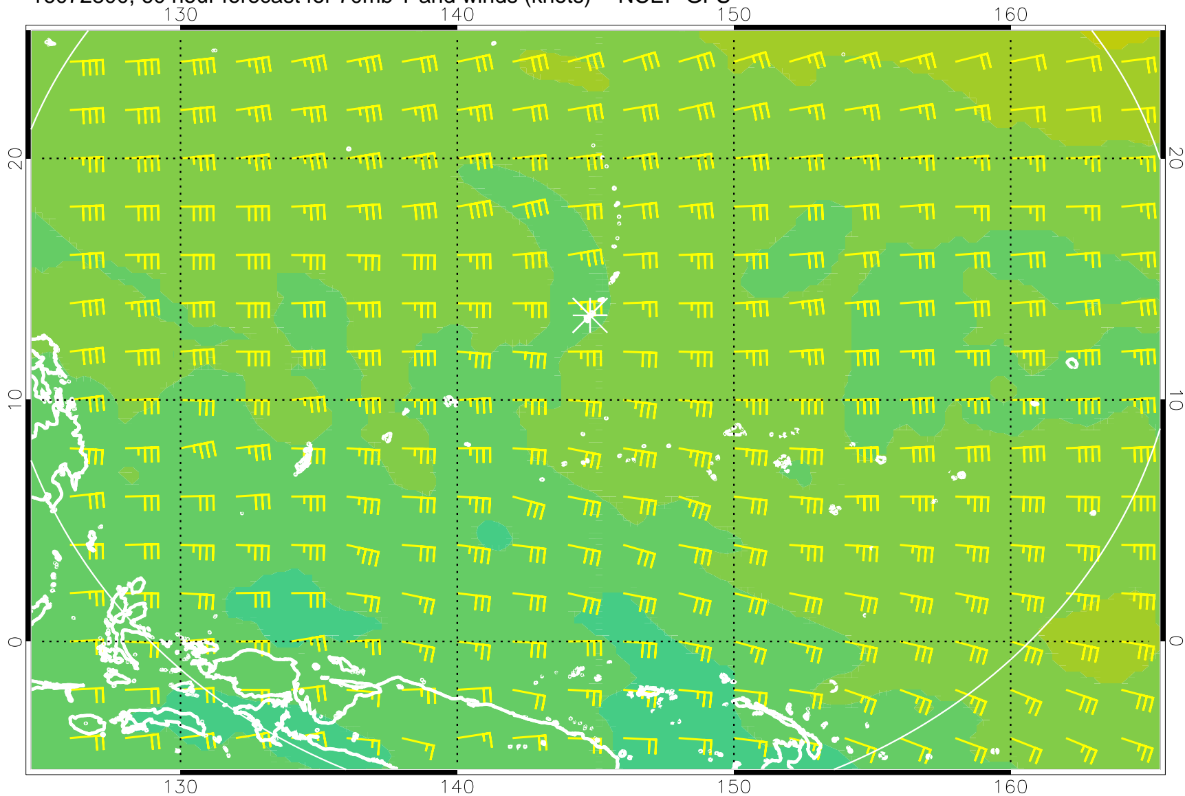
16072800, 60 hour forecast for 70mb T and winds (knots) -- NCEP GFS
