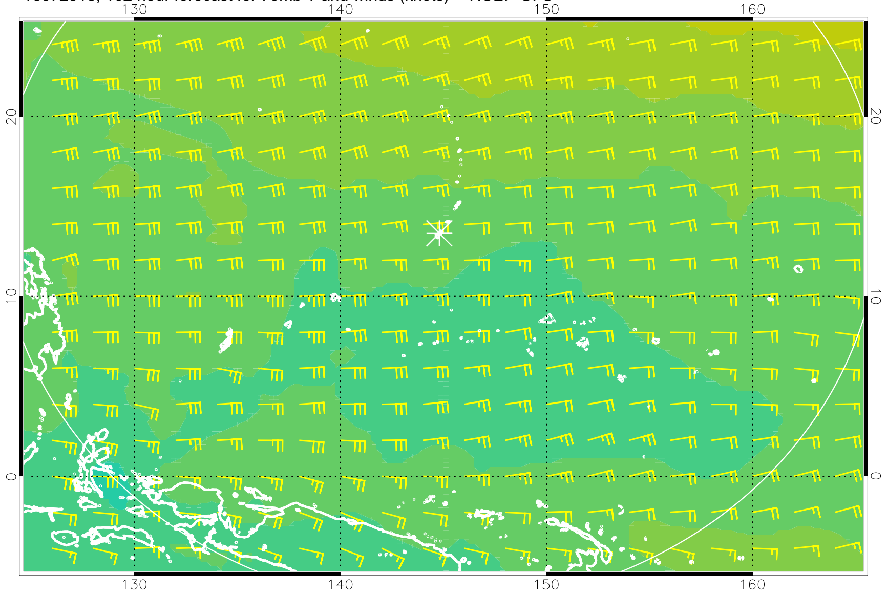
16072918, 102 hour forecast for 70mb T and winds (knots) -- NCEP GFS
