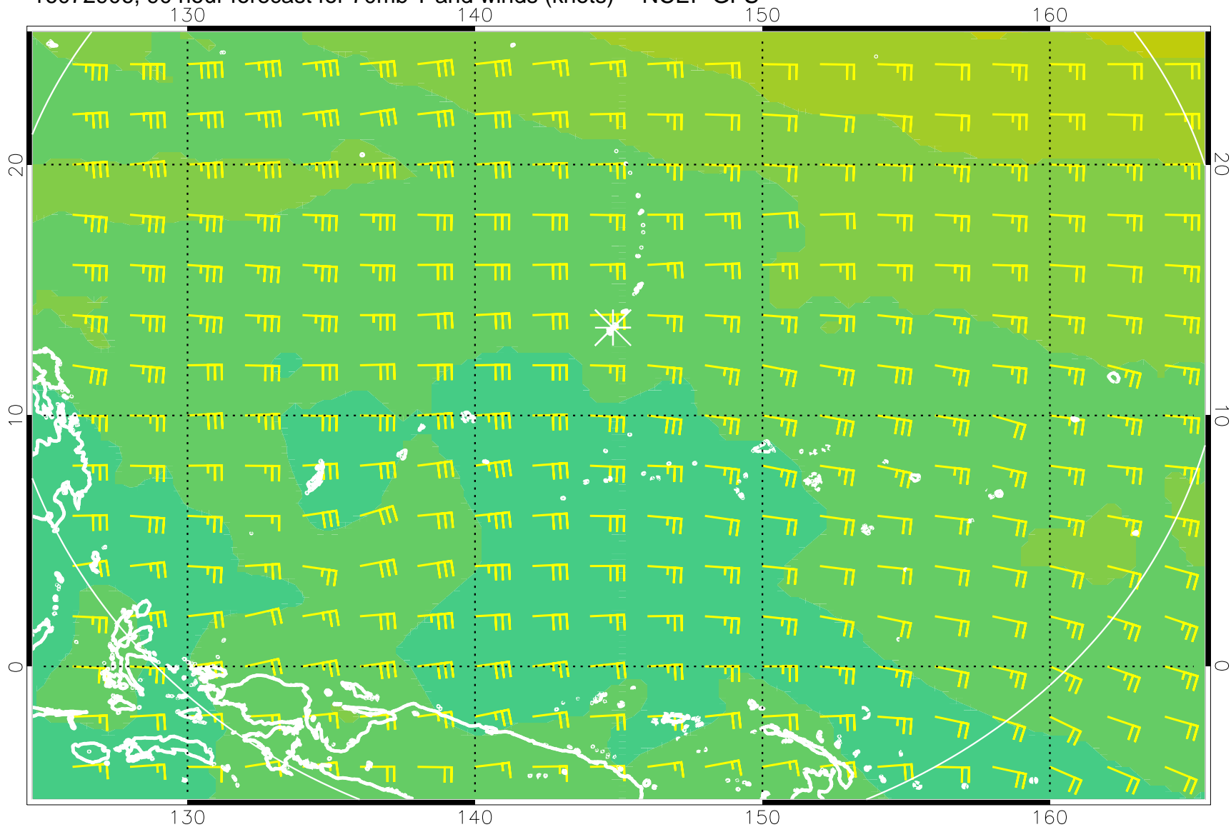
16072906, 90 hour forecast for 70mb T and winds (knots) -- NCEP GFS
