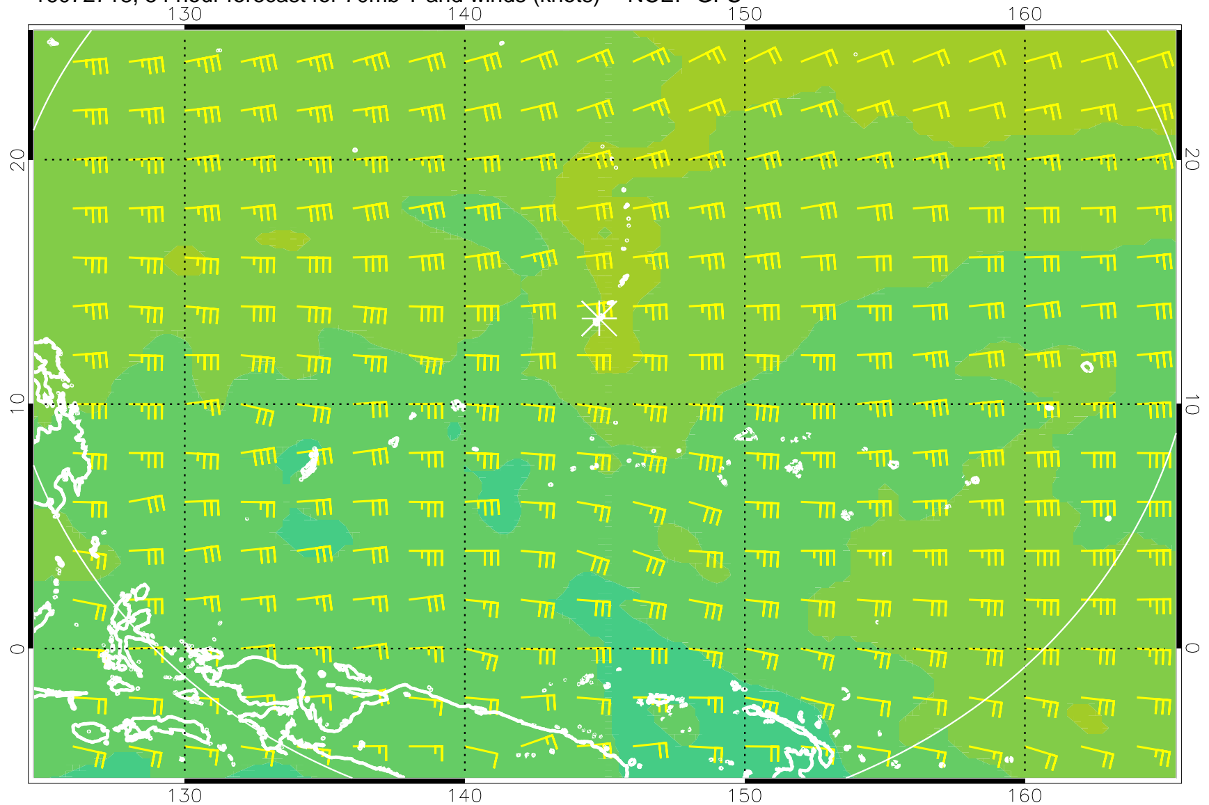
16072718, 54 hour forecast for 70mb T and winds (knots) -- NCEP GFS
