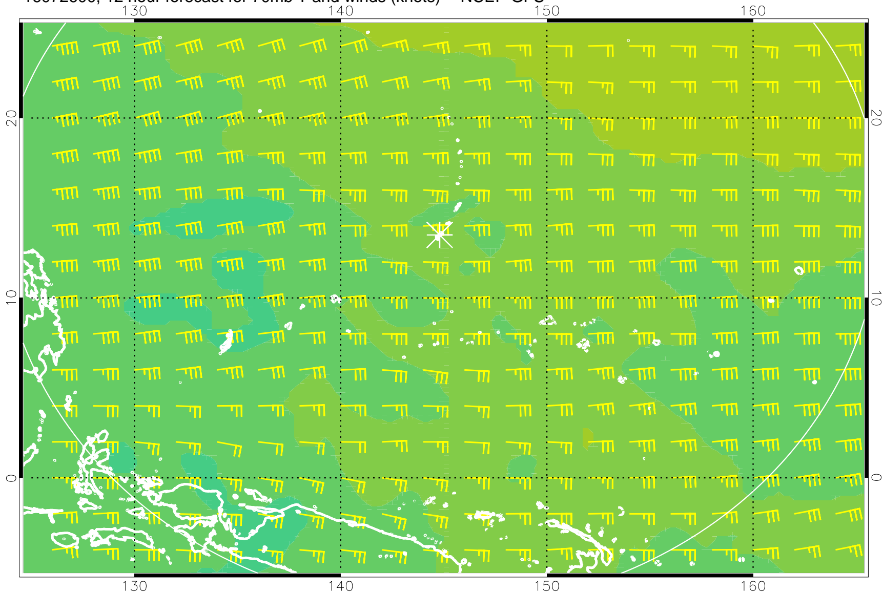
16072600, 12 hour forecast for 70mb T and winds (knots) -- NCEP GFS
