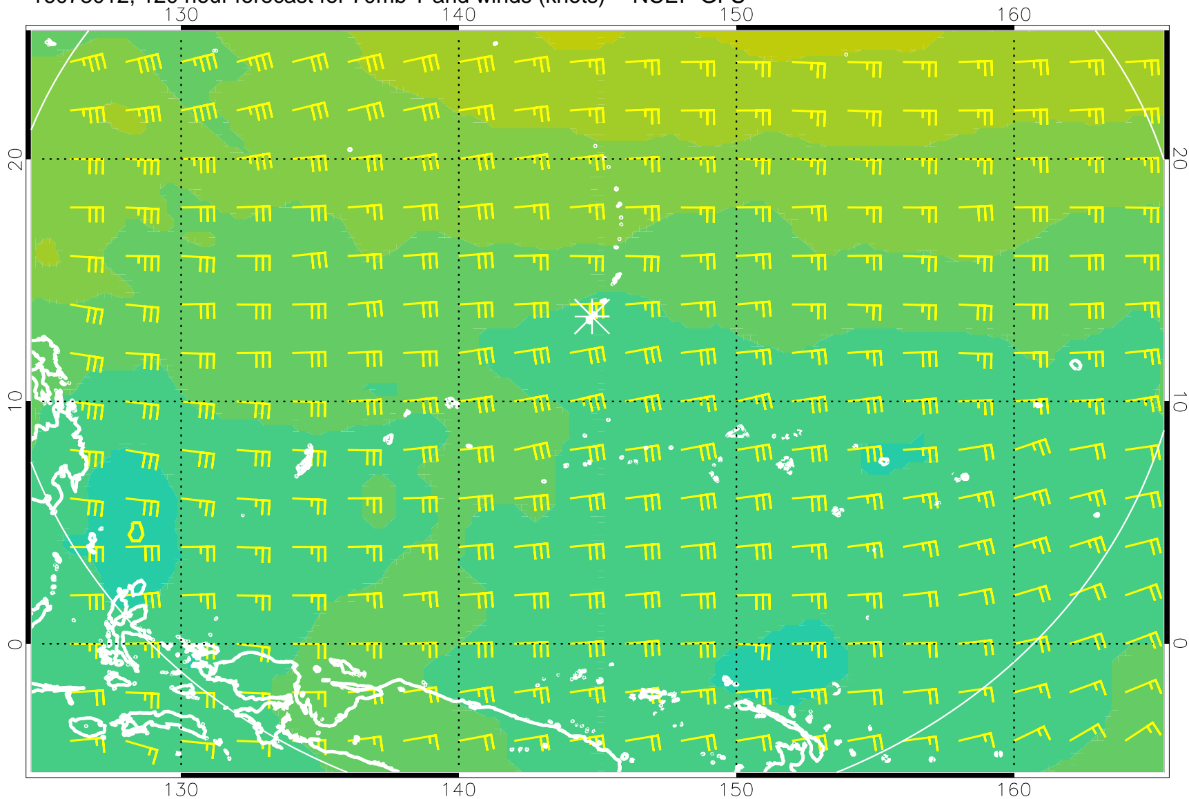
16073012, 120 hour forecast for 70mb T and winds (knots) -- NCEP GFS
