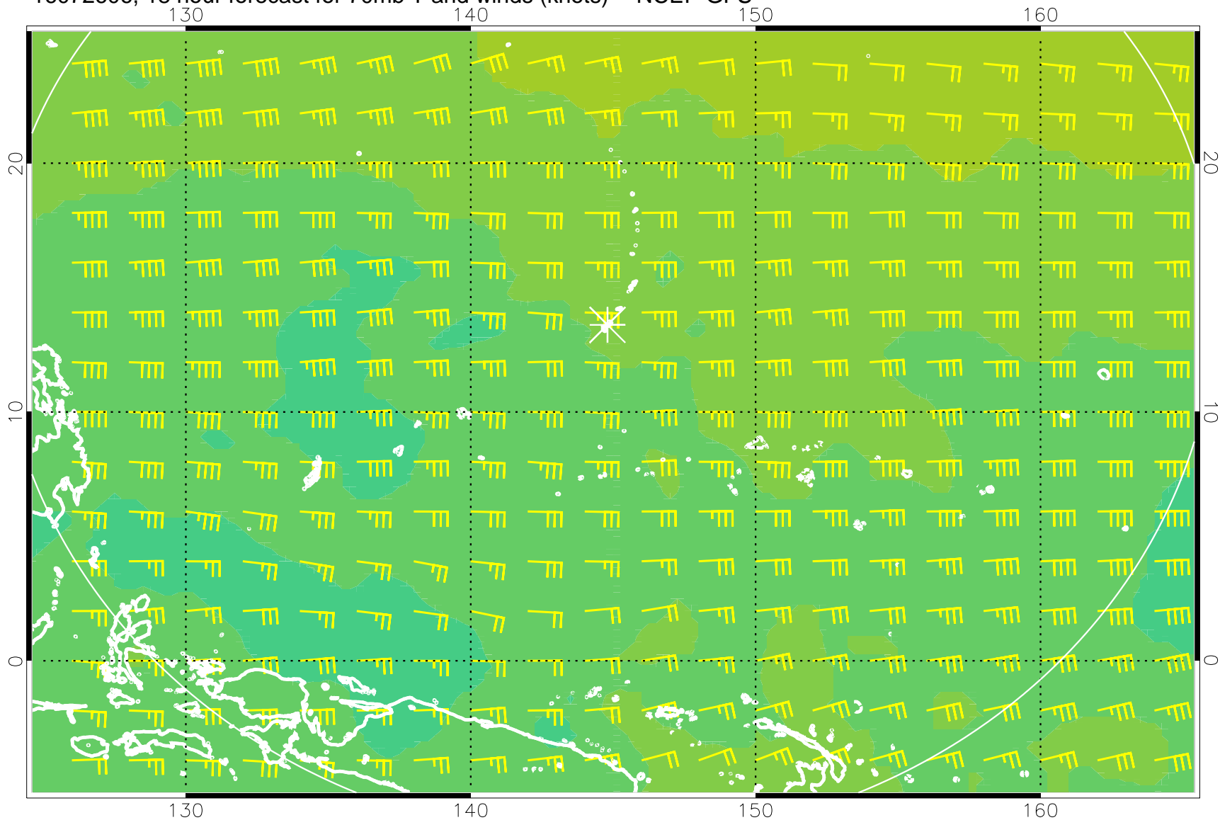
16072606, 18 hour forecast for 70mb T and winds (knots) -- NCEP GFS
