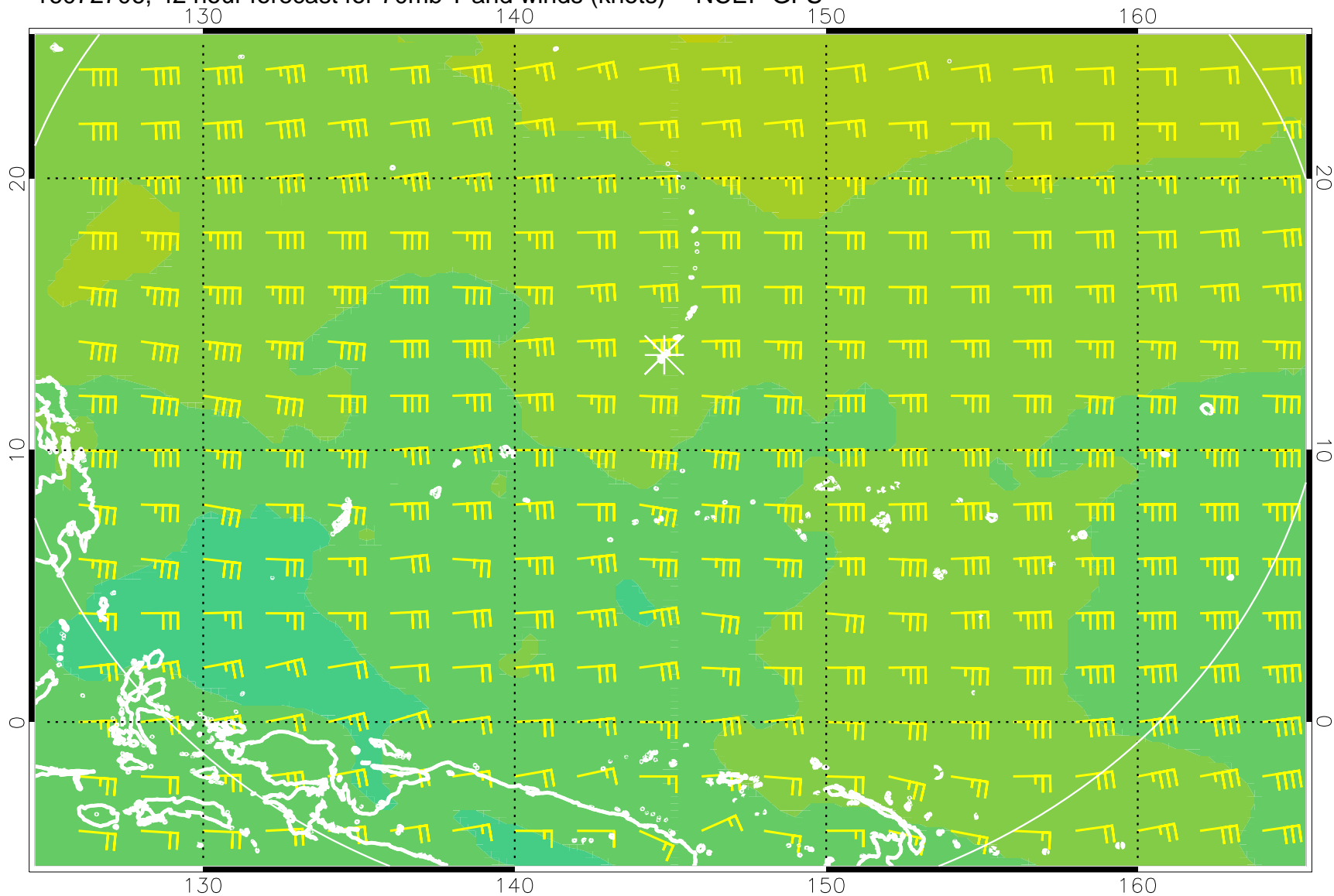
16072706, 42 hour forecast for 70mb T and winds (knots) -- NCEP GFS
