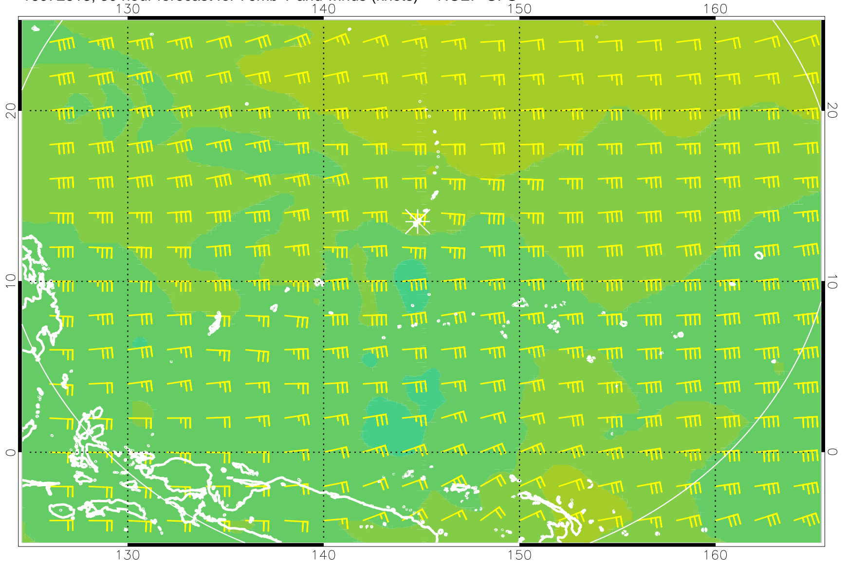
16072618, 30 hour forecast for 70mb T and winds (knots) -- NCEP GFS
