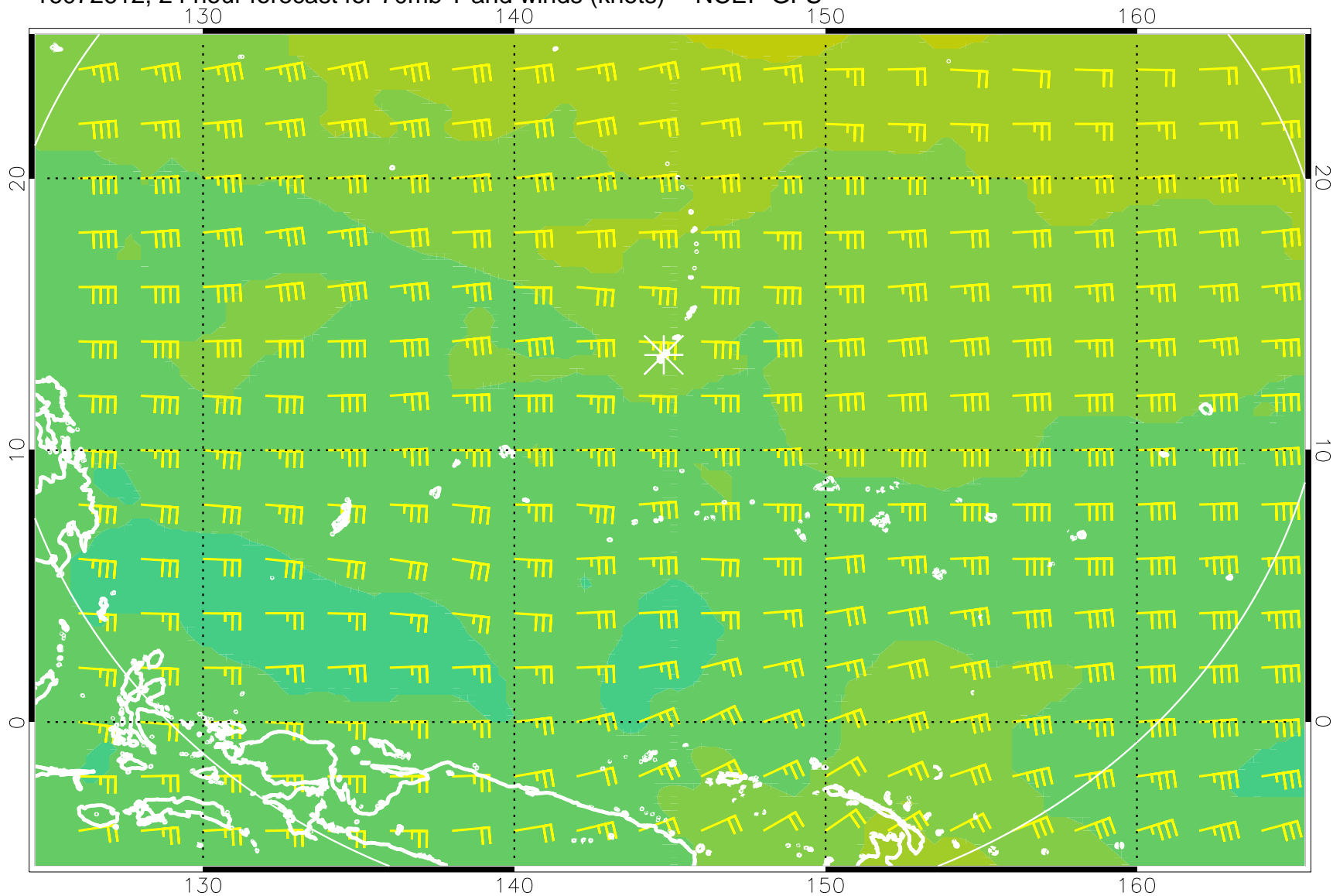
16072612, 24 hour forecast for 70mb T and winds (knots) -- NCEP GFS
