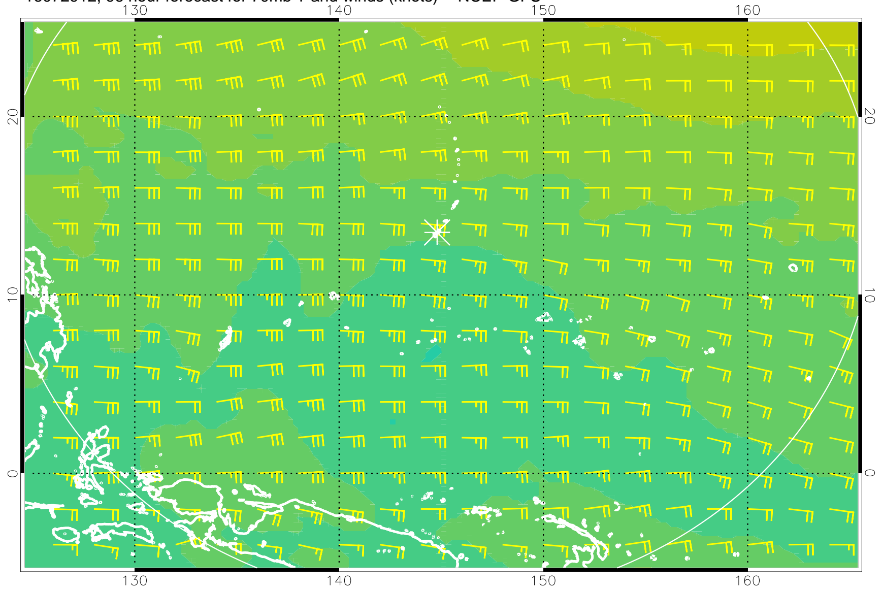
16072912, 96 hour forecast for 70mb T and winds (knots) -- NCEP GFS
