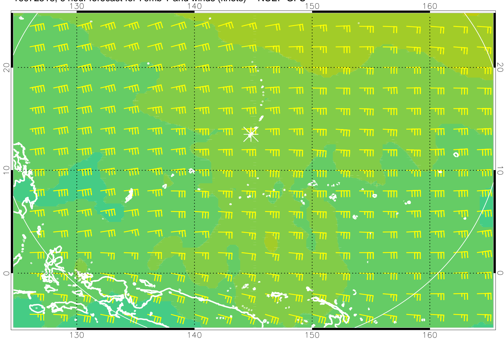
16072518, 6 hour forecast for 70mb T and winds (knots) -- NCEP GFS
