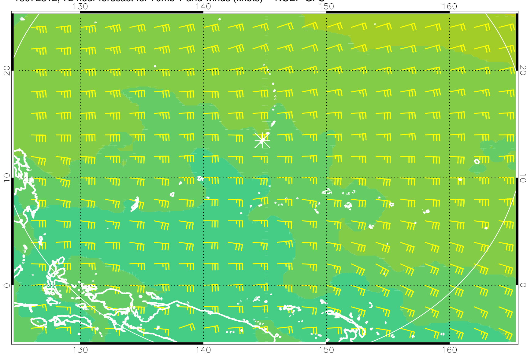
16072812, 72 hour forecast for 70mb T and winds (knots) -- NCEP GFS
