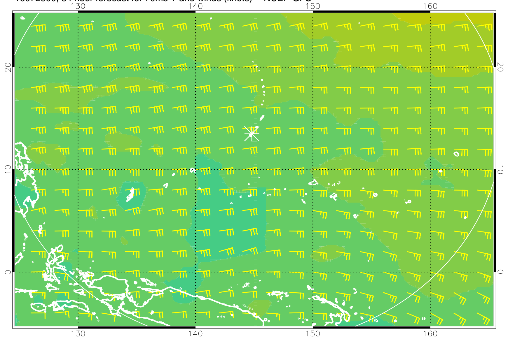
16072900, 84 hour forecast for 70mb T and winds (knots) -- NCEP GFS
