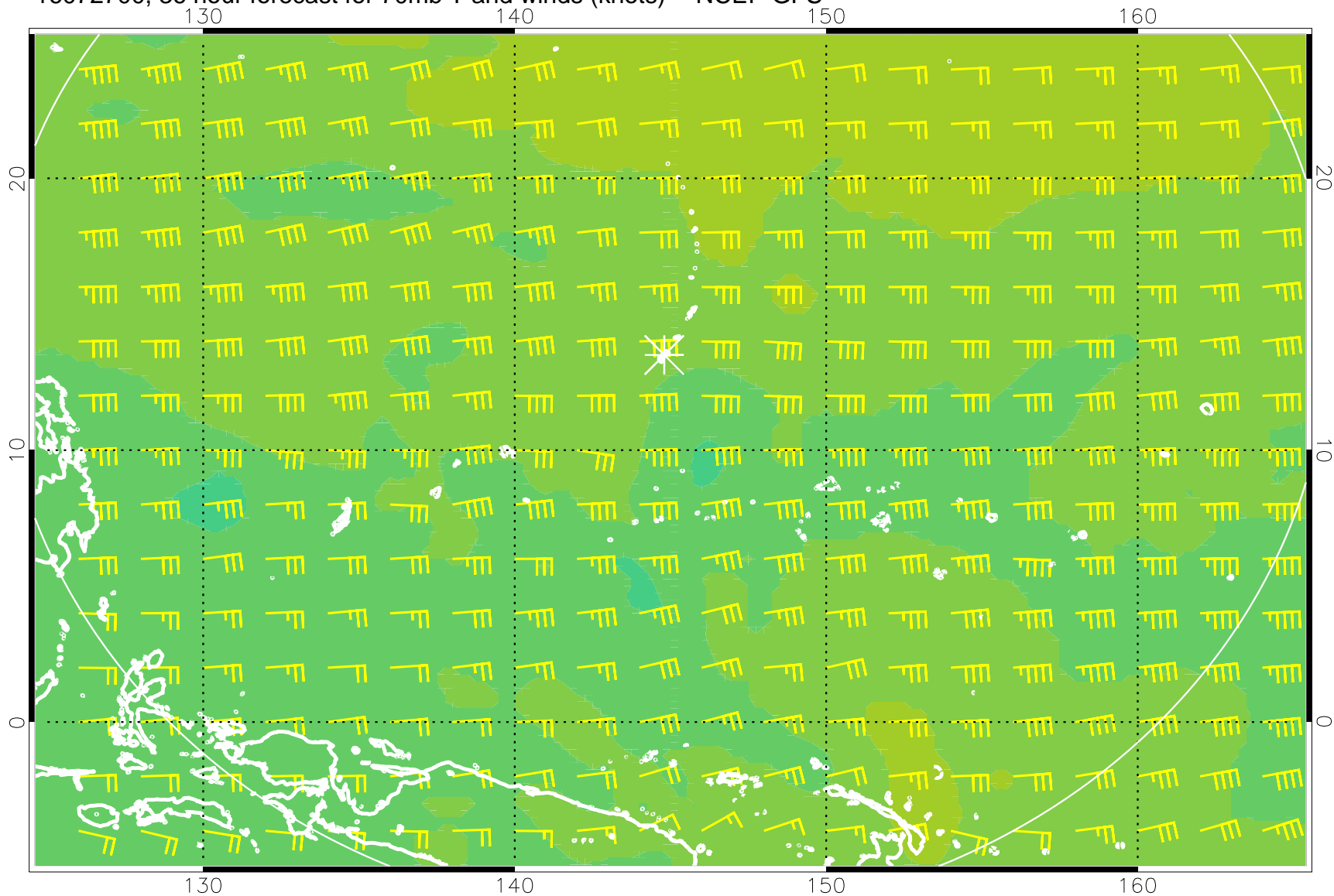
16072700, 36 hour forecast for 70mb T and winds (knots) -- NCEP GFS
