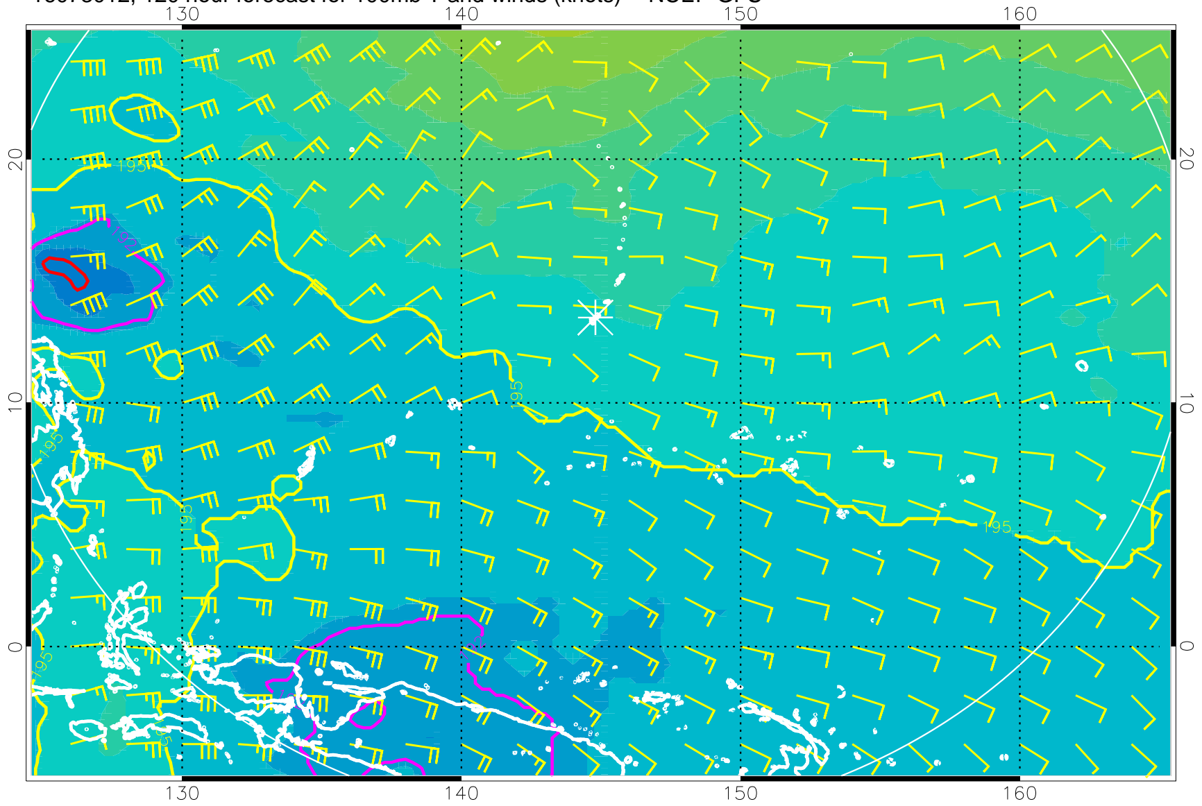
16073012, 120 hour forecast for 100mb T and winds (knots) -- NCEP GFS
