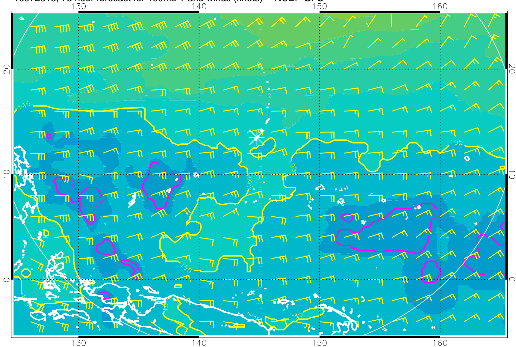
16072818, 78 hour forecast for 100mb T and winds (knots) -- NCEP GFS
