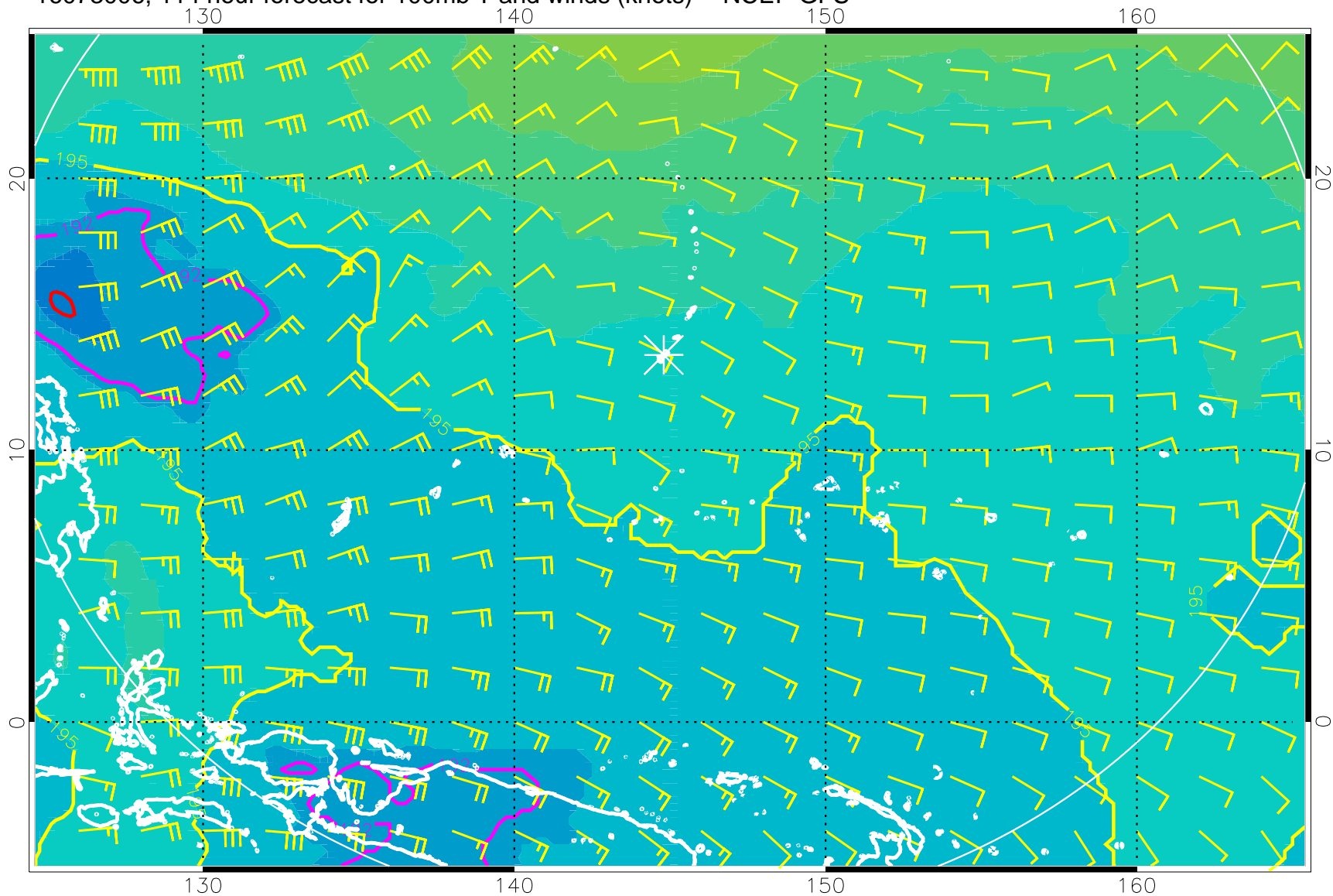
16073006, 114 hour forecast for 100mb T and winds (knots) -- NCEP GFS
