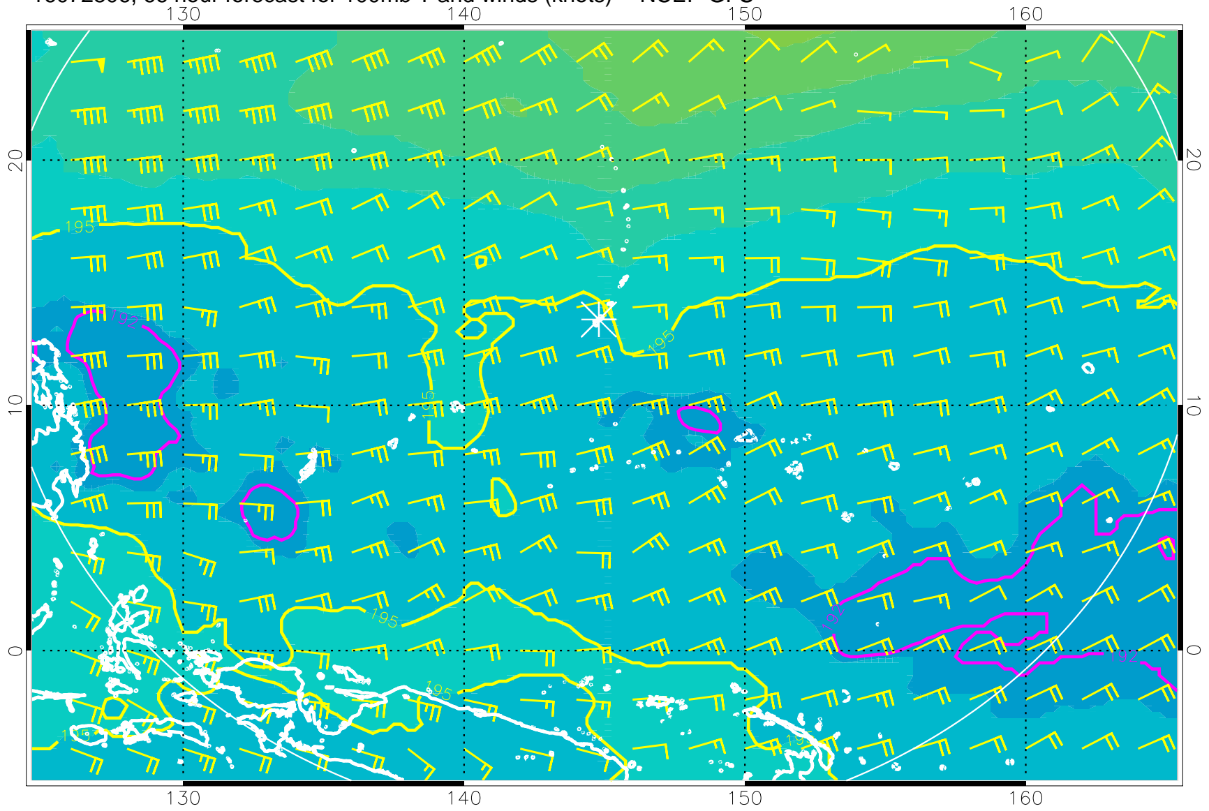
16072806, 66 hour forecast for 100mb T and winds (knots) -- NCEP GFS
