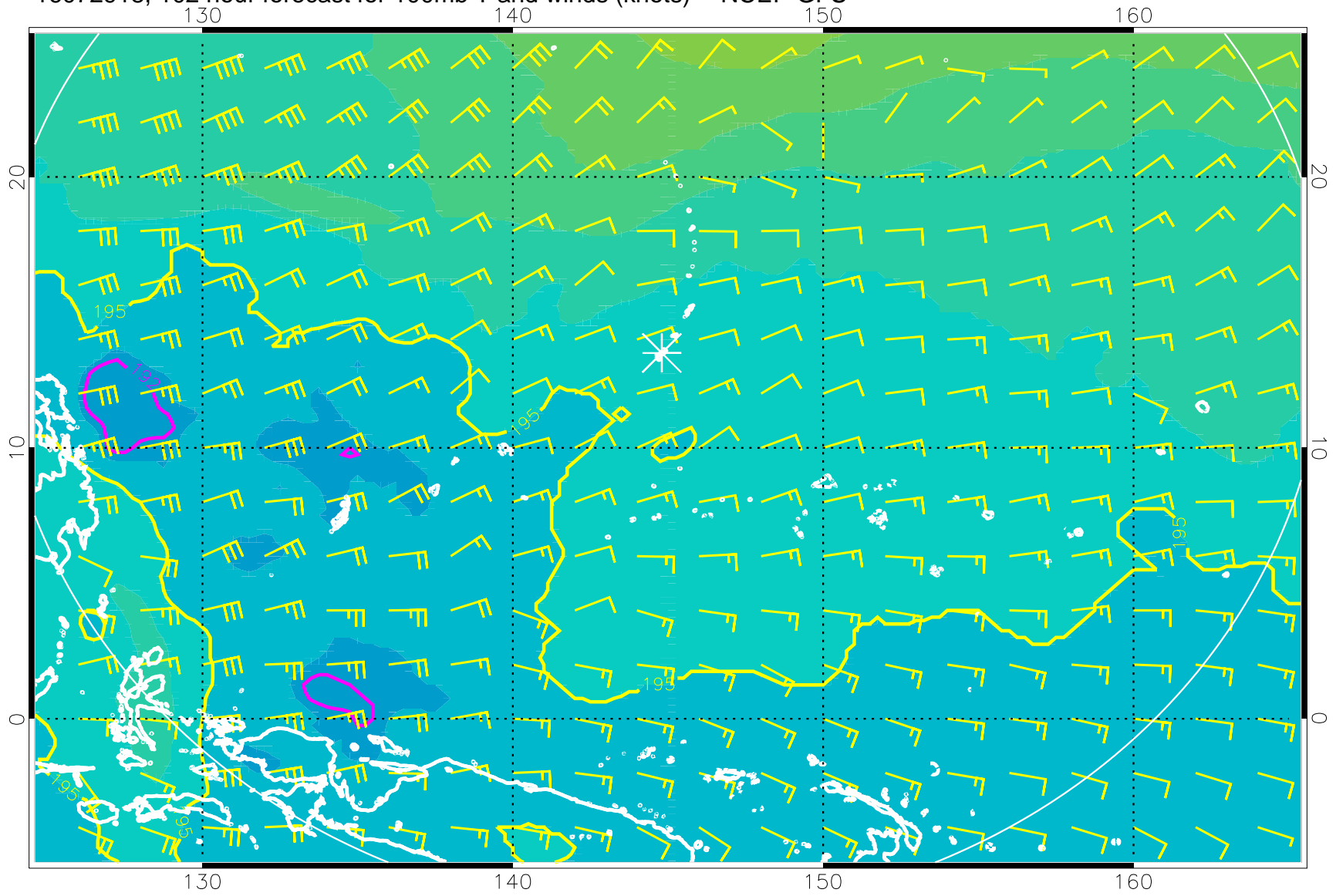
16072918, 102 hour forecast for 100mb T and winds (knots) -- NCEP GFS
