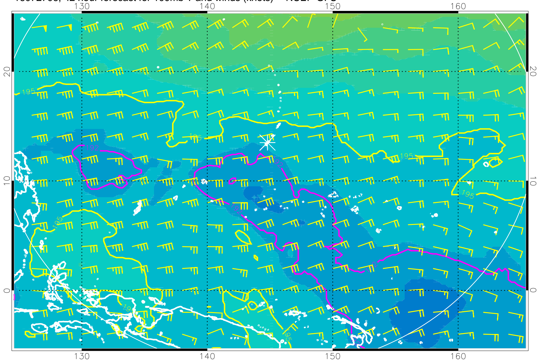
16072706, 42 hour forecast for 100mb T and winds (knots) -- NCEP GFS
