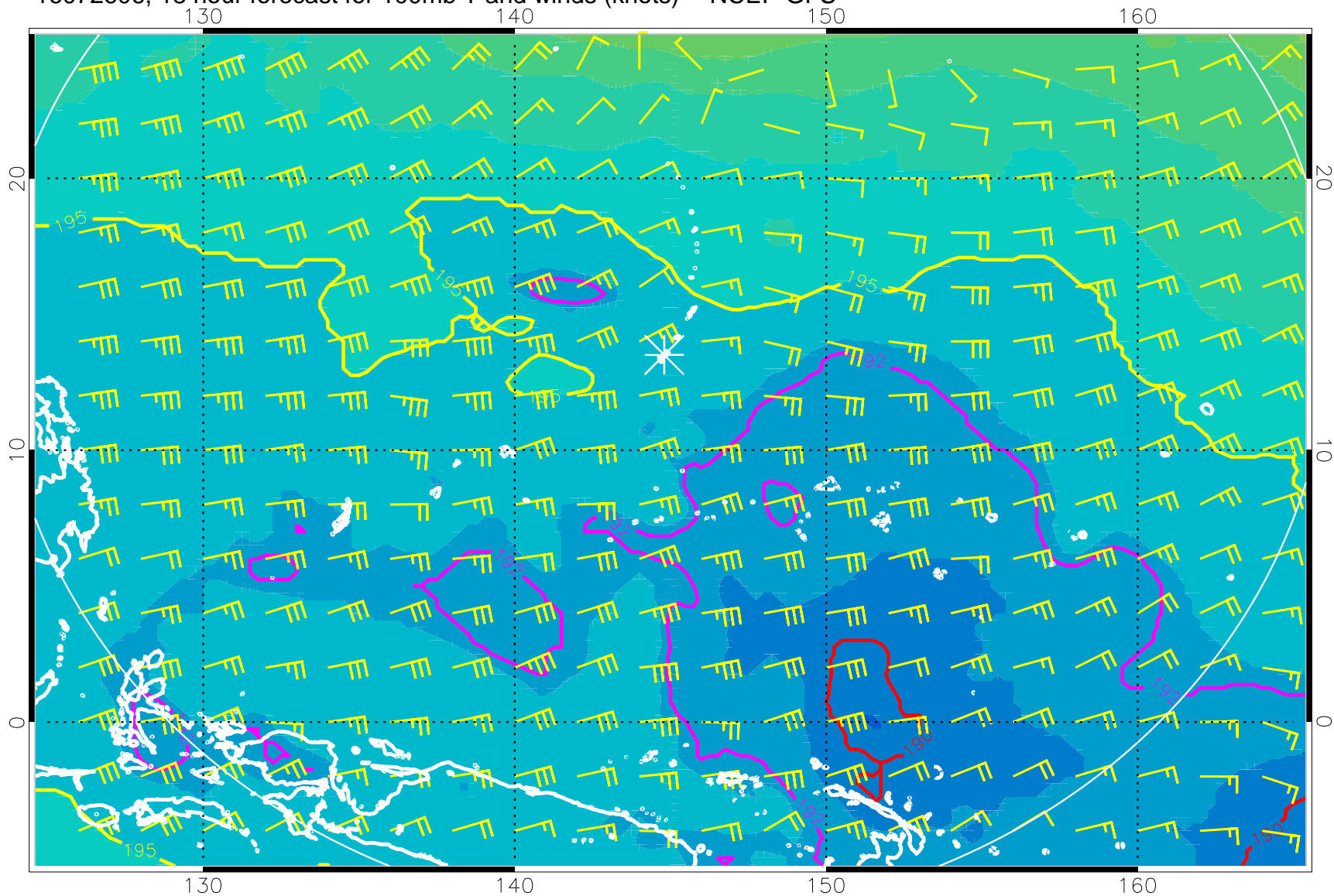
16072606, 18 hour forecast for 100mb T and winds (knots) -- NCEP GFS
