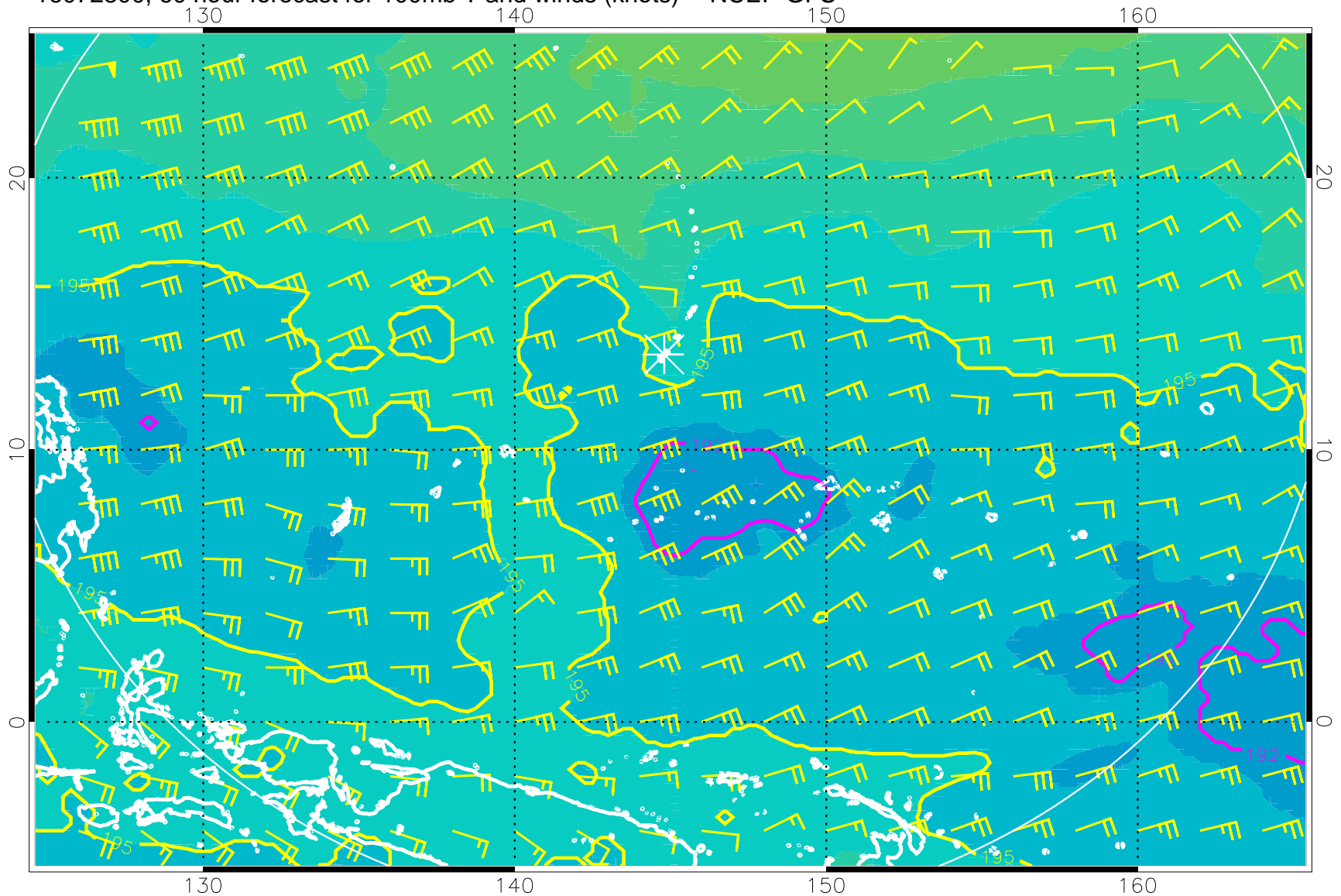
16072800, 60 hour forecast for 100mb T and winds (knots) -- NCEP GFS
