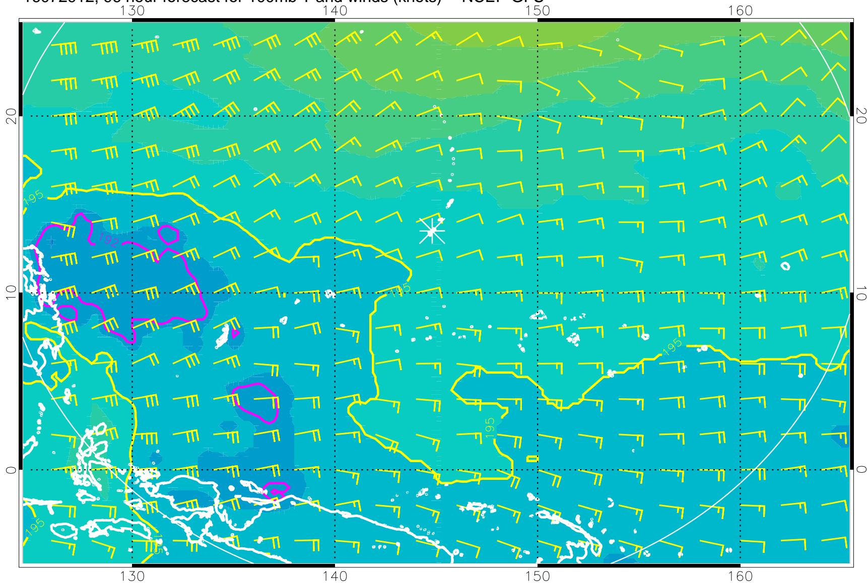
16072912, 96 hour forecast for 100mb T and winds (knots) -- NCEP GFS
