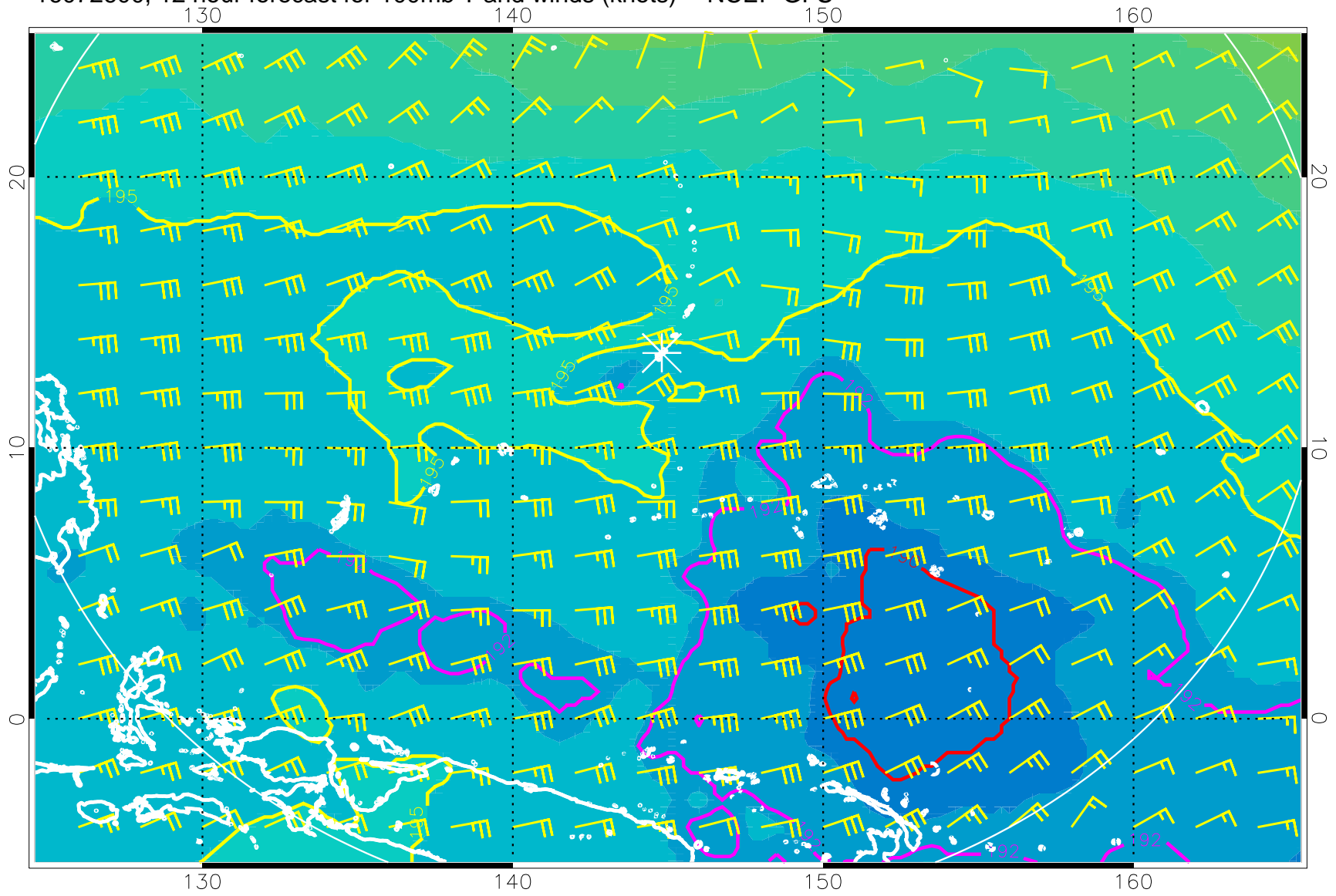
16072600, 12 hour forecast for 100mb T and winds (knots) -- NCEP GFS
