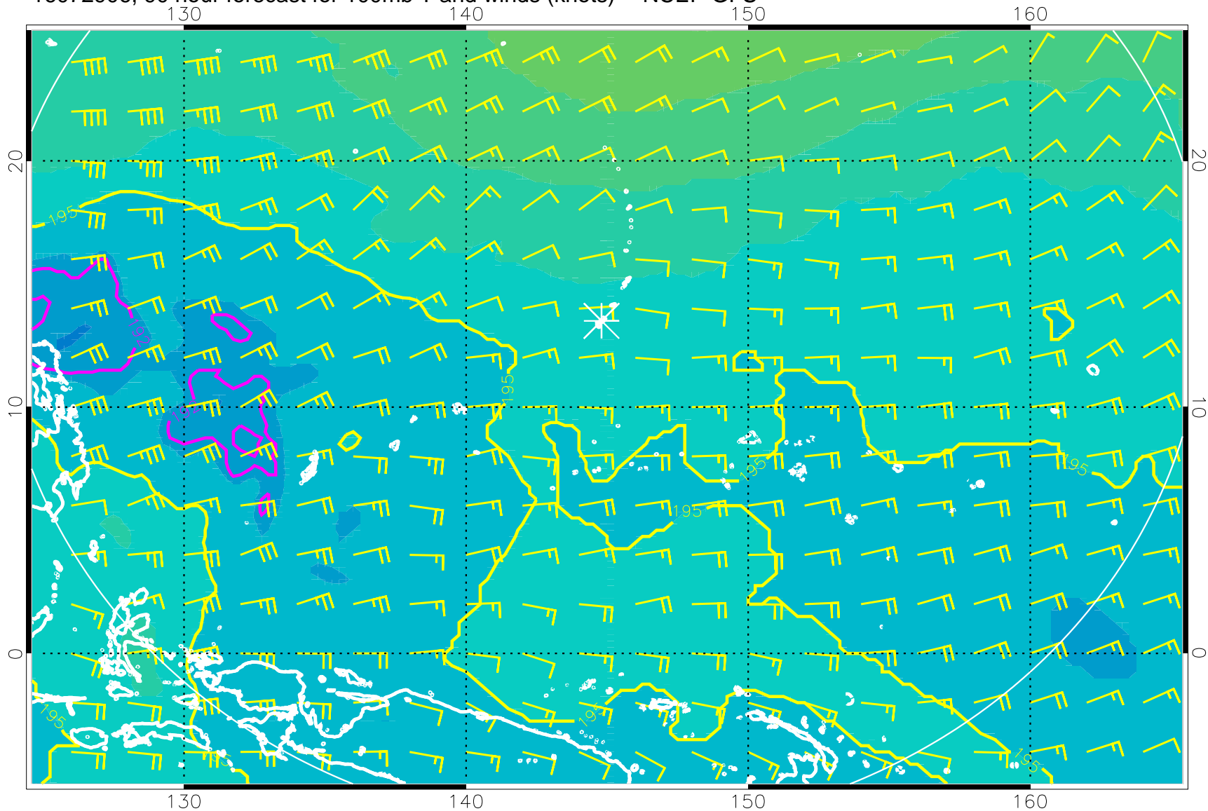
16072906, 90 hour forecast for 100mb T and winds (knots) -- NCEP GFS
