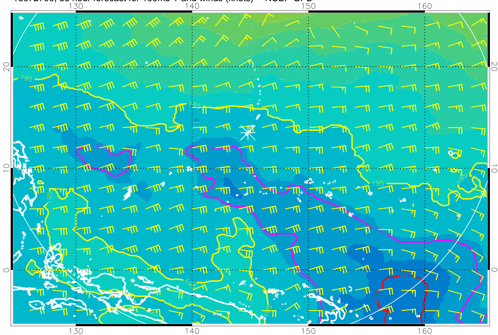
16072700, 36 hour forecast for 100mb T and winds (knots) -- NCEP GFS
