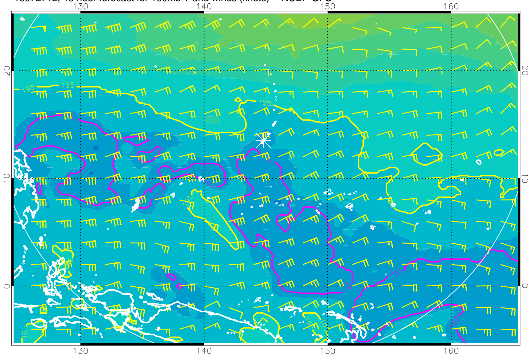
16072712, 48 hour forecast for 100mb T and winds (knots) -- NCEP GFS
