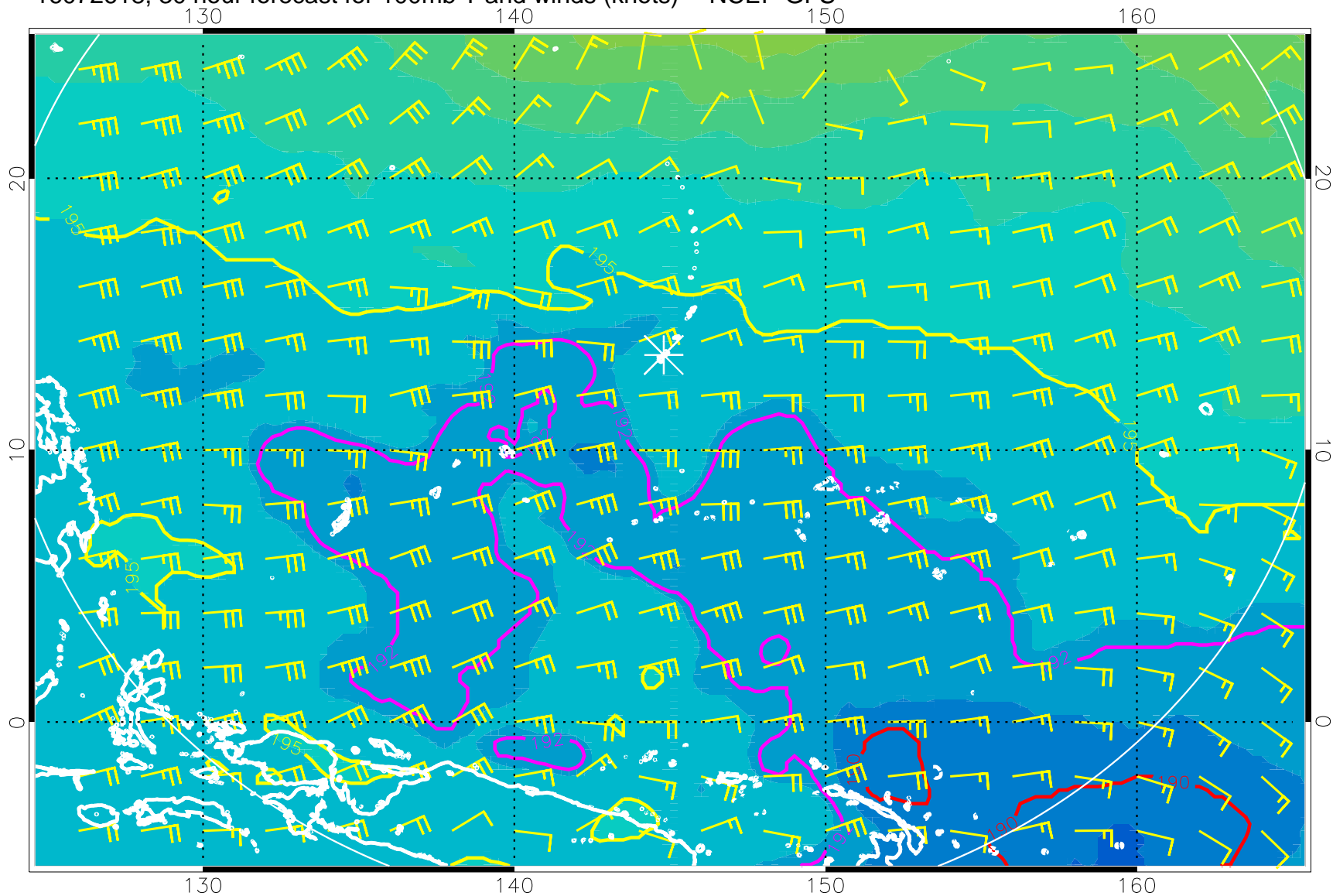
16072618, 30 hour forecast for 100mb T and winds (knots) -- NCEP GFS
