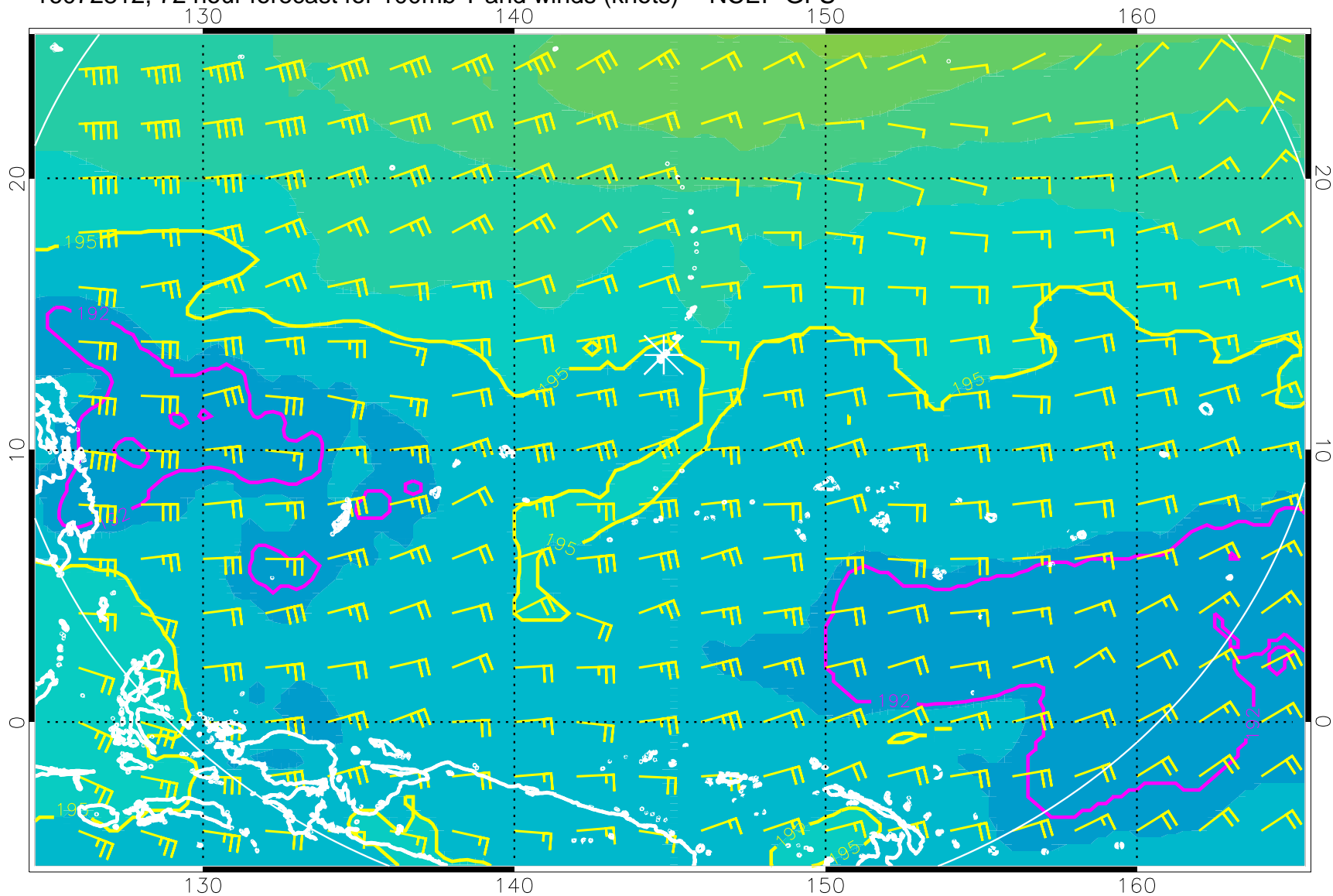
16072812, 72 hour forecast for 100mb T and winds (knots) -- NCEP GFS
