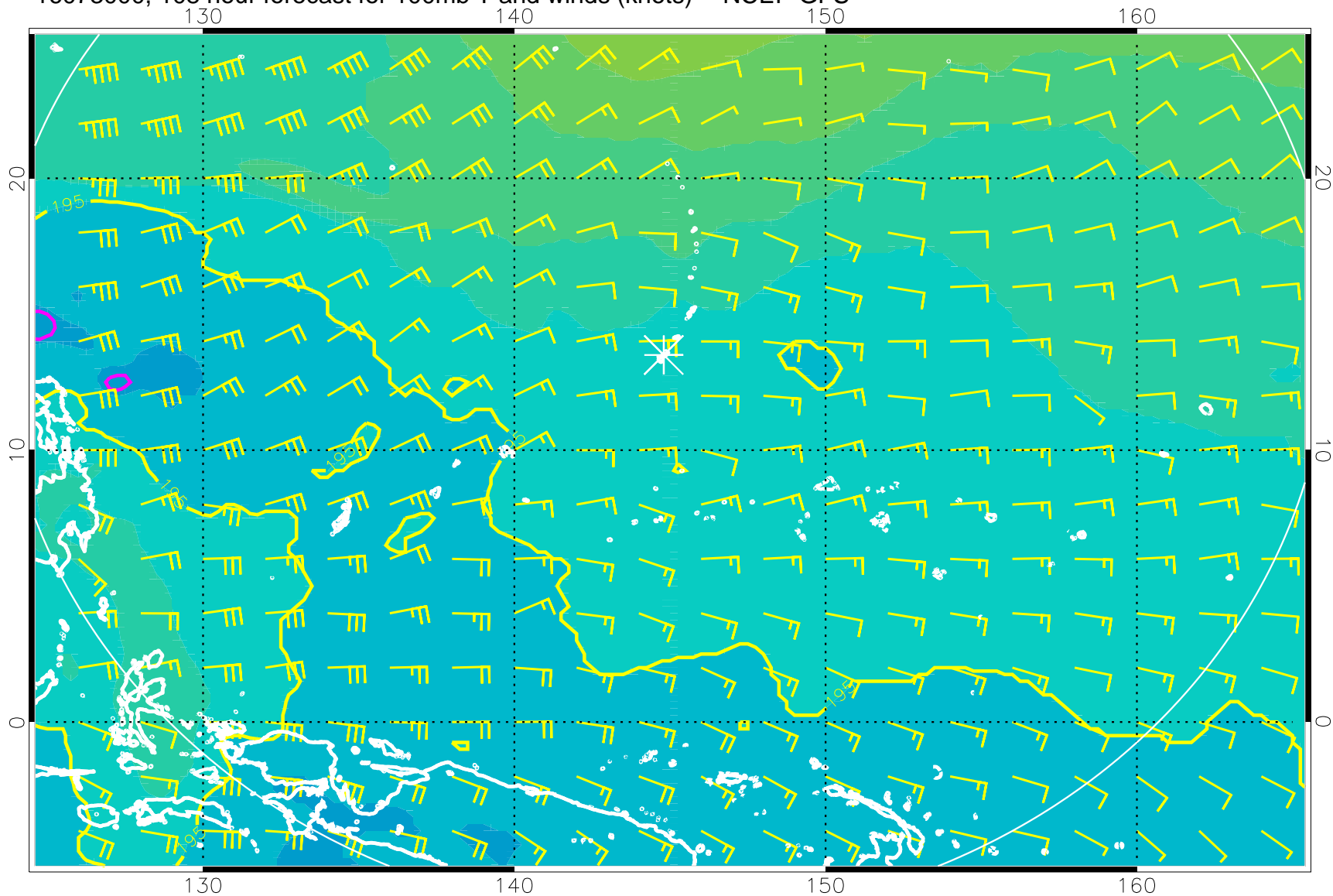
16073000, 108 hour forecast for 100mb T and winds (knots) -- NCEP GFS
