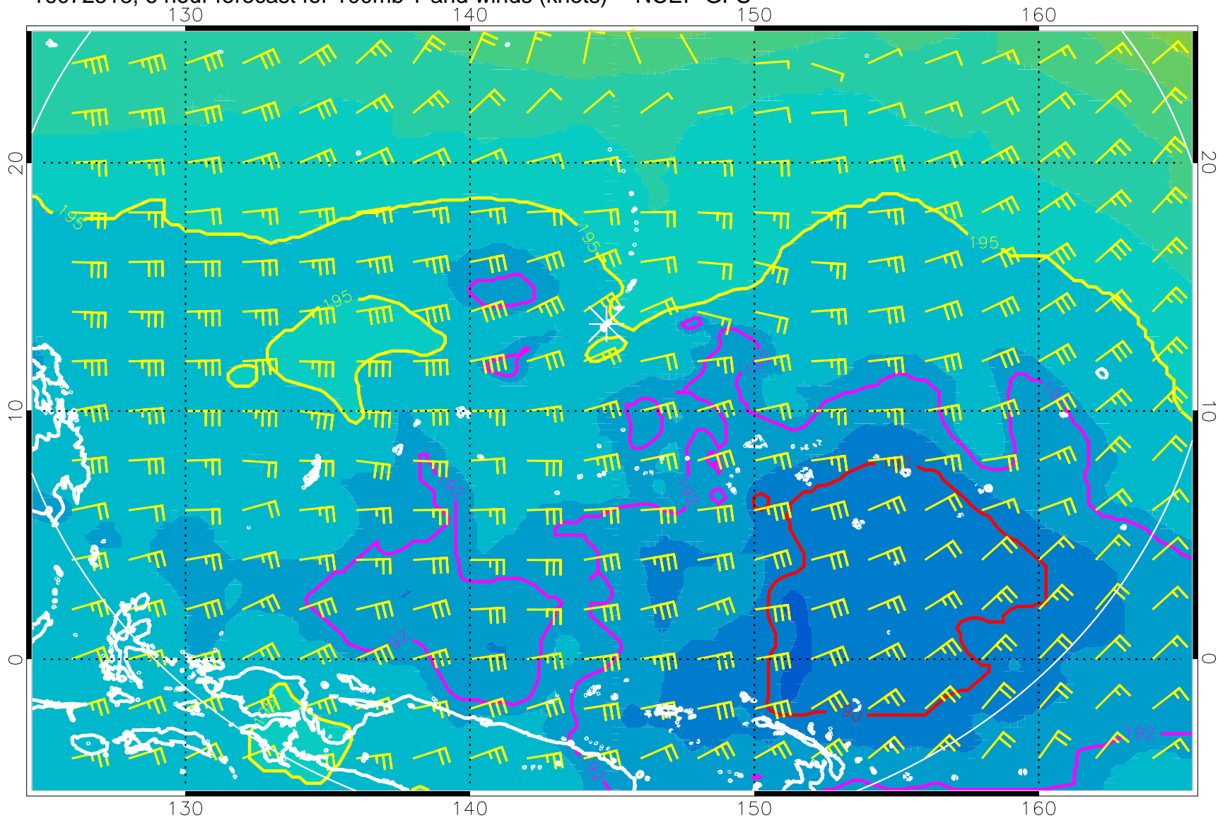
16072518, 6 hour forecast for 100mb T and winds (knots) -- NCEP GFS
