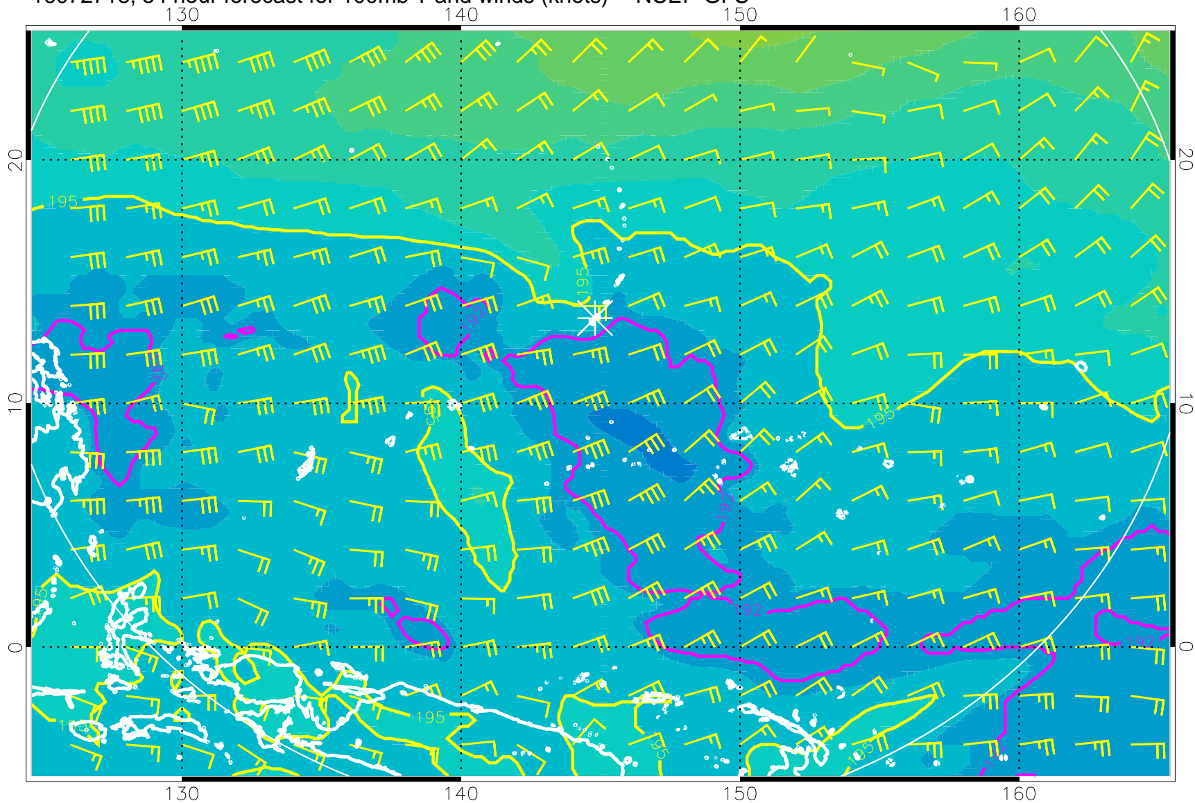
16072718, 54 hour forecast for 100mb T and winds (knots) -- NCEP GFS
