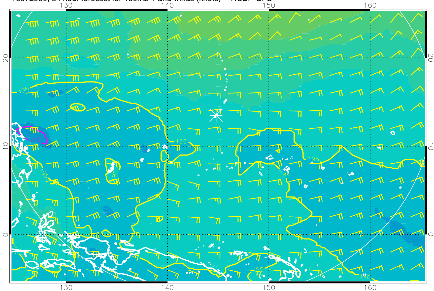
16072900, 84 hour forecast for 100mb T and winds (knots) -- NCEP GFS
