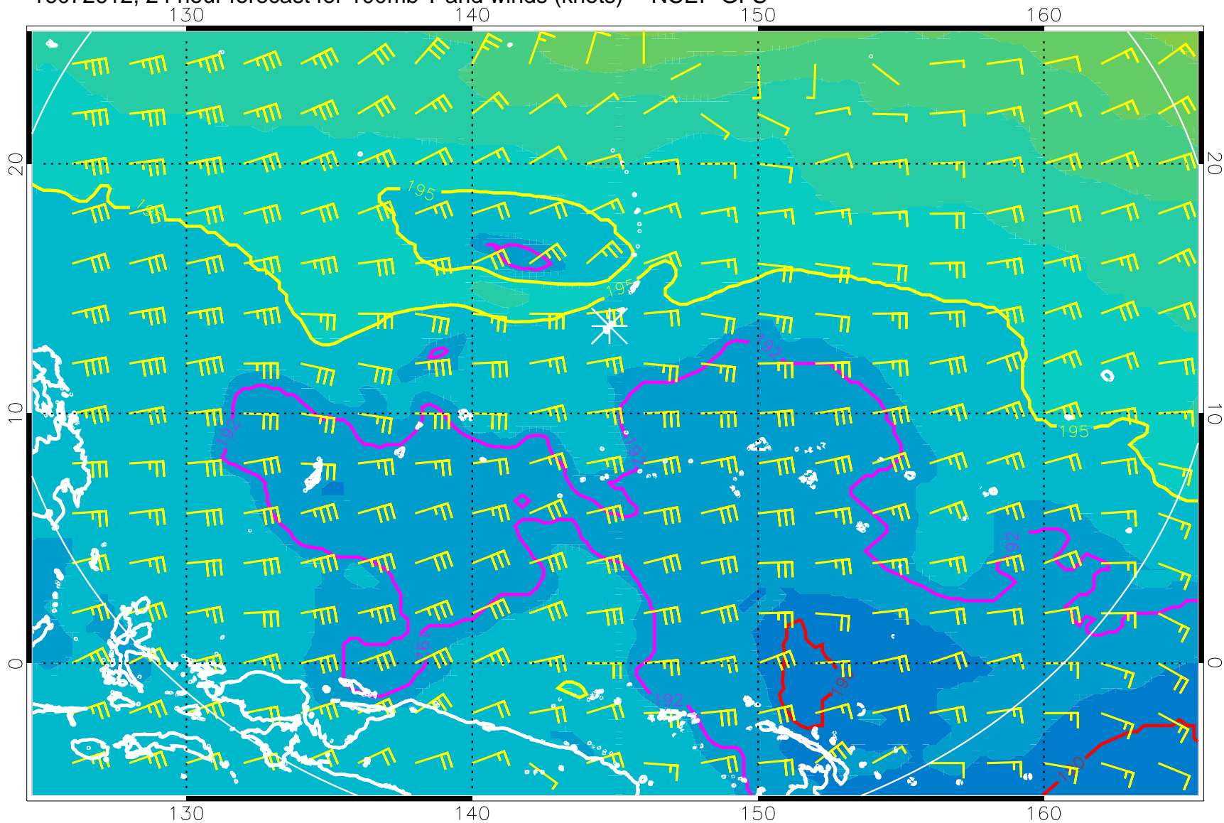
16072612, 24 hour forecast for 100mb T and winds (knots) -- NCEP GFS
