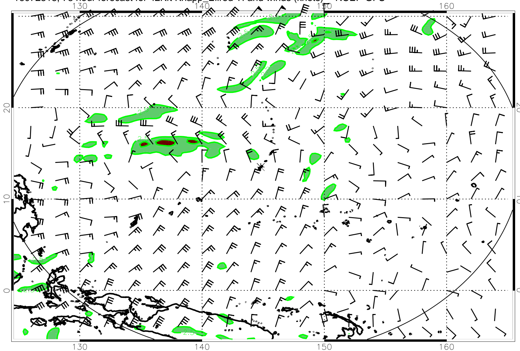
16072818, 78 hour forecast for 42Kft Knapp_Ellrod TI and winds (knots) -- NCEP GFS
