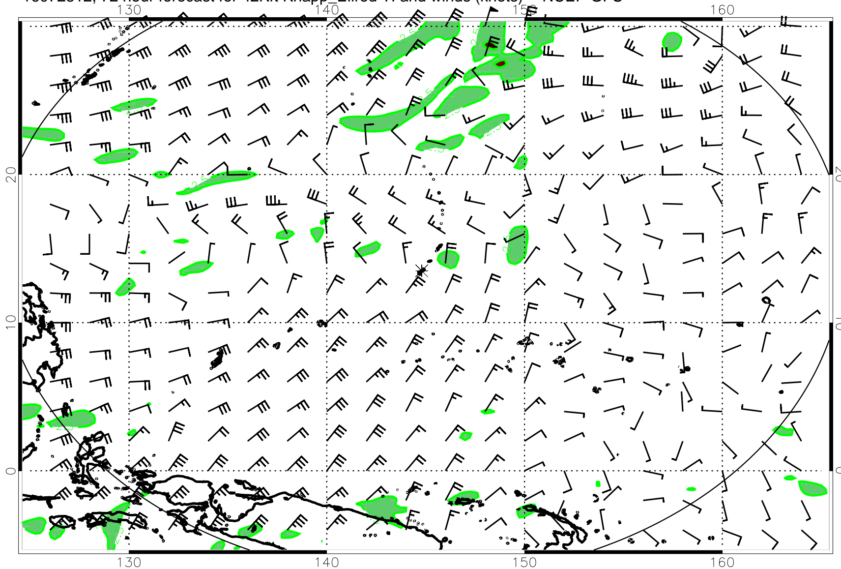
16072812, 72 hour forecast for 42Kft Knapp_Ellrod TI and winds (knots) -- NCEP GFS
