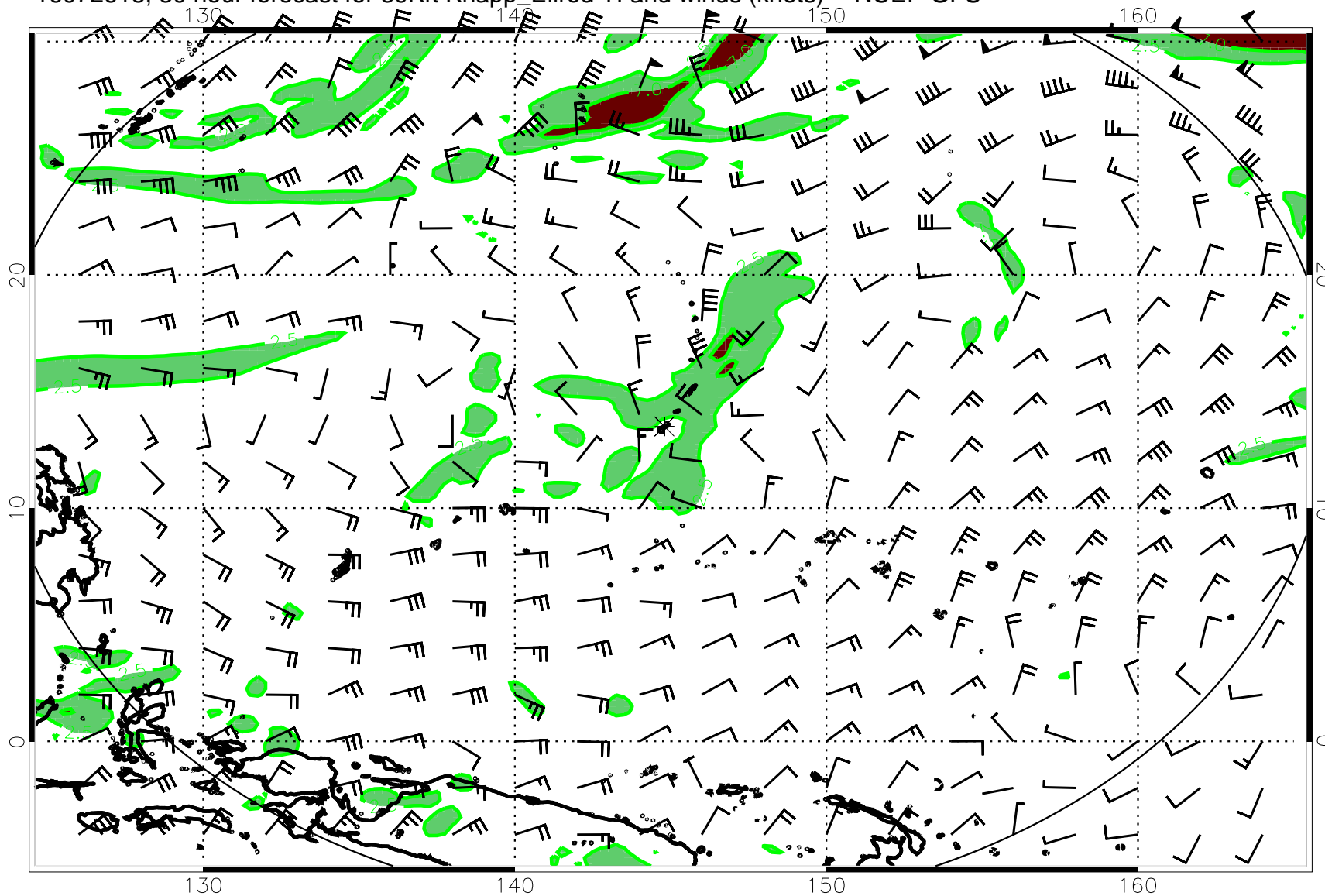
16072618, 30 hour forecast for 39Kft Knapp_Ellrod TI and winds (knots) -- NCEP GFS
