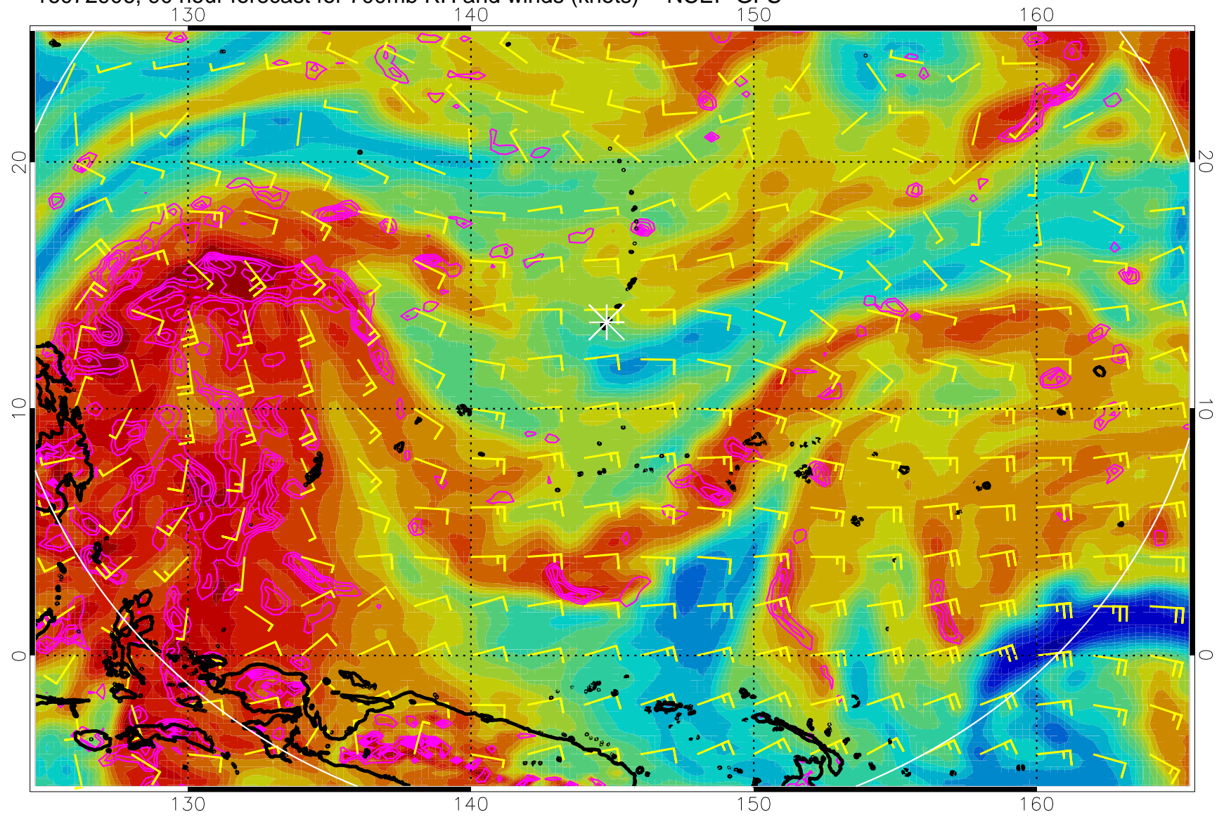
16072906, 90 hour forecast for 700mb RH and winds (knots) -- NCEP GFS
