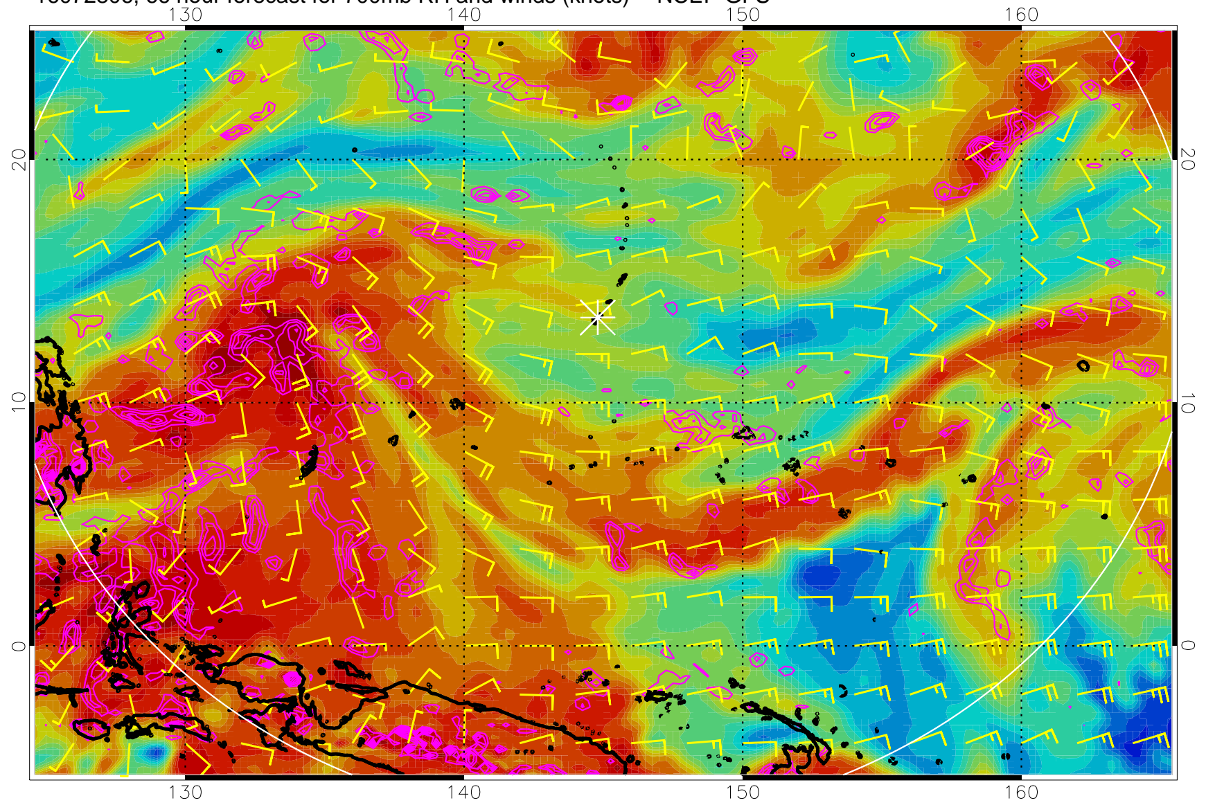
16072806, 66 hour forecast for 700mb RH and winds (knots) -- NCEP GFS
