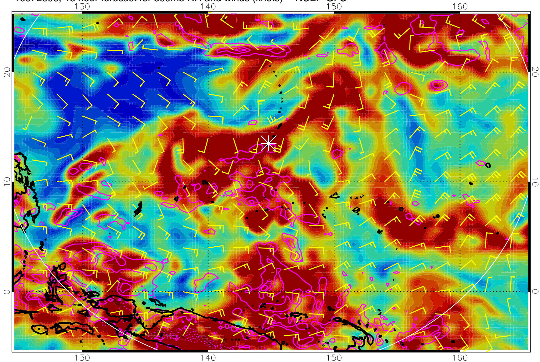
16072606, 18 hour forecast for 300mb RH and winds (knots) -- NCEP GFS
