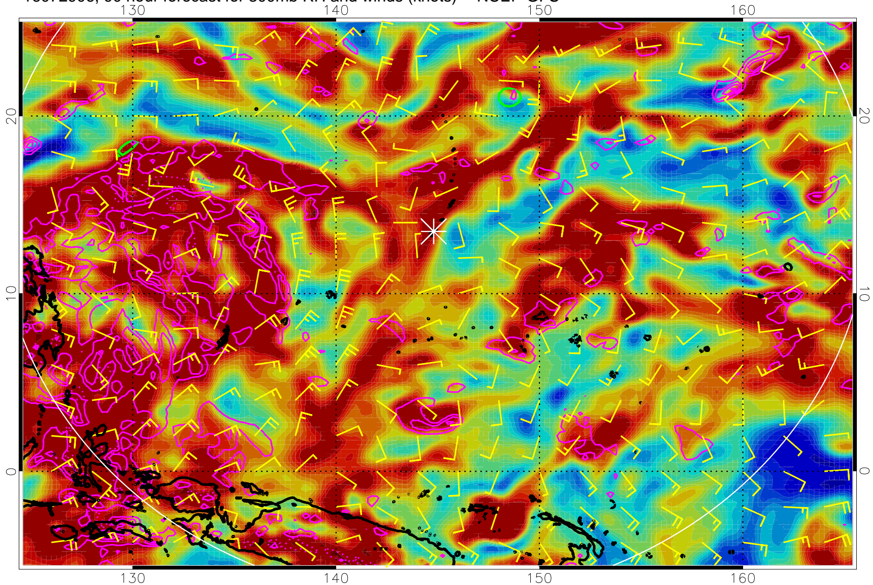
16072906, 90 hour forecast for 300mb RH and winds (knots) -- NCEP GFS
