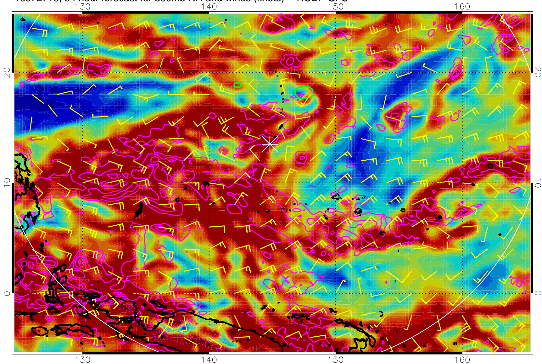
16072718, 54 hour forecast for 300mb RH and winds (knots) -- NCEP GFS
