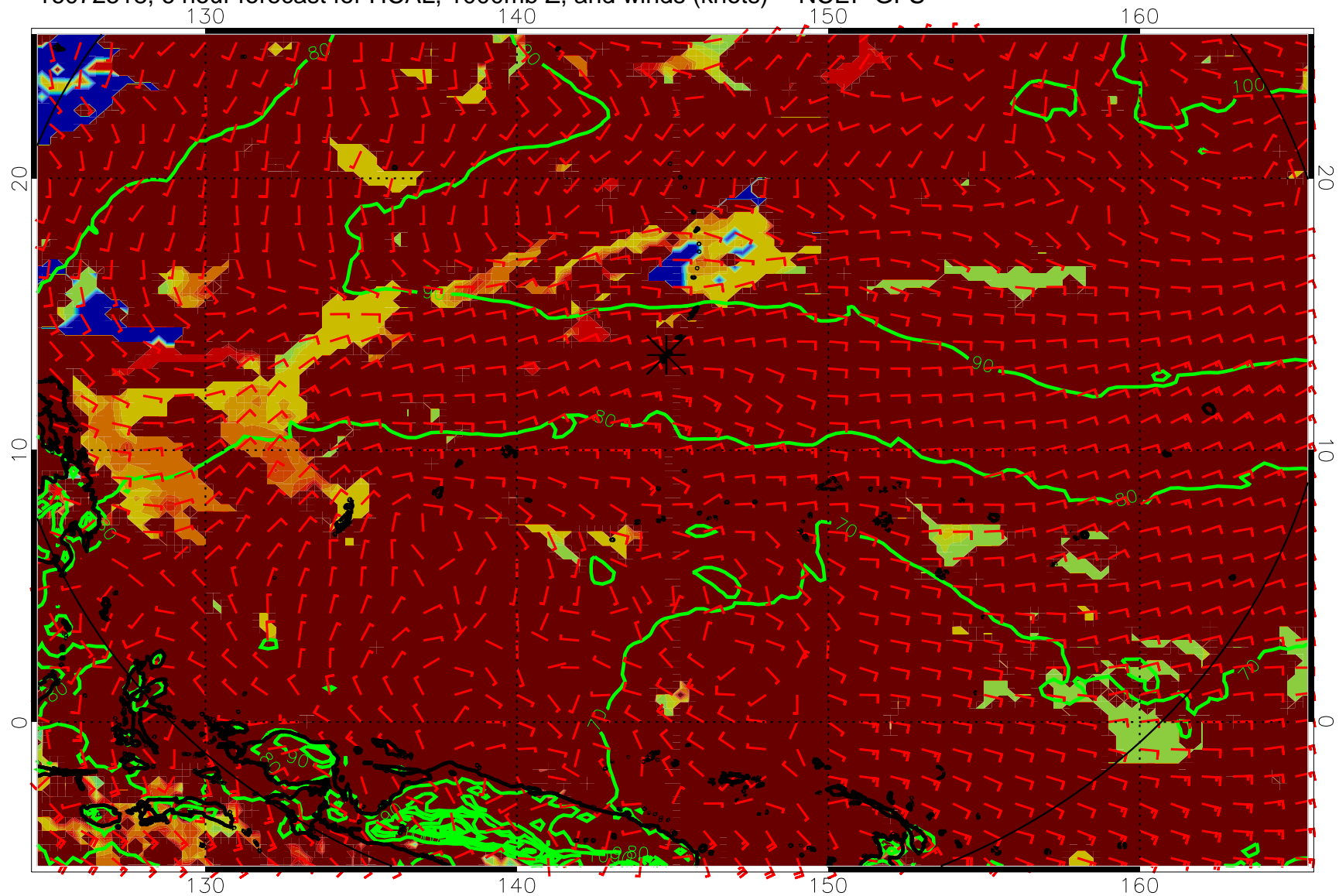
16072518, 6 hour forecast for HCAL, 1000mb Z, and winds (knots) -- NCEP GFS
