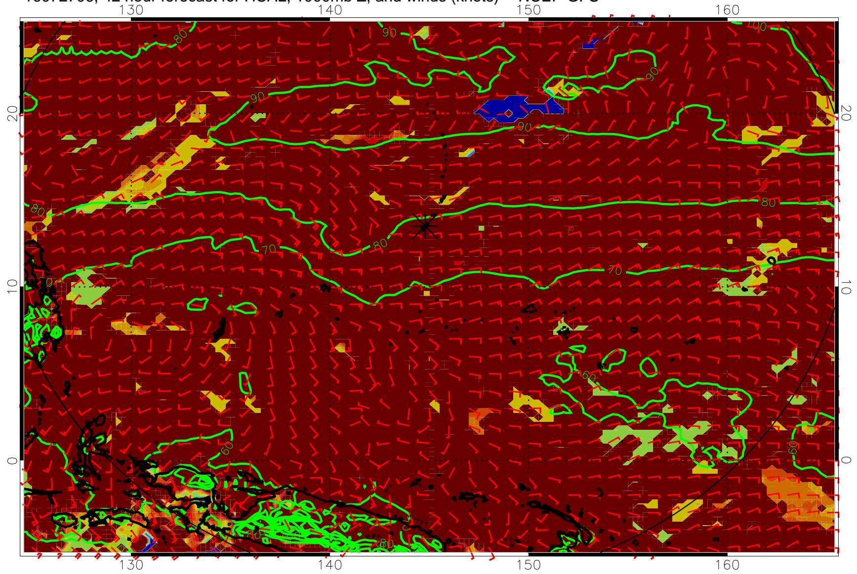
16072706, 42 hour forecast for HCAL, 1000mb Z, and winds (knots) -- NCEP GFS
