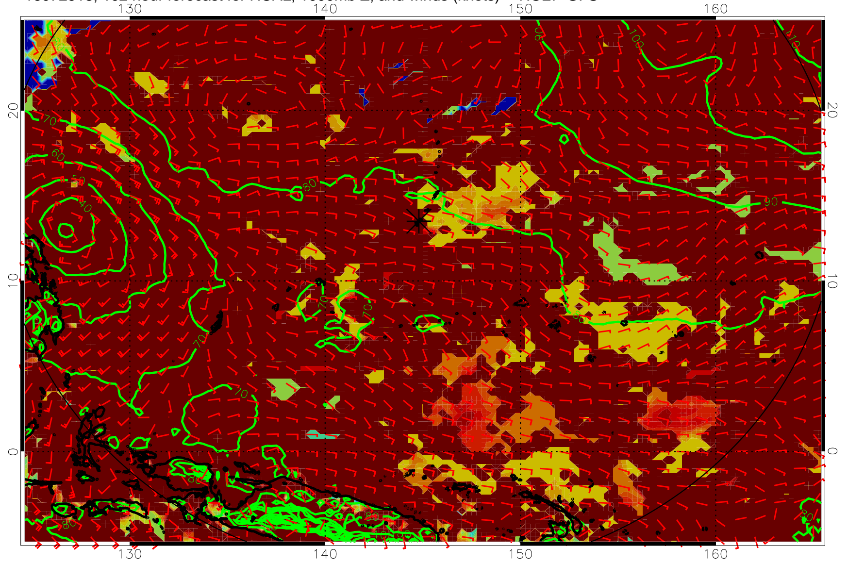
16072918, 102 hour forecast for HCAL, 1000mb Z, and winds (knots) -- NCEP GFS
