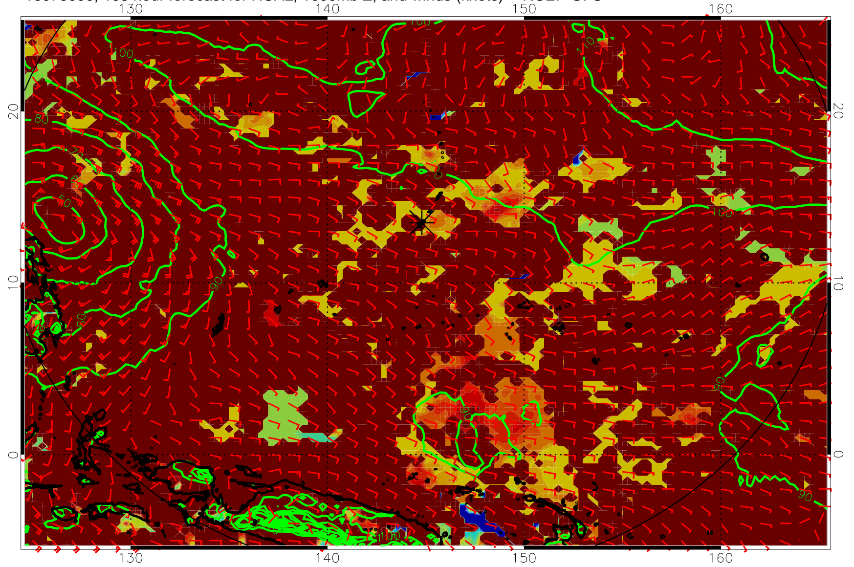
16073000, 108 hour forecast for HCAL, 1000mb Z, and winds (knots) -- NCEP GFS
