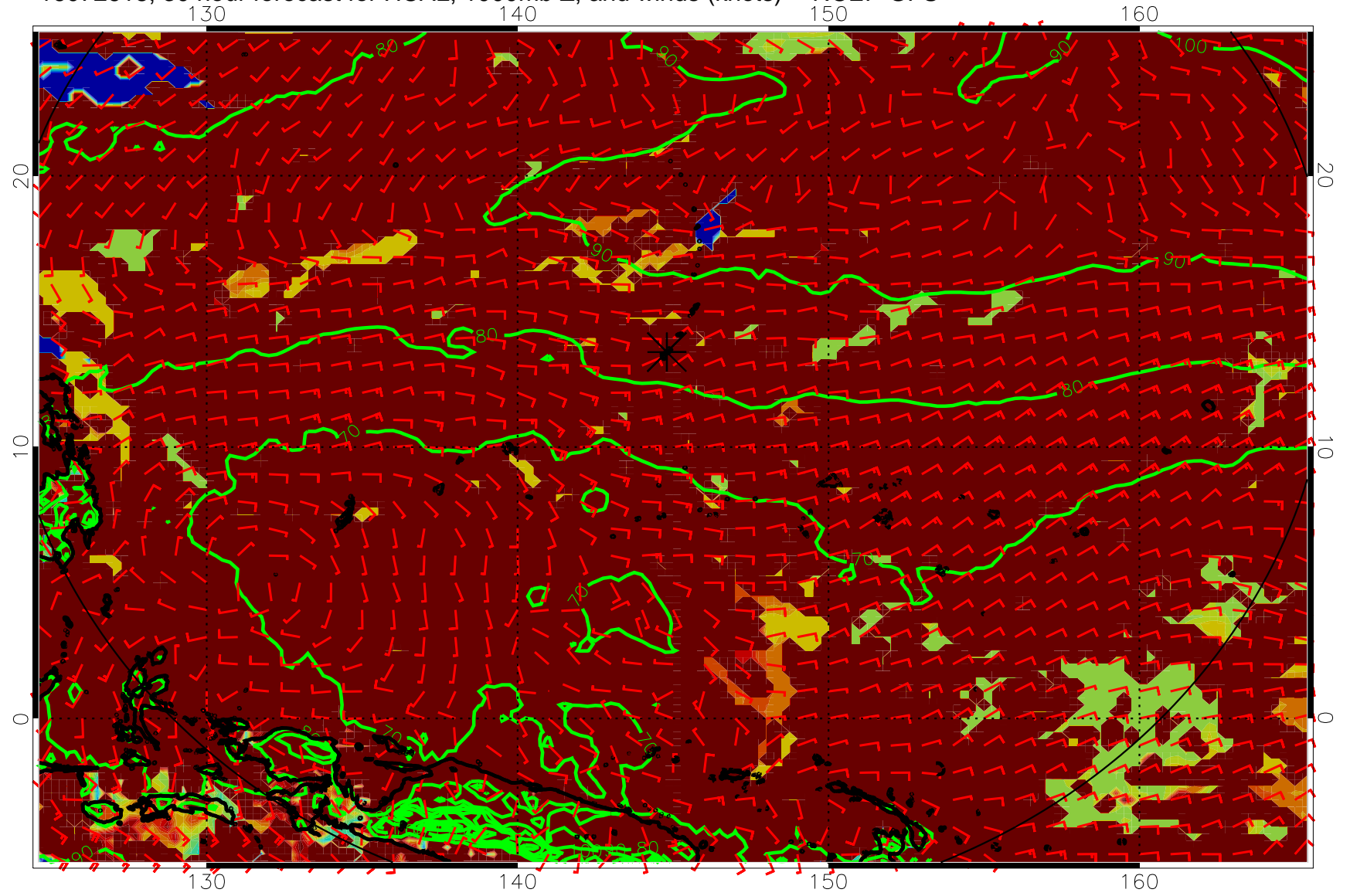
16072618, 30 hour forecast for HCAL, 1000mb Z, and winds (knots) -- NCEP GFS
