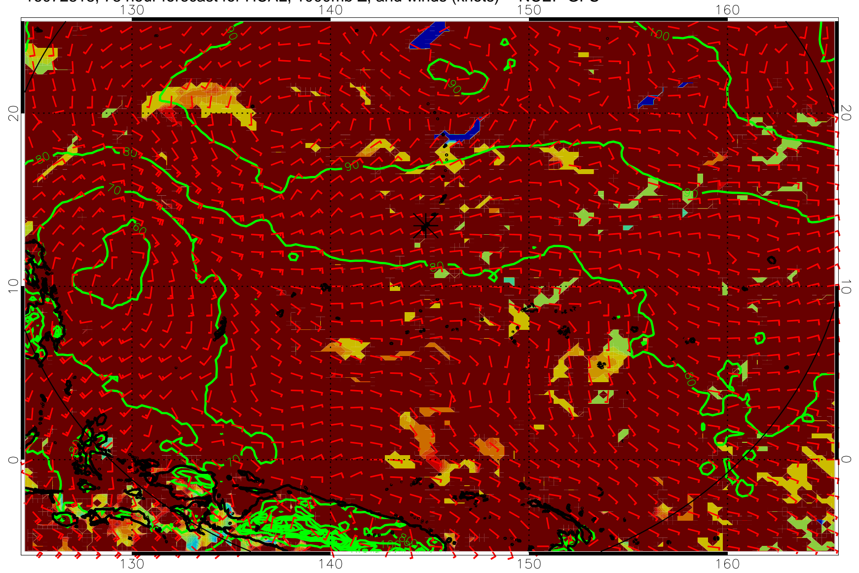
16072818, 78 hour forecast for HCAL, 1000mb Z, and winds (knots) -- NCEP GFS
