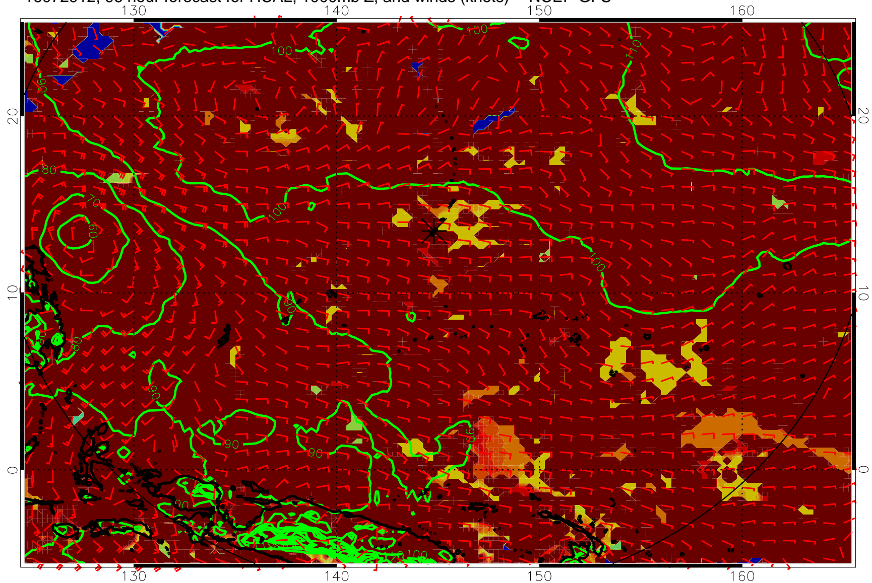
16072912, 96 hour forecast for HCAL, 1000mb Z, and winds (knots) -- NCEP GFS
