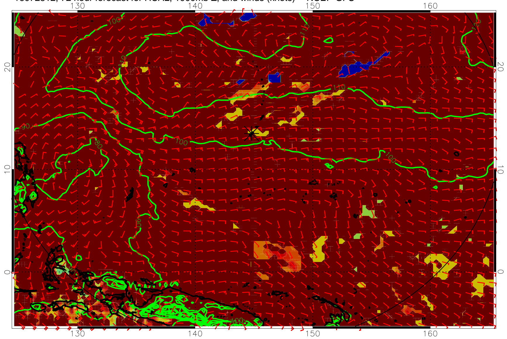
16072812, 72 hour forecast for HCAL, 1000mb Z, and winds (knots) -- NCEP GFS
