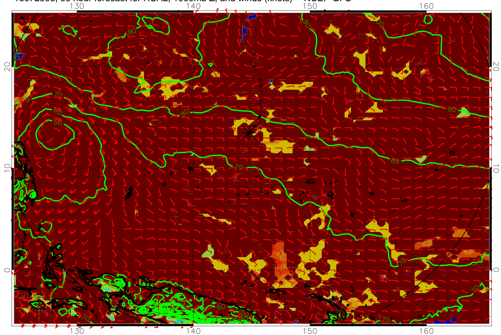
16072906, 90 hour forecast for HCAL, 1000mb Z, and winds (knots) -- NCEP GFS
