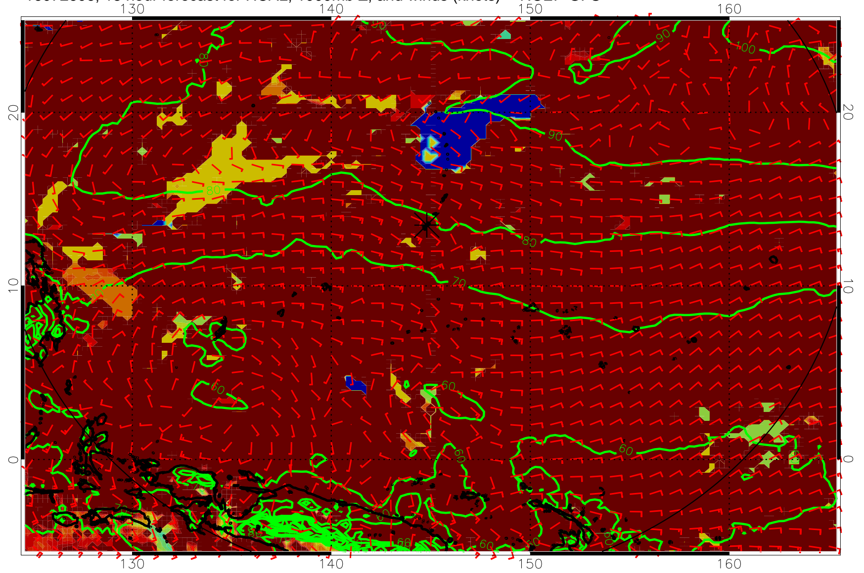
16072606, 18 hour forecast for HCAL, 1000mb Z, and winds (knots) -- NCEP GFS
