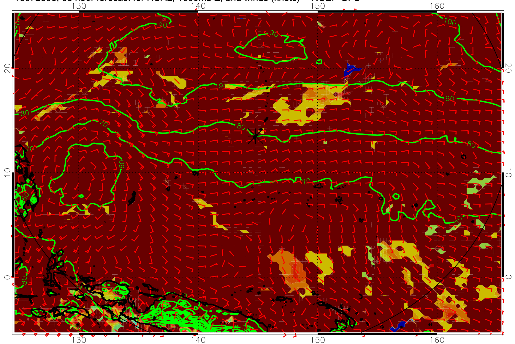
16072806, 66 hour forecast for HCAL, 1000mb Z, and winds (knots) -- NCEP GFS
