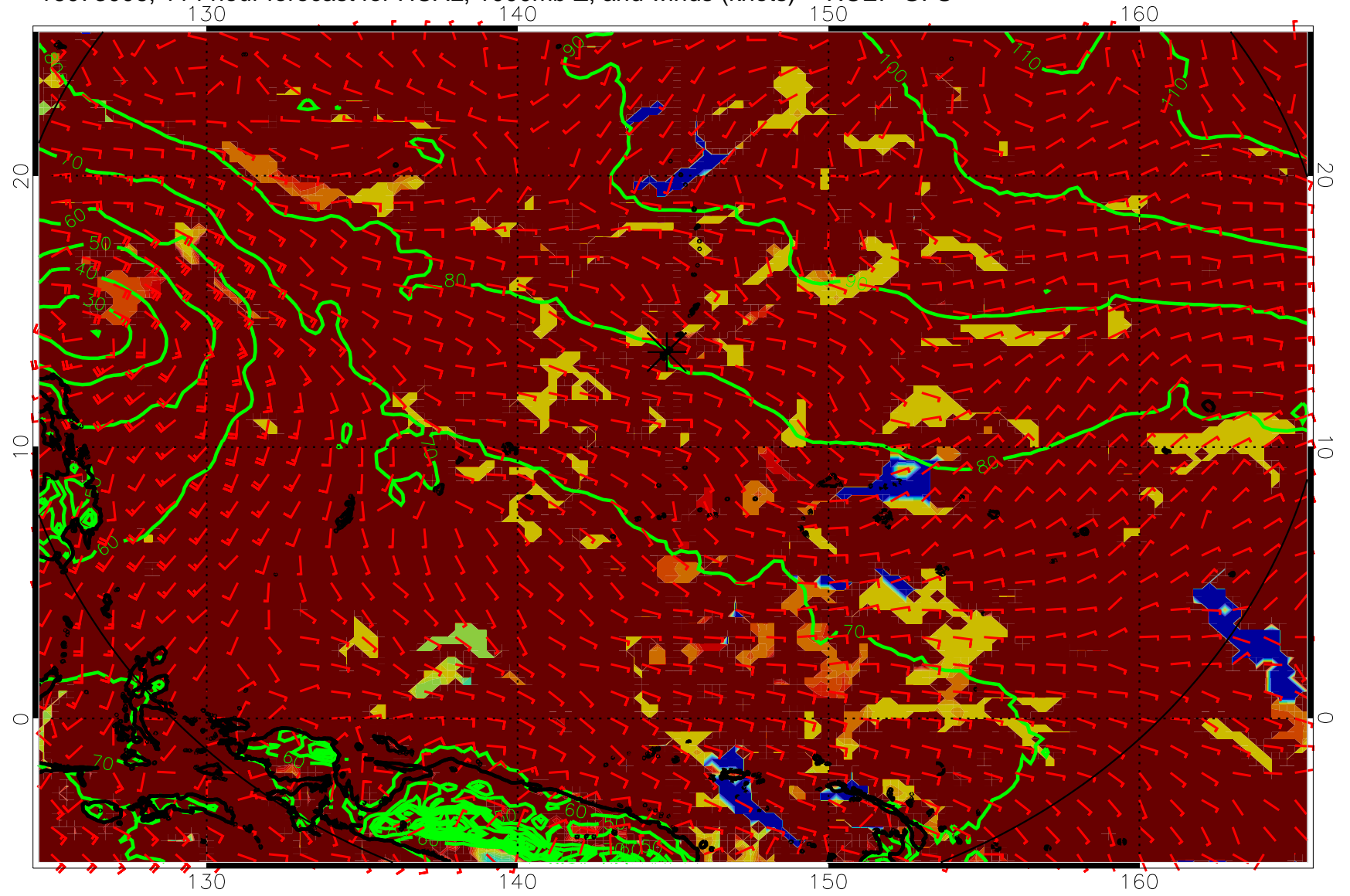
16073006, 114 hour forecast for HCAL, 1000mb Z, and winds (knots) -- NCEP GFS
