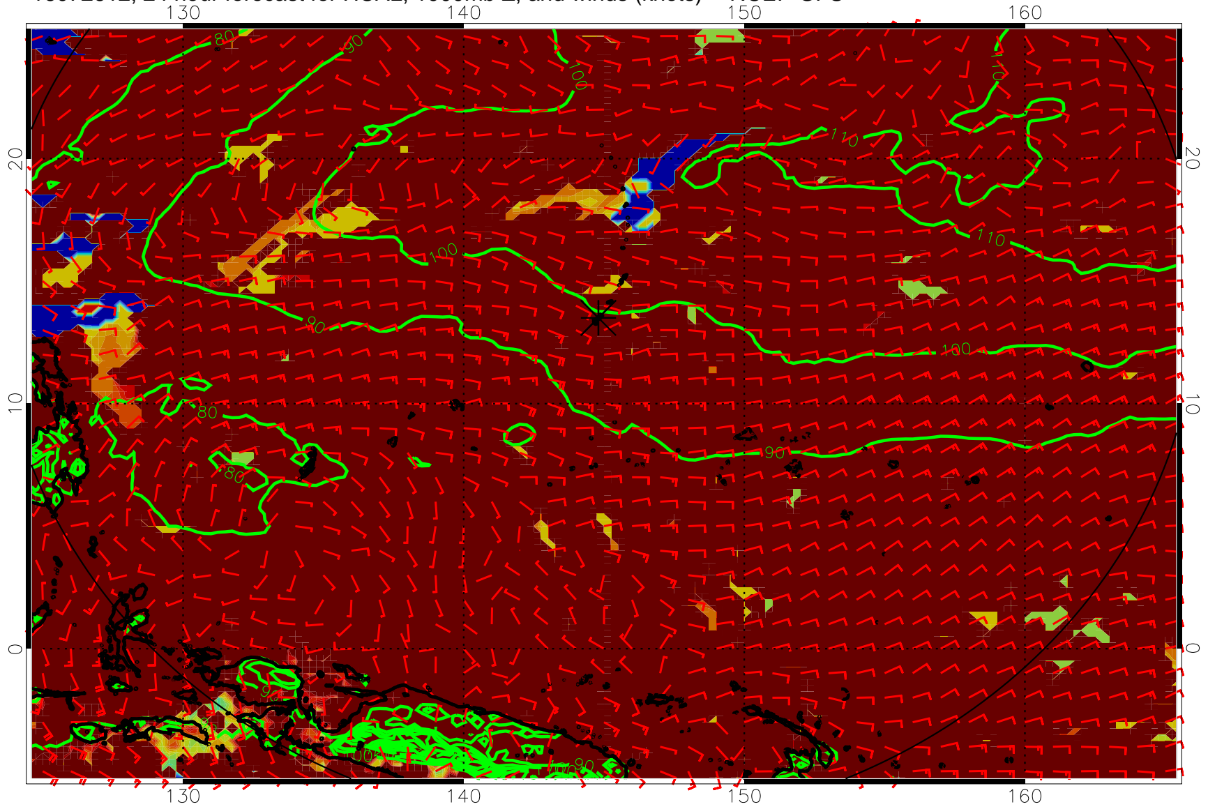
16072612, 24 hour forecast for HCAL, 1000mb Z, and winds (knots) -- NCEP GFS
