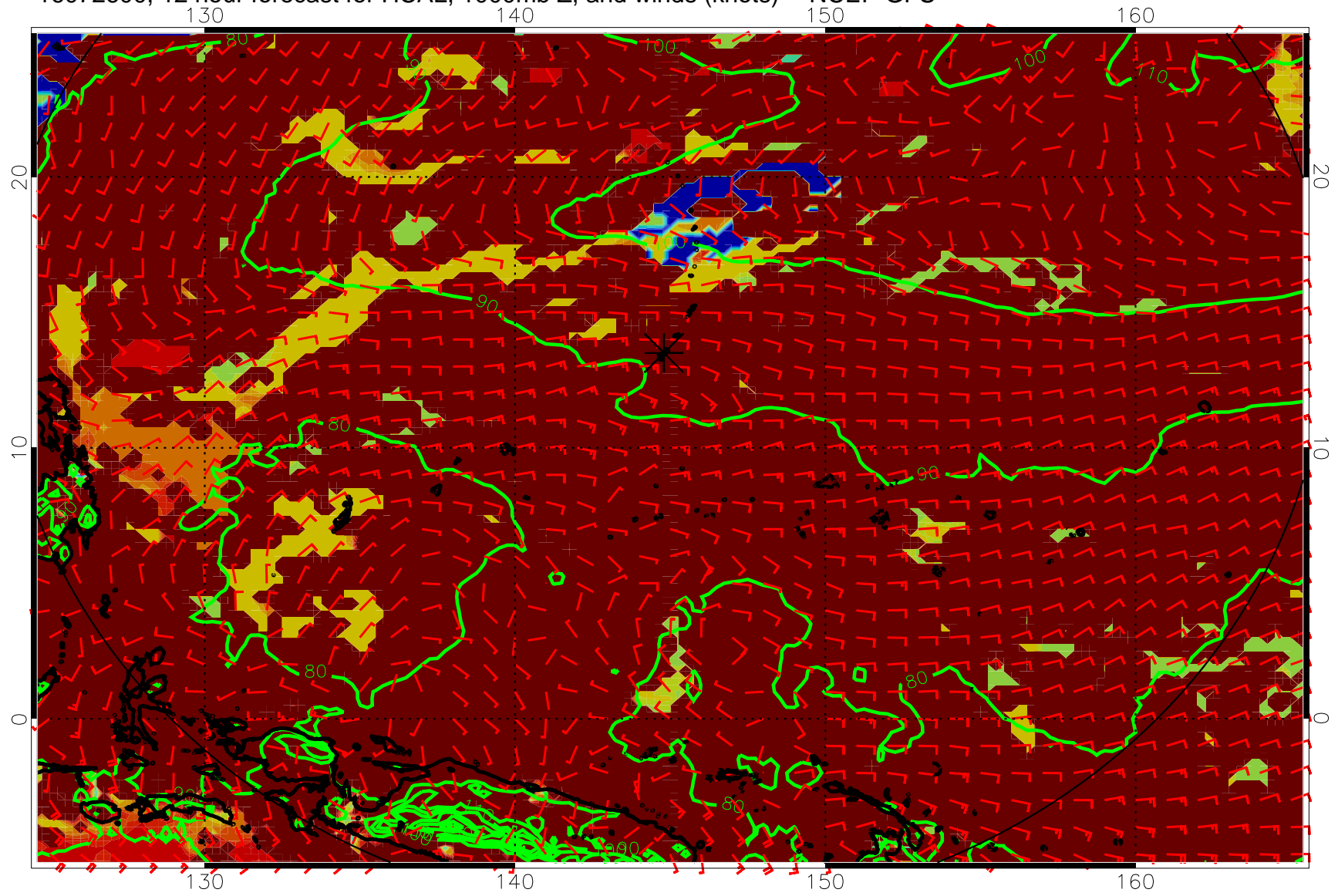
16072600, 12 hour forecast for HCAL, 1000mb Z, and winds (knots) -- NCEP GFS
