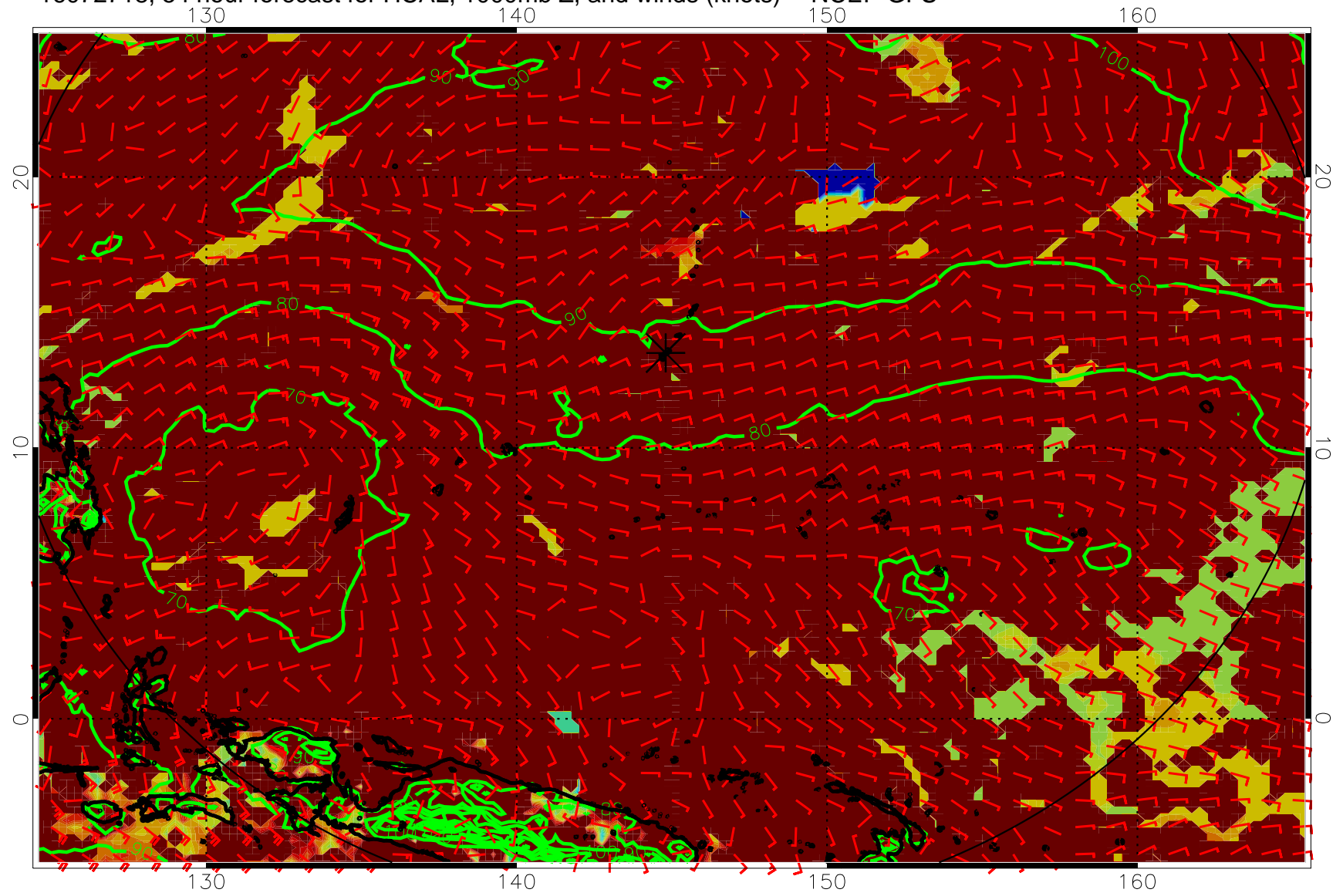
16072718, 54 hour forecast for HCAL, 1000mb Z, and winds (knots) -- NCEP GFS
