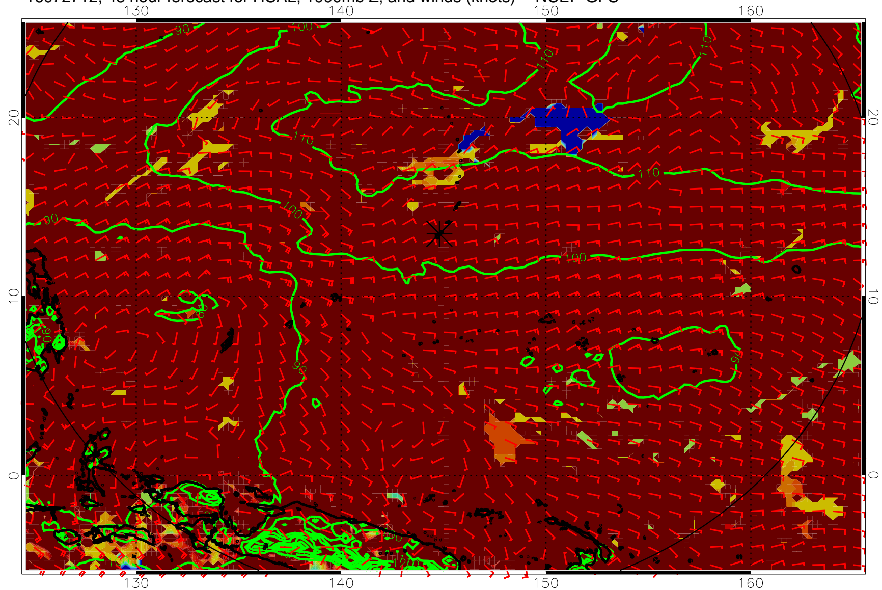
16072712, 48 hour forecast for HCAL, 1000mb Z, and winds (knots) -- NCEP GFS
