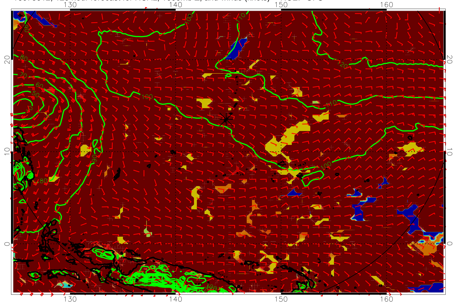
16073012, 120 hour forecast for HCAL, 1000mb Z, and winds (knots) -- NCEP GFS
