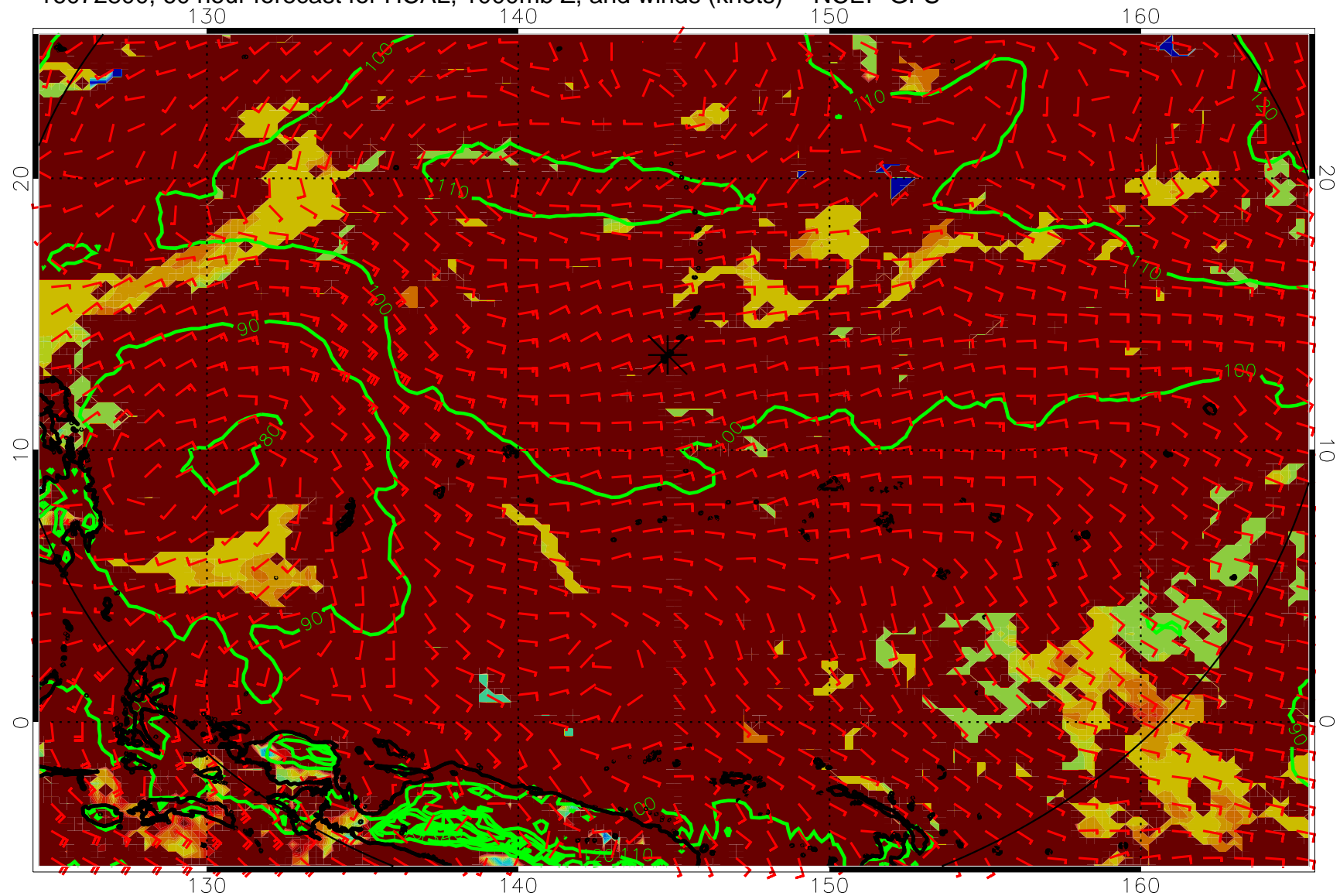
16072800, 60 hour forecast for HCAL, 1000mb Z, and winds (knots) -- NCEP GFS
