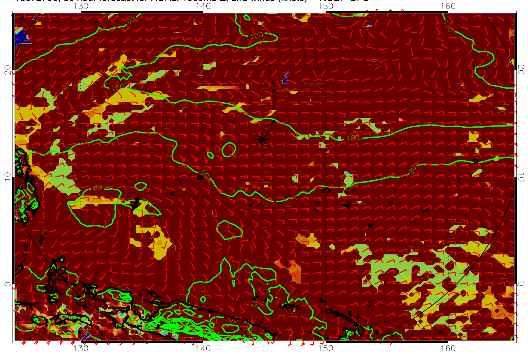
16072700, 36 hour forecast for HCAL, 1000mb Z, and winds (knots) -- NCEP GFS
