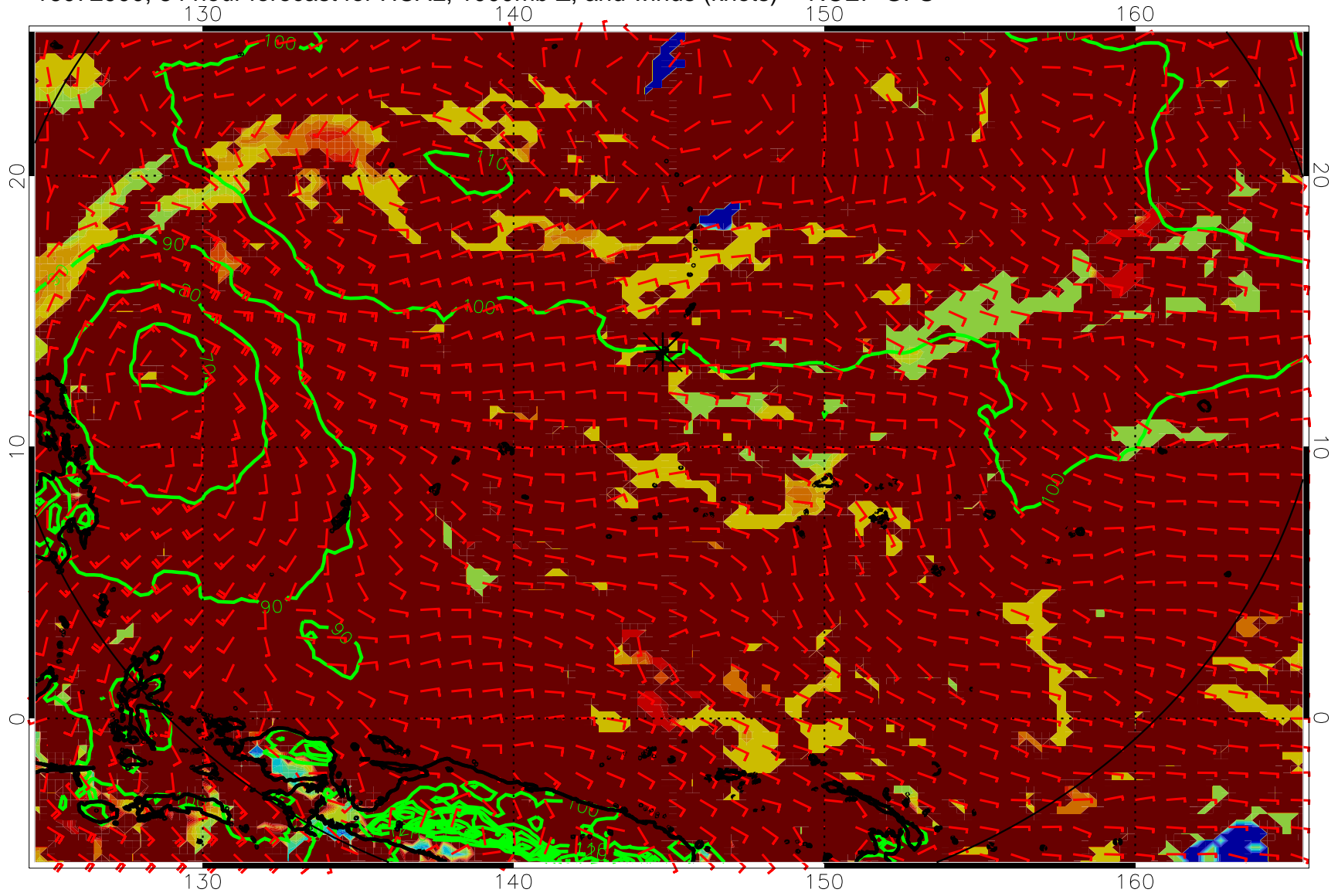
16072900, 84 hour forecast for HCAL, 1000mb Z, and winds (knots) -- NCEP GFS
