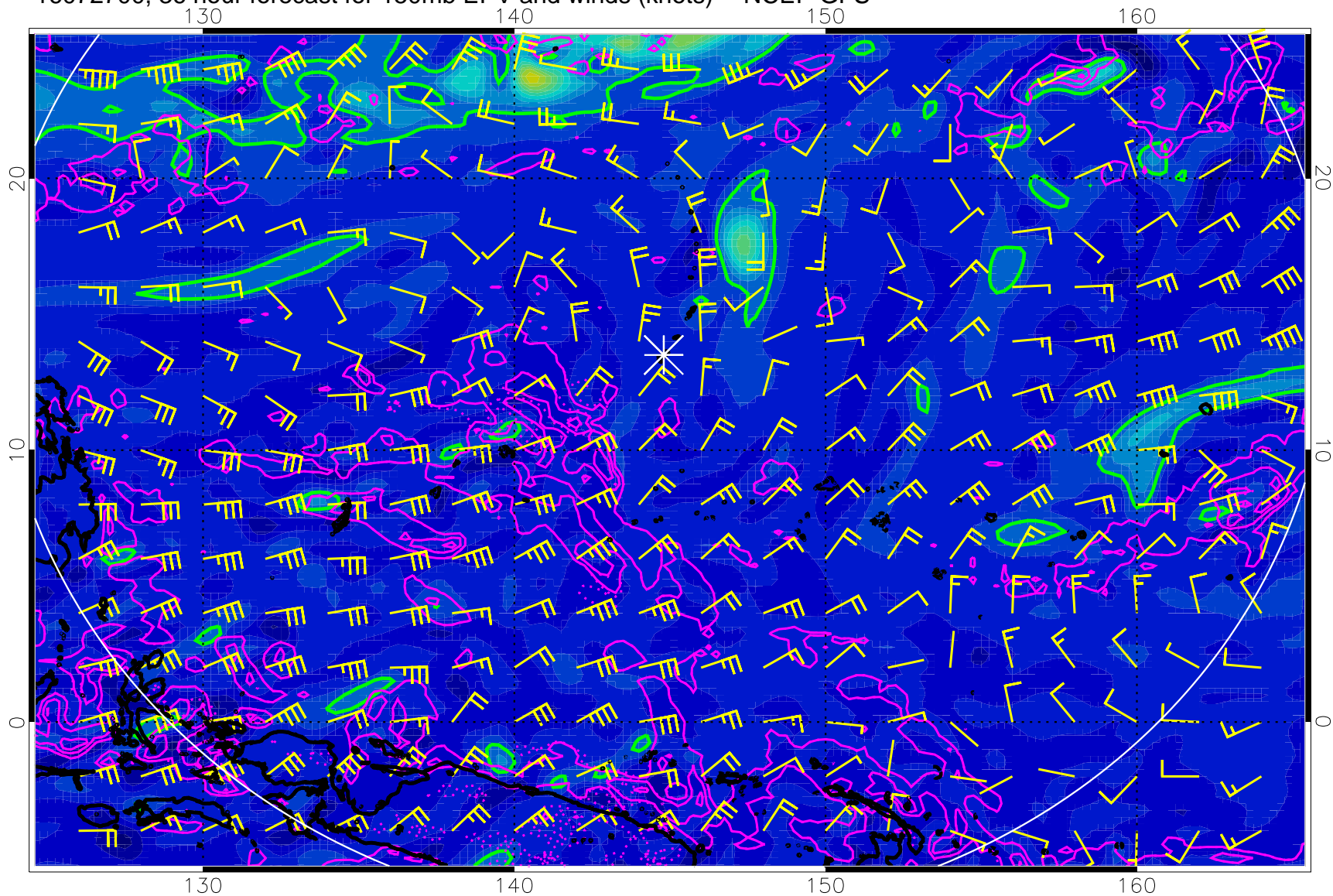
16072700, 36 hour forecast for 150mb EPV and winds (knots) -- NCEP GFS
