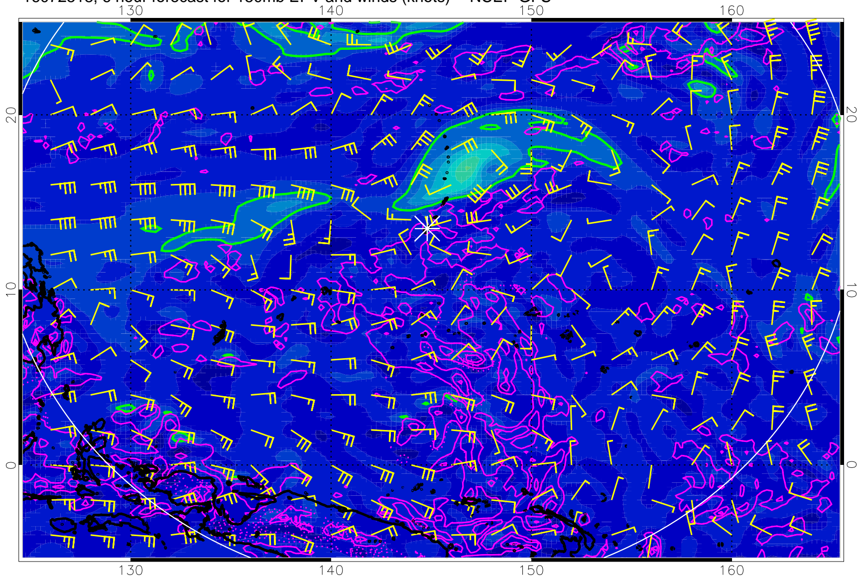
16072518, 6 hour forecast for 150mb EPV and winds (knots) -- NCEP GFS
