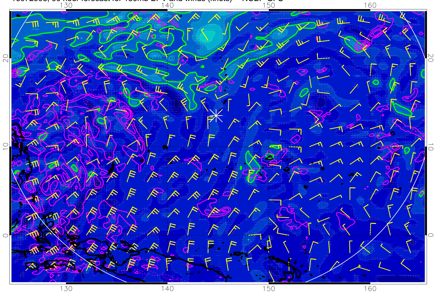
16072906, 90 hour forecast for 150mb EPV and winds (knots) -- NCEP GFS
