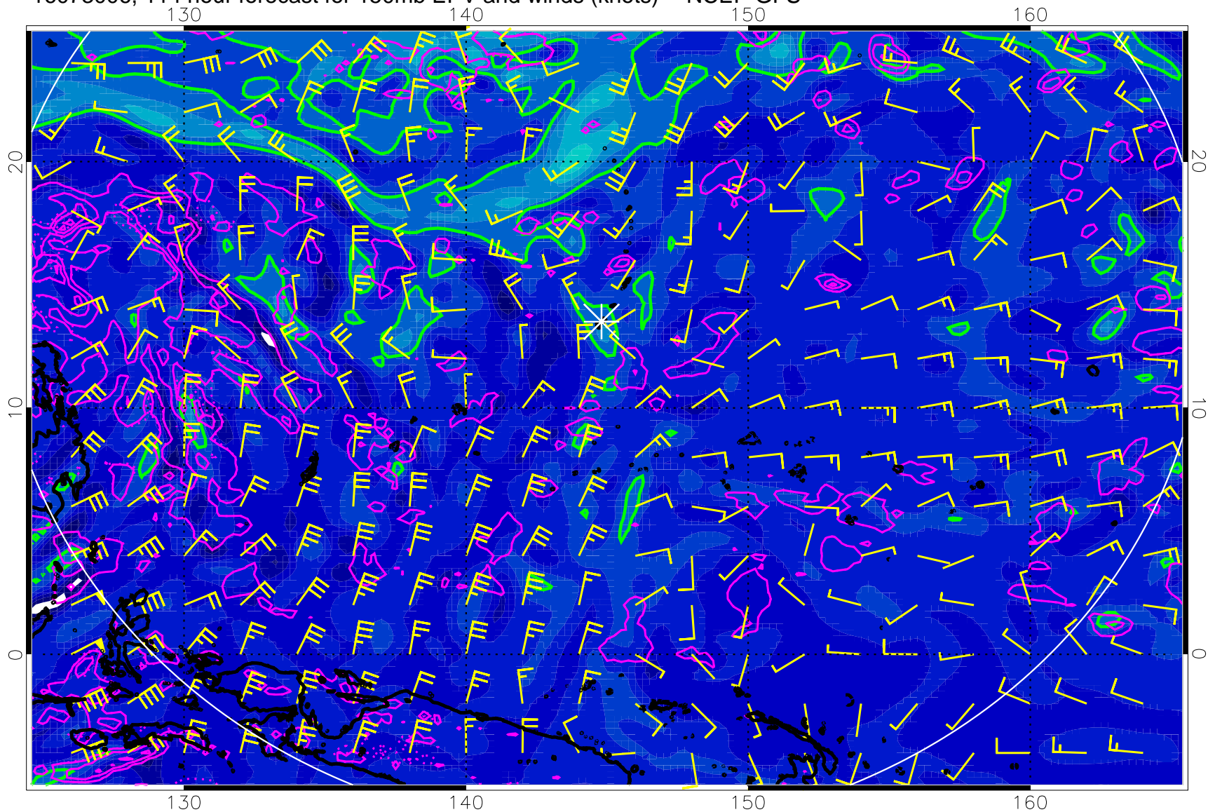
16073006, 114 hour forecast for 150mb EPV and winds (knots) -- NCEP GFS
