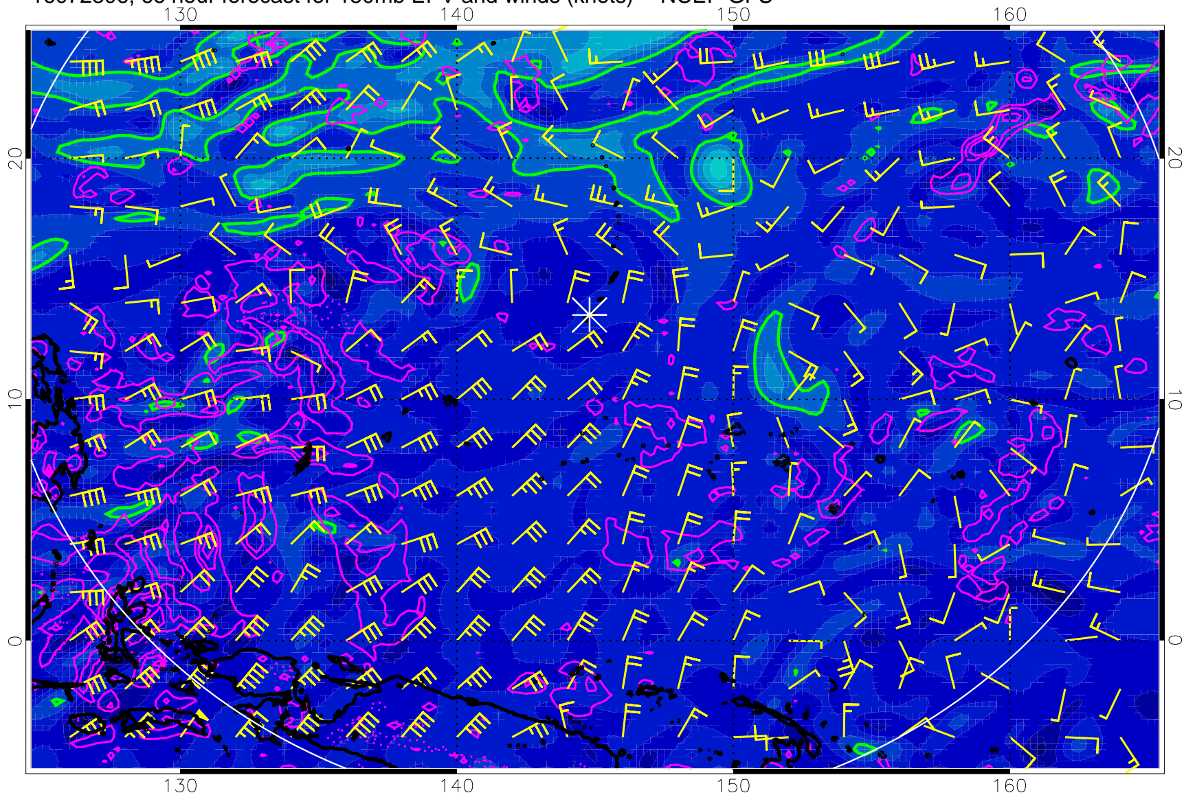
16072806, 66 hour forecast for 150mb EPV and winds (knots) -- NCEP GFS
