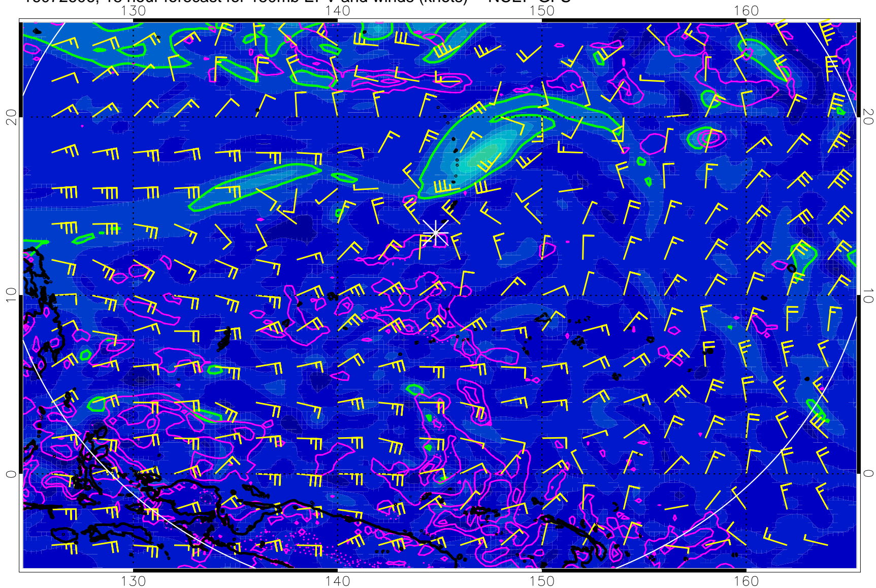
16072606, 18 hour forecast for 150mb EPV and winds (knots) -- NCEP GFS
