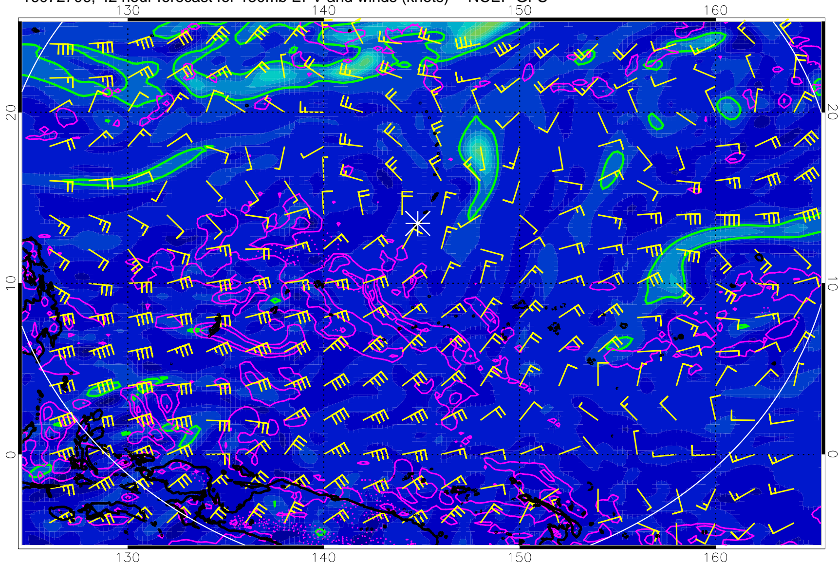
16072706, 42 hour forecast for 150mb EPV and winds (knots) -- NCEP GFS
