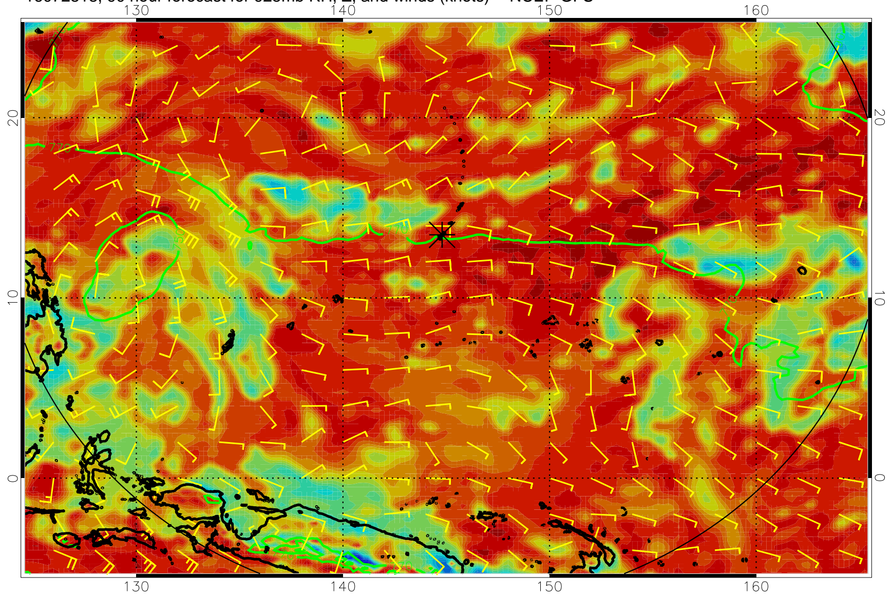
16072818, 90 hour forecast for 925mb RH, Z, and winds (knots) -- NCEP GFS
