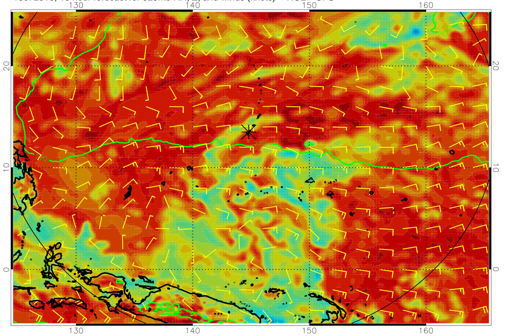
16072518, 18 hour forecast for 925mb RH, Z, and winds (knots) -- NCEP GFS
