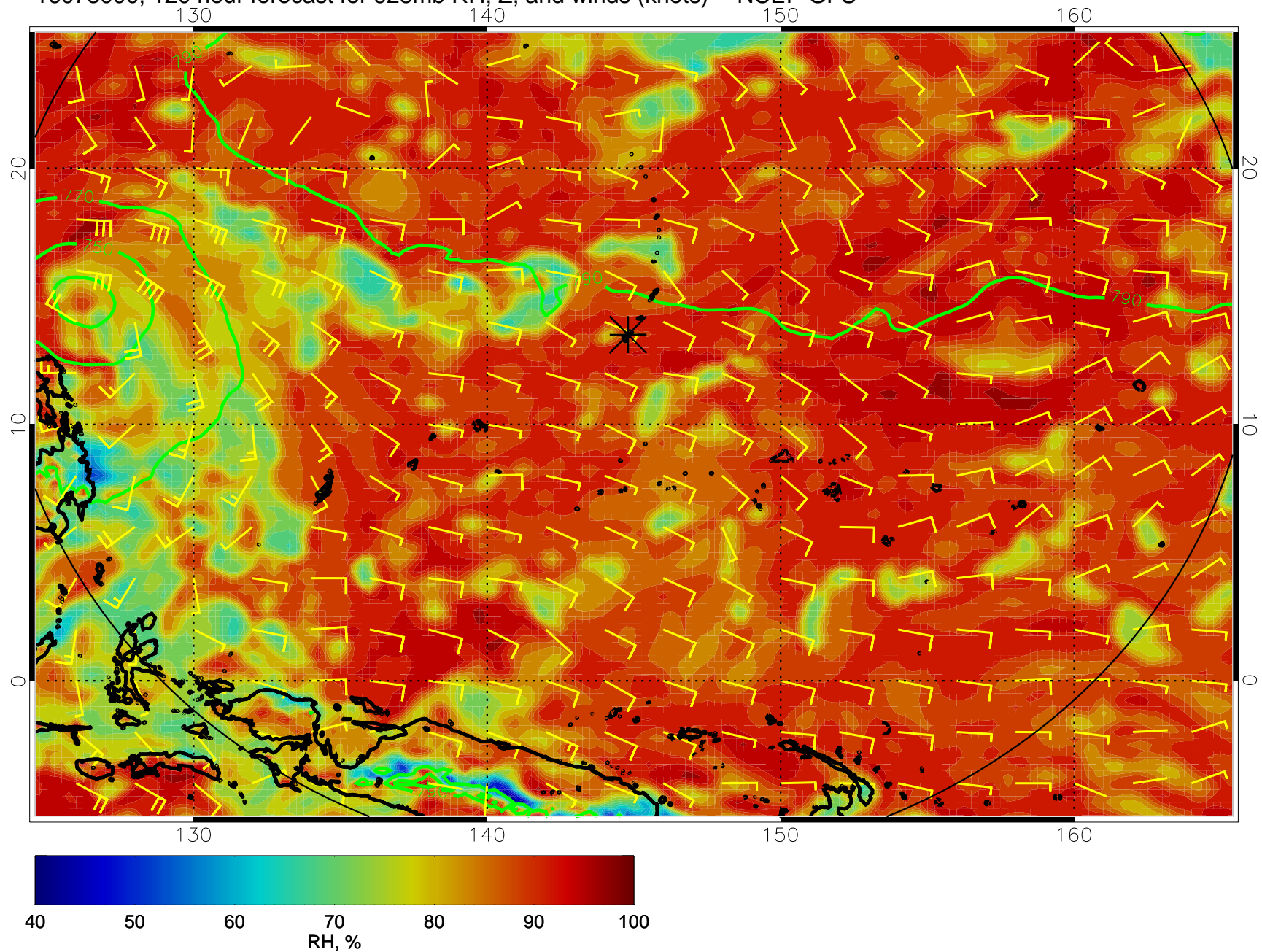
16073000, 120 hour forecast for 925mb RH, Z, and winds (knots) -- NCEP GFS
