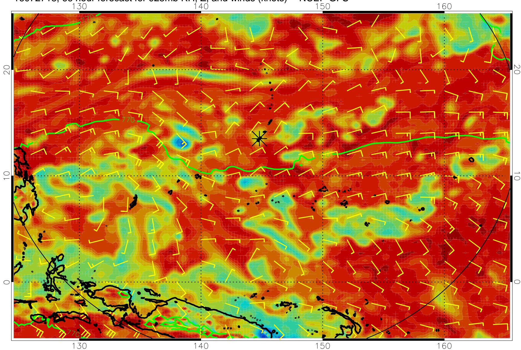
16072718, 66 hour forecast for 925mb RH, Z, and winds (knots) -- NCEP GFS
