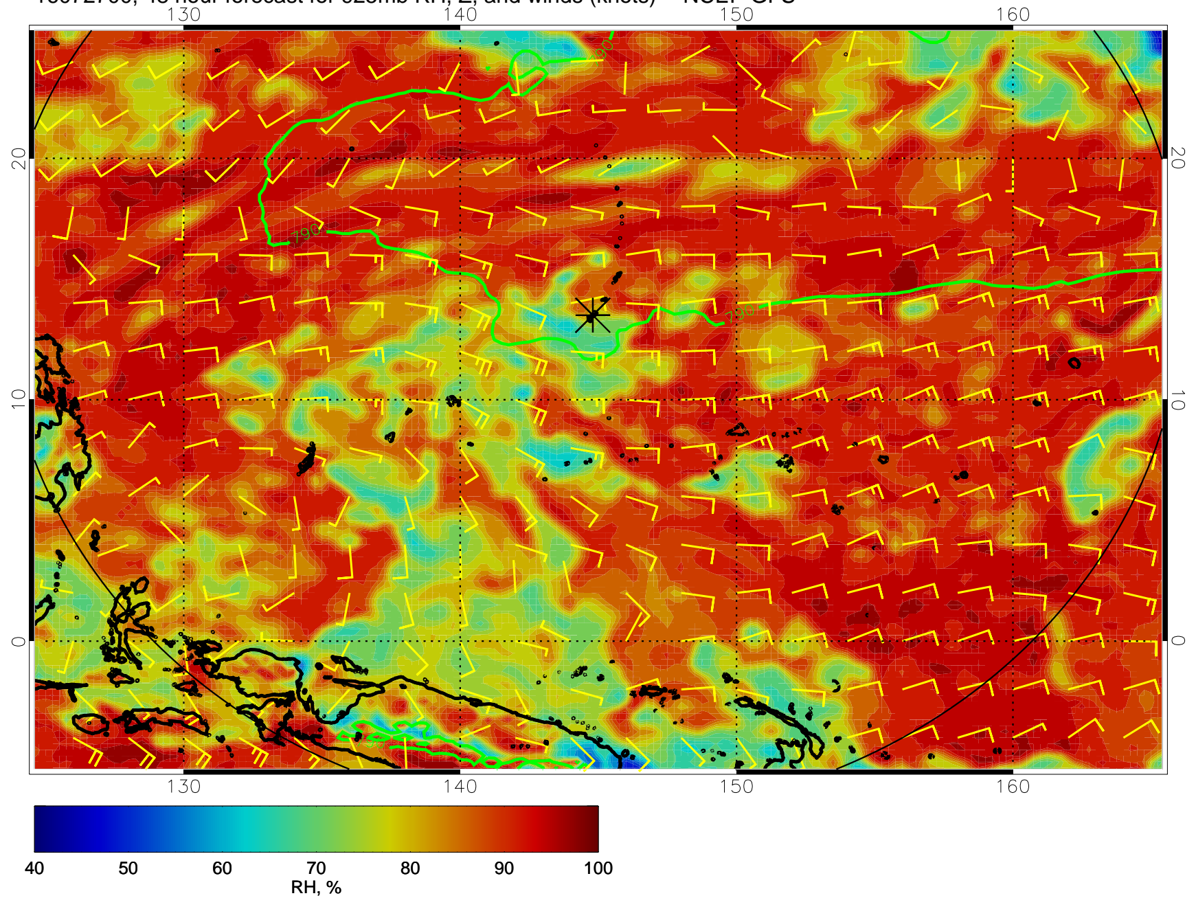
16072700, 48 hour forecast for 925mb RH, Z, and winds (knots) -- NCEP GFS
