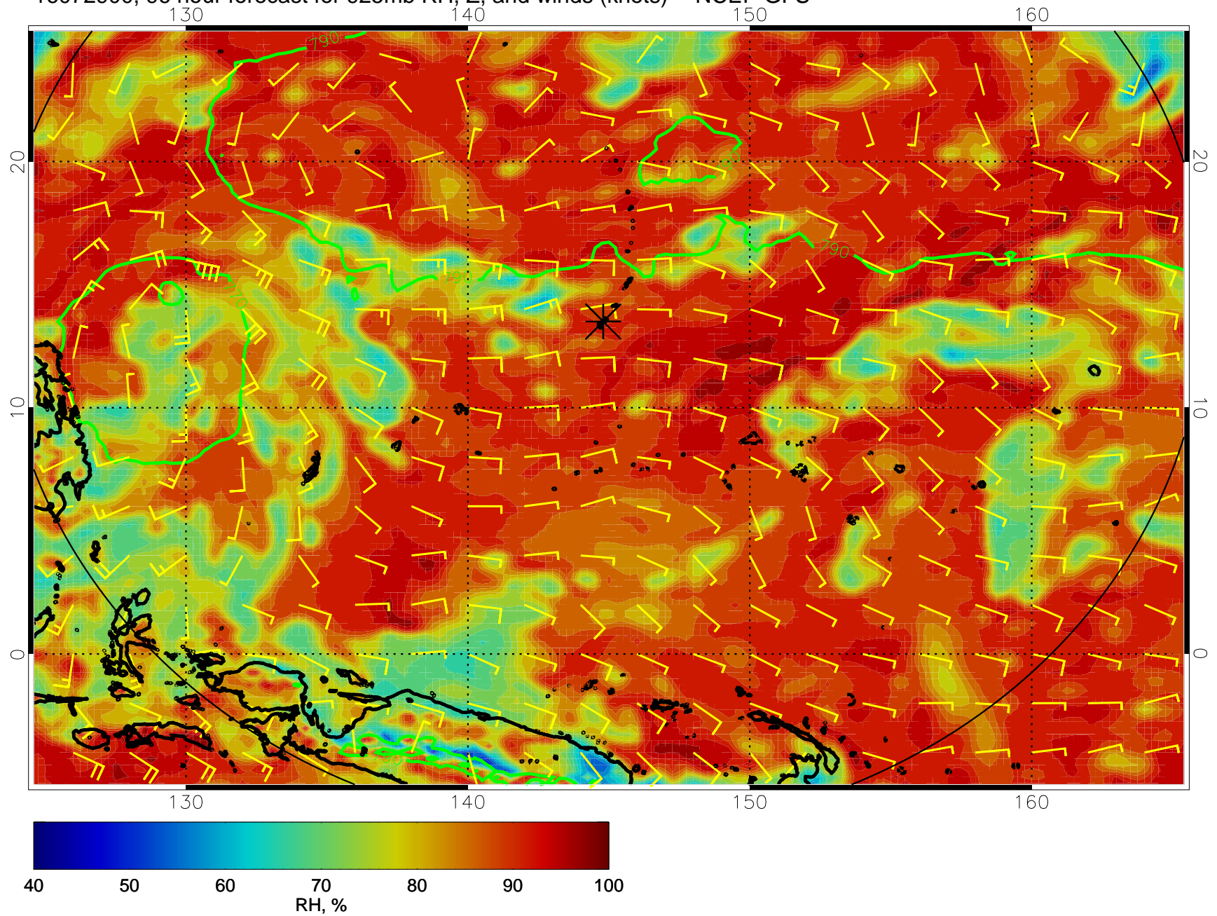
16072900, 96 hour forecast for 925mb RH, Z, and winds (knots) -- NCEP GFS
