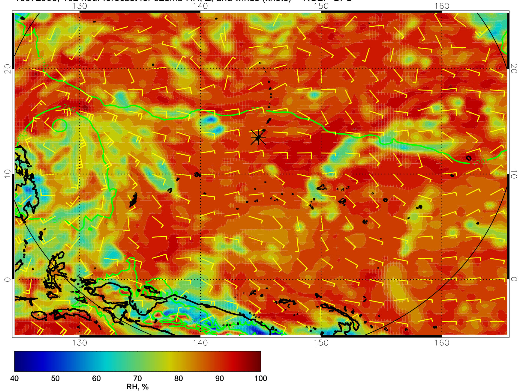
16072906, 102 hour forecast for 925mb RH, Z, and winds (knots) -- NCEP GFS
