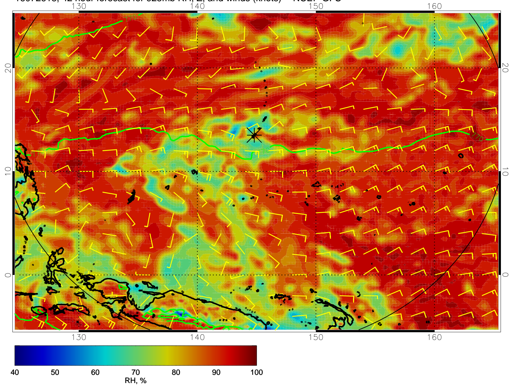
16072618, 42 hour forecast for 925mb RH, Z, and winds (knots) -- NCEP GFS
