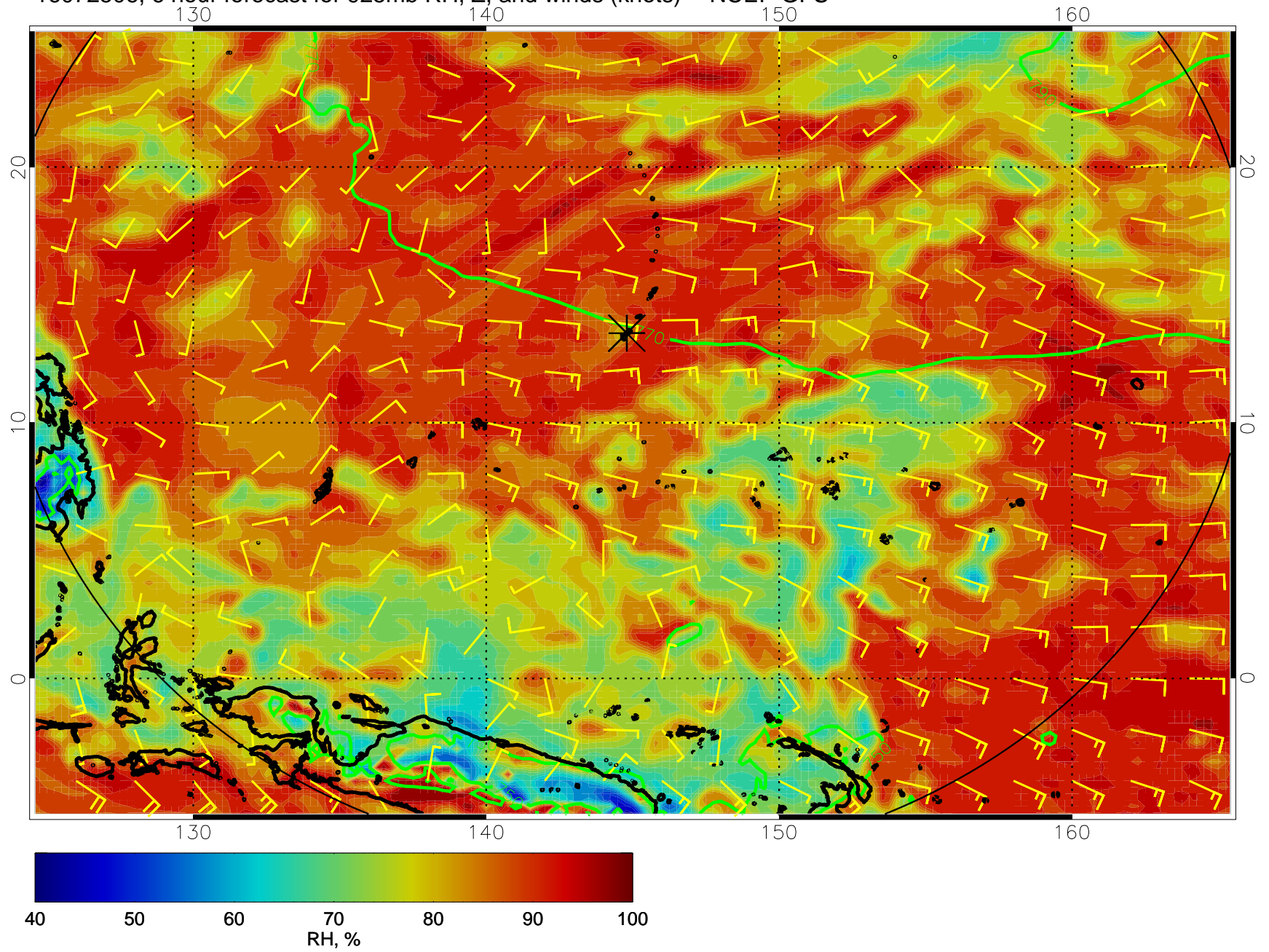
16072506, 6 hour forecast for 925mb RH, Z, and winds (knots) -- NCEP GFS
