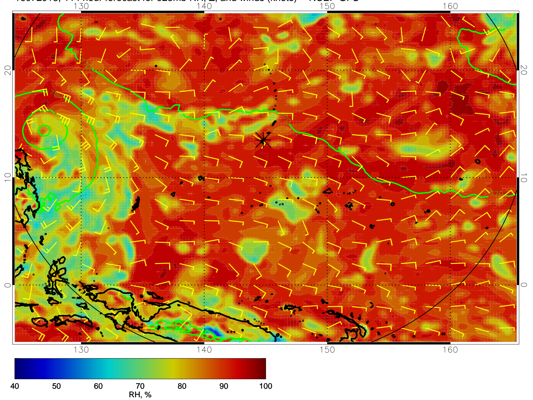
16072918, 114 hour forecast for 925mb RH, Z, and winds (knots) -- NCEP GFS
