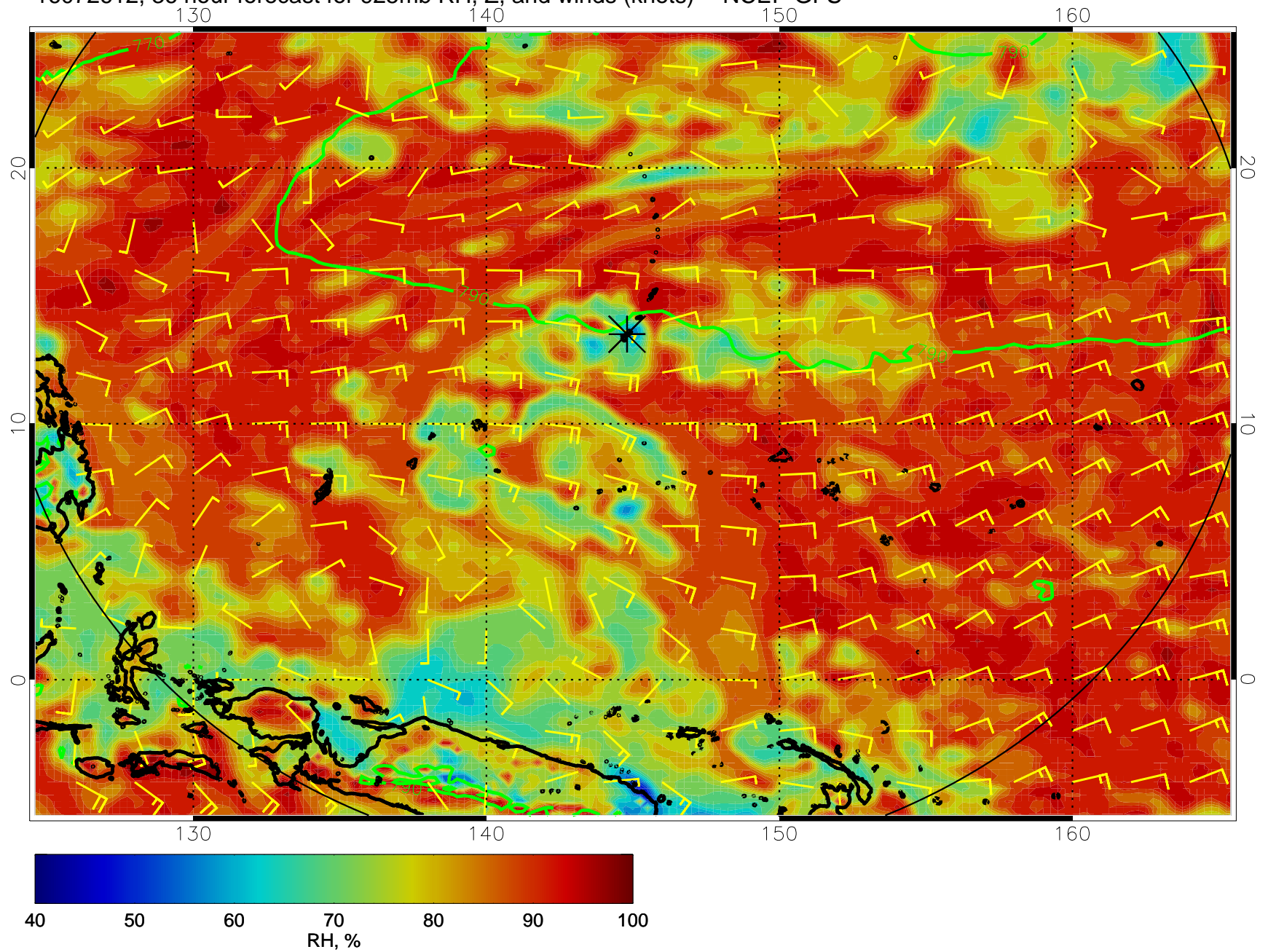
16072612, 36 hour forecast for 925mb RH, Z, and winds (knots) -- NCEP GFS
