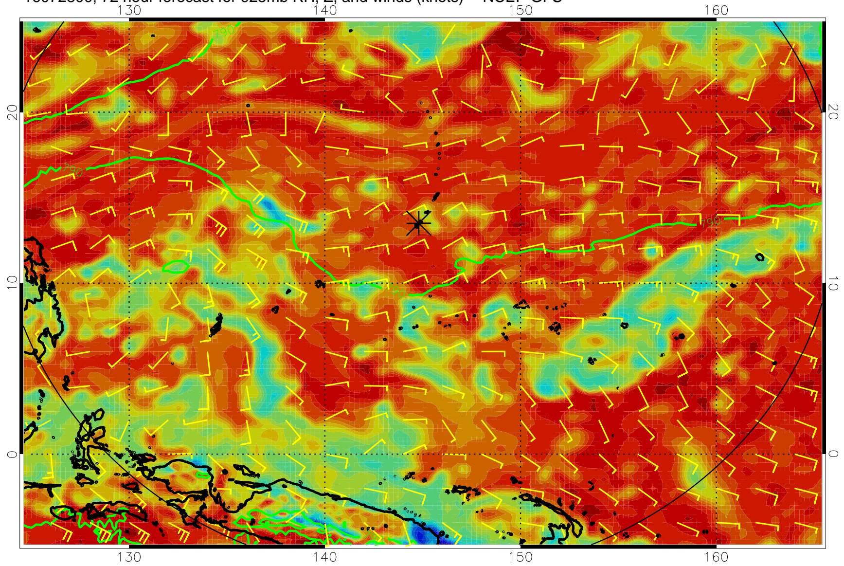
16072800, 72 hour forecast for 925mb RH, Z, and winds (knots) -- NCEP GFS
