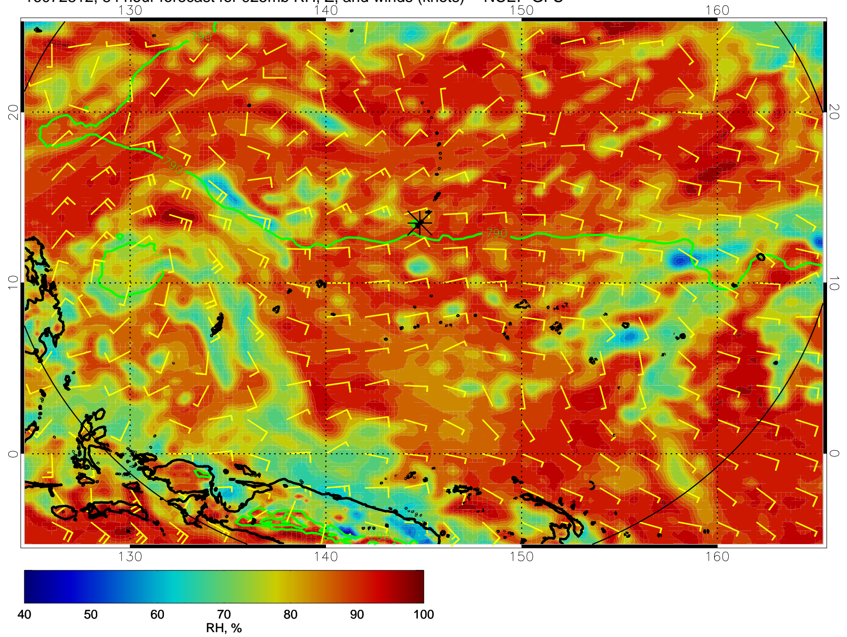
16072812, 84 hour forecast for 925mb RH, Z, and winds (knots) -- NCEP GFS
