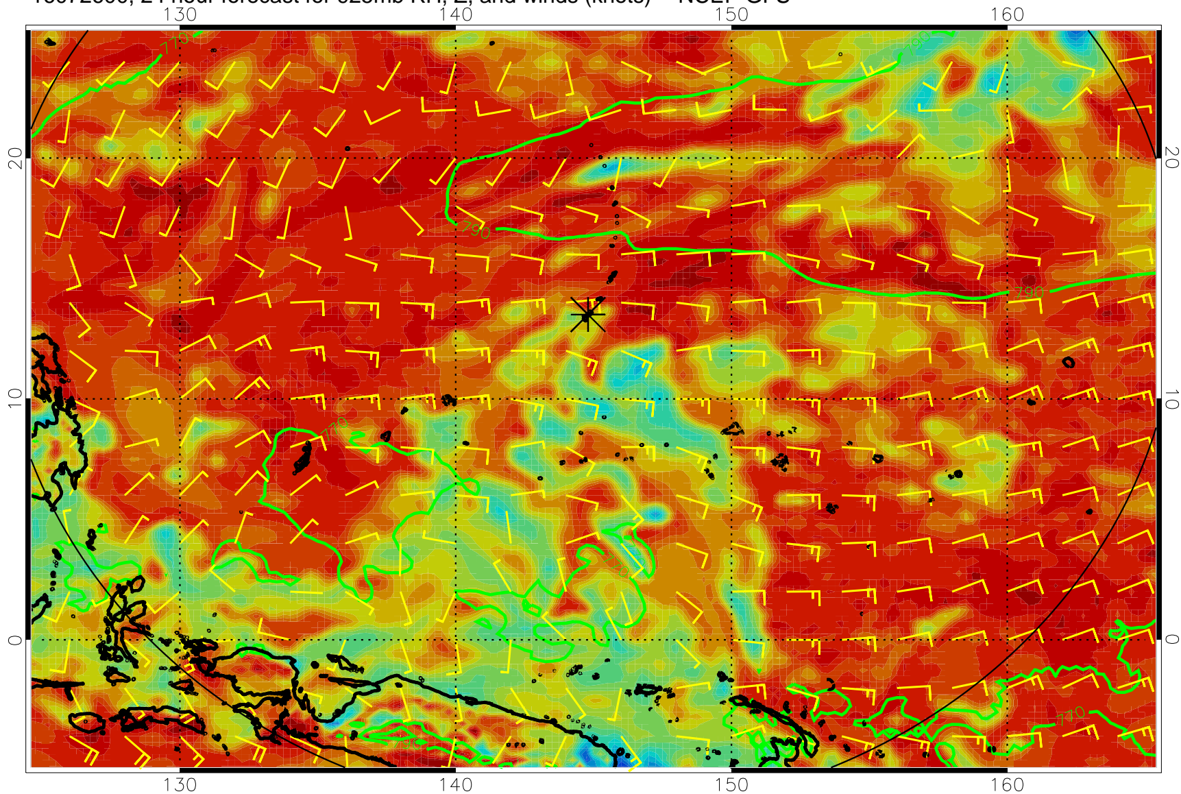
16072600, 24 hour forecast for 925mb RH, Z, and winds (knots) -- NCEP GFS
