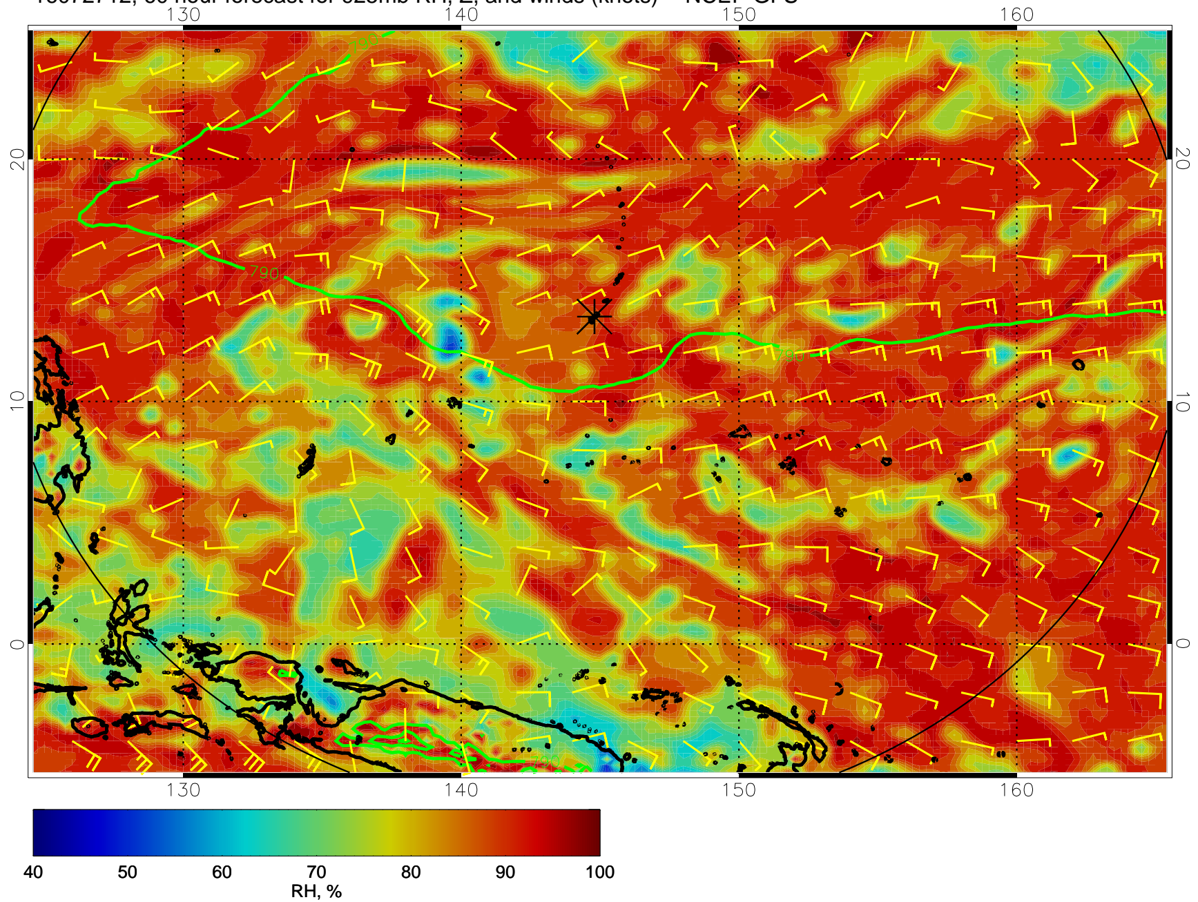
16072712, 60 hour forecast for 925mb RH, Z, and winds (knots) -- NCEP GFS
