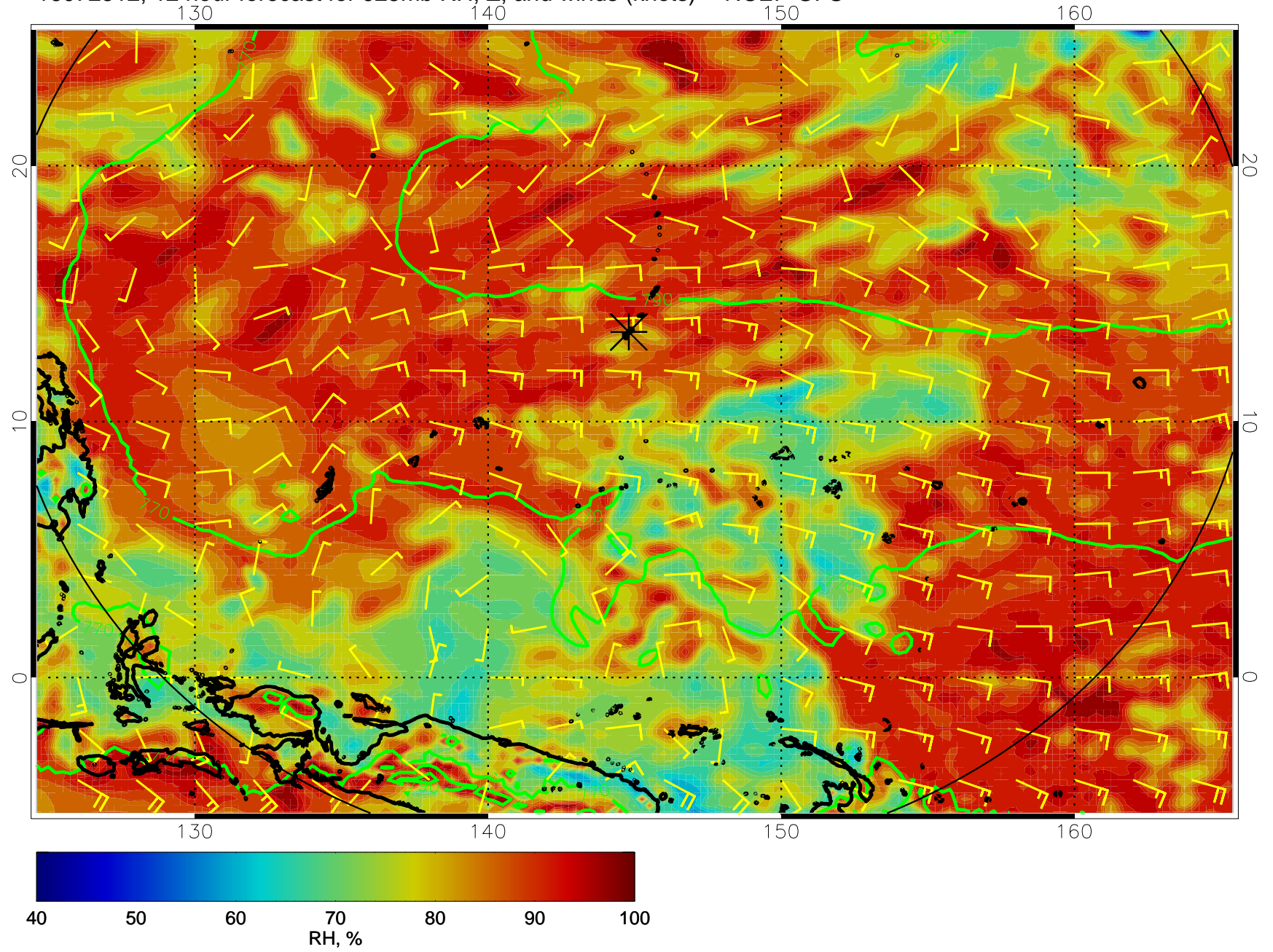
16072512, 12 hour forecast for 925mb RH, Z, and winds (knots) -- NCEP GFS
