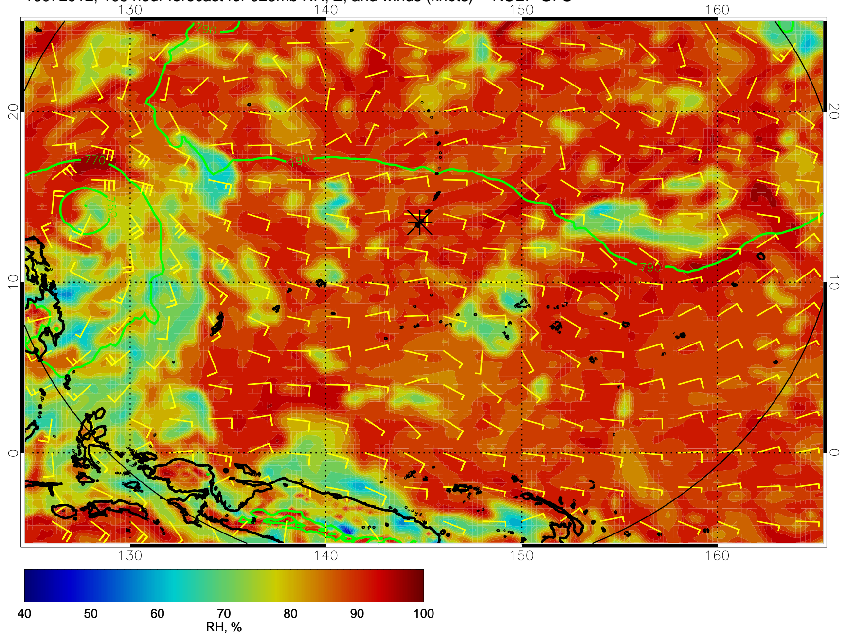
16072912, 108 hour forecast for 925mb RH, Z, and winds (knots) -- NCEP GFS
