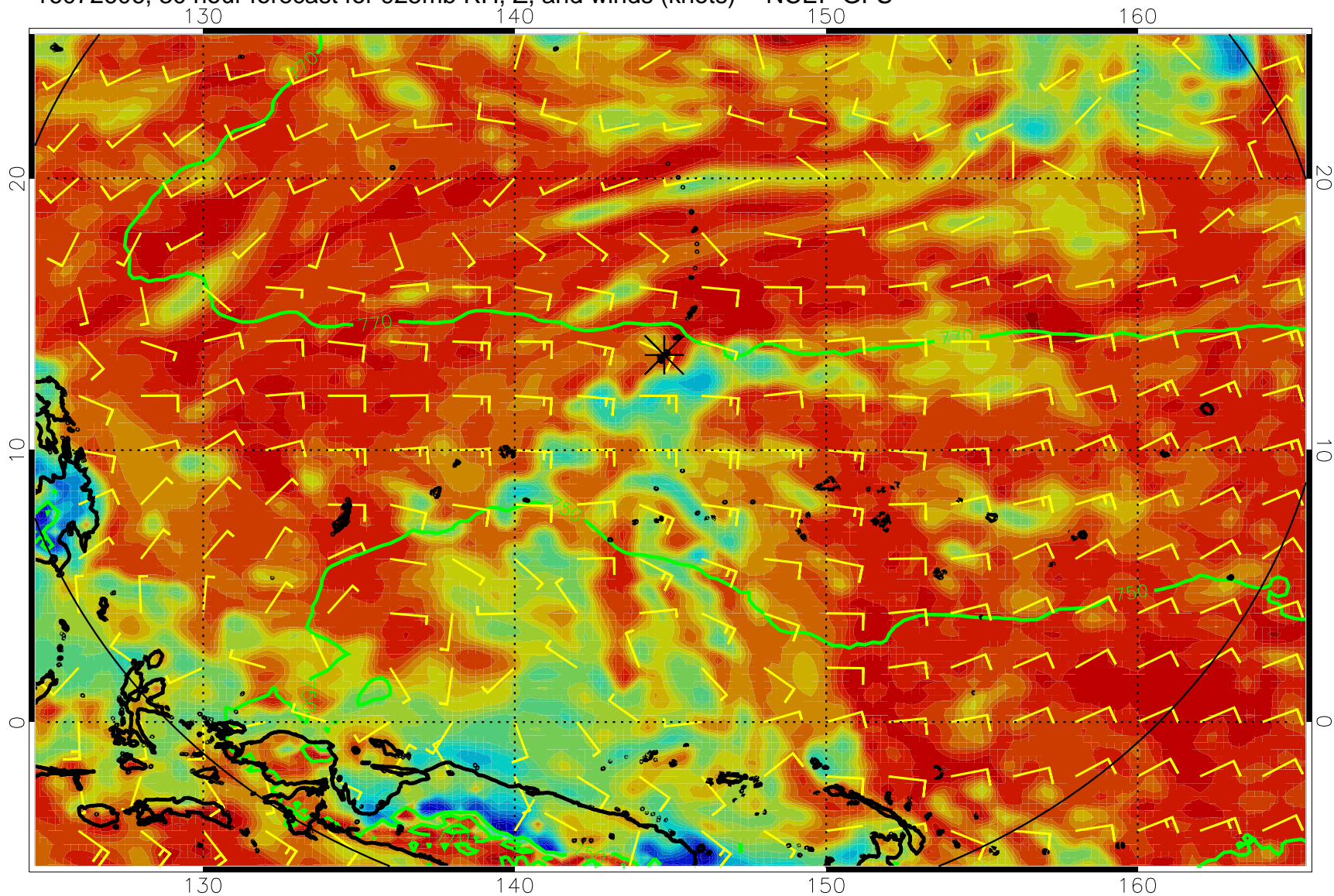
16072606, 30 hour forecast for 925mb RH, Z, and winds (knots) -- NCEP GFS
