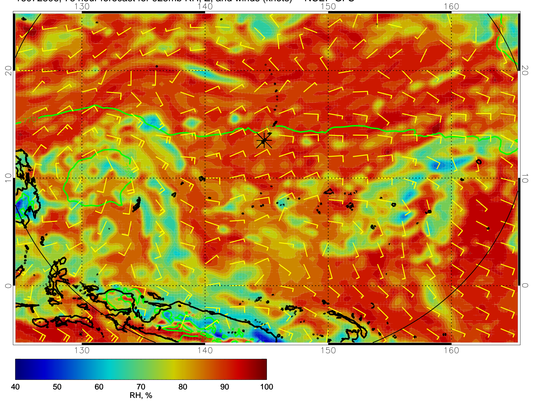
16072806, 78 hour forecast for 925mb RH, Z, and winds (knots) -- NCEP GFS
