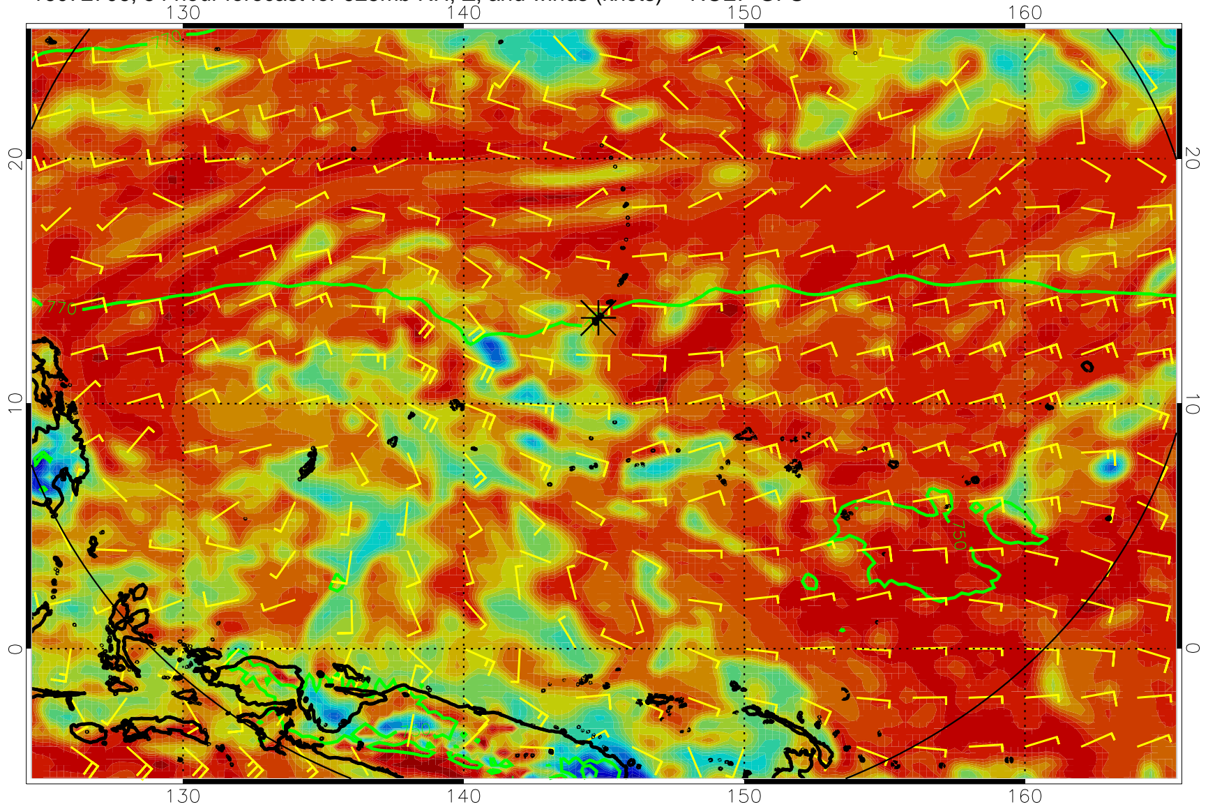
16072706, 54 hour forecast for 925mb RH, Z, and winds (knots) -- NCEP GFS
