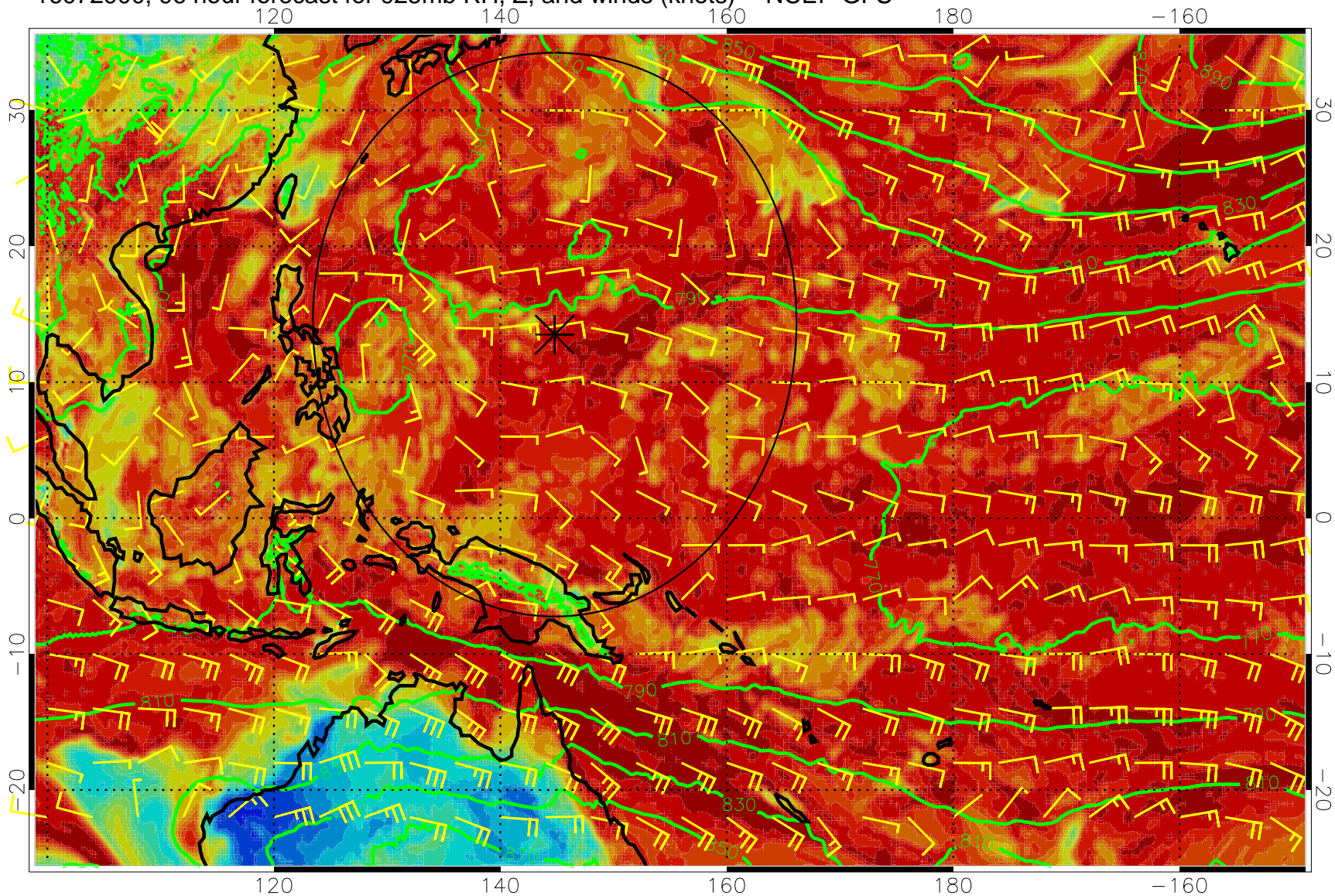
16072900, 96 hour forecast for 925mb RH, Z, and winds (knots) -- NCEP GFS
