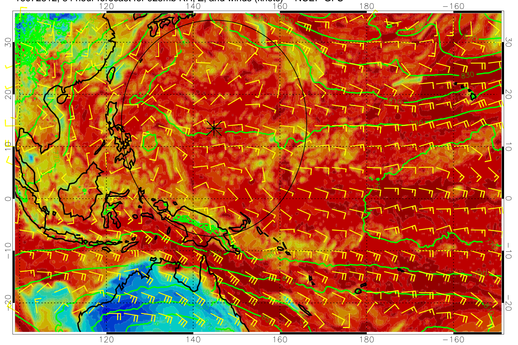
16072812, 84 hour forecast for 925mb RH, Z, and winds (knots) -- NCEP GFS
