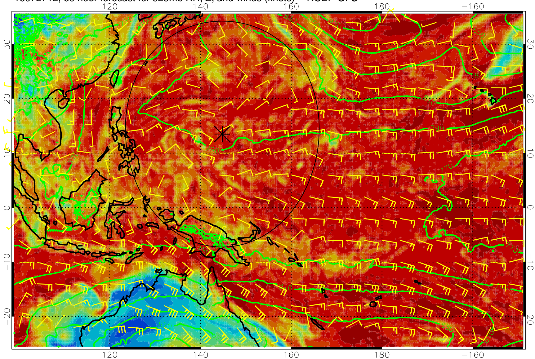
16072712, 60 hour forecast for 925mb RH, Z, and winds (knots) -- NCEP GFS
