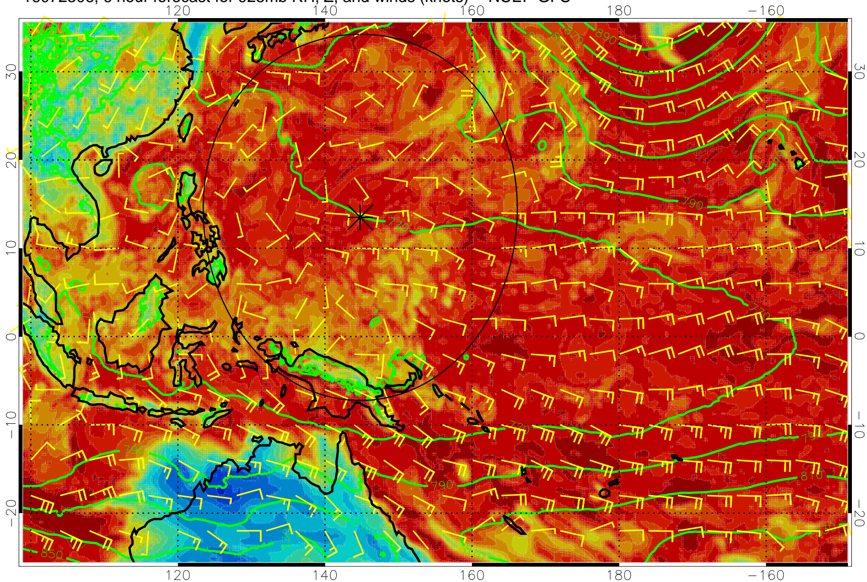
16072506, 6 hour forecast for 925mb RH, Z, and winds (knots) -- NCEP GFS
