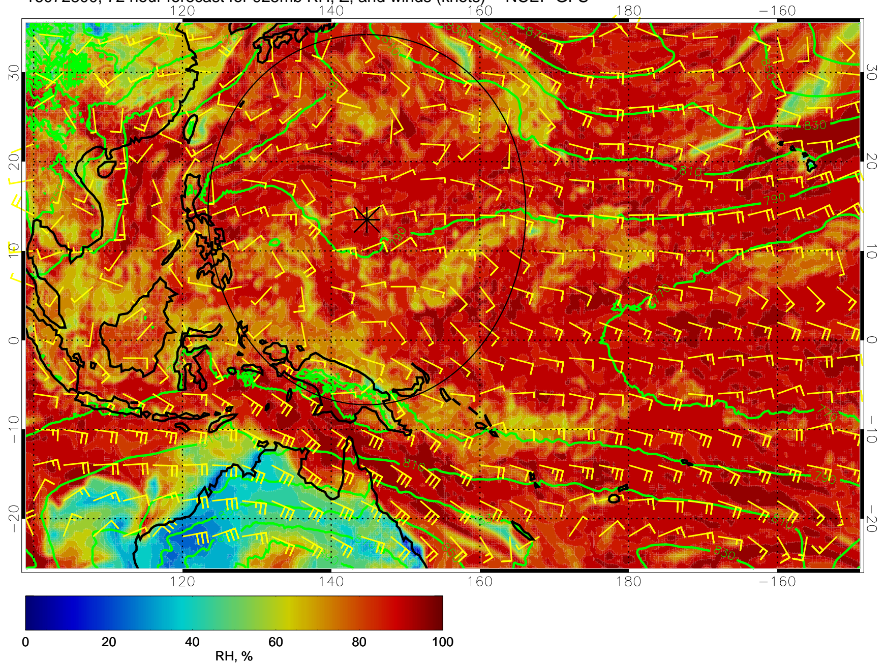
16072800, 72 hour forecast for 925mb RH, Z, and winds (knots) -- NCEP GFS
