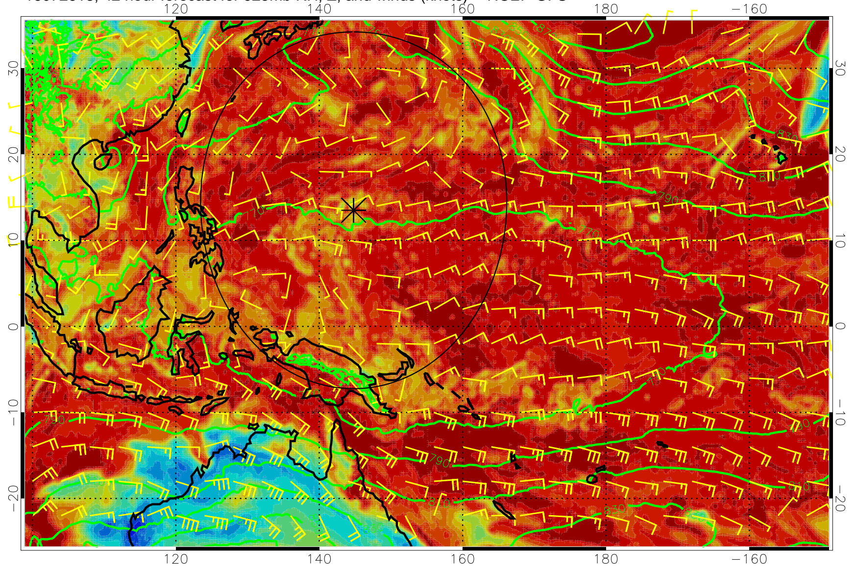
16072618, 42 hour forecast for 925mb RH, Z, and winds (knots) -- NCEP GFS
