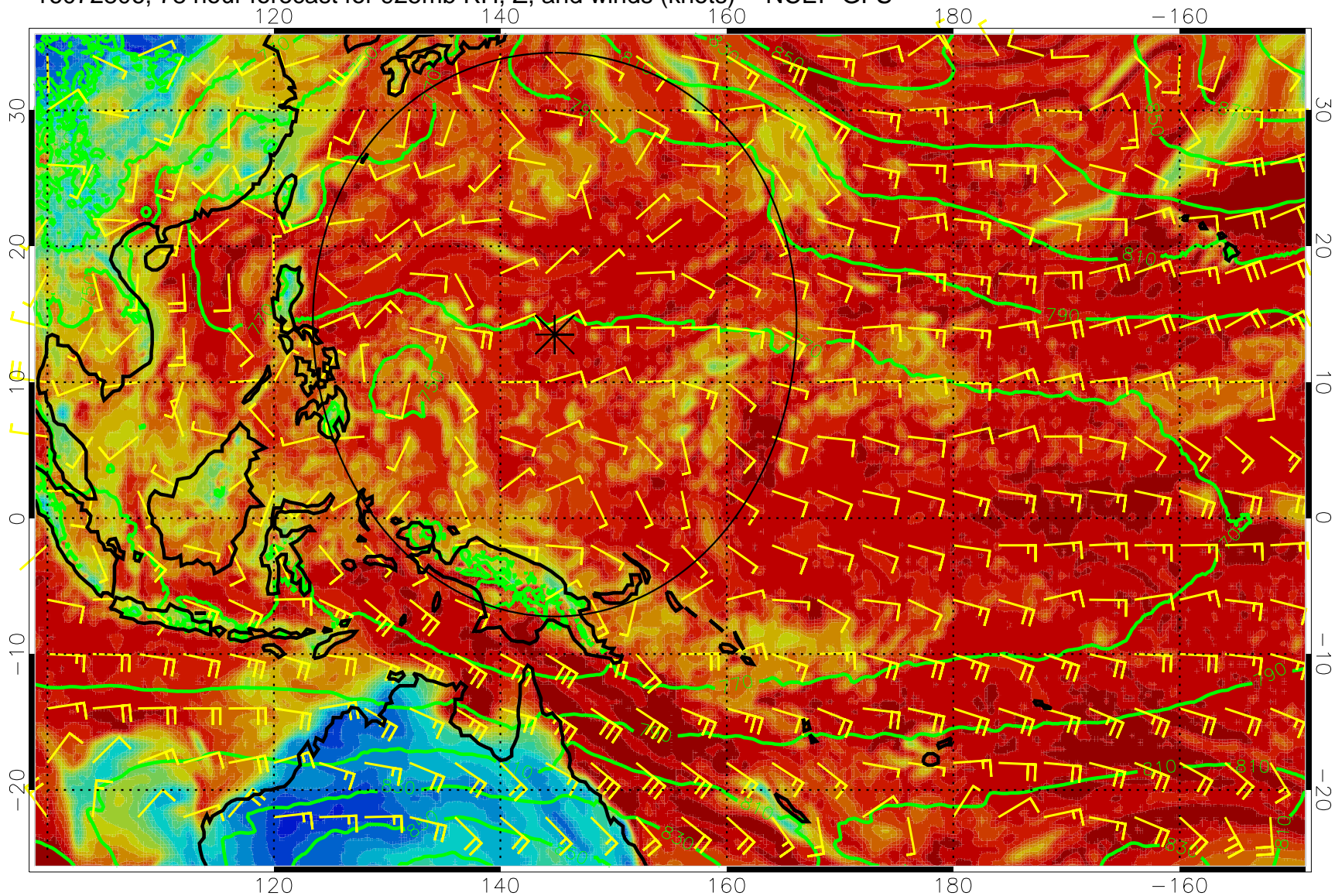
16072806, 78 hour forecast for 925mb RH, Z, and winds (knots) -- NCEP GFS
