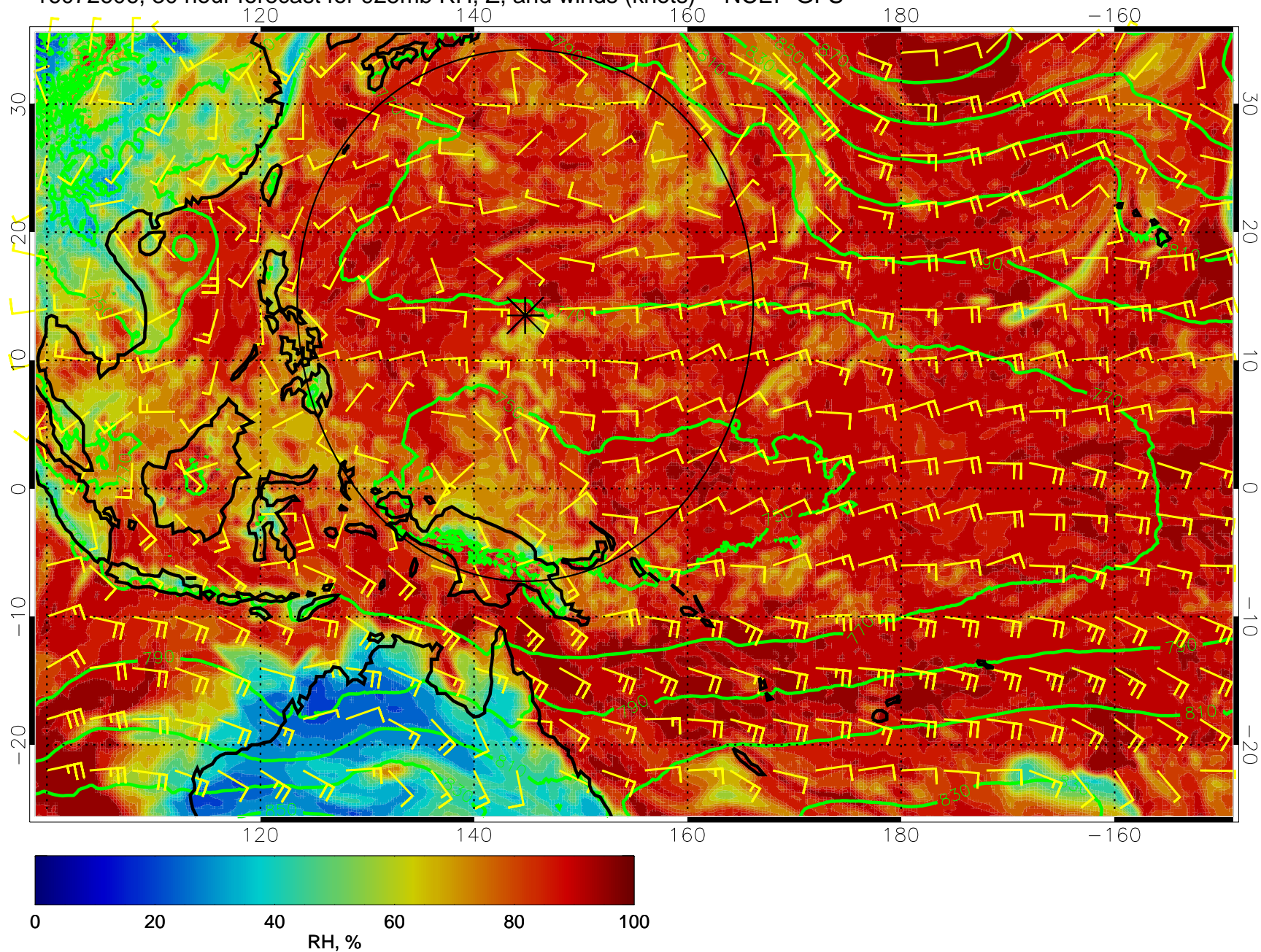
16072606, 30 hour forecast for 925mb RH, Z, and winds (knots) -- NCEP GFS
