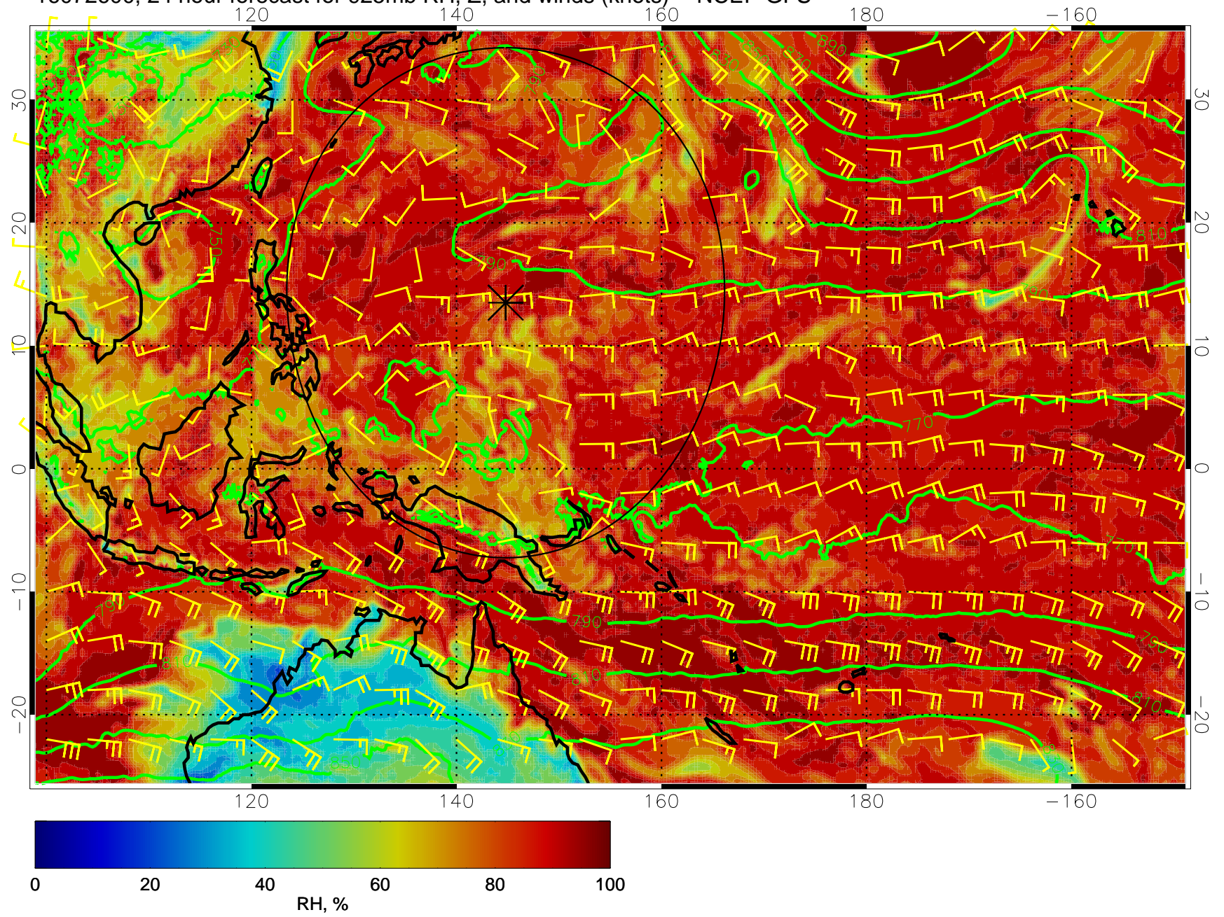
16072600, 24 hour forecast for 925mb RH, Z, and winds (knots) -- NCEP GFS
