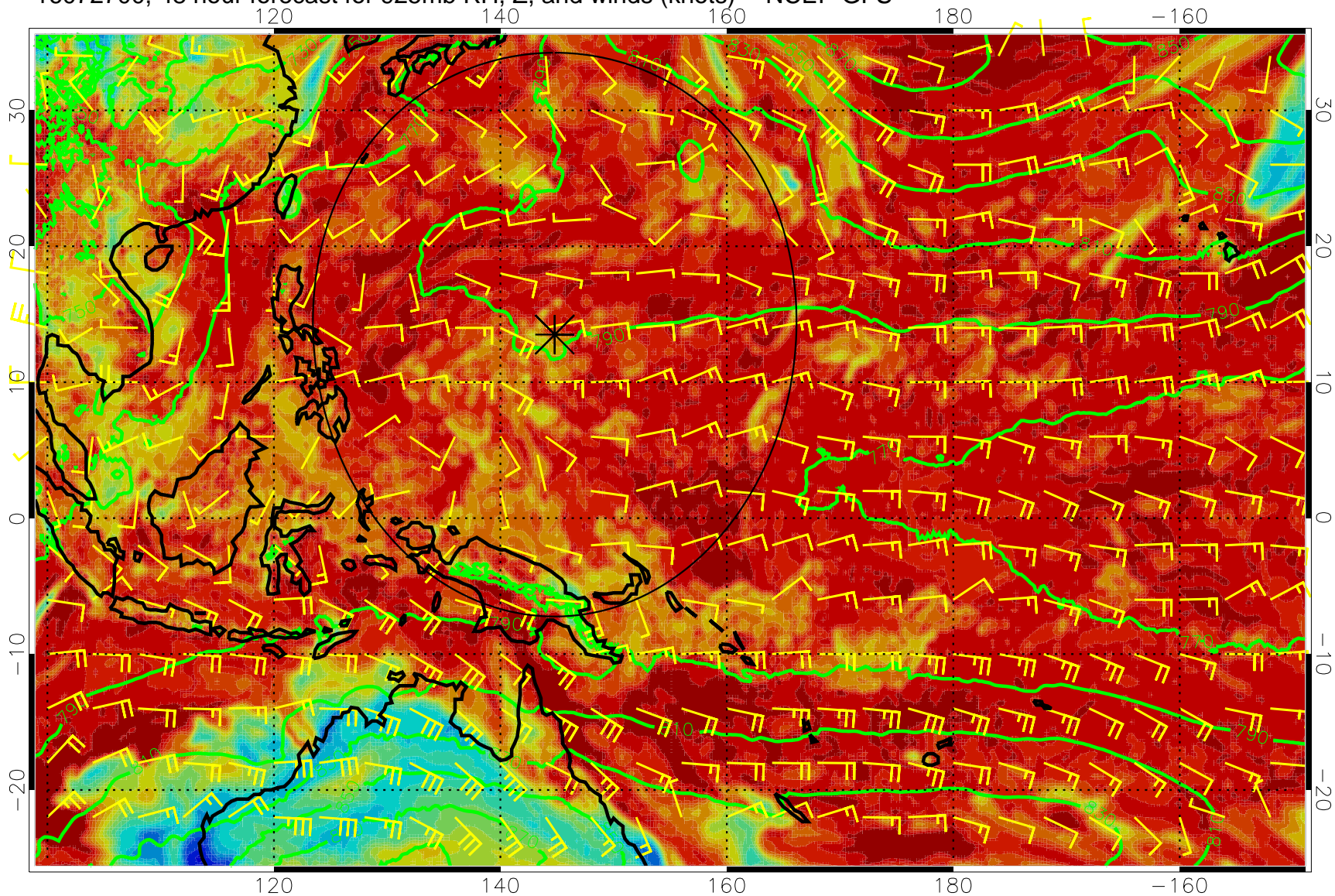
16072700, 48 hour forecast for 925mb RH, Z, and winds (knots) -- NCEP GFS
