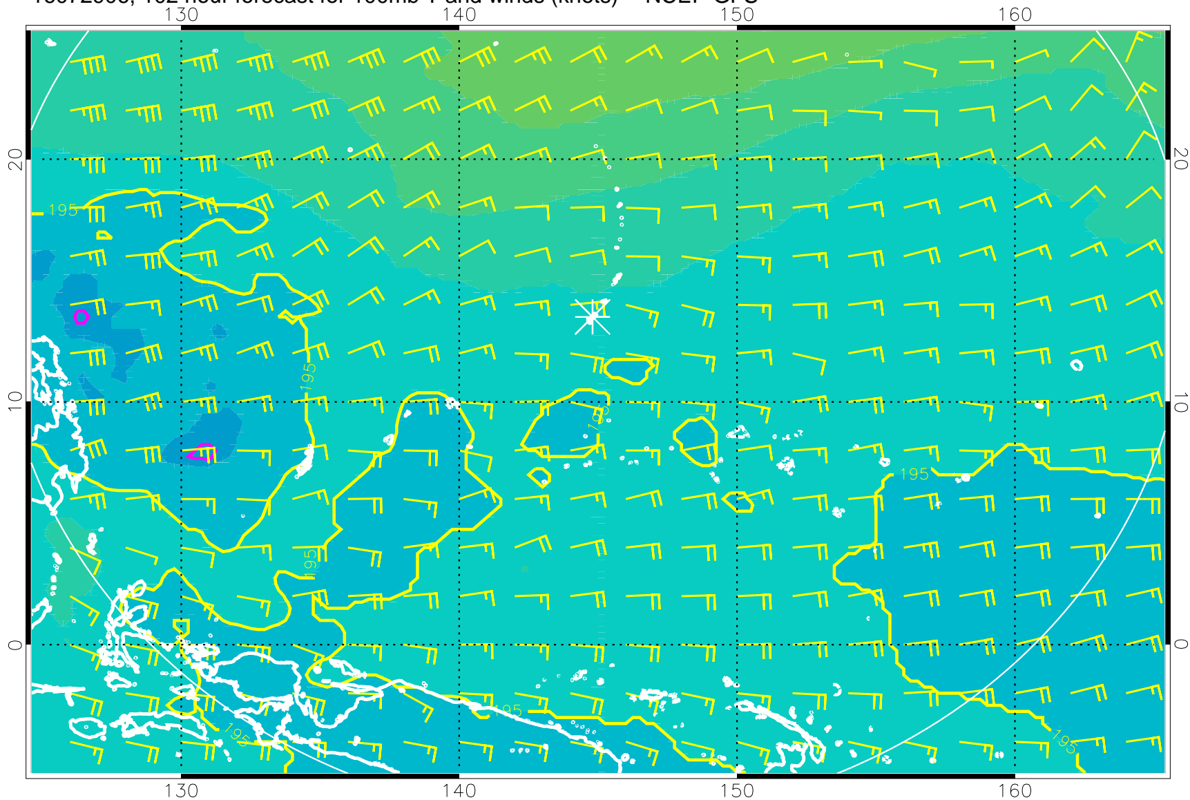
16072906, 102 hour forecast for 100mb T and winds (knots) -- NCEP GFS
