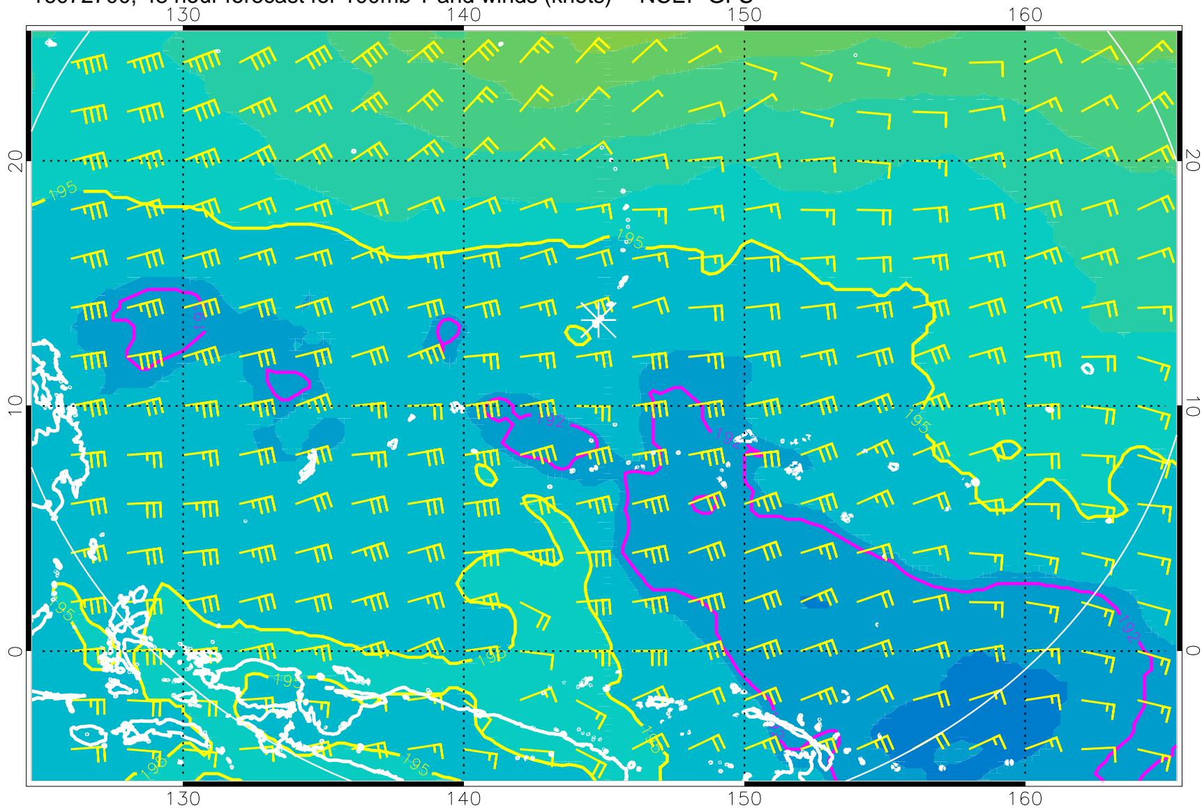
16072700, 48 hour forecast for 100mb T and winds (knots) -- NCEP GFS
