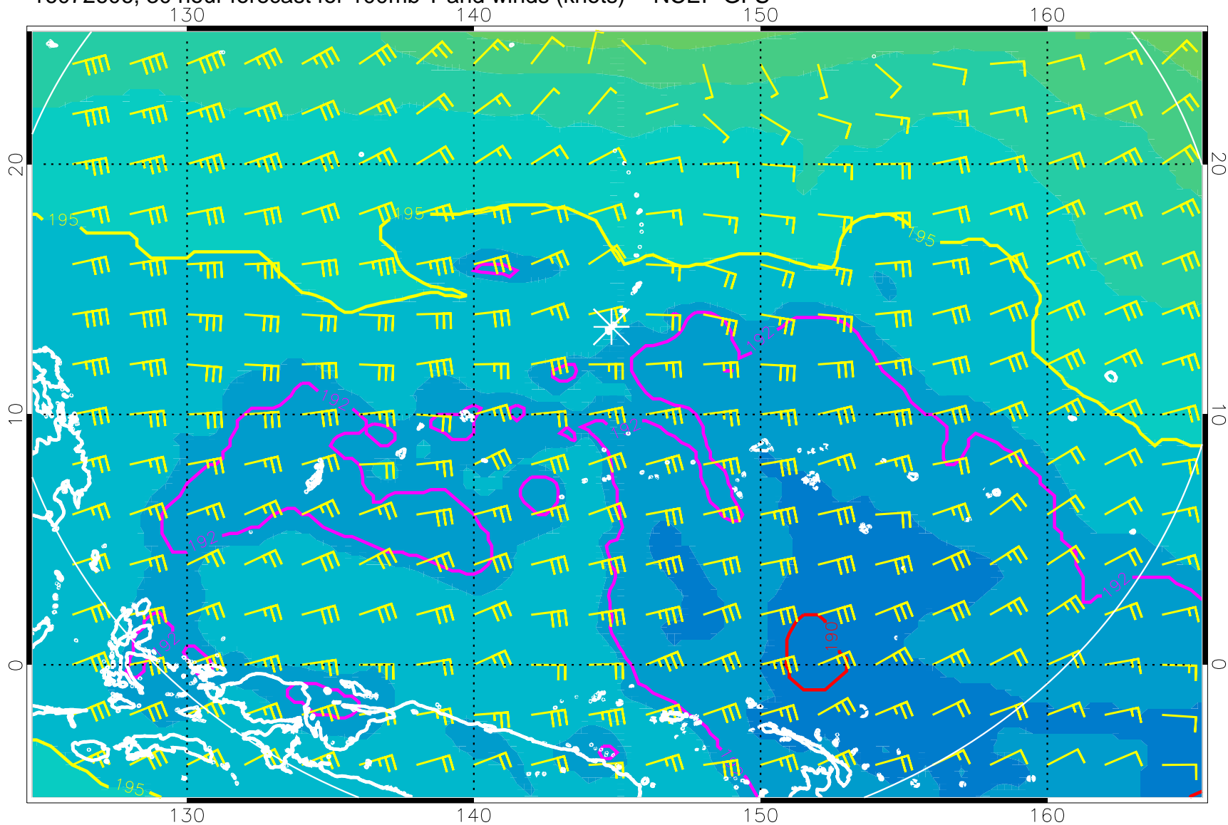
16072606, 30 hour forecast for 100mb T and winds (knots) -- NCEP GFS
