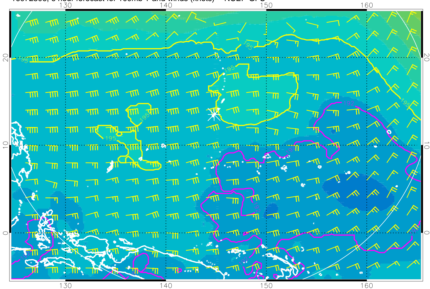
16072506, 6 hour forecast for 100mb T and winds (knots) -- NCEP GFS
