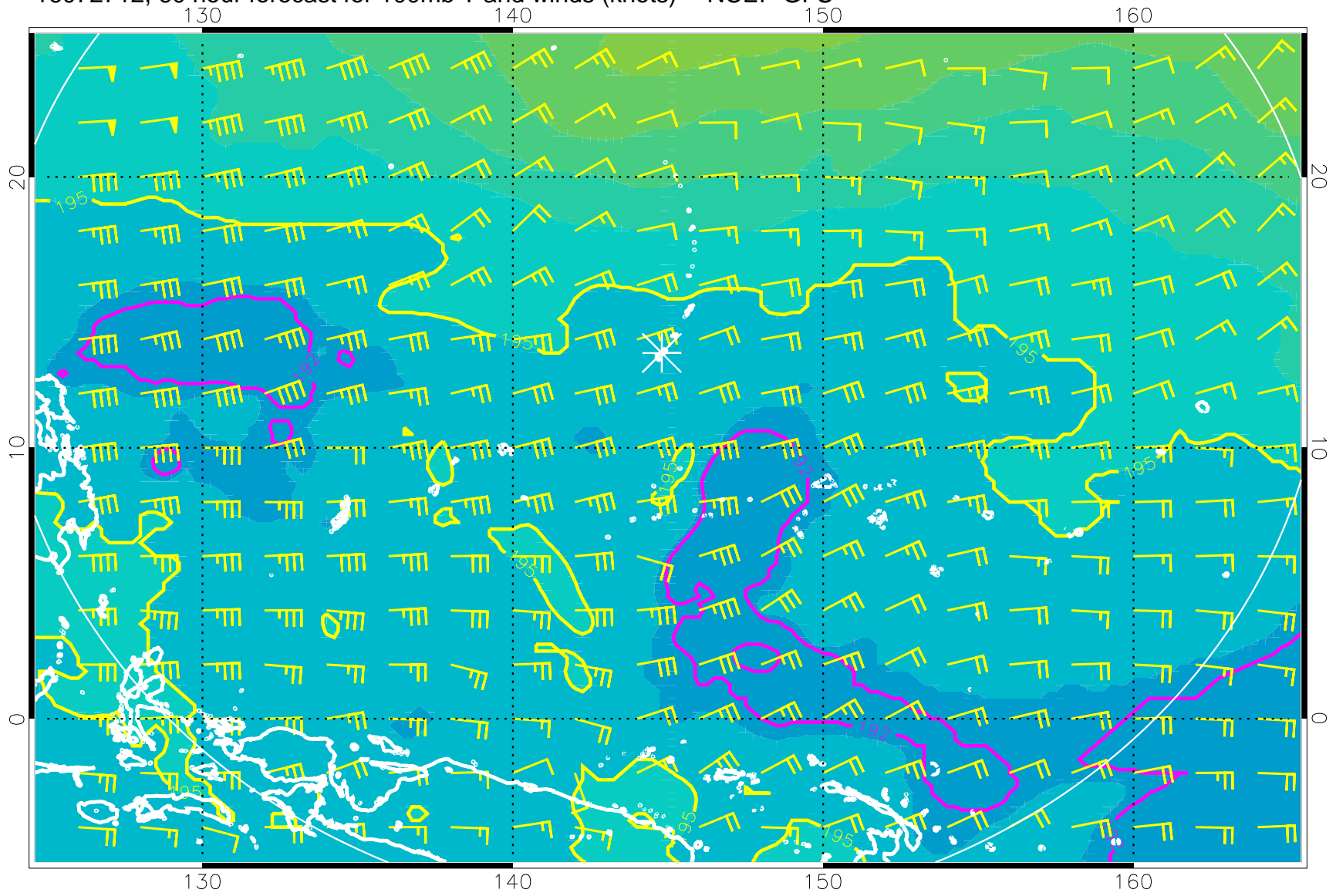
16072712, 60 hour forecast for 100mb T and winds (knots) -- NCEP GFS
