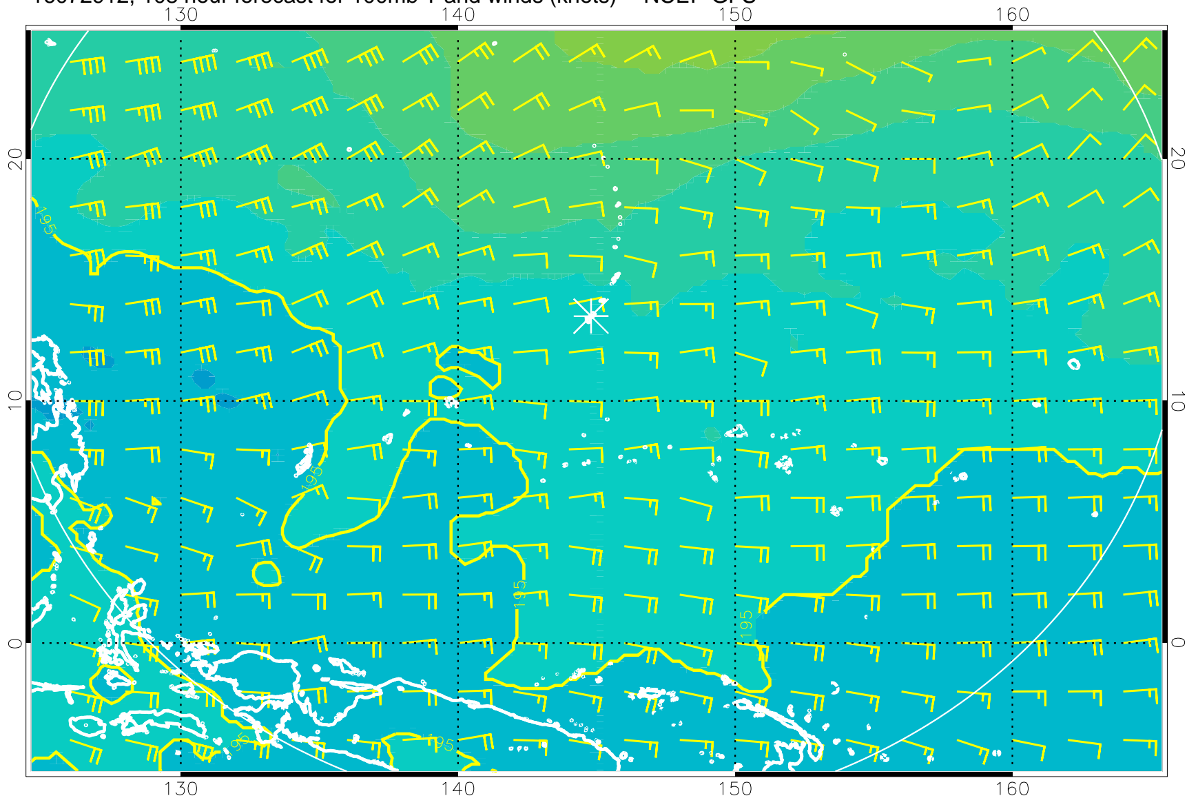
16072912, 108 hour forecast for 100mb T and winds (knots) -- NCEP GFS
