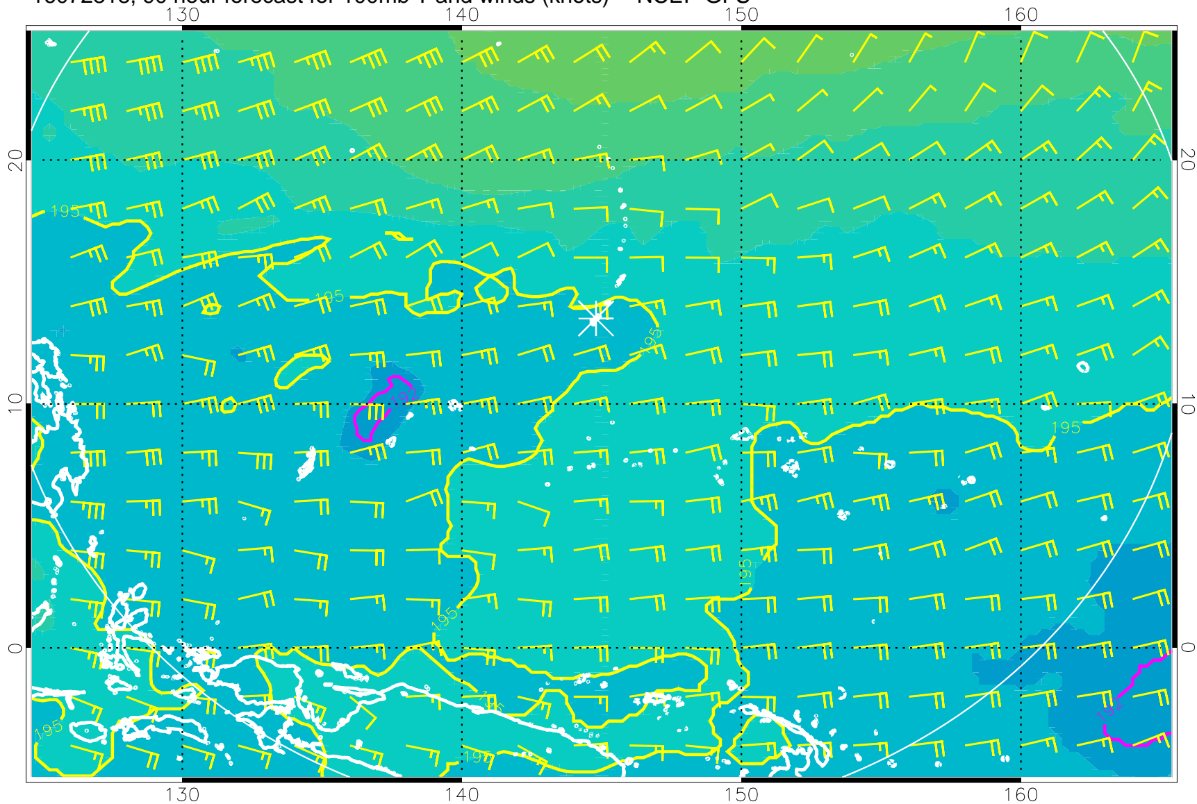
16072818, 90 hour forecast for 100mb T and winds (knots) -- NCEP GFS
