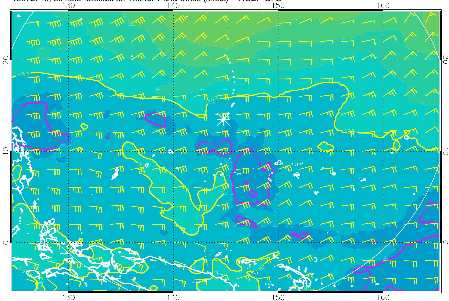
16072718, 66 hour forecast for 100mb T and winds (knots) -- NCEP GFS
