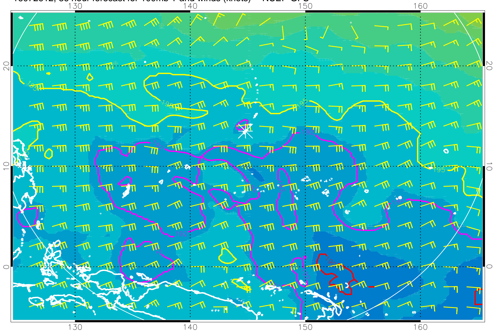
16072612, 36 hour forecast for 100mb T and winds (knots) -- NCEP GFS
