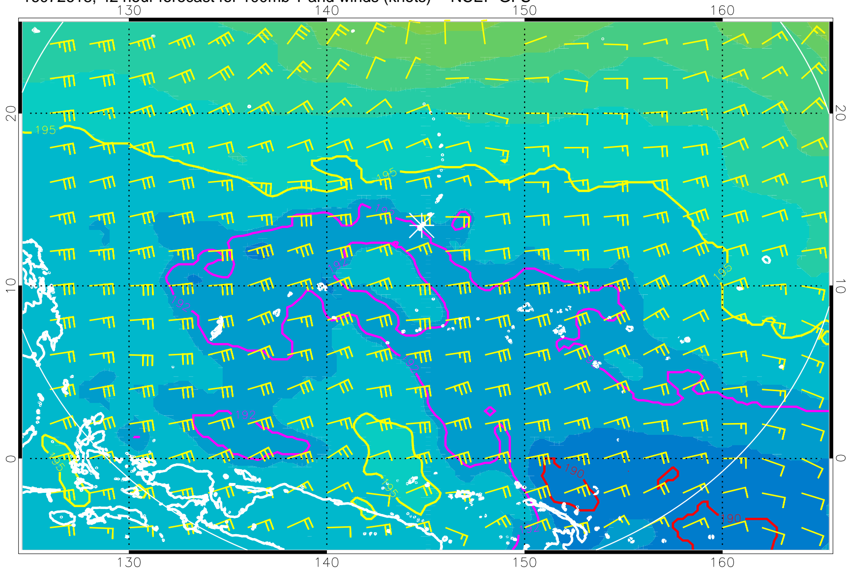
16072618, 42 hour forecast for 100mb T and winds (knots) -- NCEP GFS
