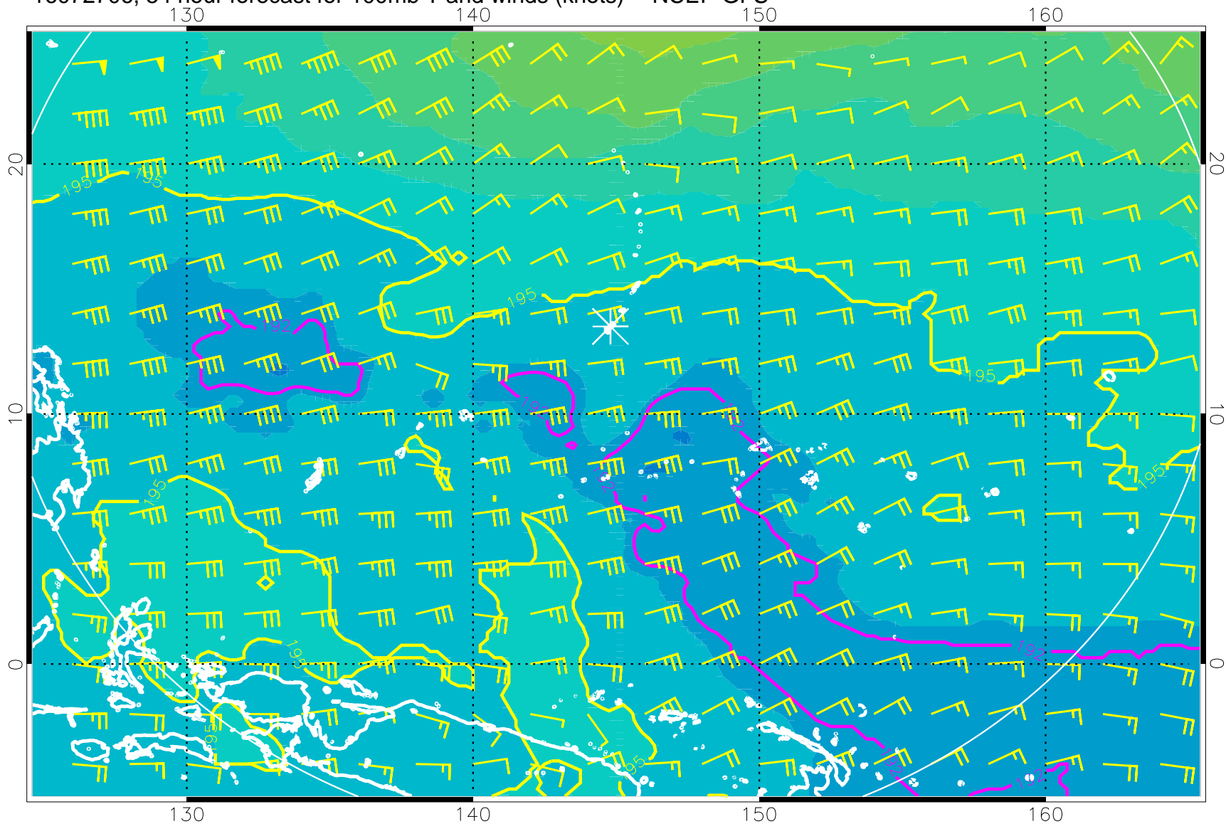
16072706, 54 hour forecast for 100mb T and winds (knots) -- NCEP GFS
