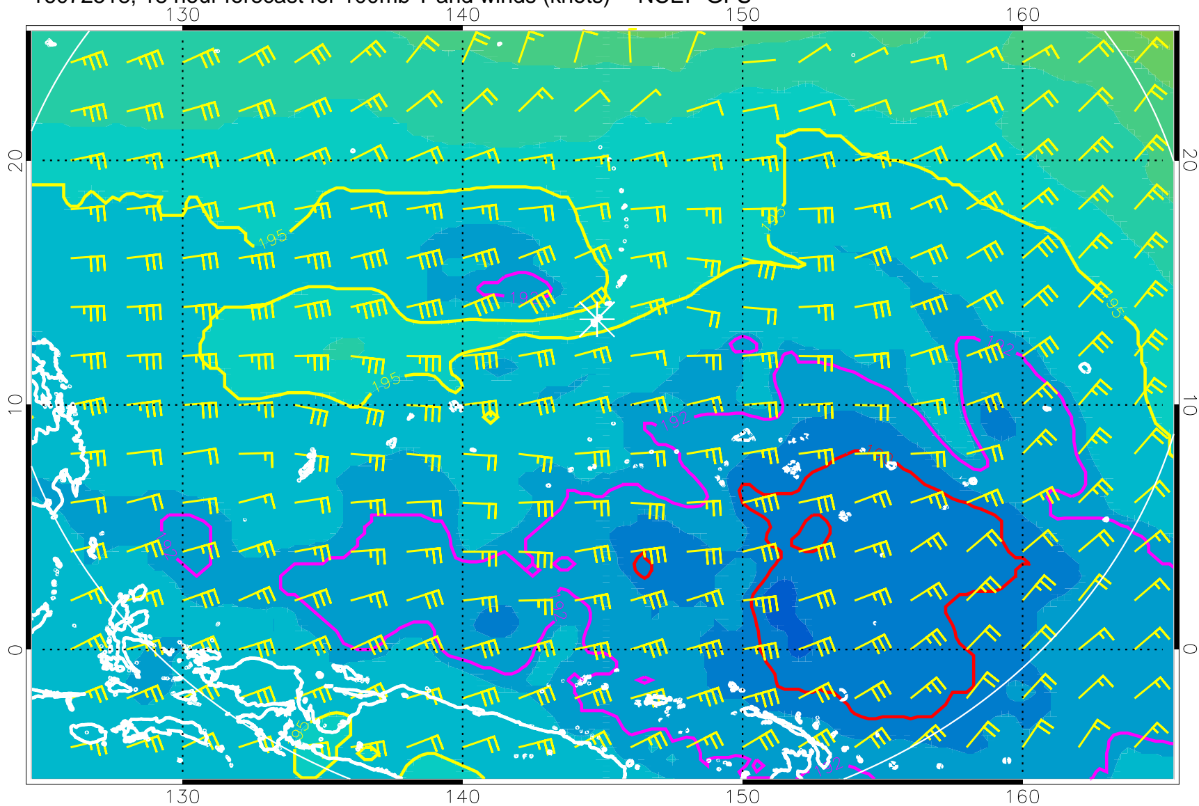
16072518, 18 hour forecast for 100mb T and winds (knots) -- NCEP GFS
