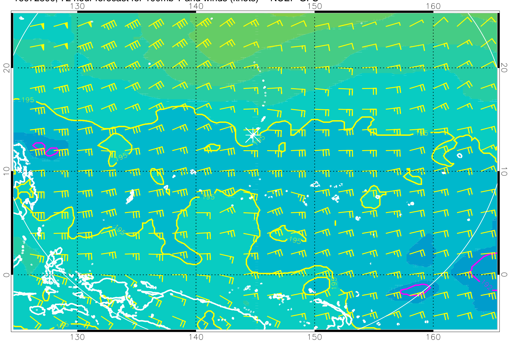
16072800, 72 hour forecast for 100mb T and winds (knots) -- NCEP GFS
