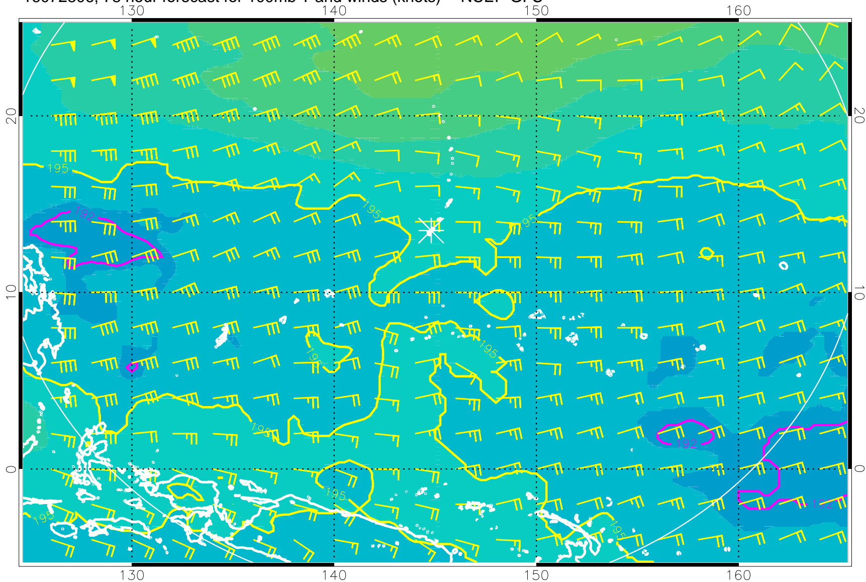
16072806, 78 hour forecast for 100mb T and winds (knots) -- NCEP GFS
