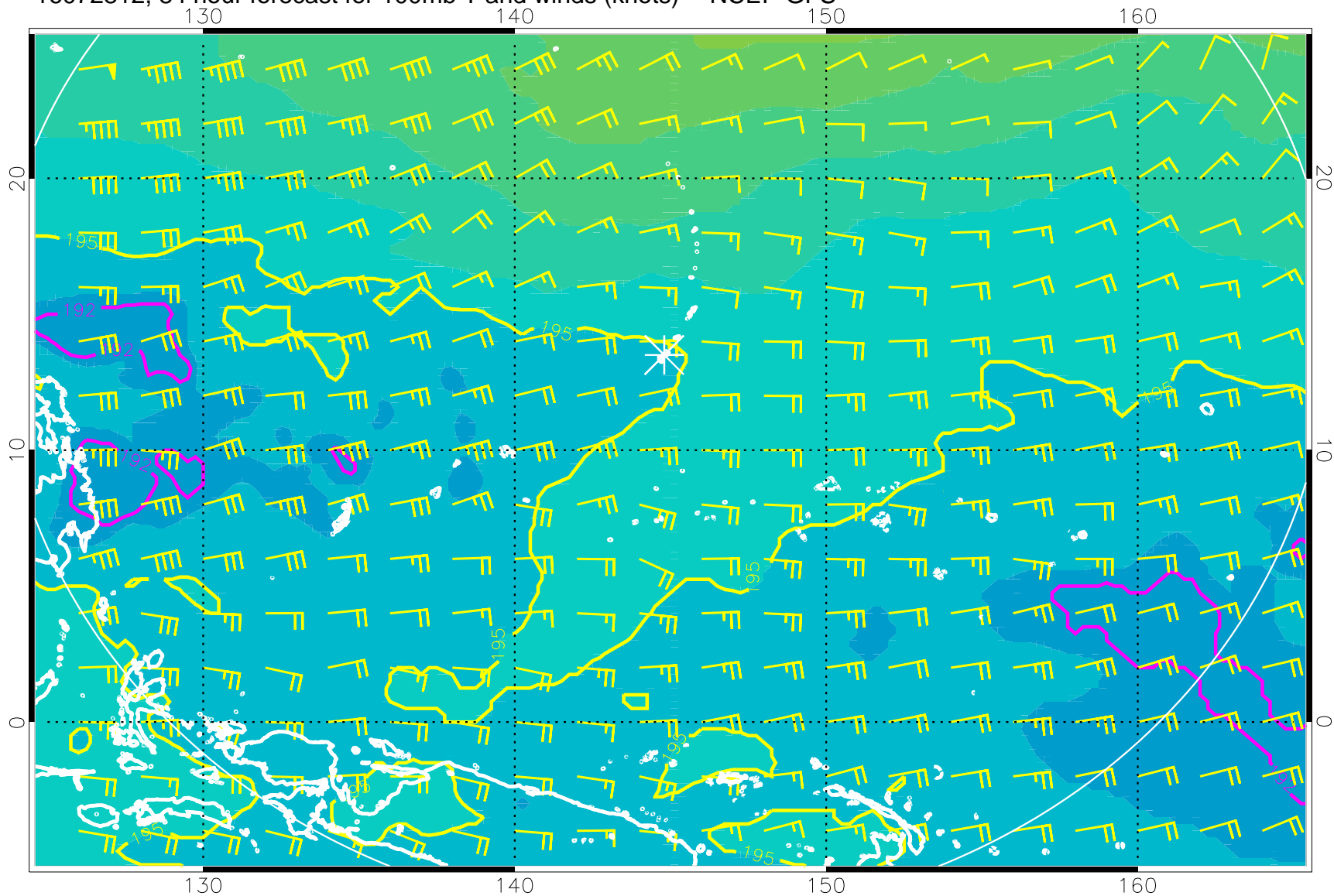
16072812, 84 hour forecast for 100mb T and winds (knots) -- NCEP GFS
