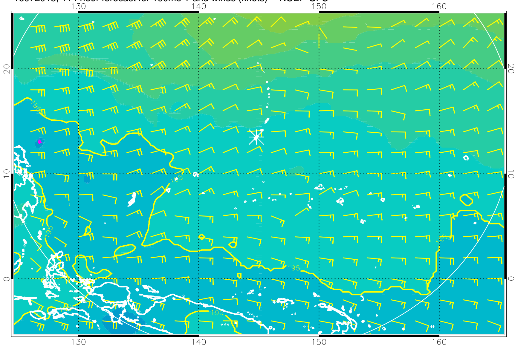
16072918, 114 hour forecast for 100mb T and winds (knots) -- NCEP GFS
