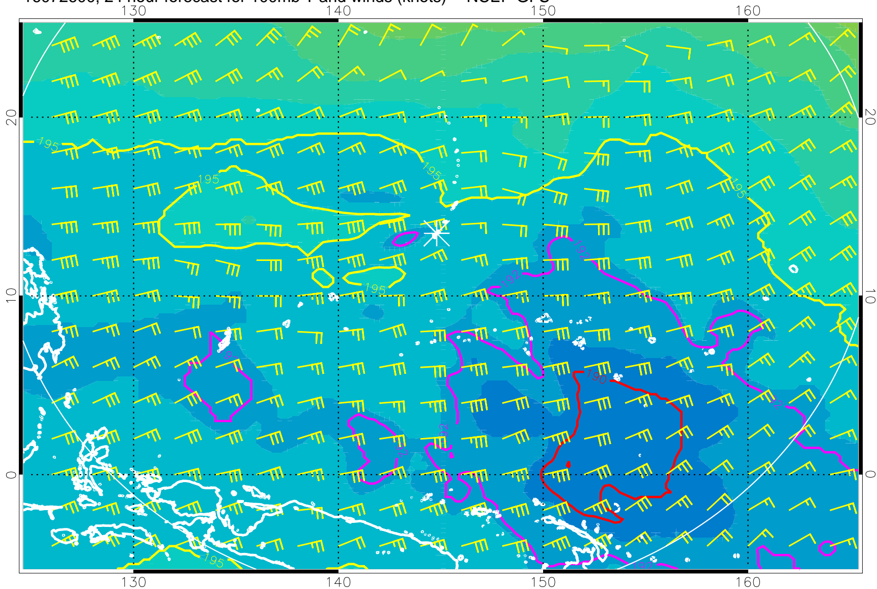
16072600, 24 hour forecast for 100mb T and winds (knots) -- NCEP GFS
