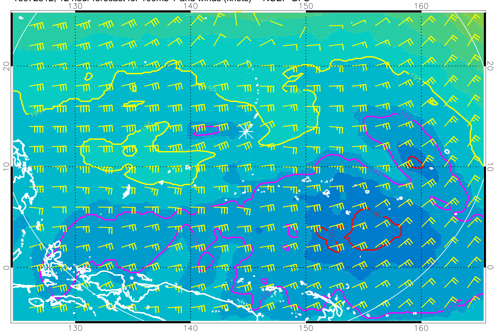
16072512, 12 hour forecast for 100mb T and winds (knots) -- NCEP GFS
