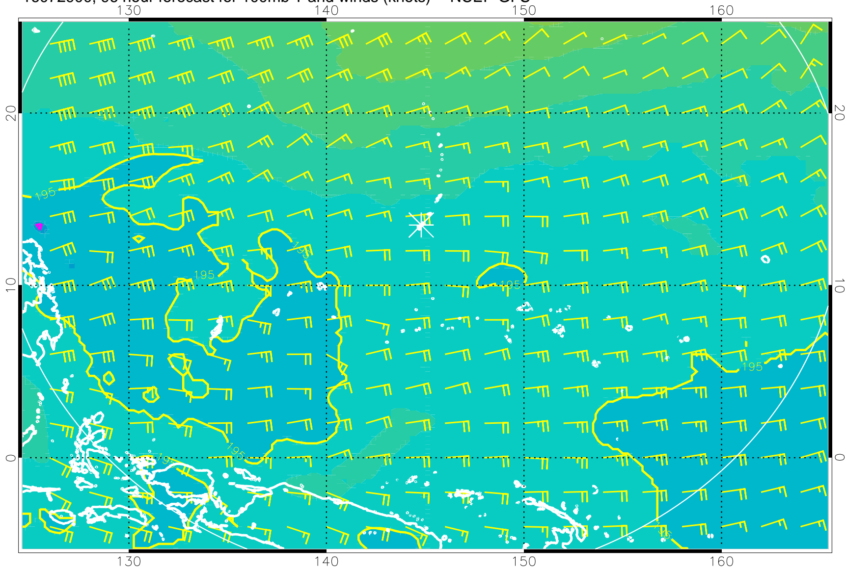
16072900, 96 hour forecast for 100mb T and winds (knots) -- NCEP GFS
