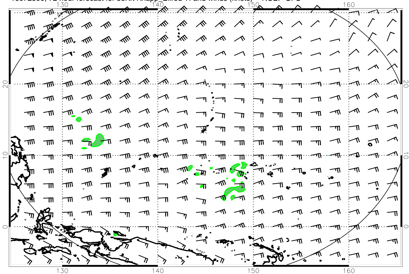
16072800, 72 hour forecast for 53Kft Knapp_Ellrod TI and winds (knots) -- NCEP GFS
