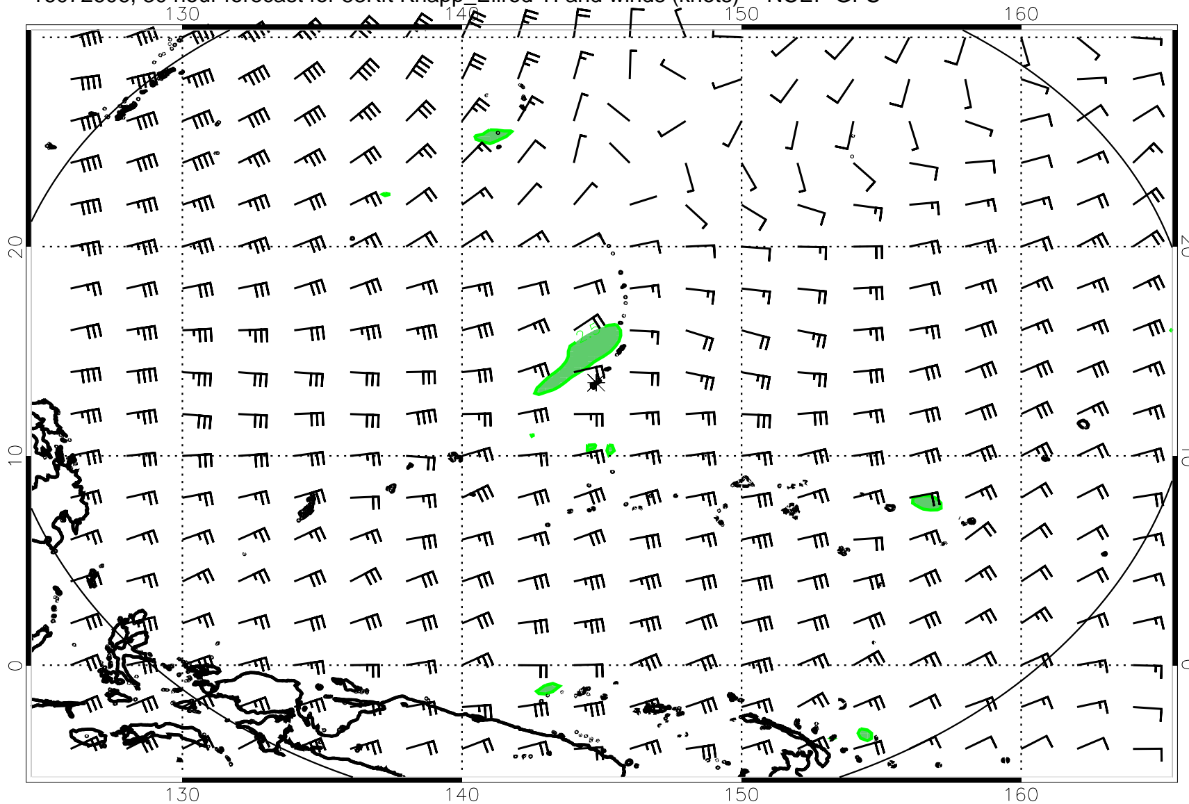
16072606, 30 hour forecast for 53Kft Knapp_Ellrod TI and winds (knots) -- NCEP GFS
