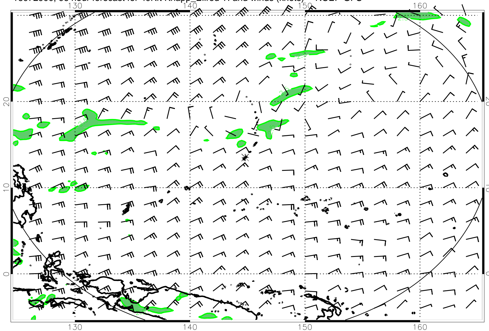
16072900, 96 hour forecast for 49Kft Knapp_Ellrod TI and winds (knots) -- NCEP GFS
