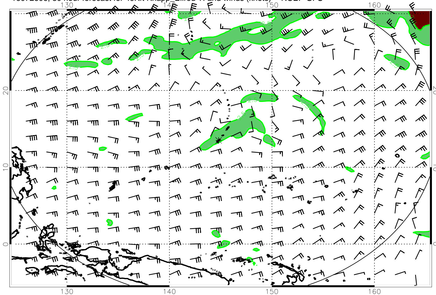
16072606, 30 hour forecast for 49Kft Knapp_Ellrod TI and winds (knots) -- NCEP GFS
