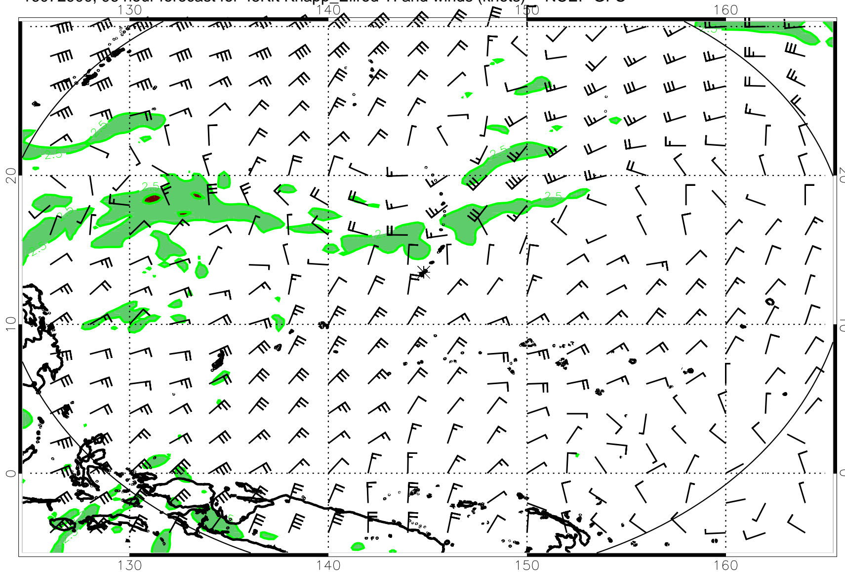
16072900, 96 hour forecast for 45Kft Knapp_Ellrod TI and winds (knots) -- NCEP GFS
