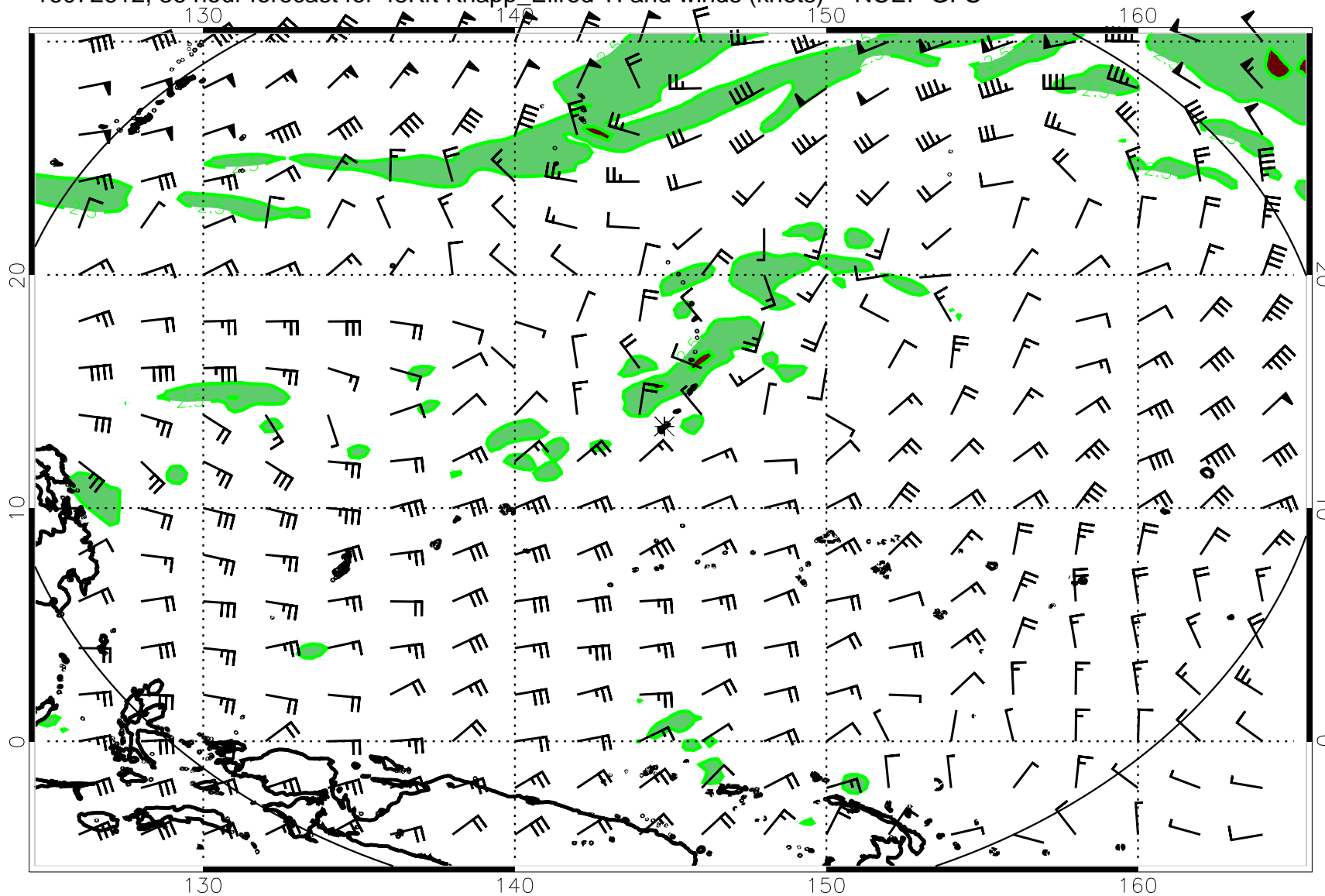
16072612, 36 hour forecast for 45Kft Knapp_Ellrod TI and winds (knots) -- NCEP GFS
