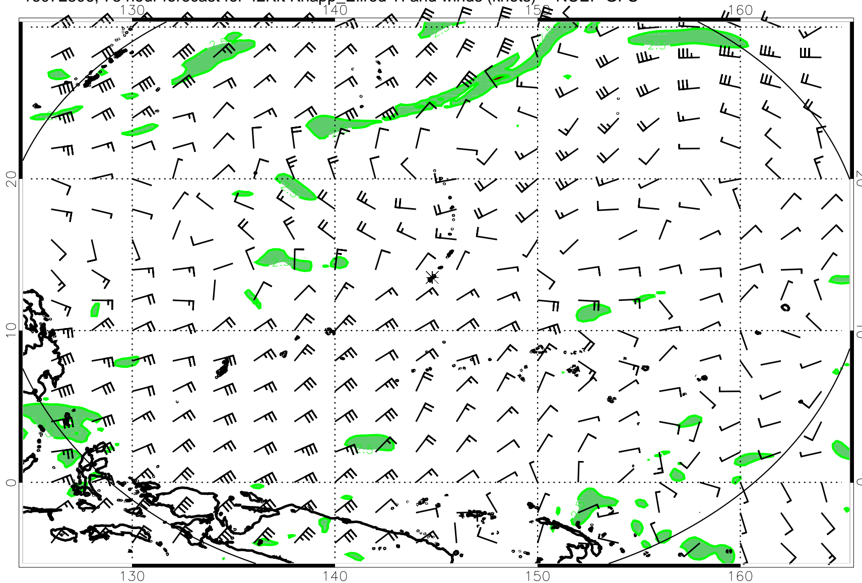
16072806, 78 hour forecast for 42Kft Knapp_Ellrod TI and winds (knots) -- NCEP GFS
