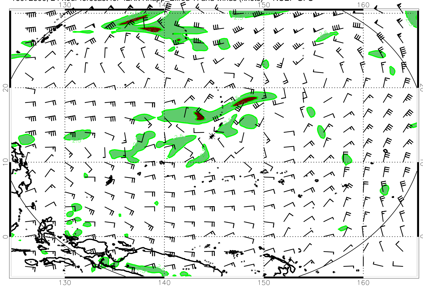
16072600, 24 hour forecast for 42Kft Knapp_Ellrod TI and winds (knots) -- NCEP GFS
