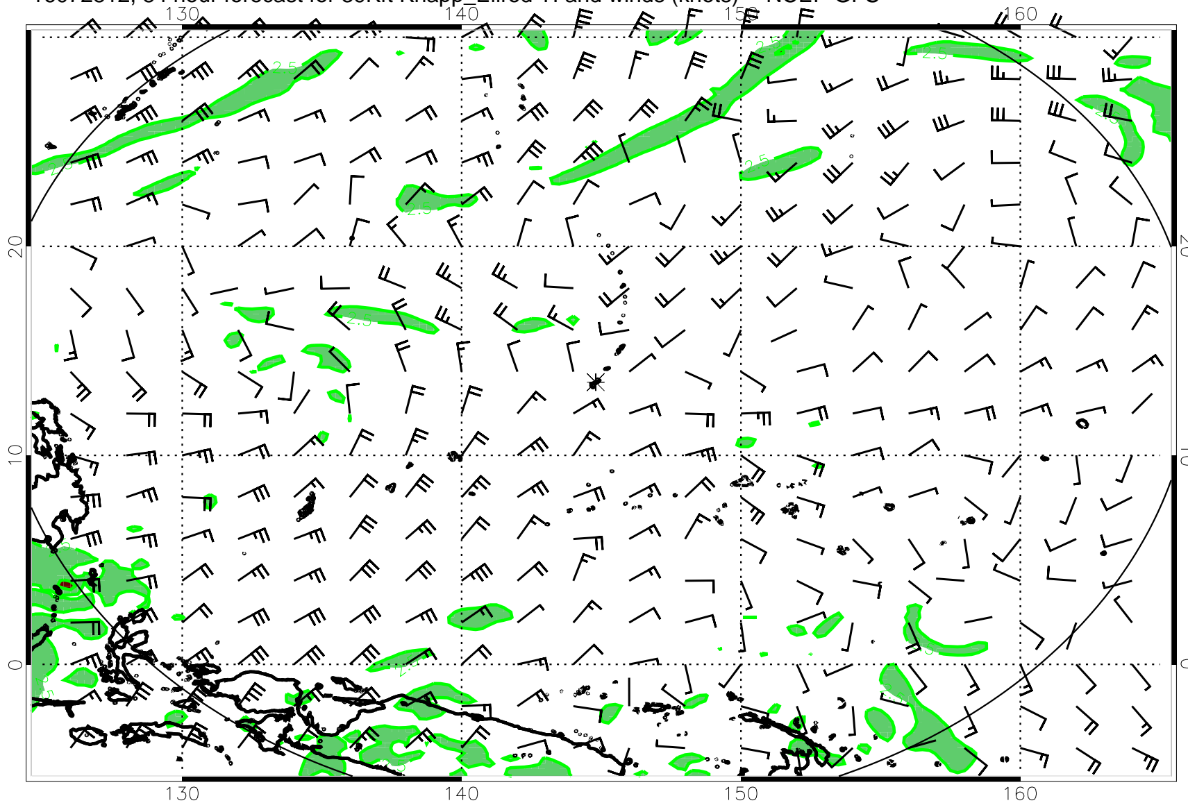
16072812, 84 hour forecast for 39Kft Knapp_Ellrod TI and winds (knots) -- NCEP GFS
