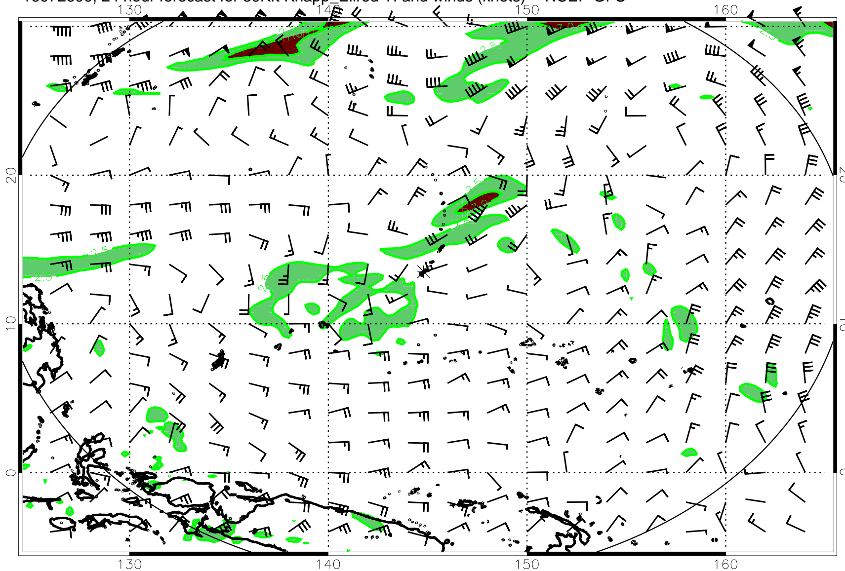
16072600, 24 hour forecast for 39Kft Knapp_Ellrod TI and winds (knots) -- NCEP GFS
